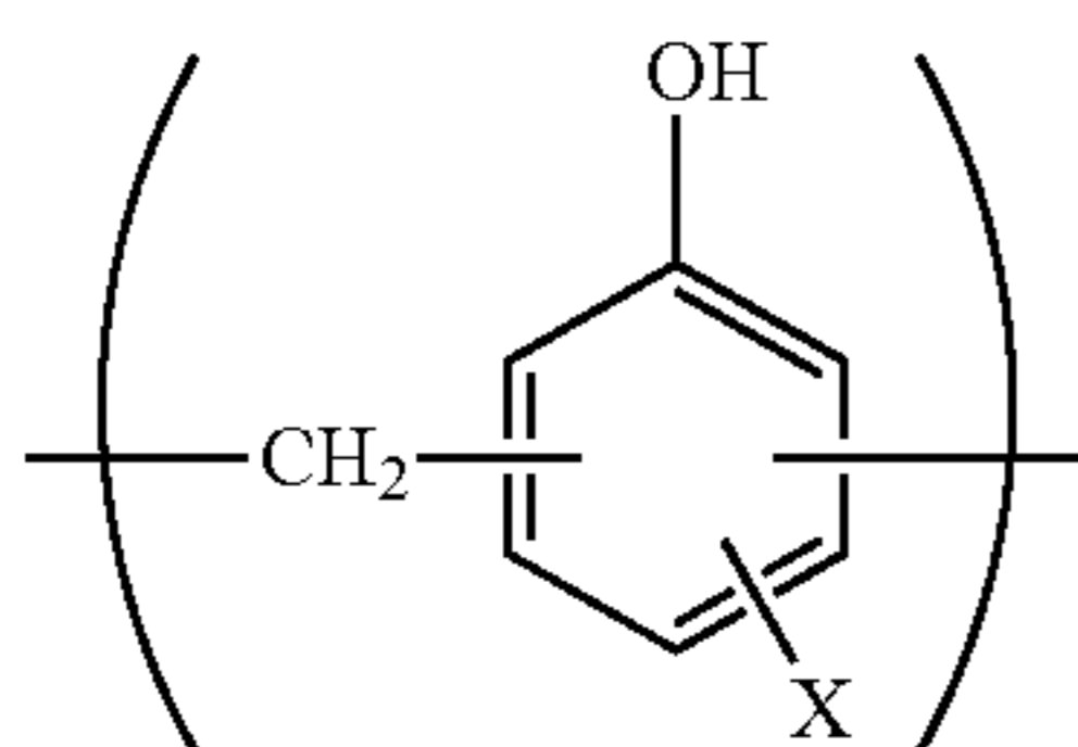
[Chemical Formula 1]
