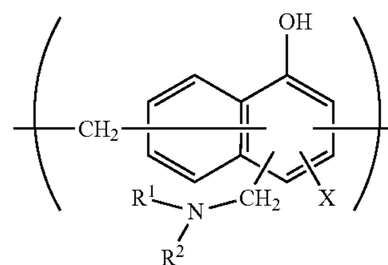
[Chemical Formula 4]
