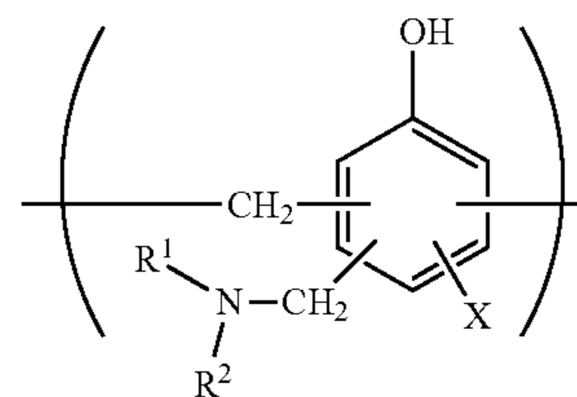
[Chemical Formula 3]
