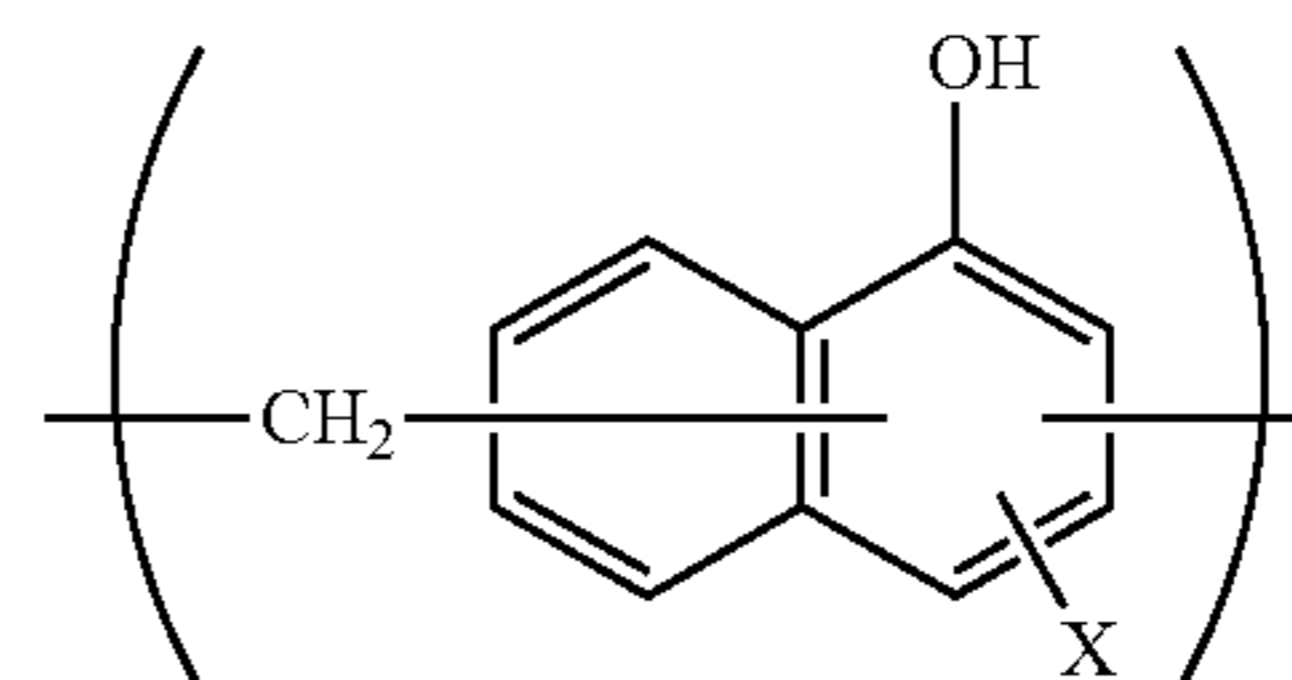
[Chemical Formula 4]
