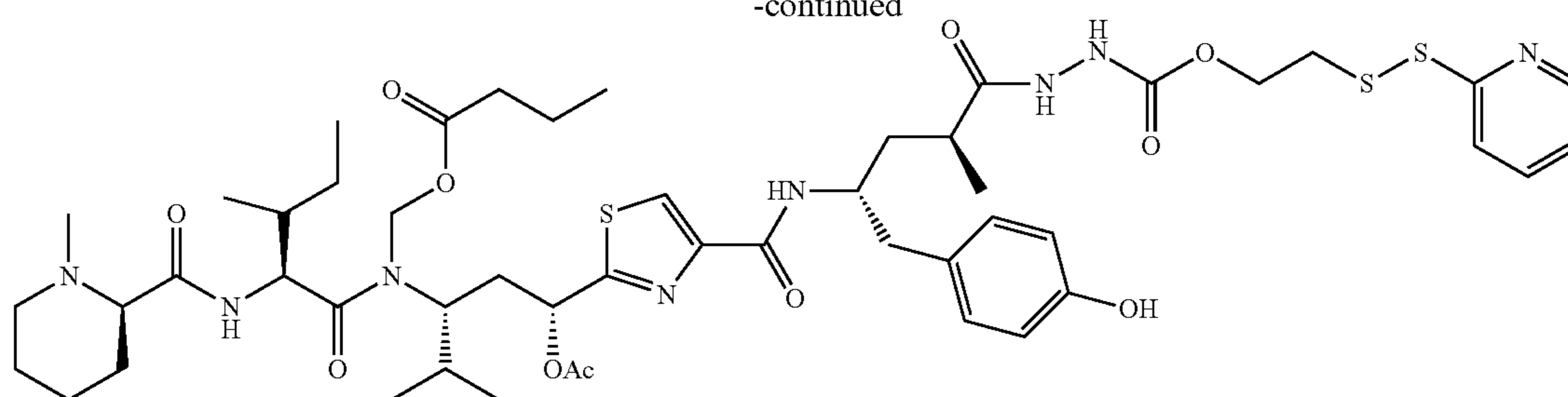
EC0312 C_{50}H_{72}N_8O_{11}S_3 Mol. Wt.: 1057.35
