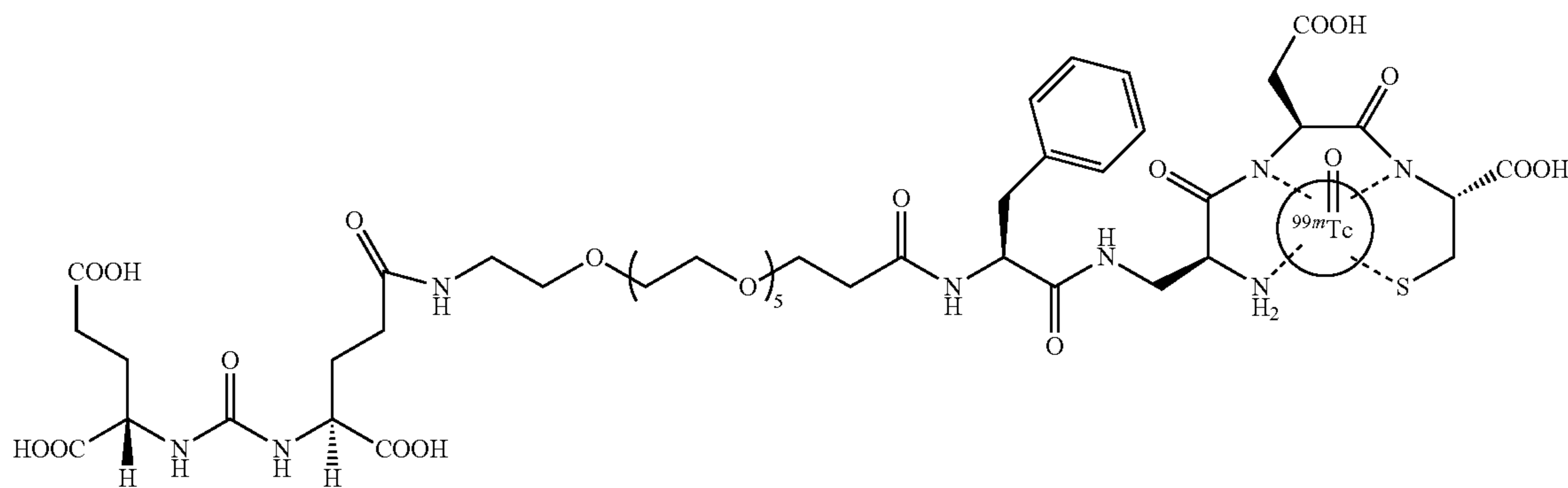
SK57- ^{99m}\text{Tc} (24-atom linker, 1.8 mg)
