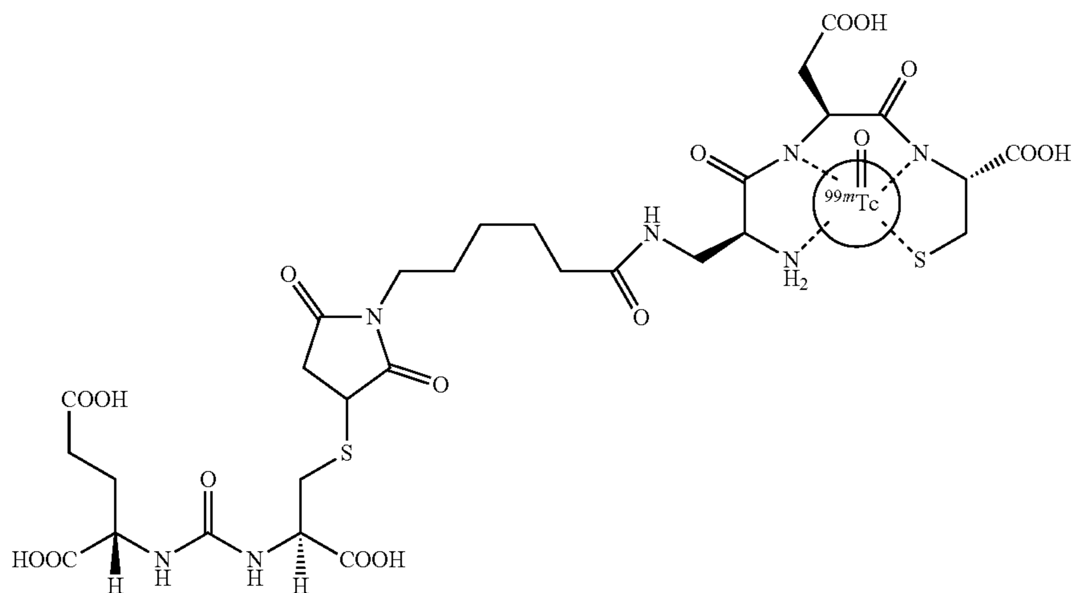
(9-atom linker)
