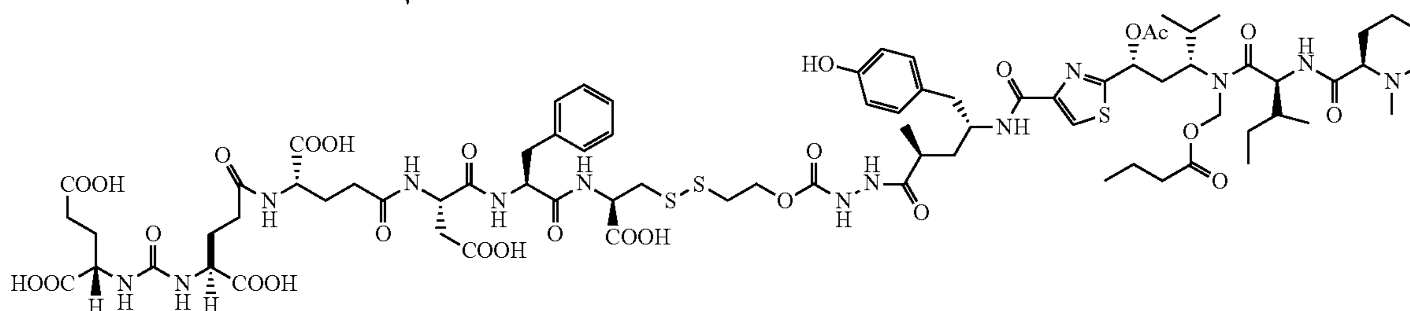
PC01SK71 C_{77}H_{109}N_{13}O_{29}S_3 Mol. Wt.: 1760.95
