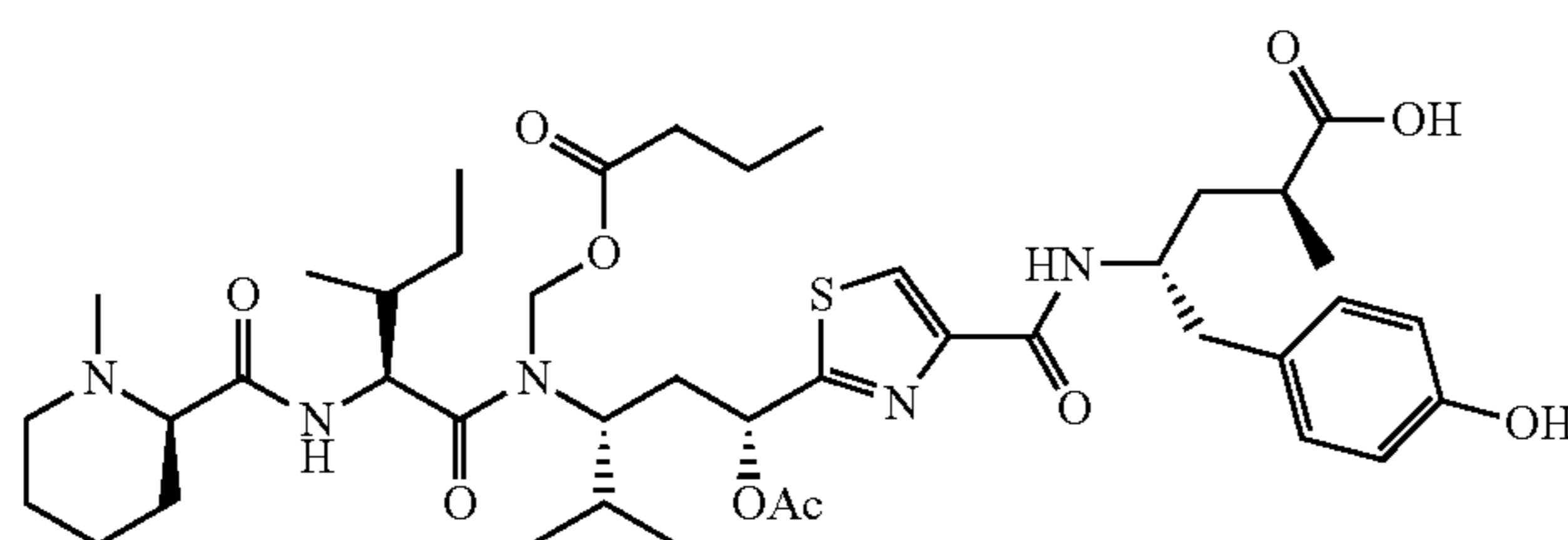
Tubulysin B C_{42}H_{63}N_5O_{10}S Mol. Wt.: 830.04
