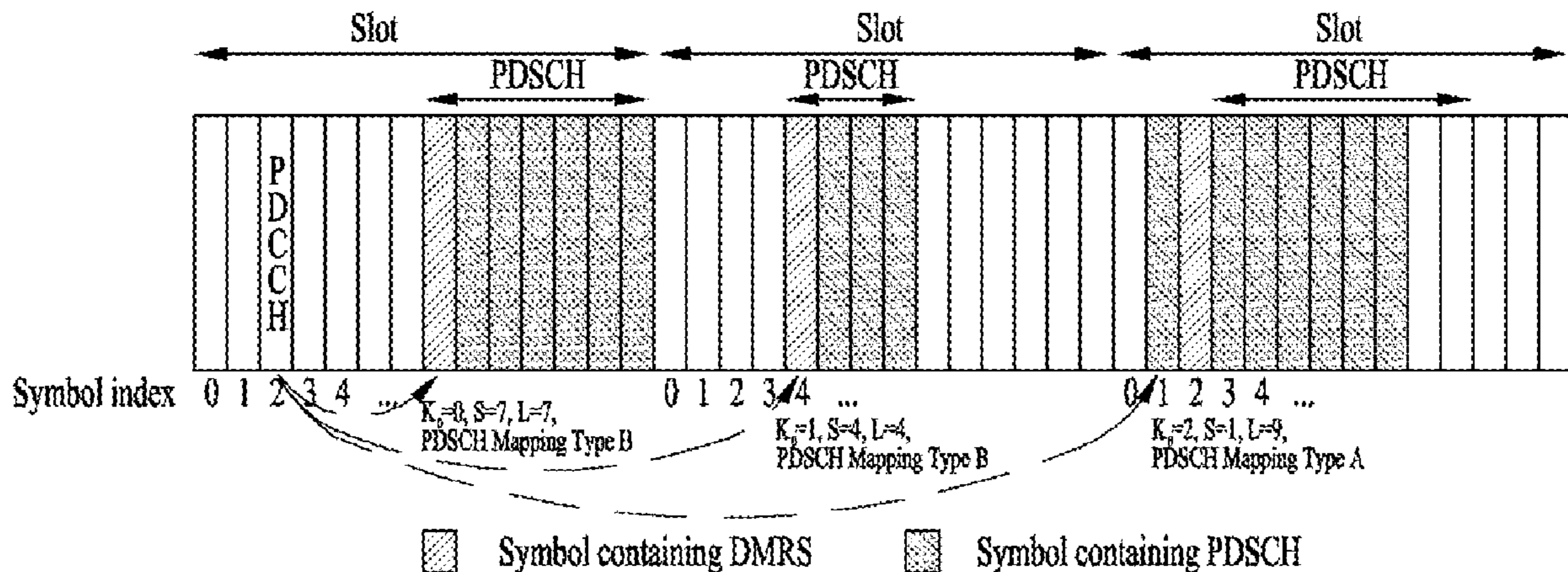
Example of PDSCH time domain resource allocation
