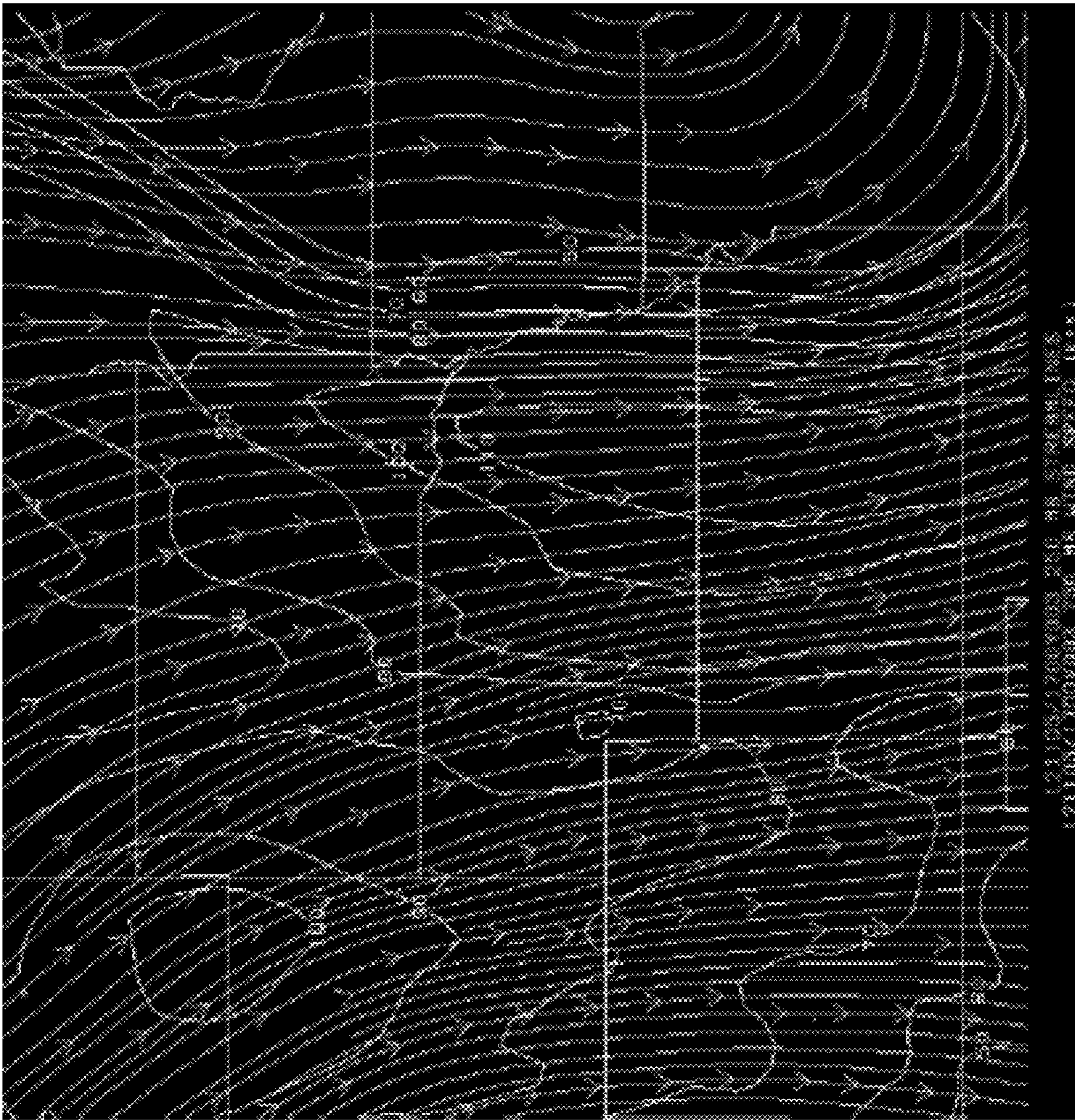
RAP Forecast Streamlines over 3 hour period 11 01
