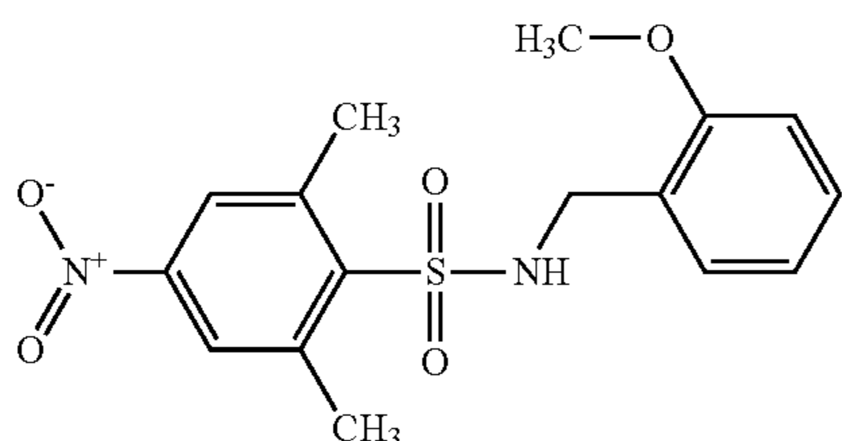
IPUAC: N-[(2-methoxyphenyl)methyl]-2,6-dimethyl-4-nitrobenzene-1-sulfonamide
