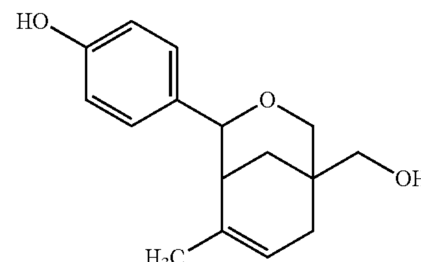
IPUAC: 4-[5-(hydroxymethyl)-2-methyl-7-oxabicyclo[3.3.1]non-2-en-8-yl]phenol
