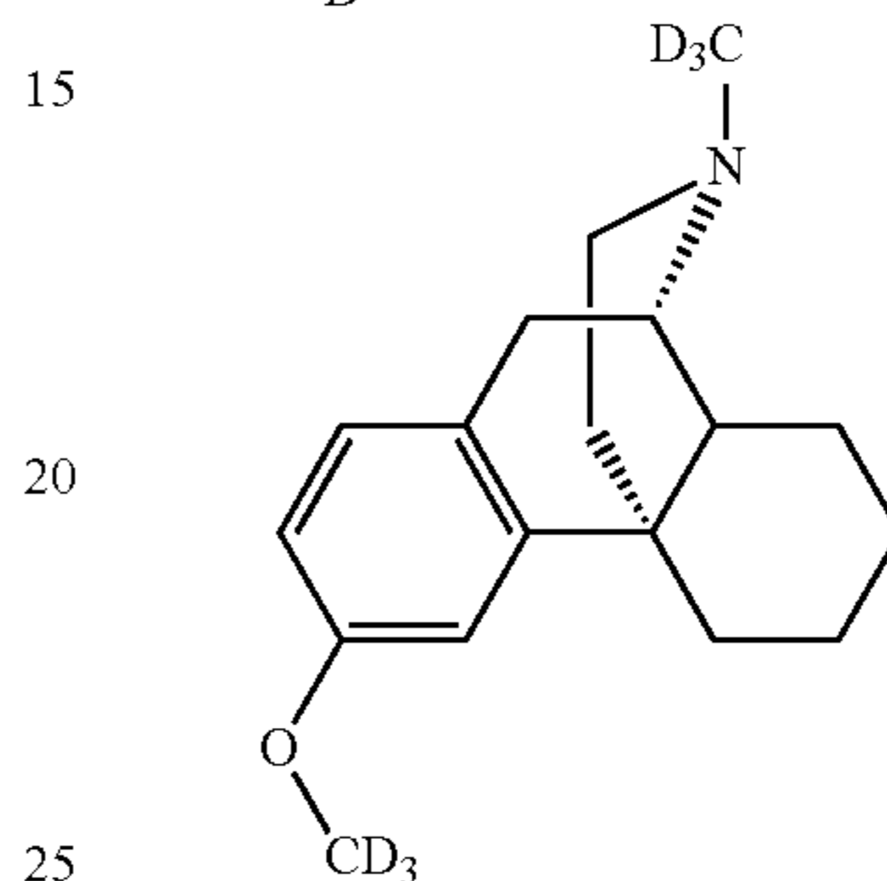
d6-dextromethorphan
