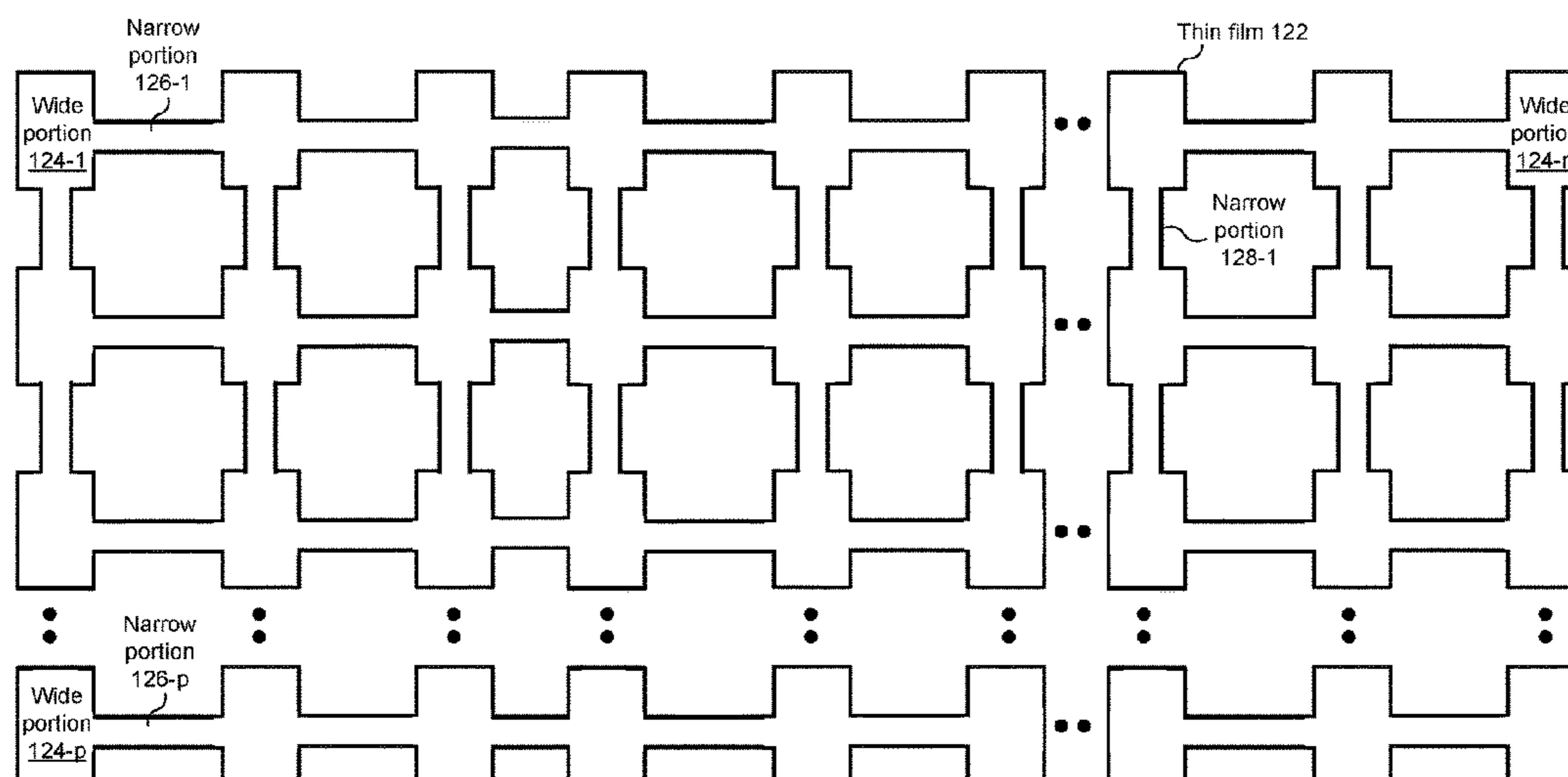
Superconducting Array 120 →
