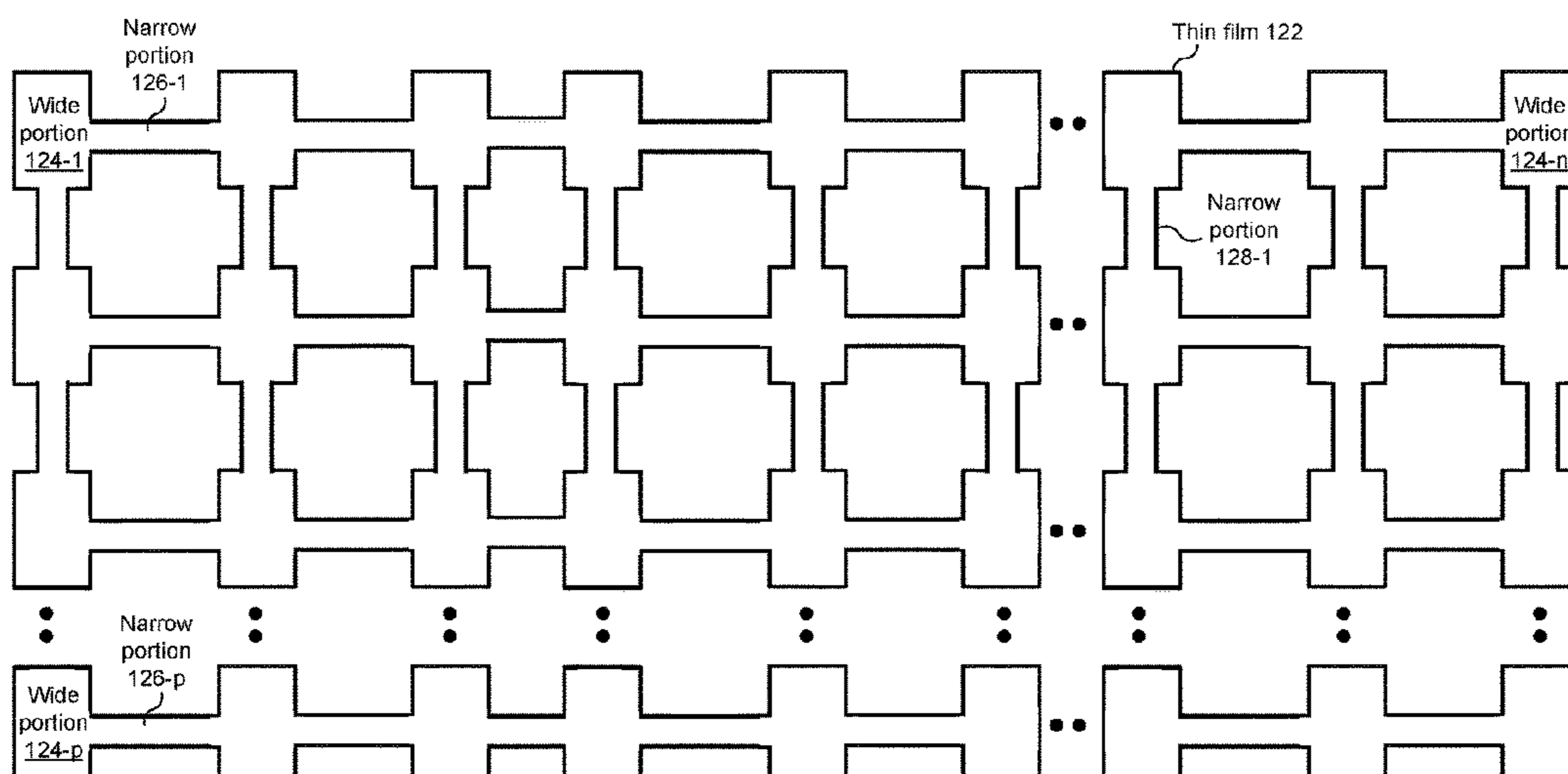
Superconducting Array 120 →
