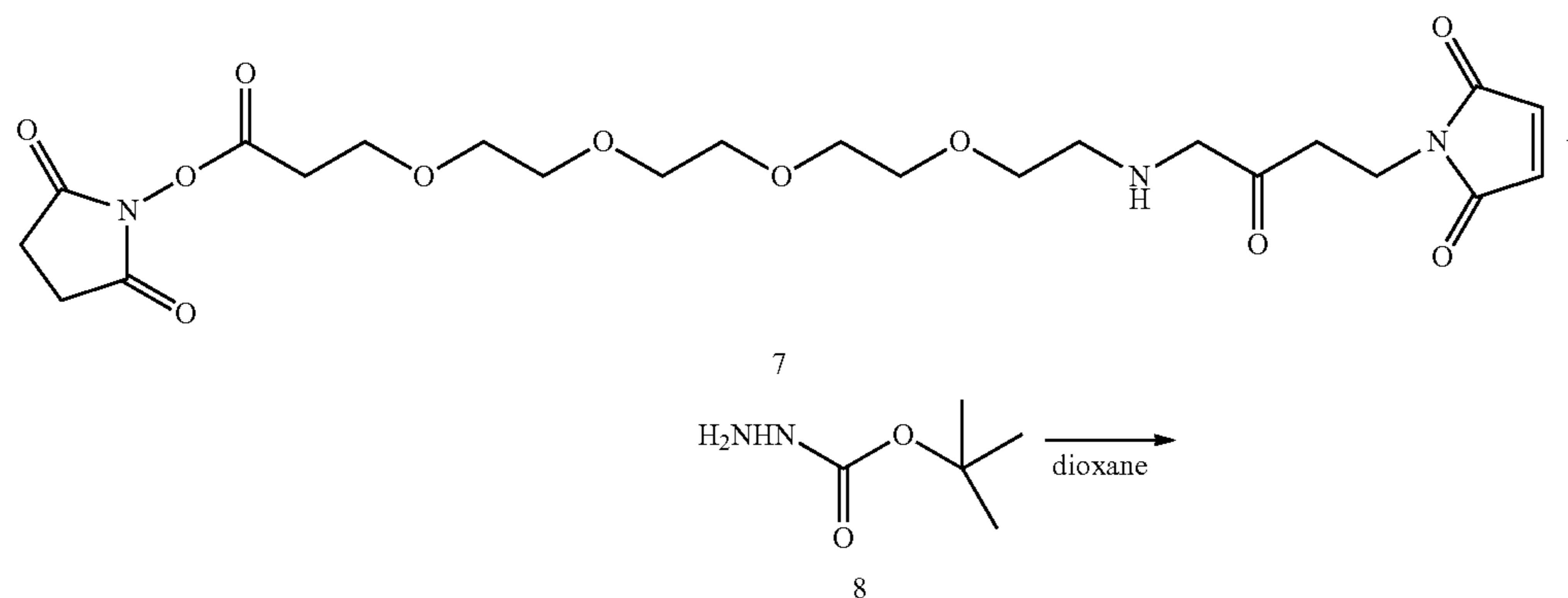
Scheme 7
