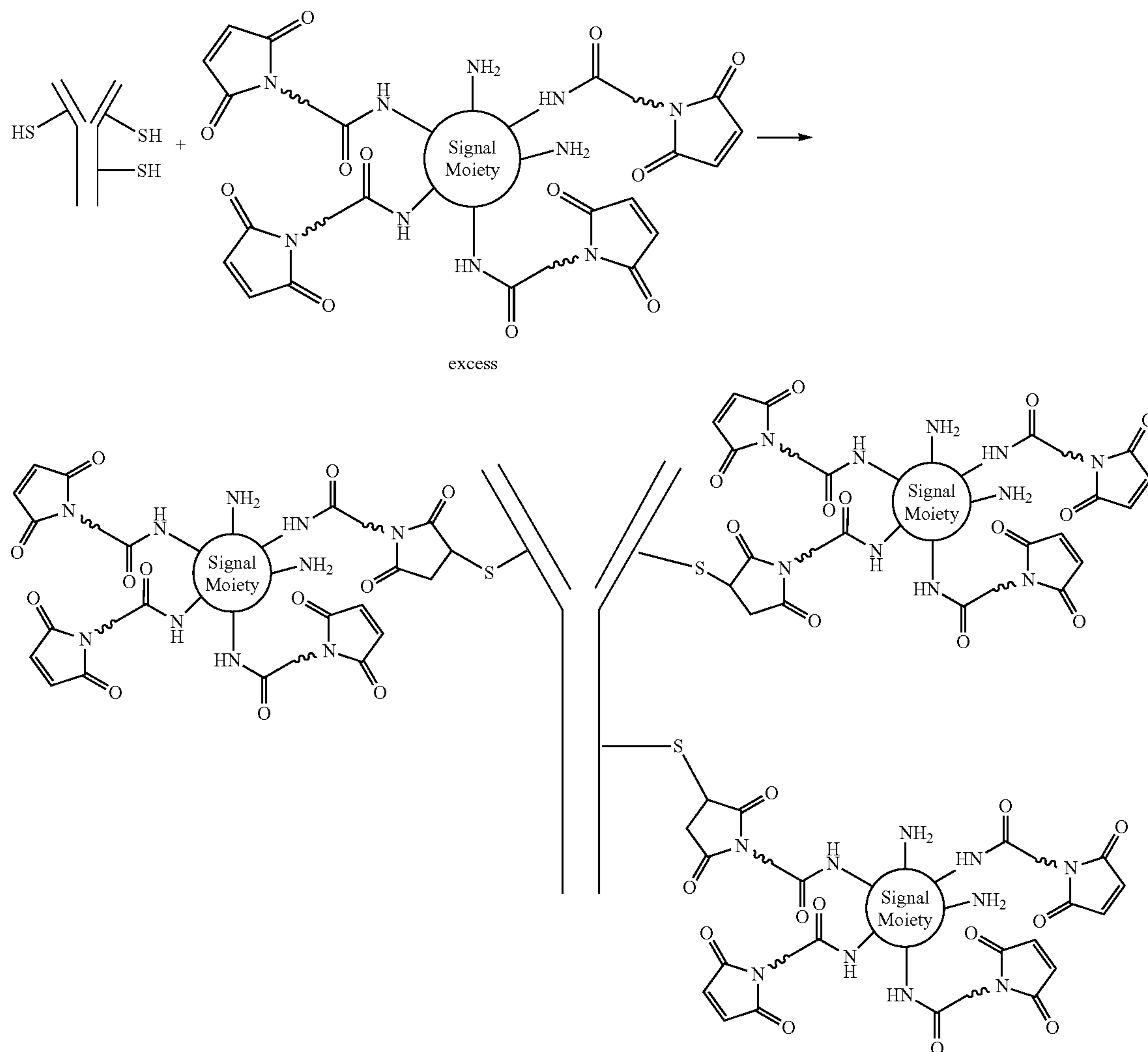
Scheme 3
