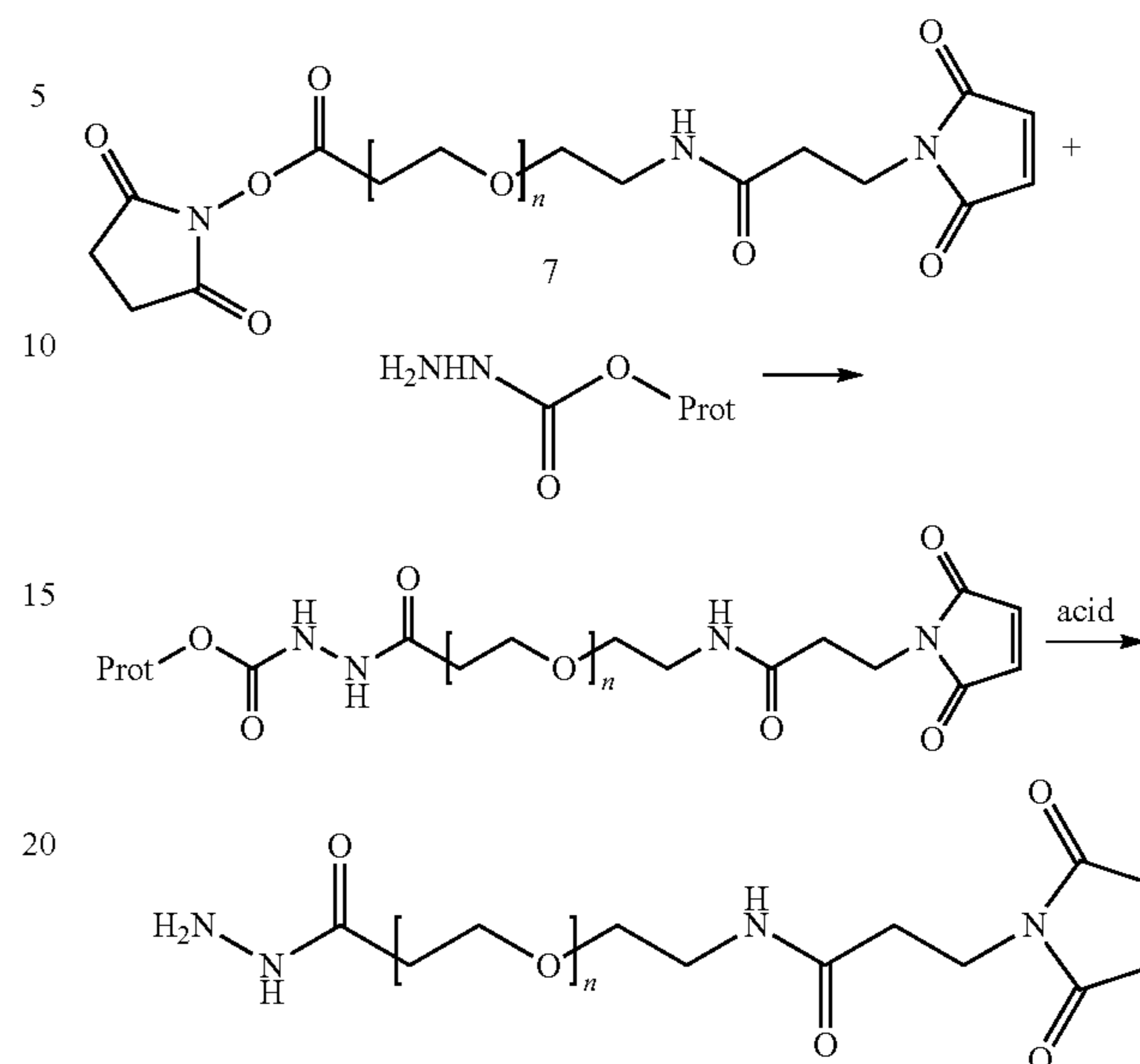
Scheme 6
