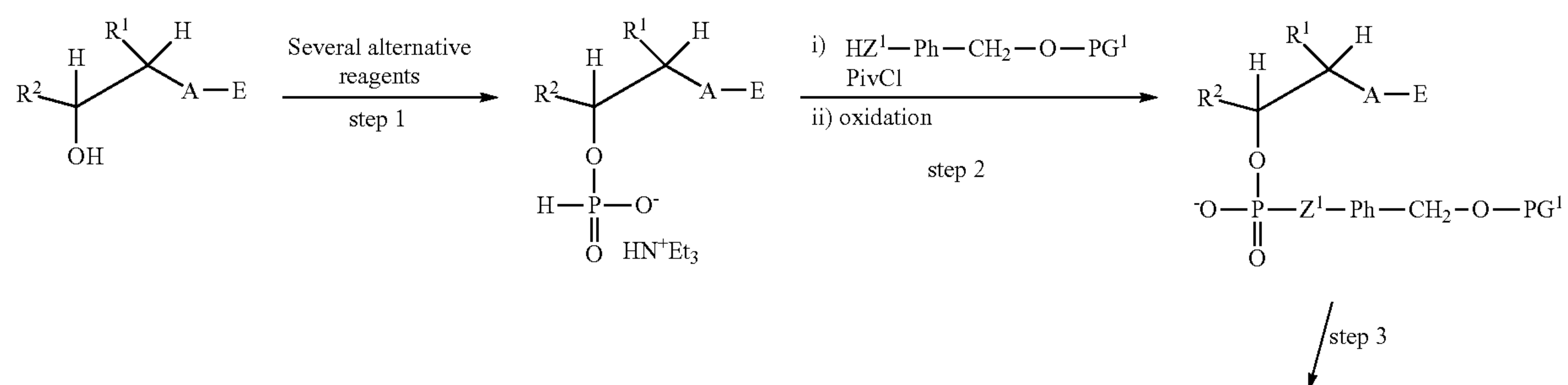
Scheme 15
