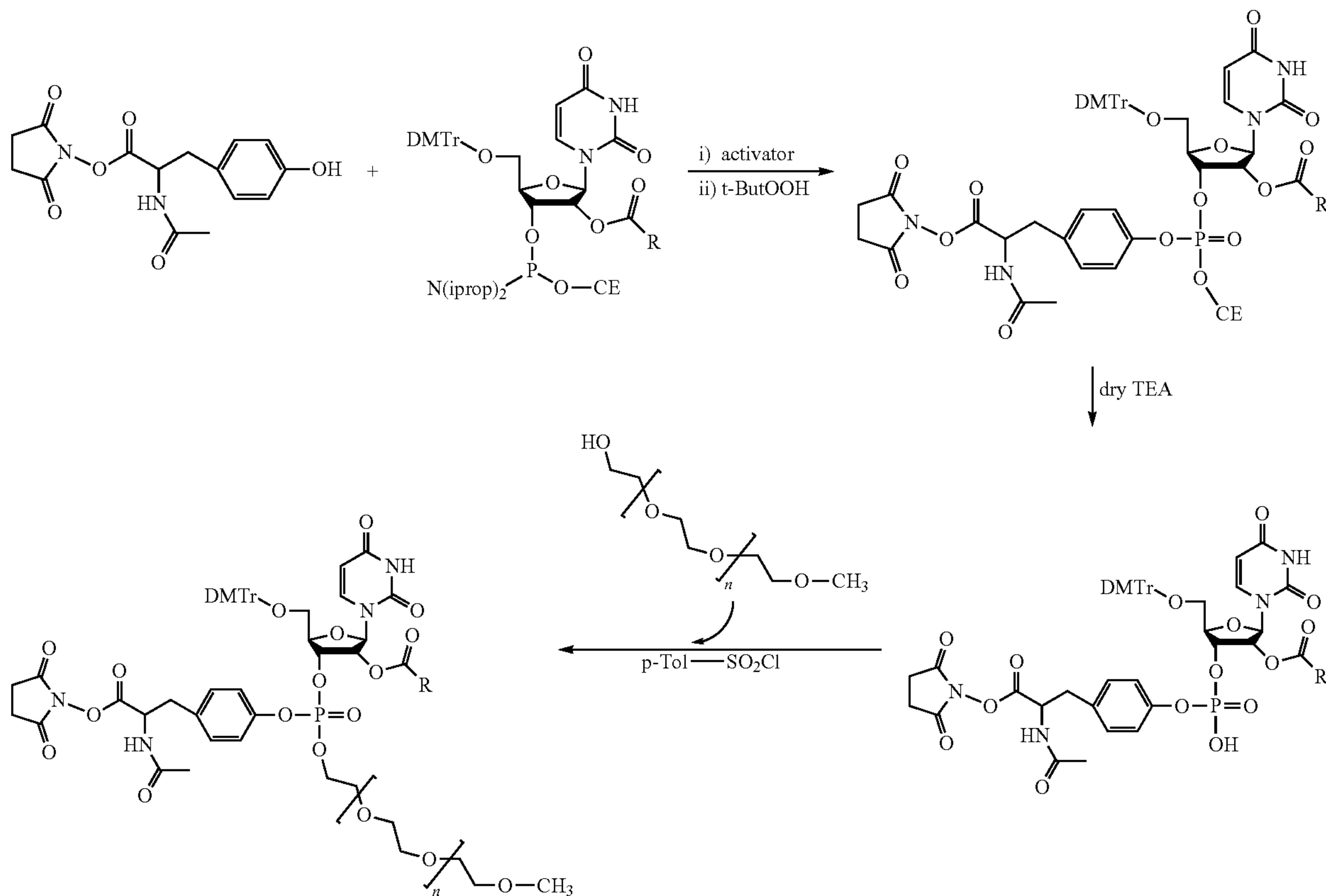
Scheme 17
