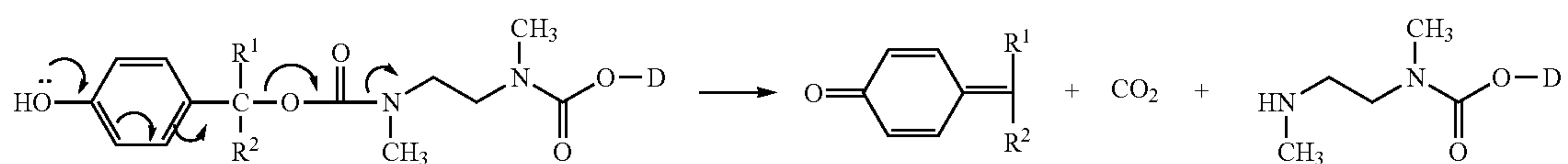
Scheme 7
