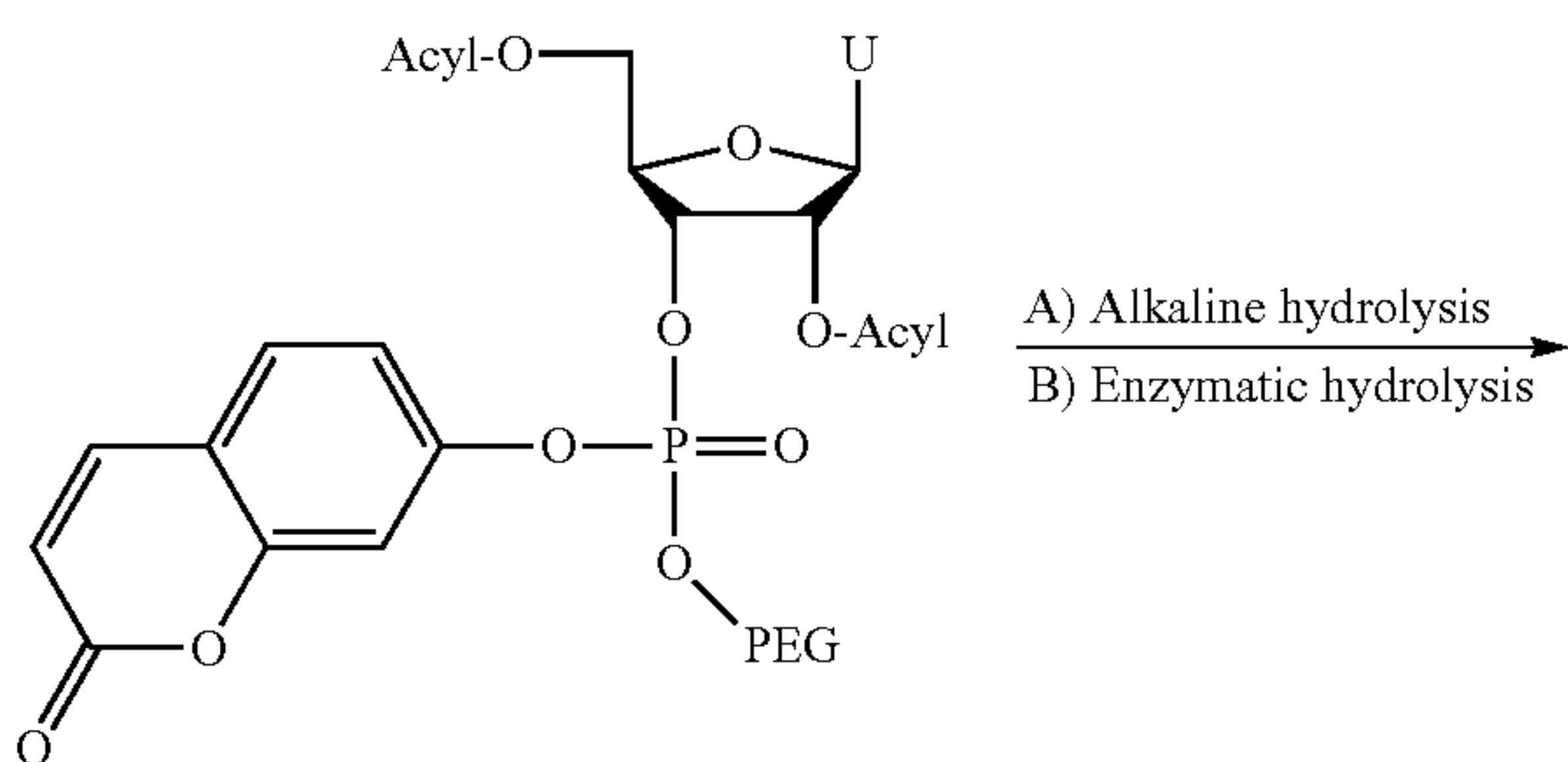
Scheme 10
