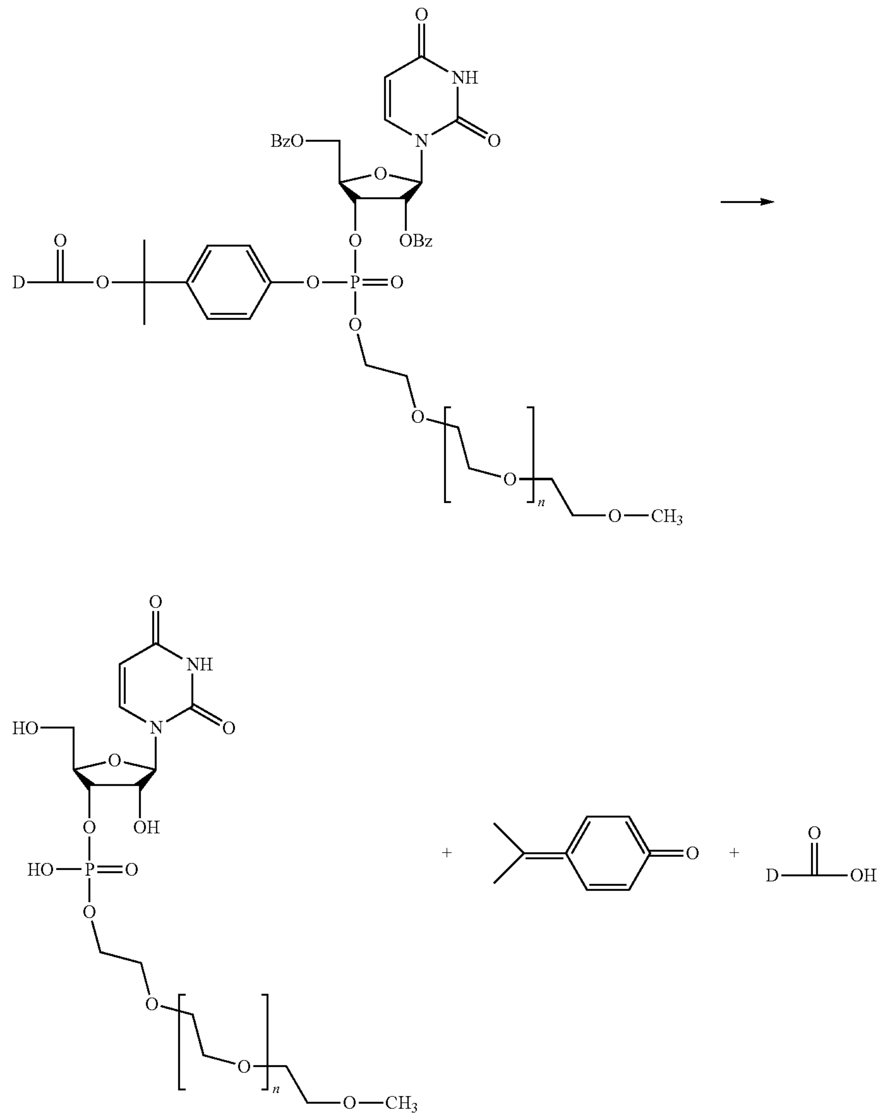
Scheme 6
