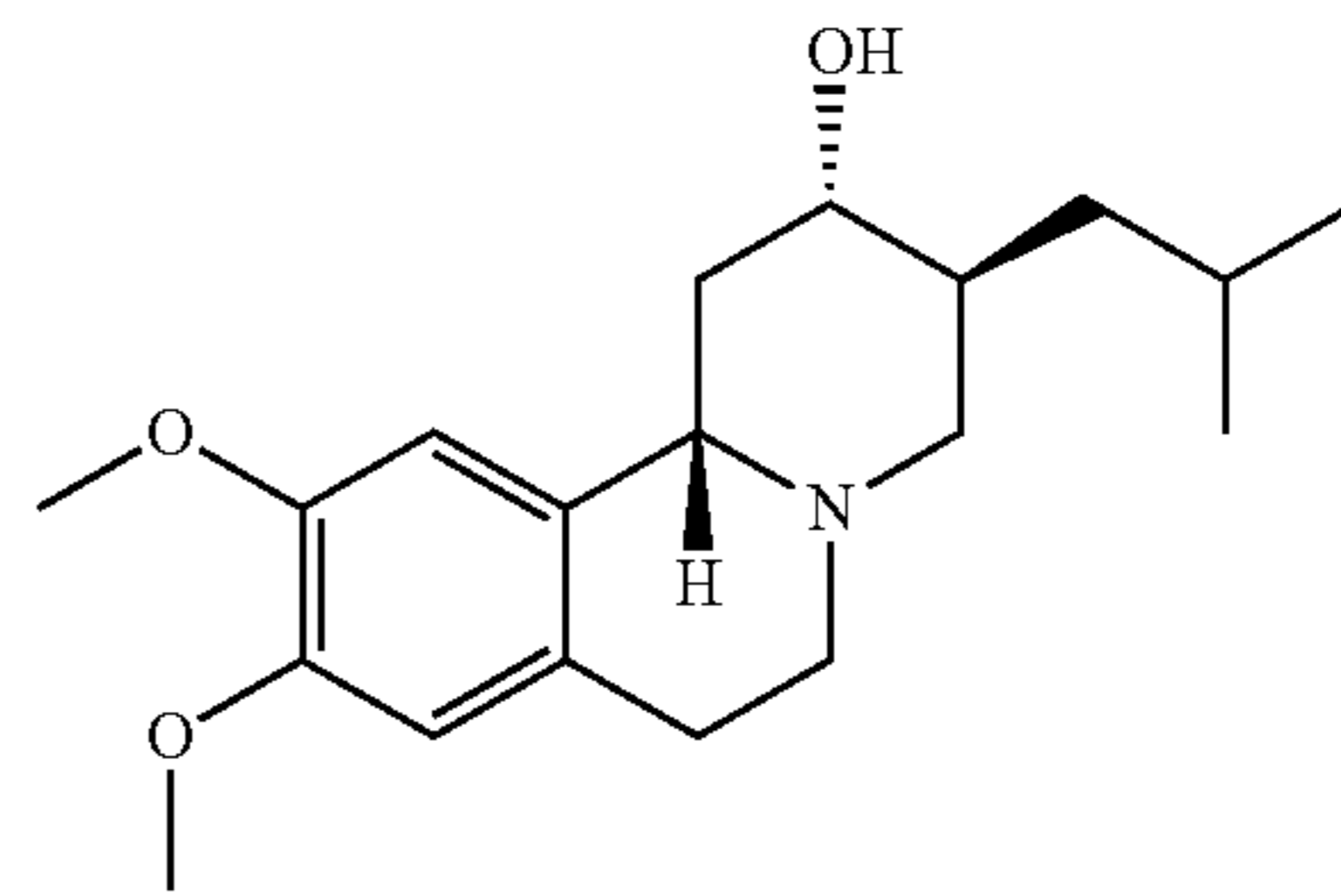
(-)-alpha-dihydrotetraabenazine
