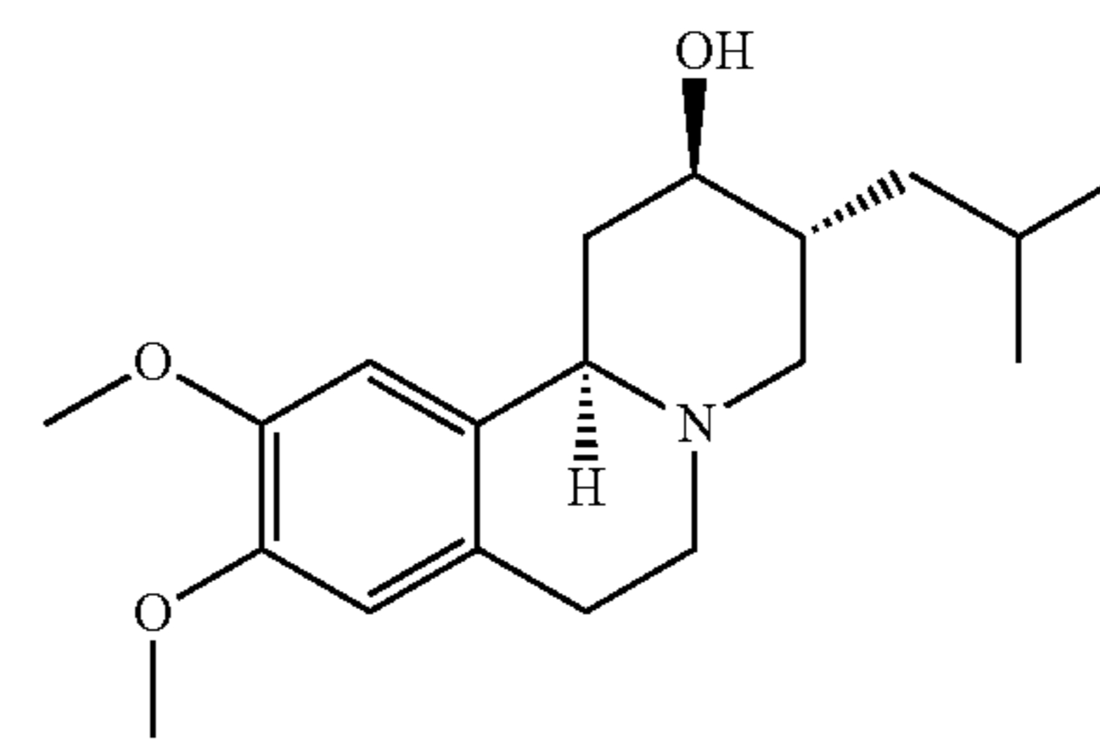
(+)-alpha-dihydrotetraabenazine
