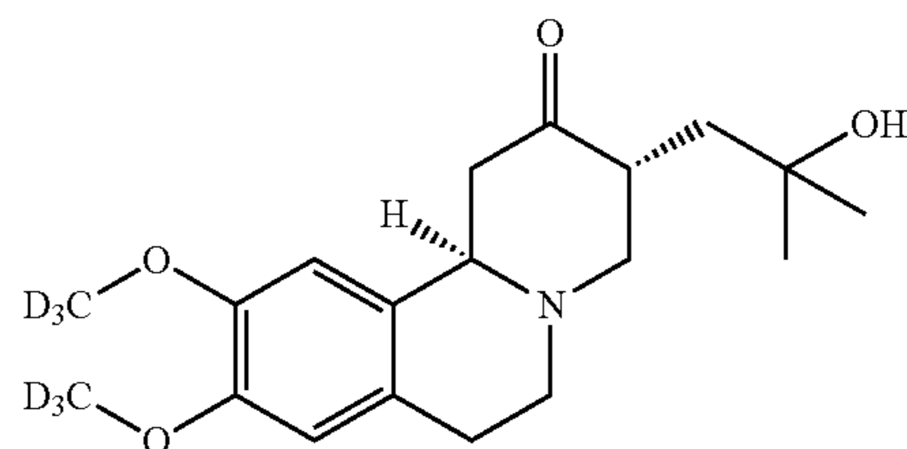
(3R, 11bR)-enantiomer
