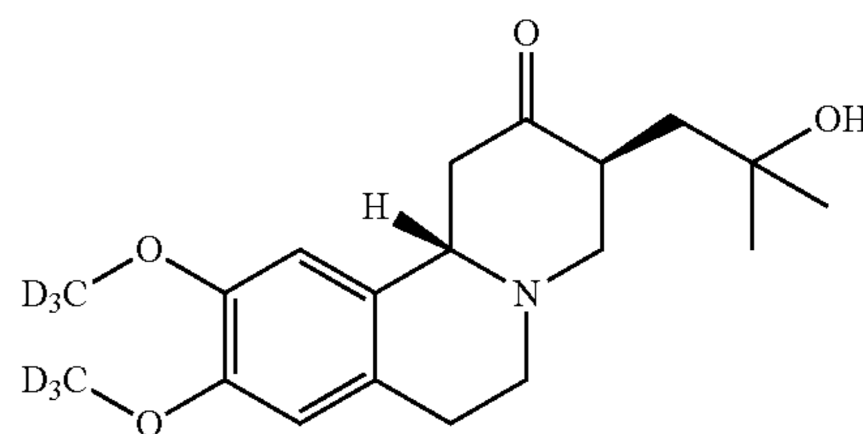
(3S, 11bS)-enantiomer
