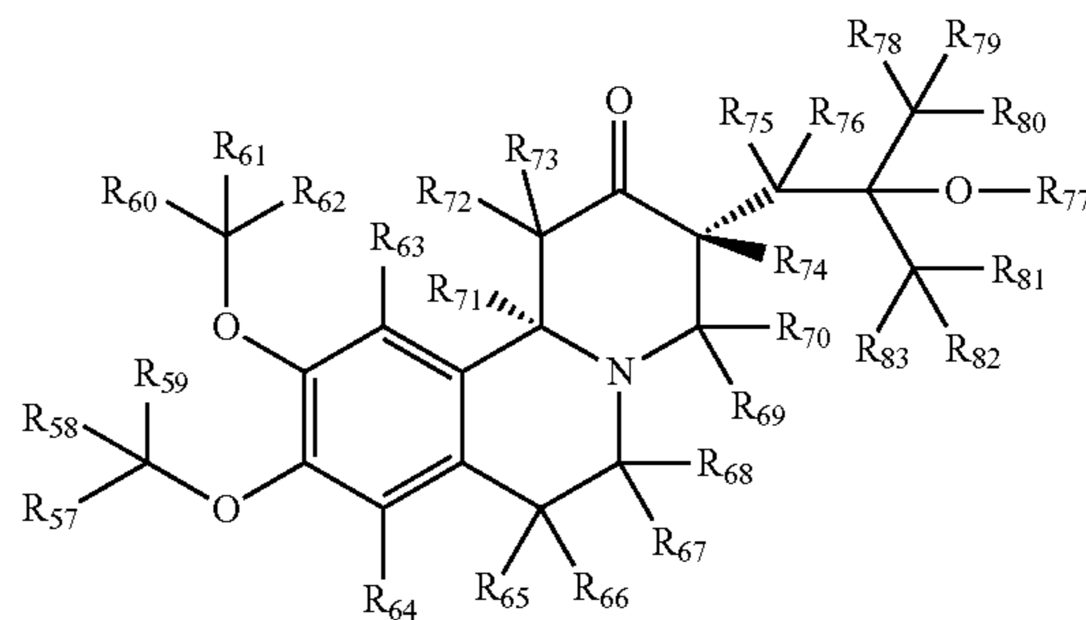
(3R, 11bR)-enantiomer
