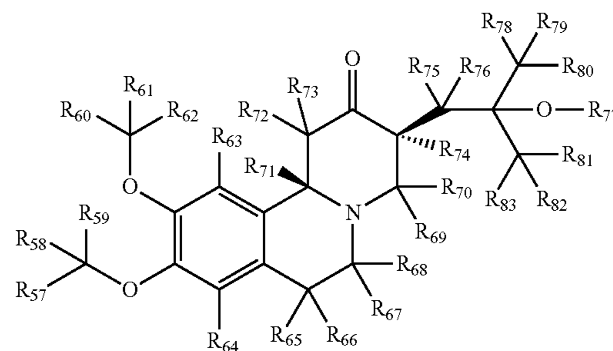
(3S, 11bS)-enantiomer
