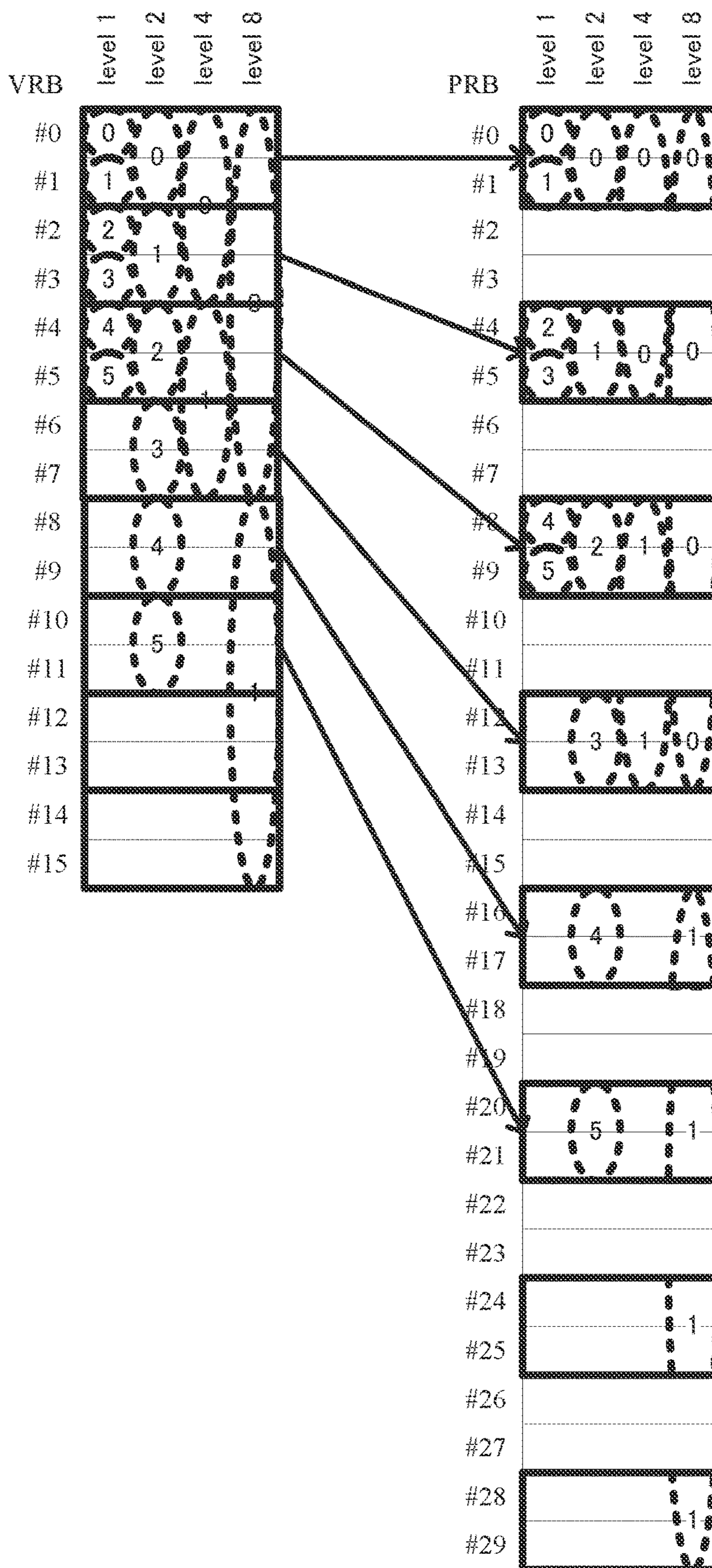
FIG. 2 (PRIOR ART)
