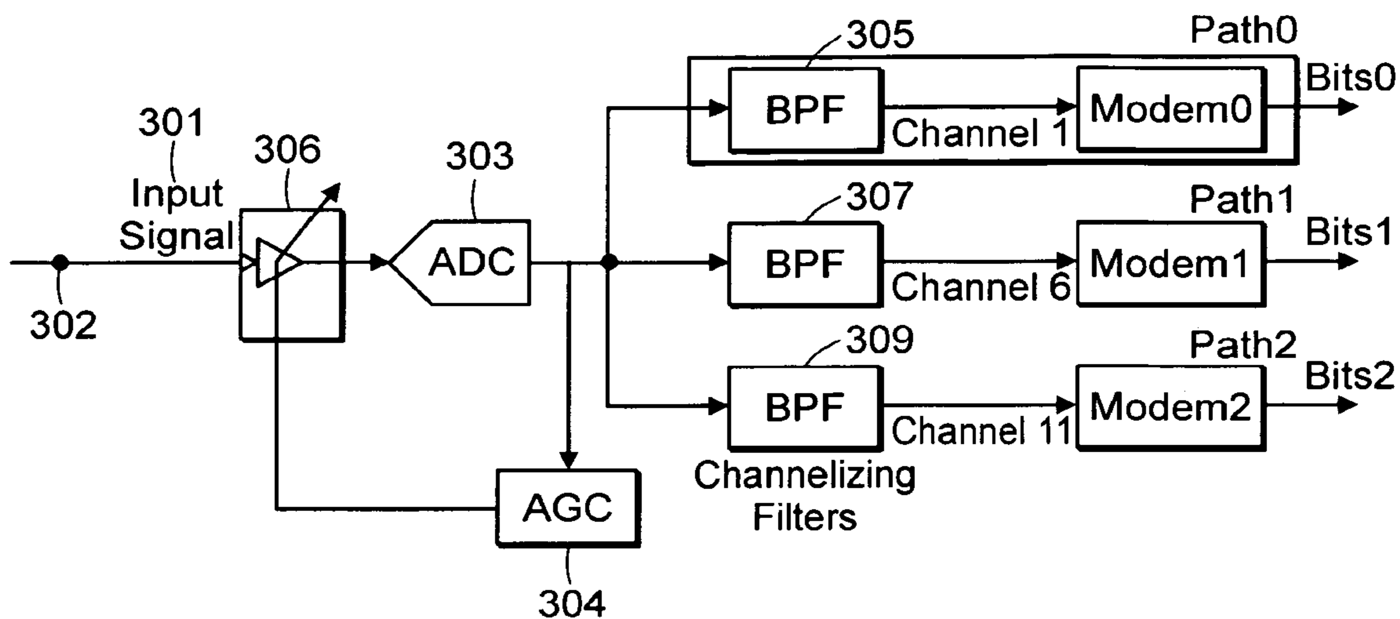
FIG. 3 PRIOR ART
