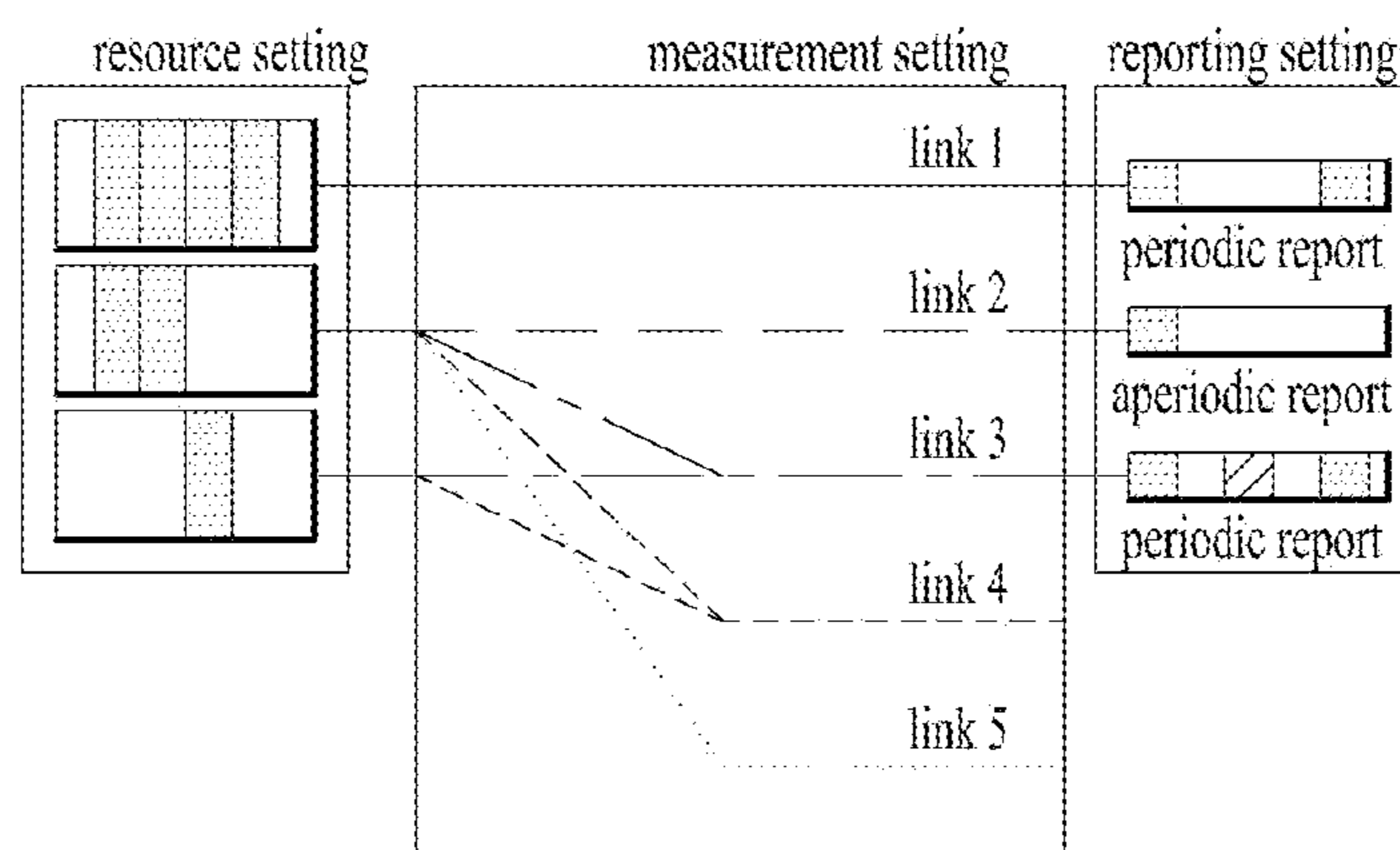
CSI acquisition/beam management framework
