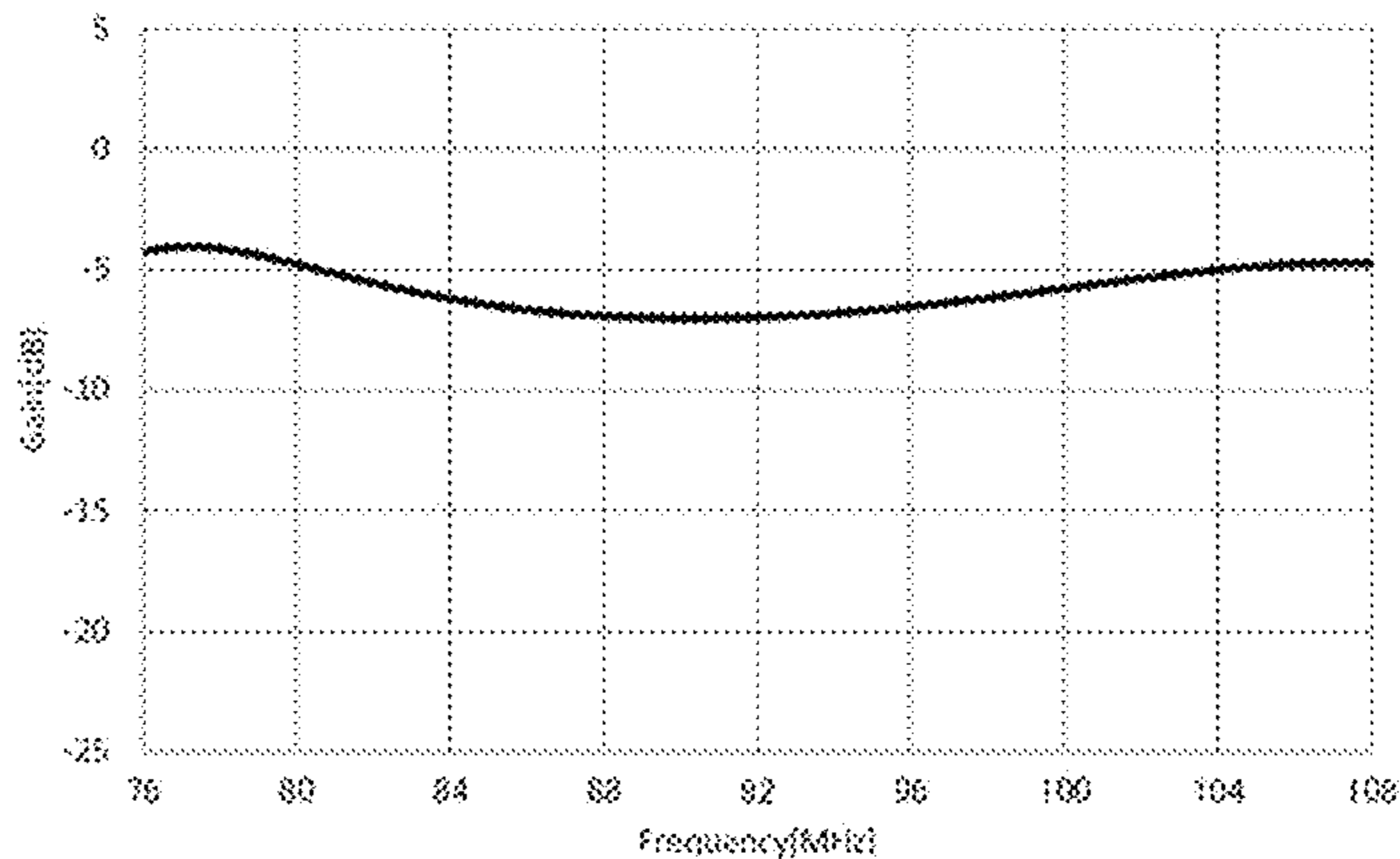
(GAIN-FREQUENCY CHARACTERISTICS)
