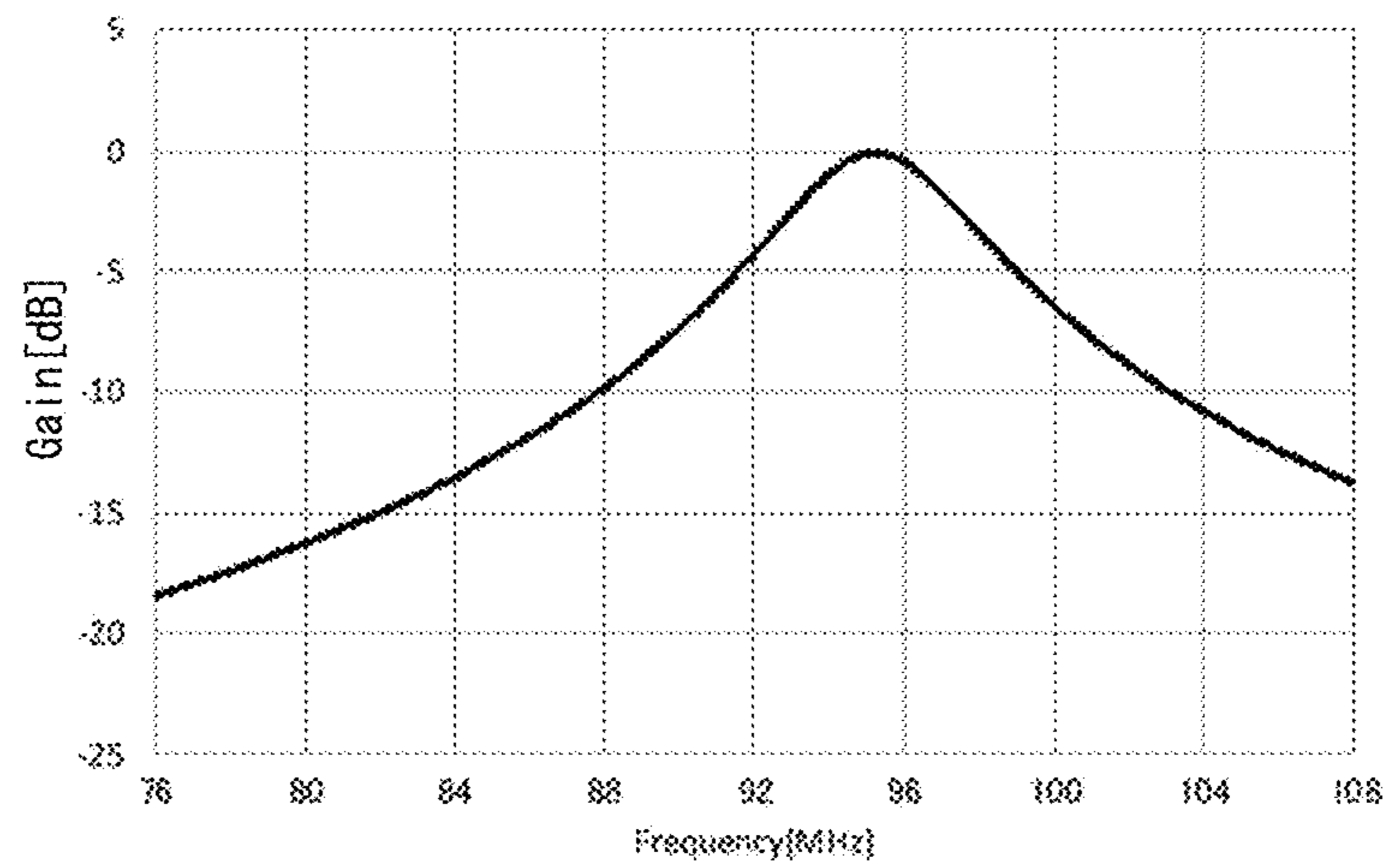
(GAIN-FREQUENCY CHARACTERISTICS)
