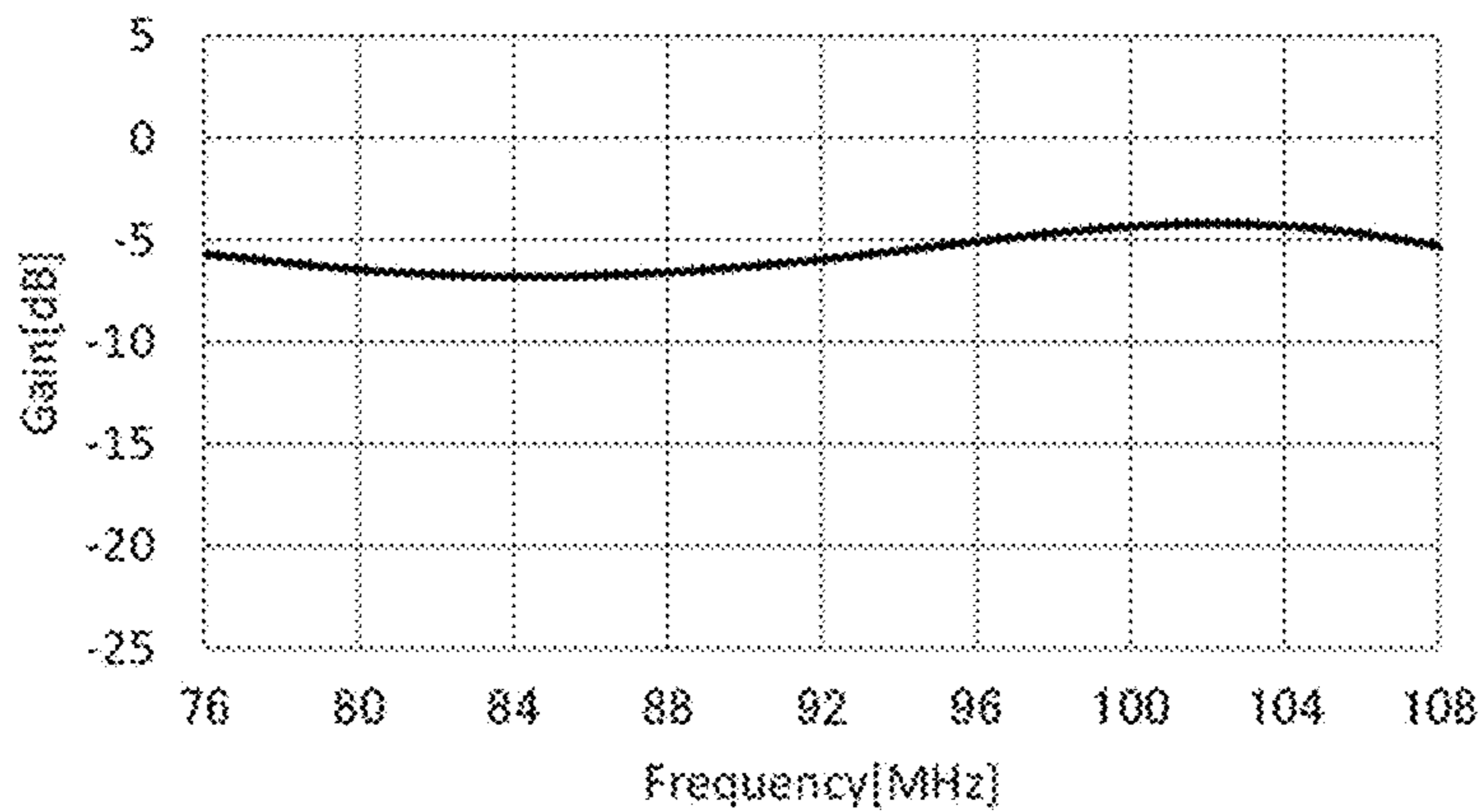
(GAIN-FREQUENCY CHARACTERISTICS)
