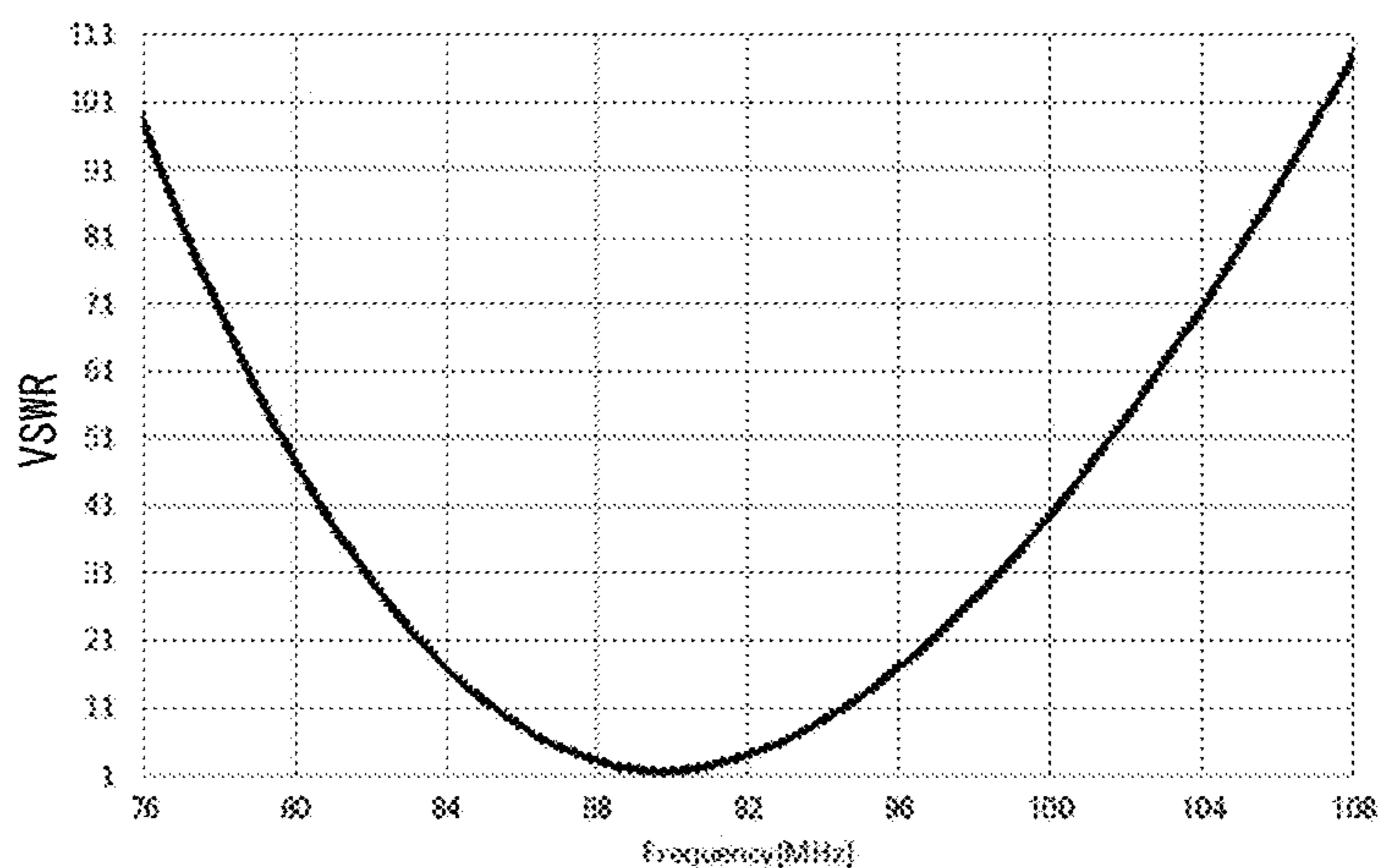
(VSWR-FREQUENCY CHARACTERISTICS)
