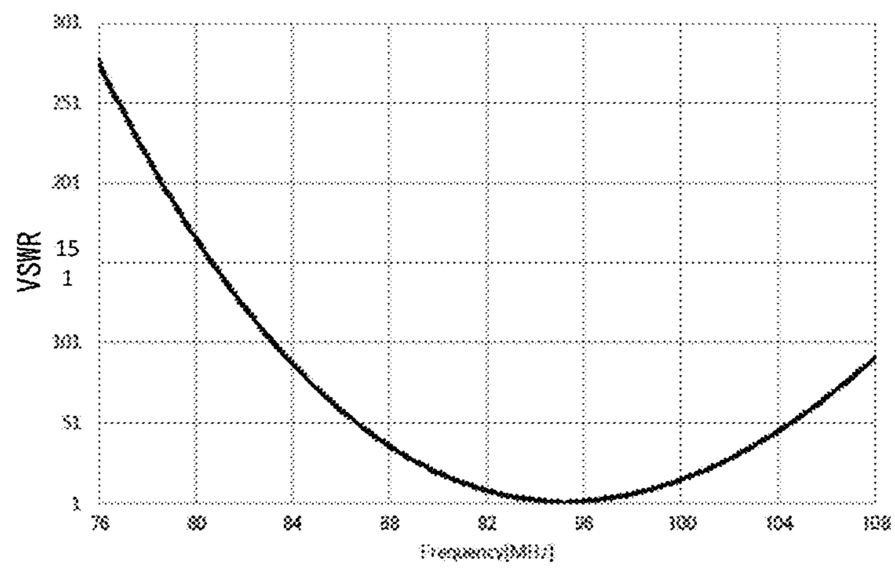
(VSWR-FREQUENCY CHARACTERISTICS)
