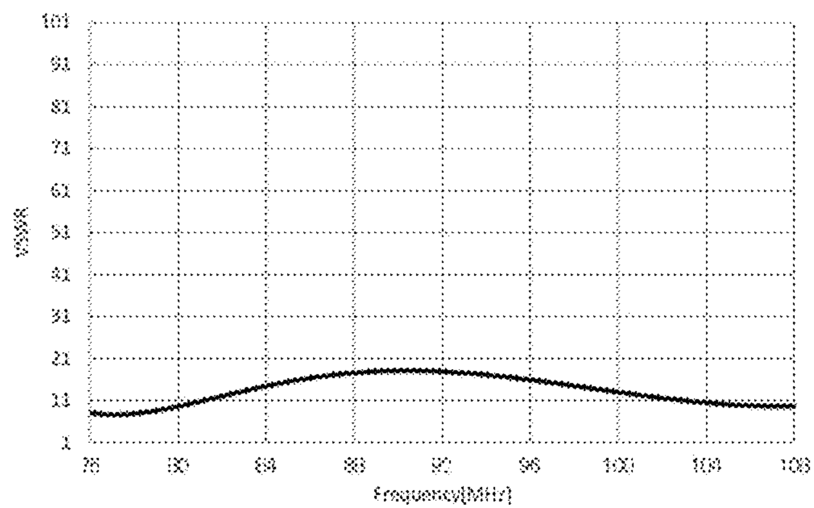
(VSWR-FREQUENCY CHARACTERISTICS)
