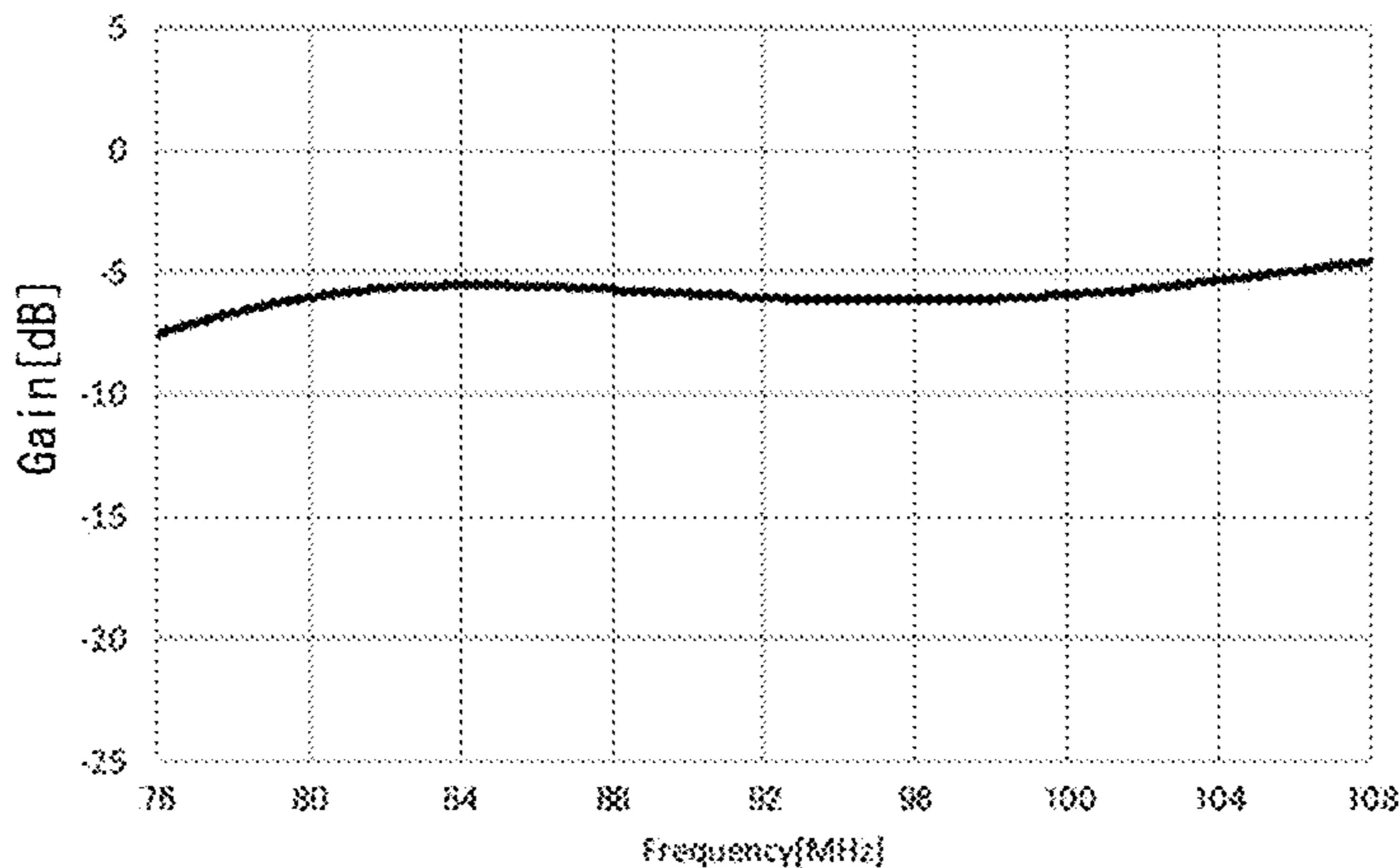
(GAIN-FREQUENCY CHARACTERISTICS)
