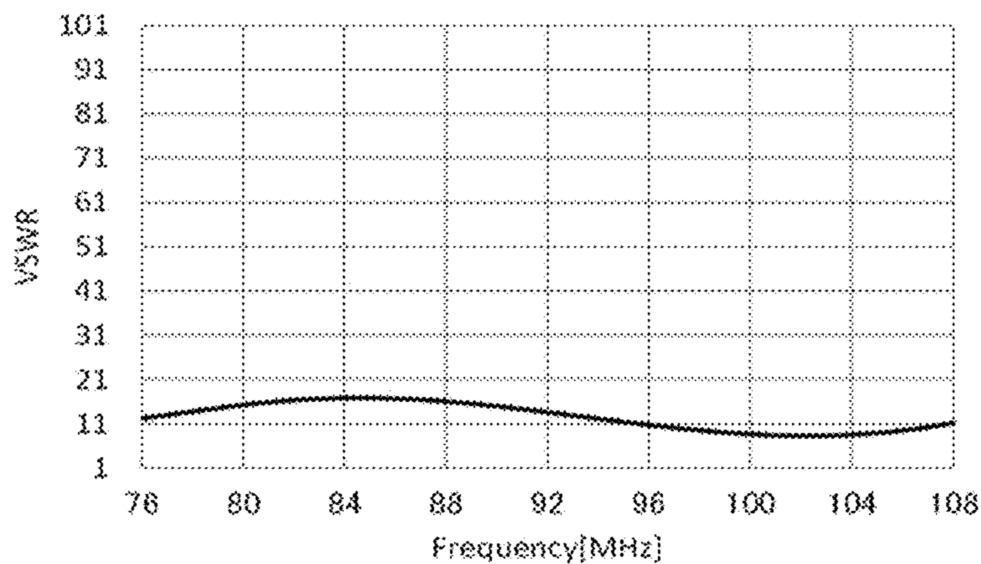
(VSWR-FREQUENCY CHARACTERISTICS)
