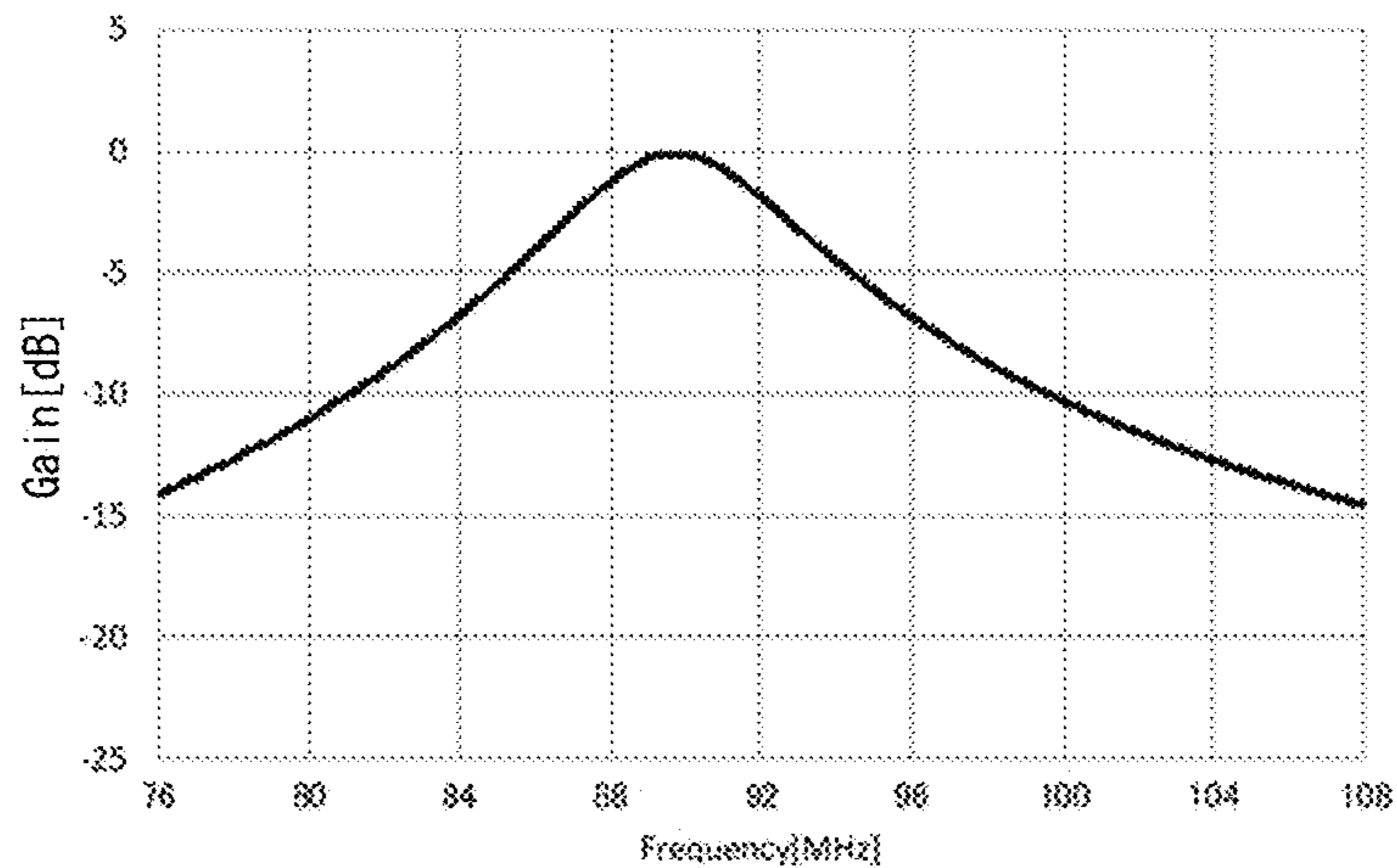
(GAIN-FREQUENCY CHARACTERISTICS)
