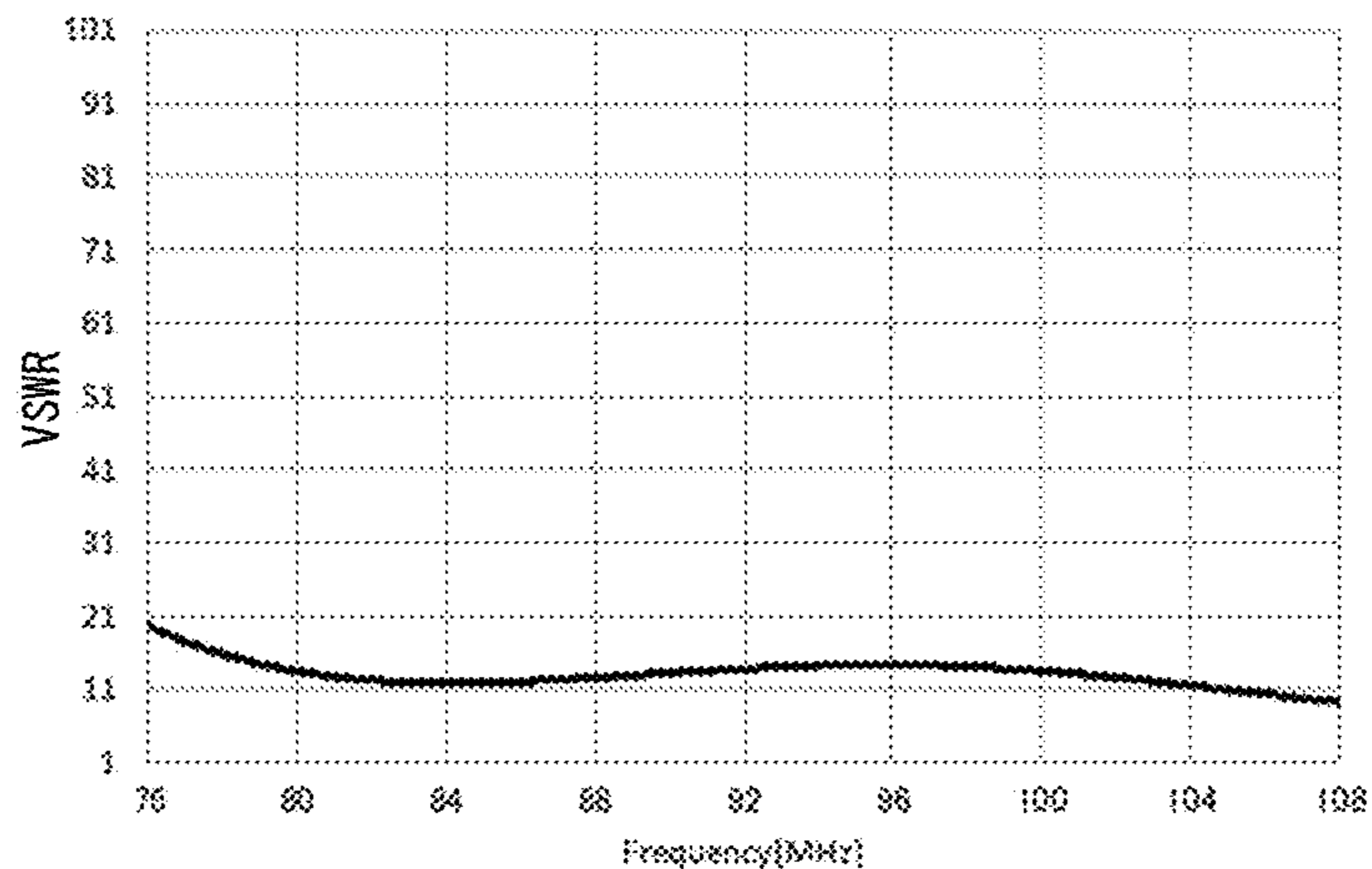
(VSWR-FREQUENCY CHARACTERISTICS)
