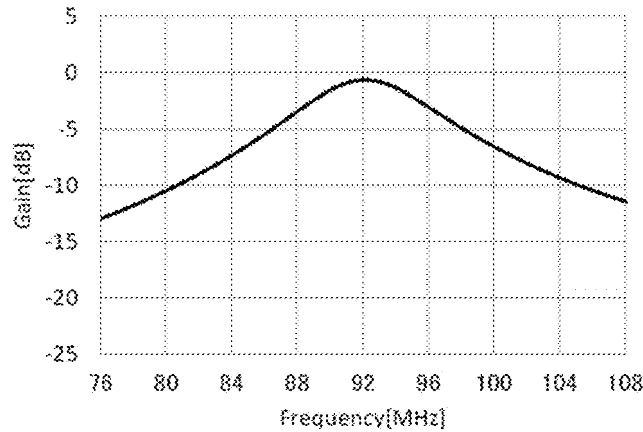
(GAIN-FREQUENCY CHARACTERISTICS)
