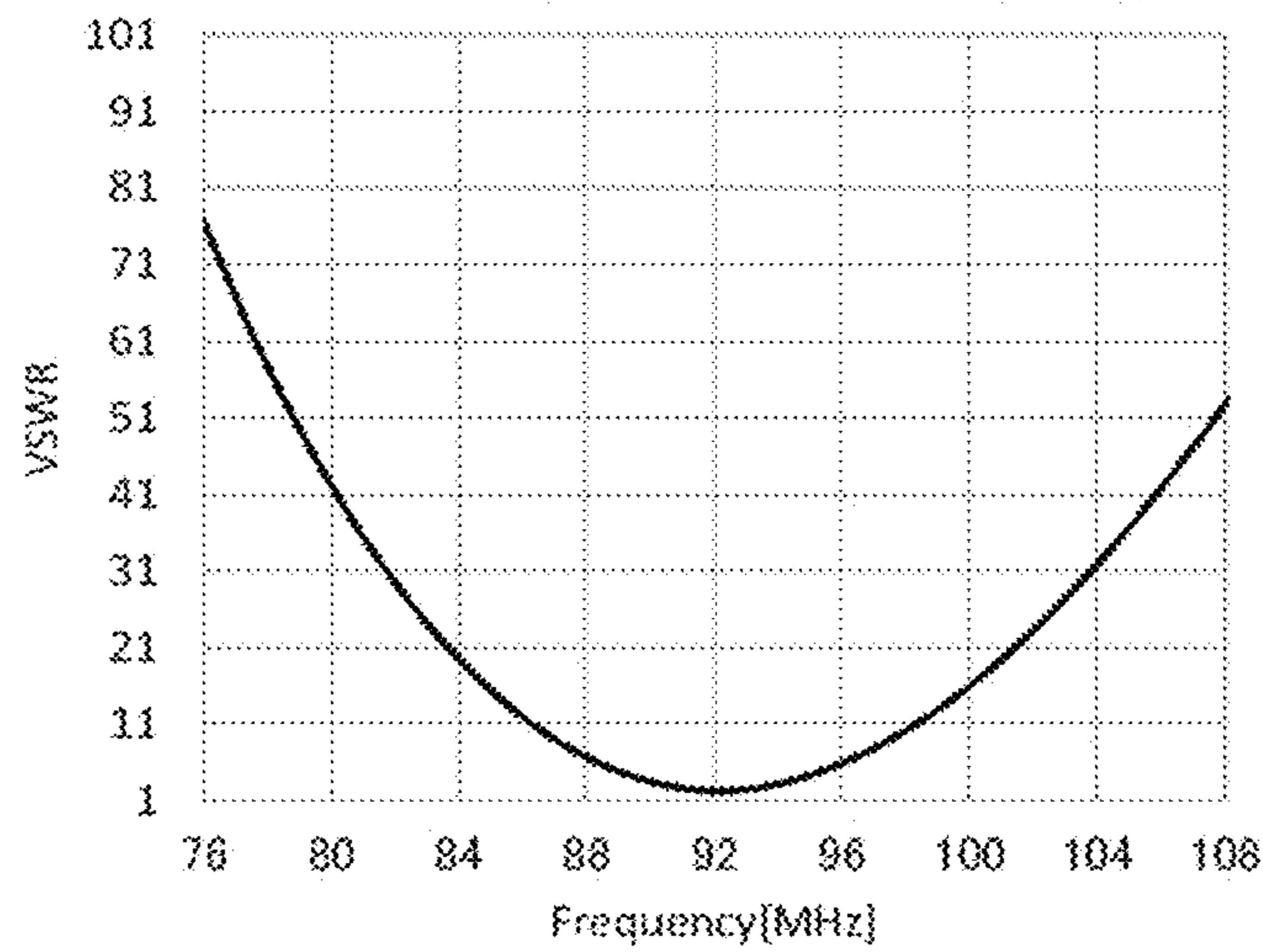
(VSWR-FREQUENCY CHARACTERISTICS)
