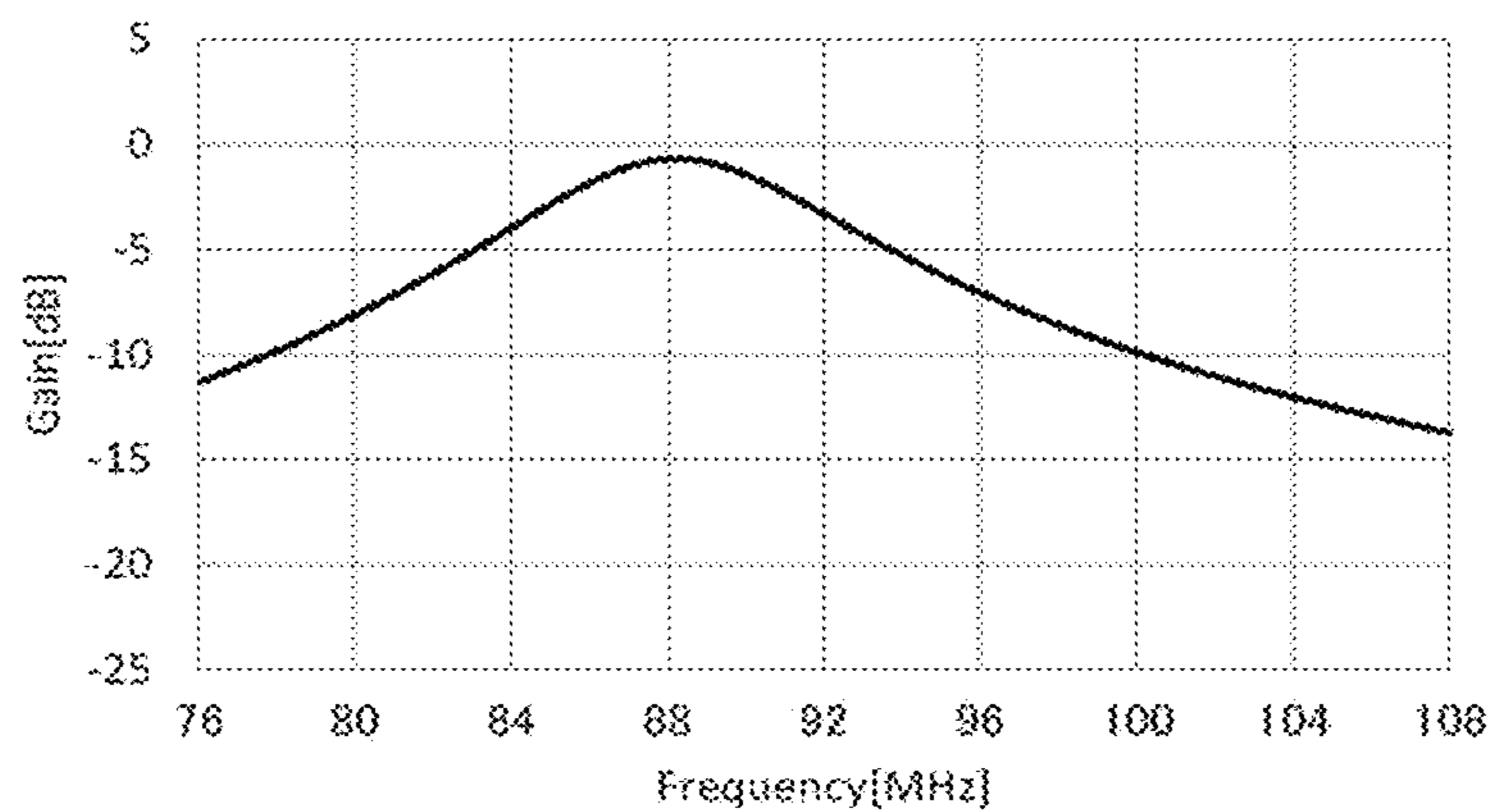
(GAIN-FREQUENCY CHARACTERISTICS)
