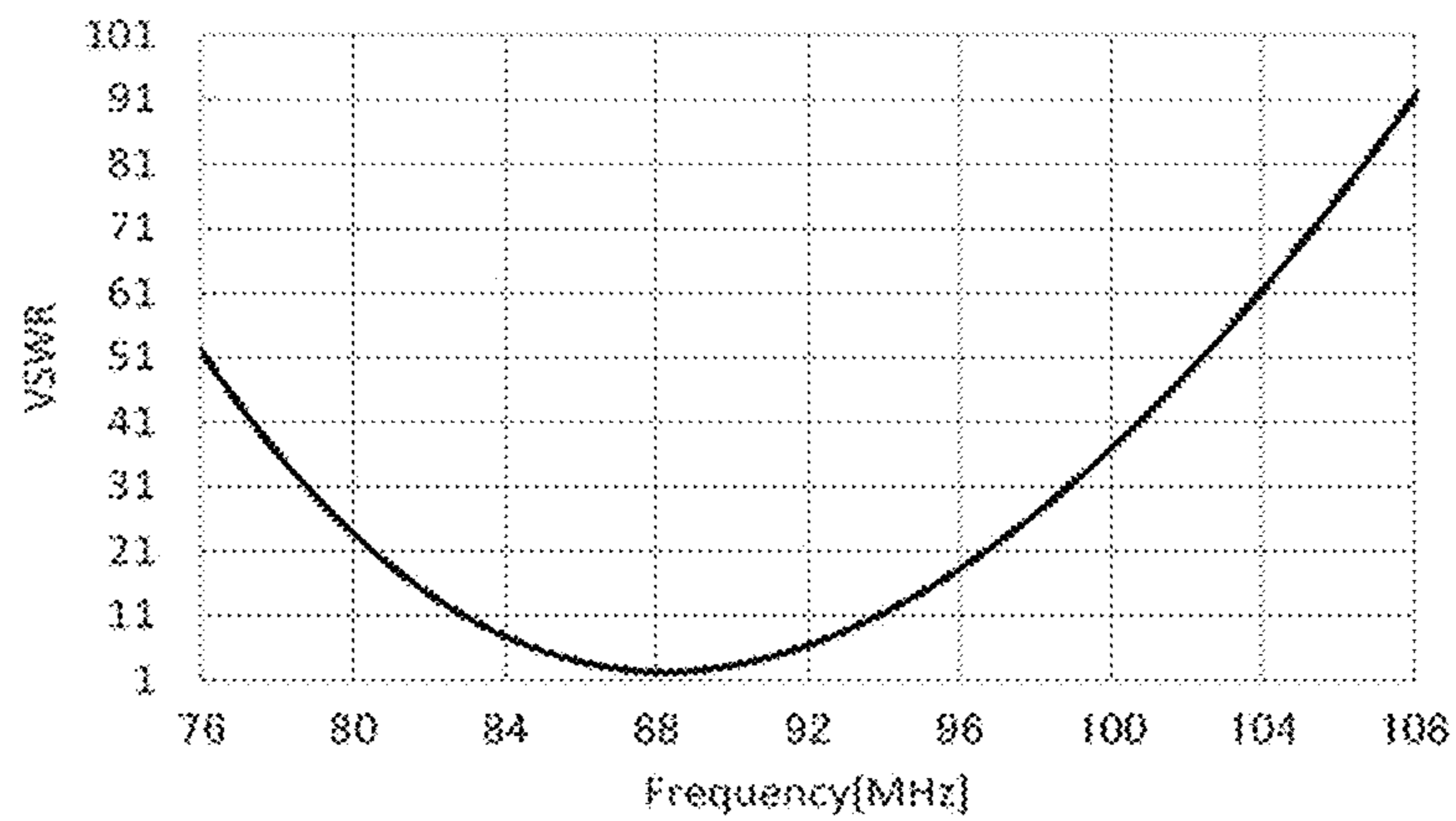
(VSWR-FREQUENCY CHARACTERISTICS)
