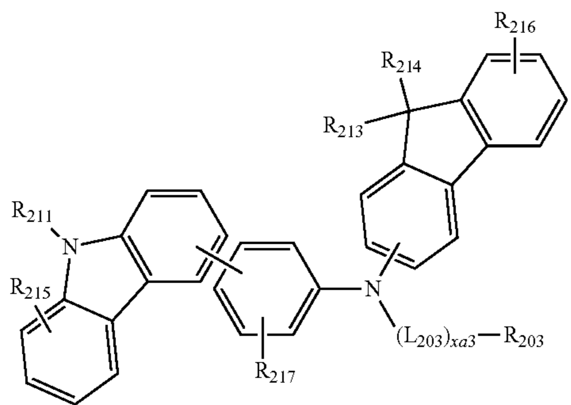
Formula 201A(1)
