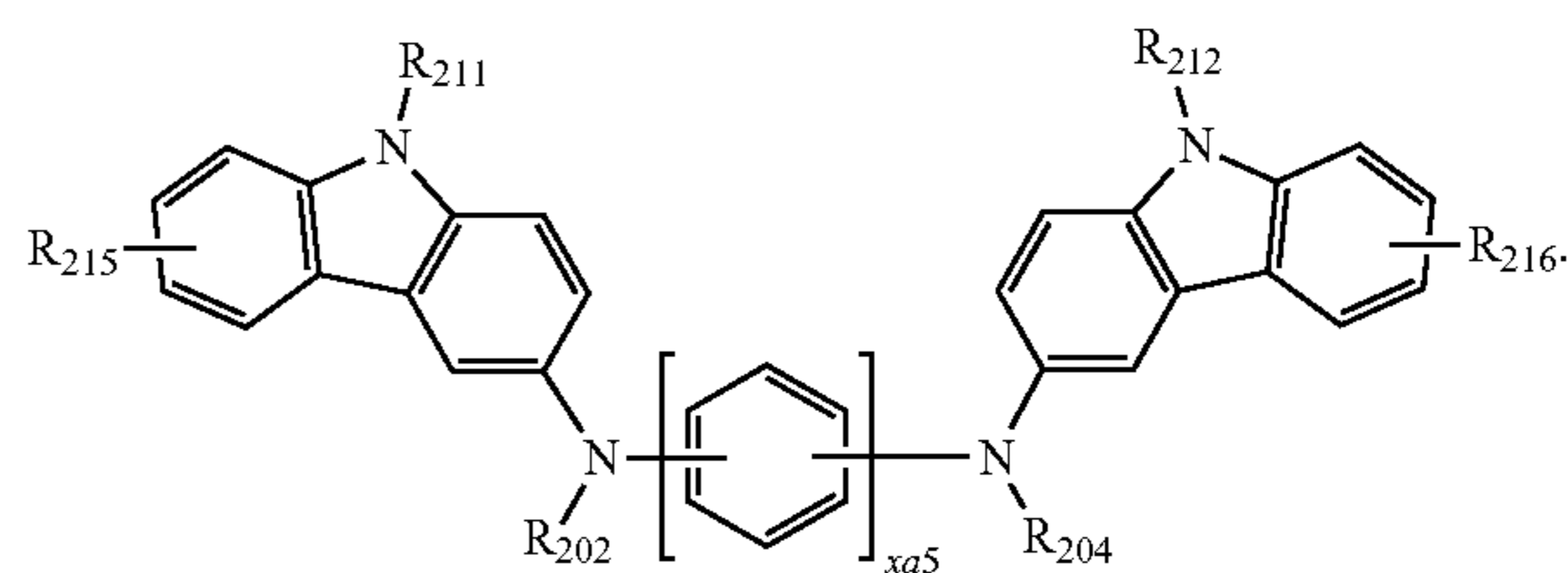
Formula 202A-1
