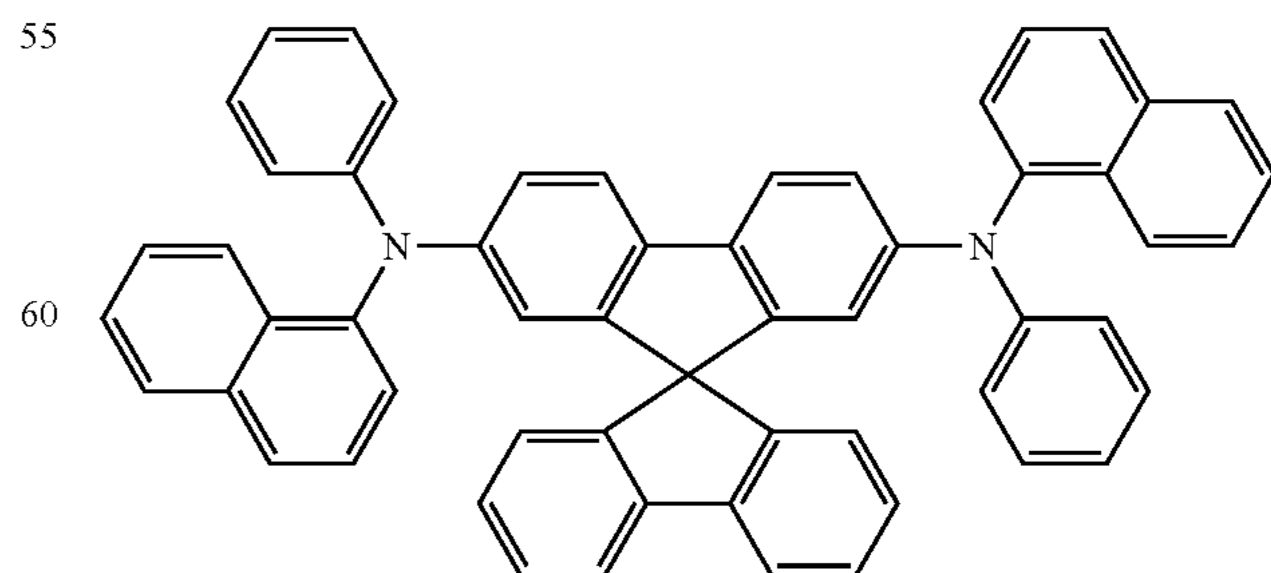
Spiro-NPB
