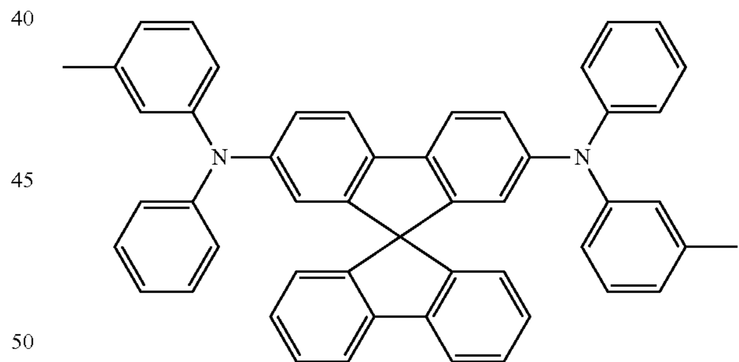
Spiro-TPD
