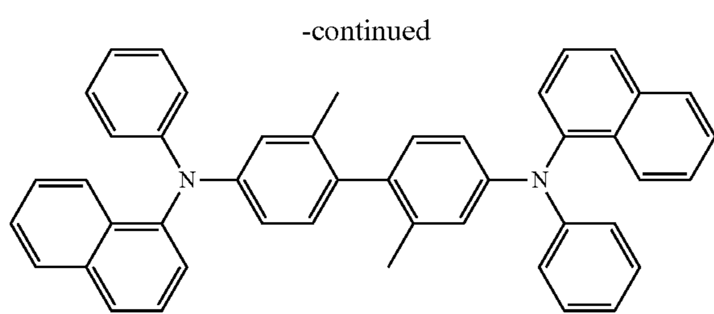
methylated NPB
