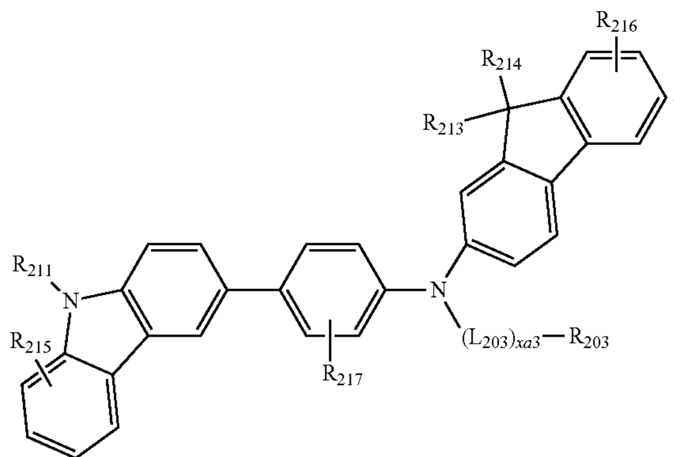
Formula 201A-1
