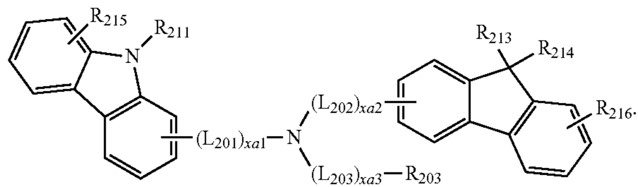
Formula 201A
