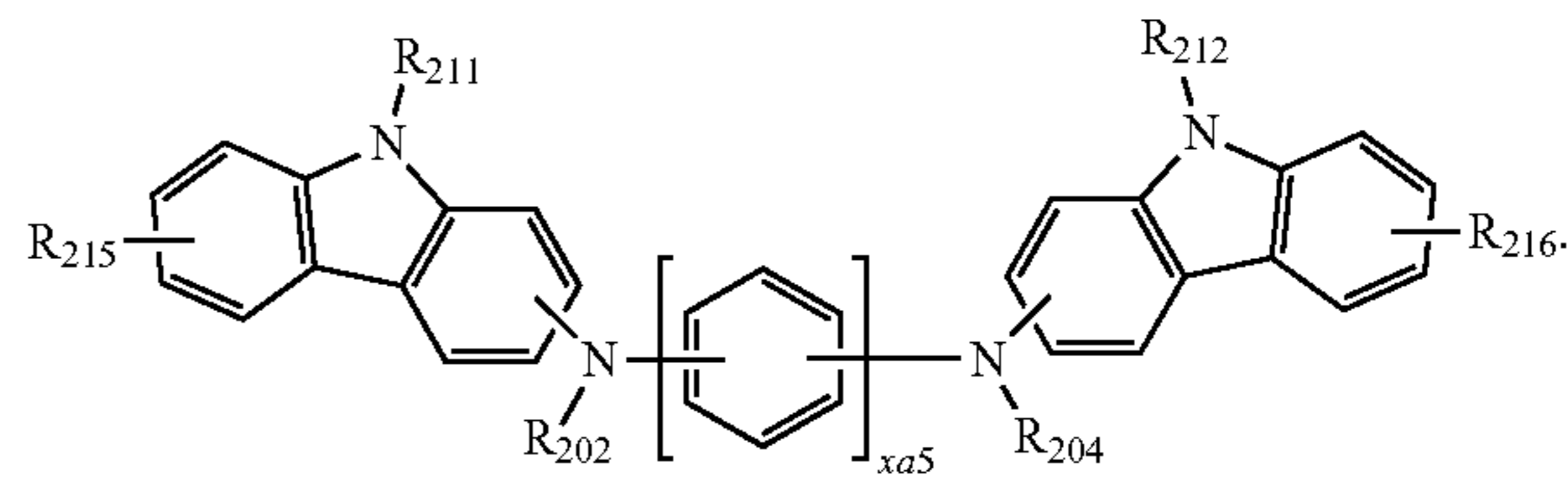
Formula 202A
