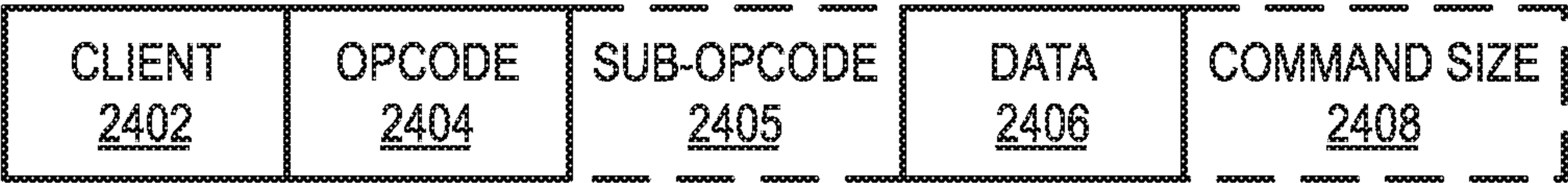
FIG. 17A GRAPHICS PROCESSOR COMMAND FORMAT 2400
