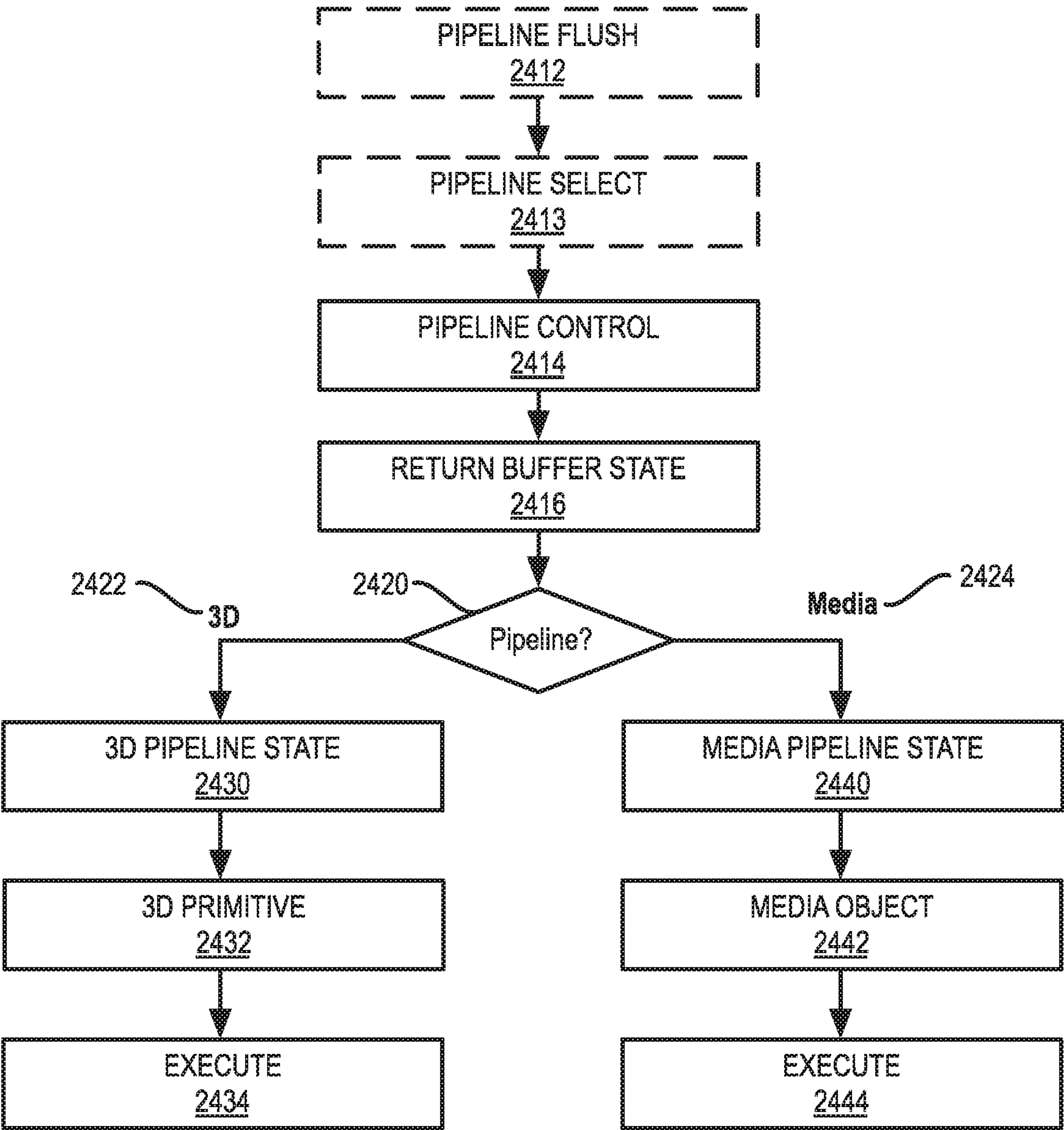
FIG. 17B GRAPHICS PROCESSOR COMMAND SEQUENCE 2410
