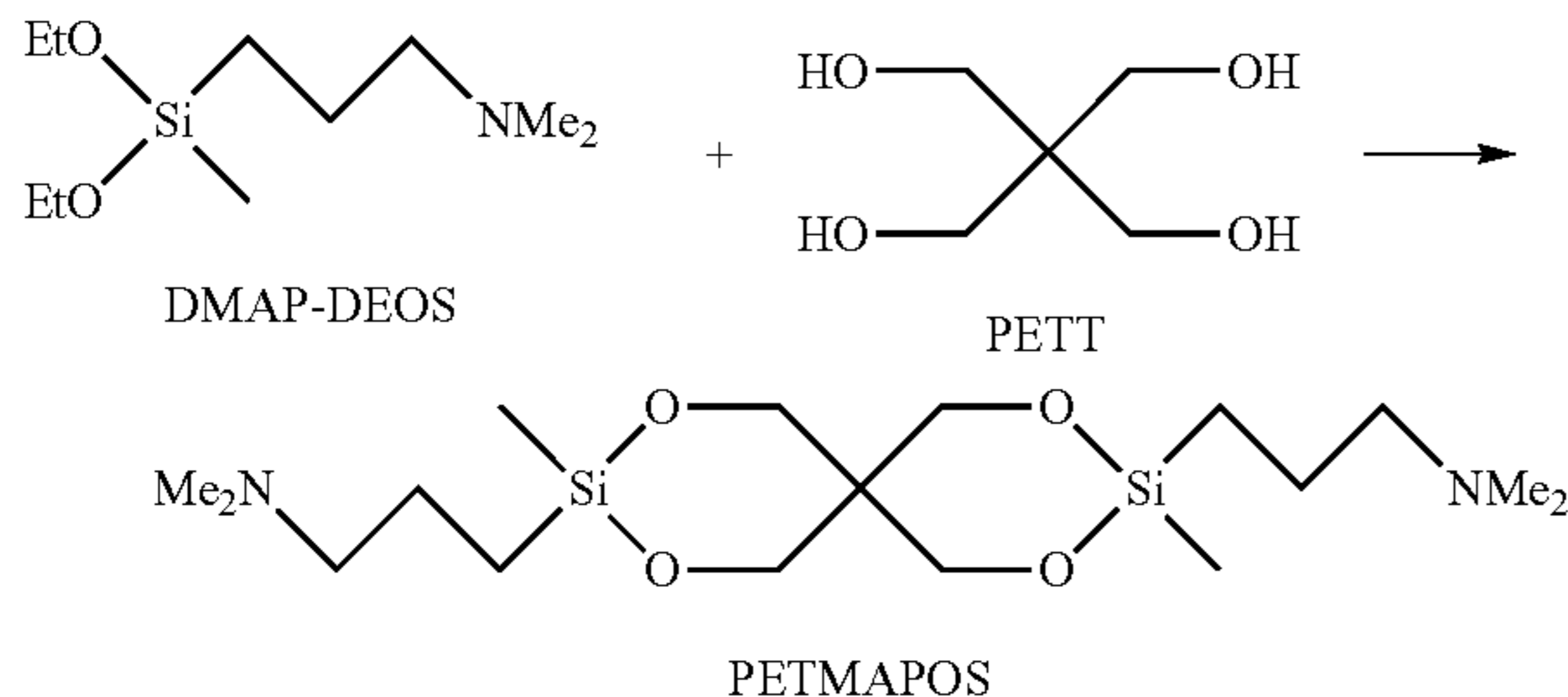
Figure 3. Synthesis of PETMAPOS
