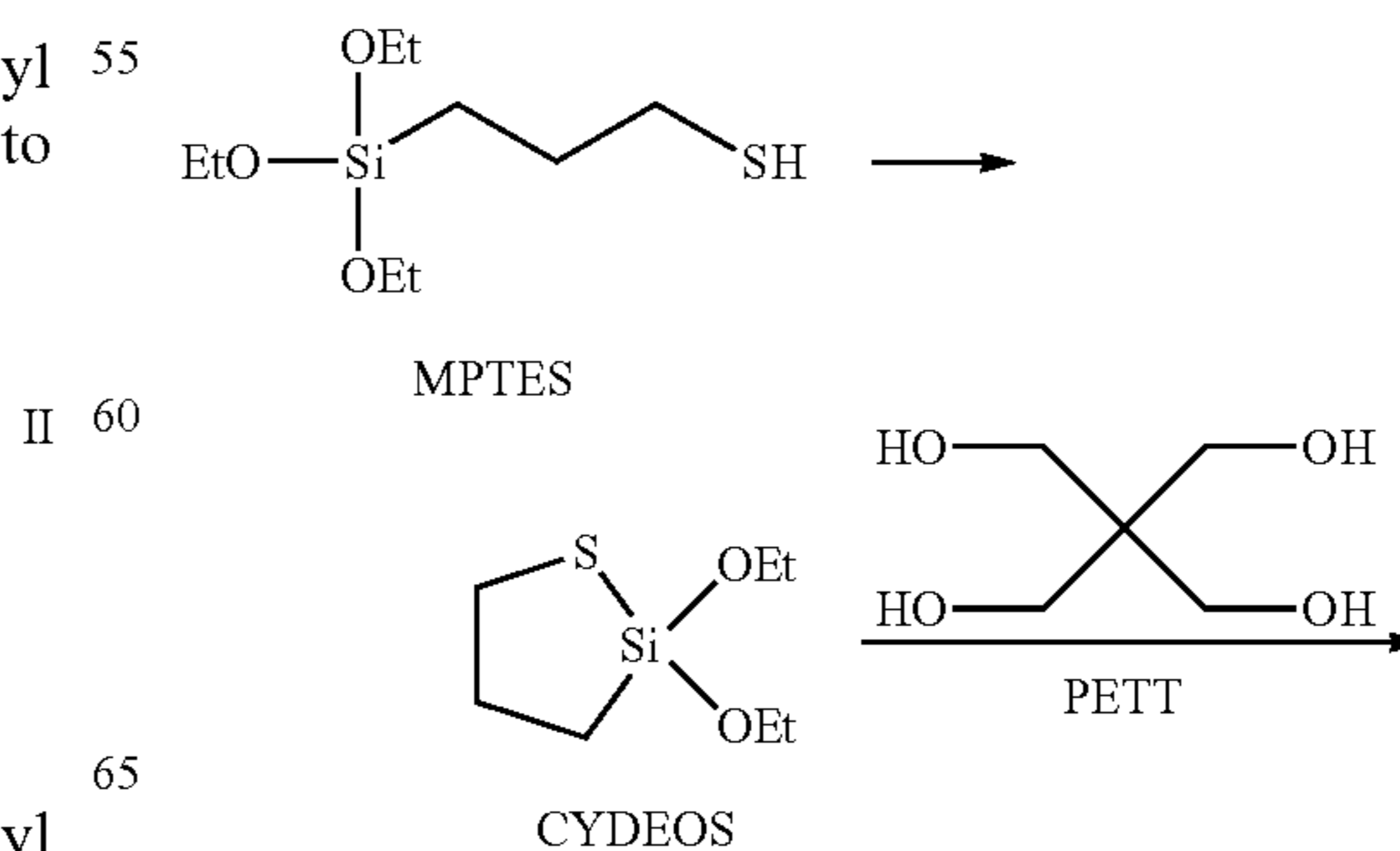
Figure 2. Synthesis of PETMOS
