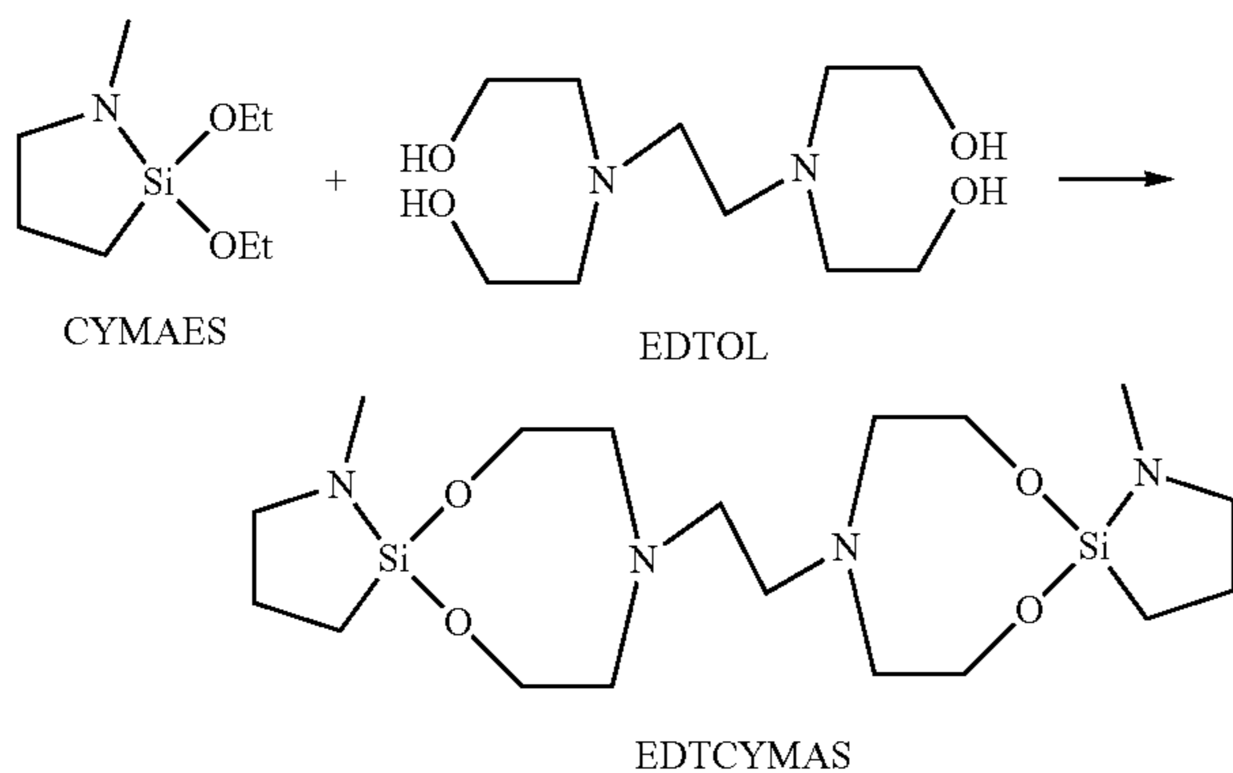
Figure 4. Synthesis of EDTCYMAS
