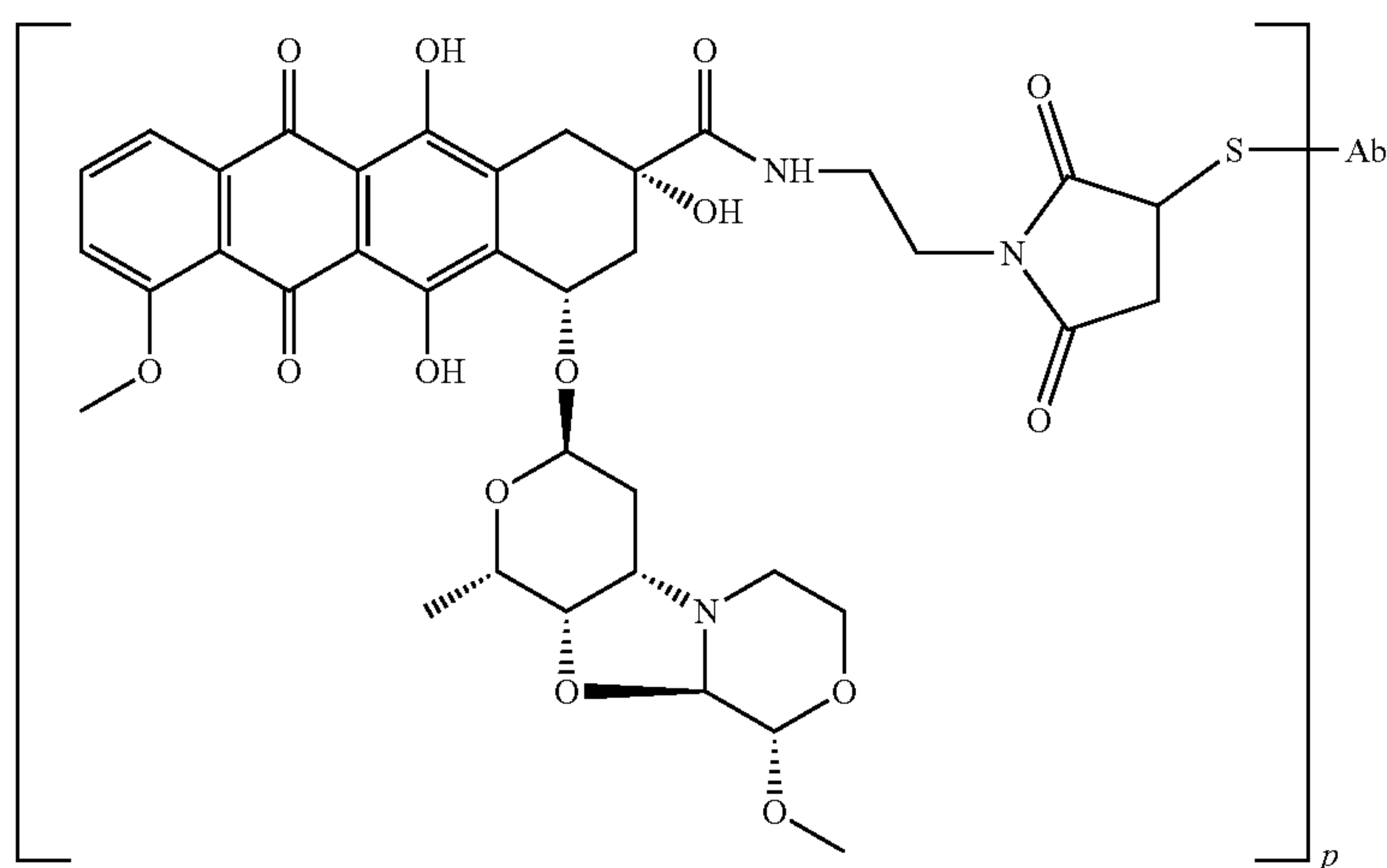
PNU-159682-maleimide-Ab
