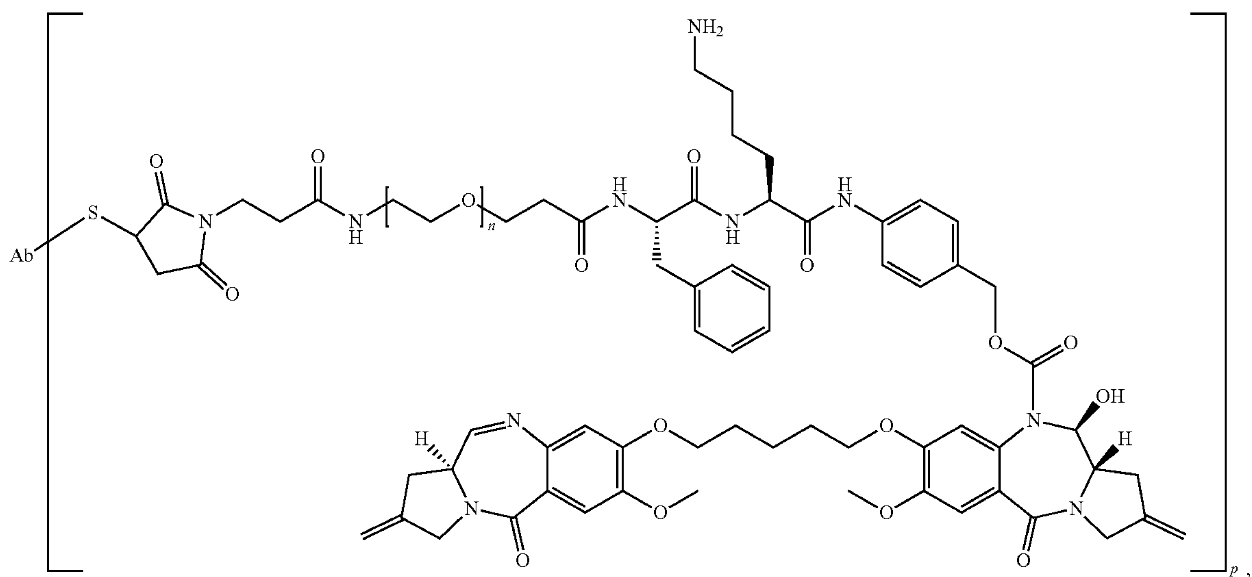
PBD dimer-maleimide-acetal-Ab
