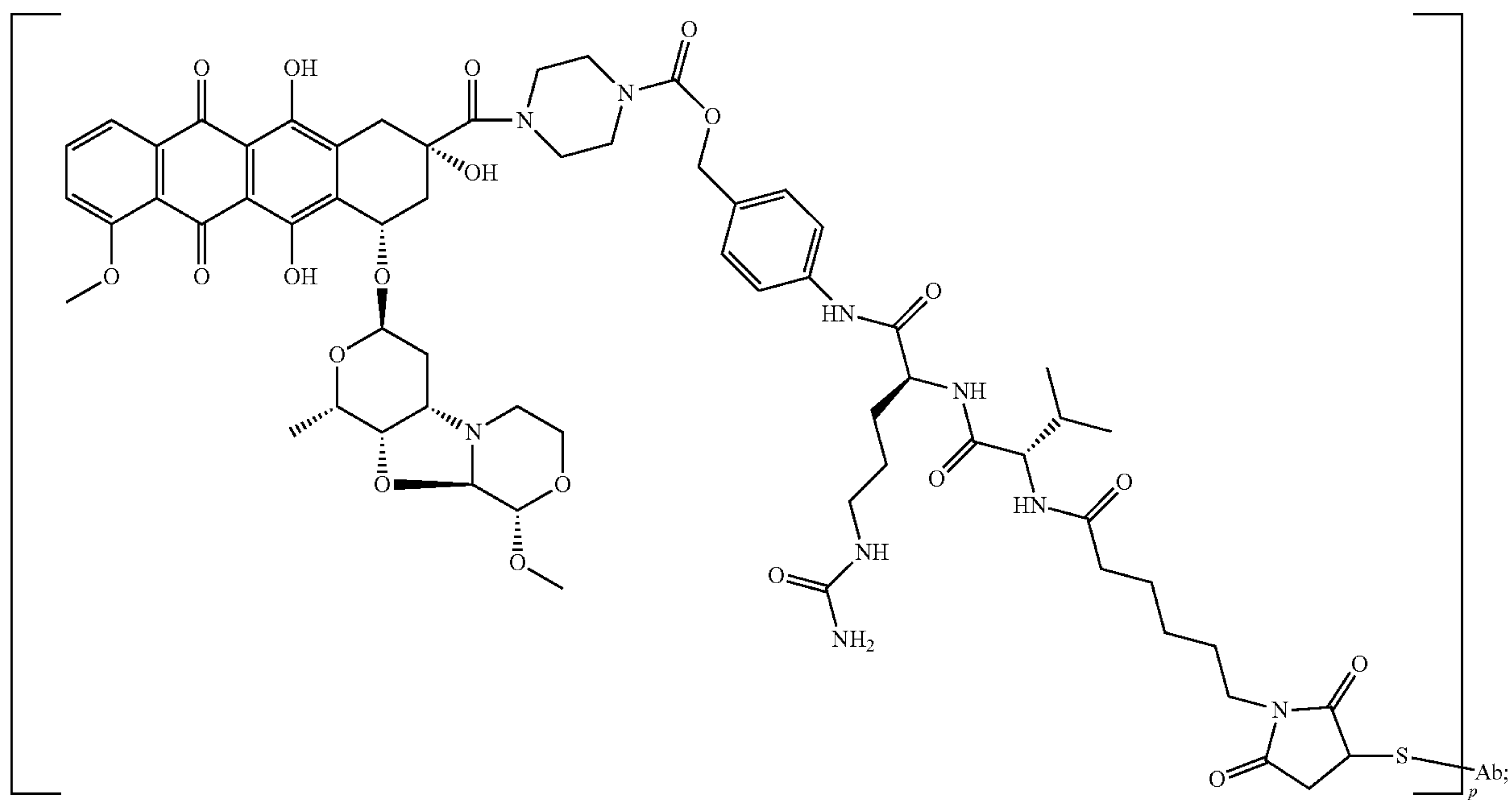
PNU-159682-val-cit-PAB-Ab
