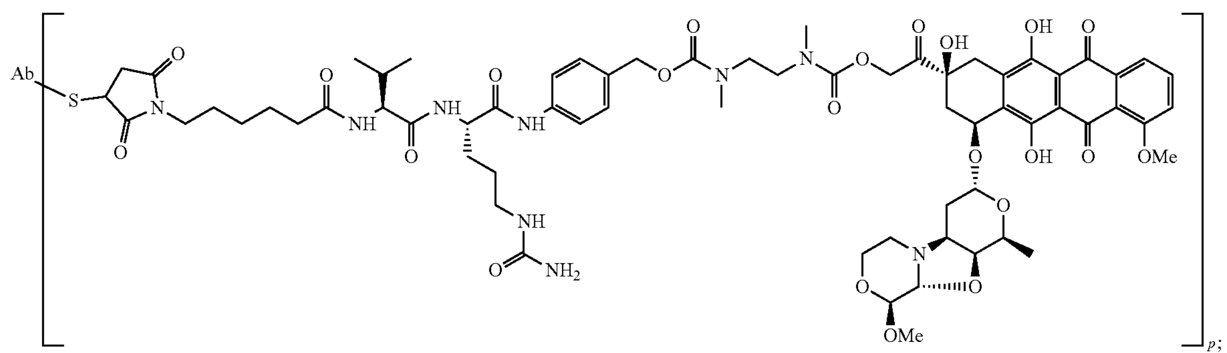
PNU-159682-val-cit-PAB-spacer-Ab
