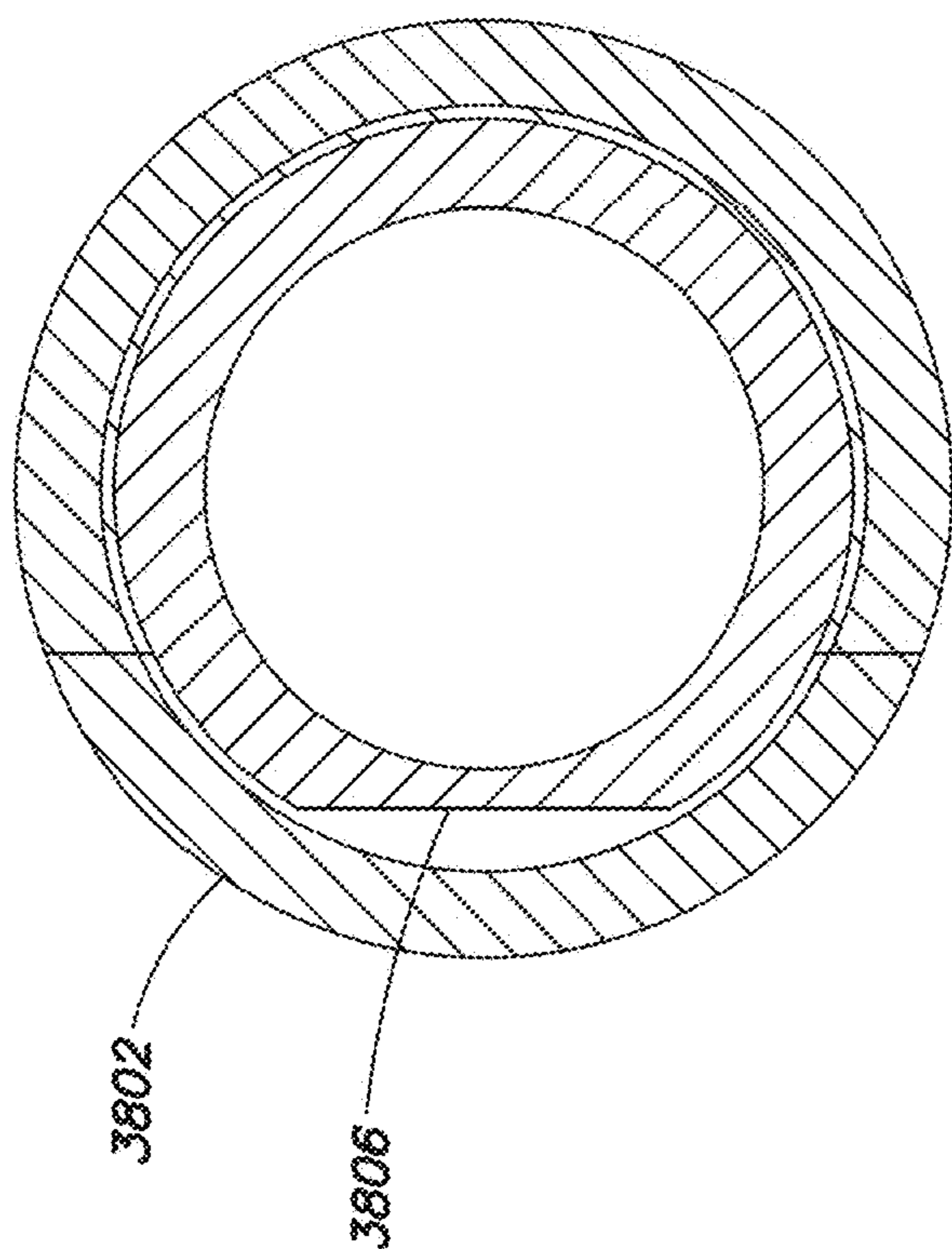
SECTION B-B
