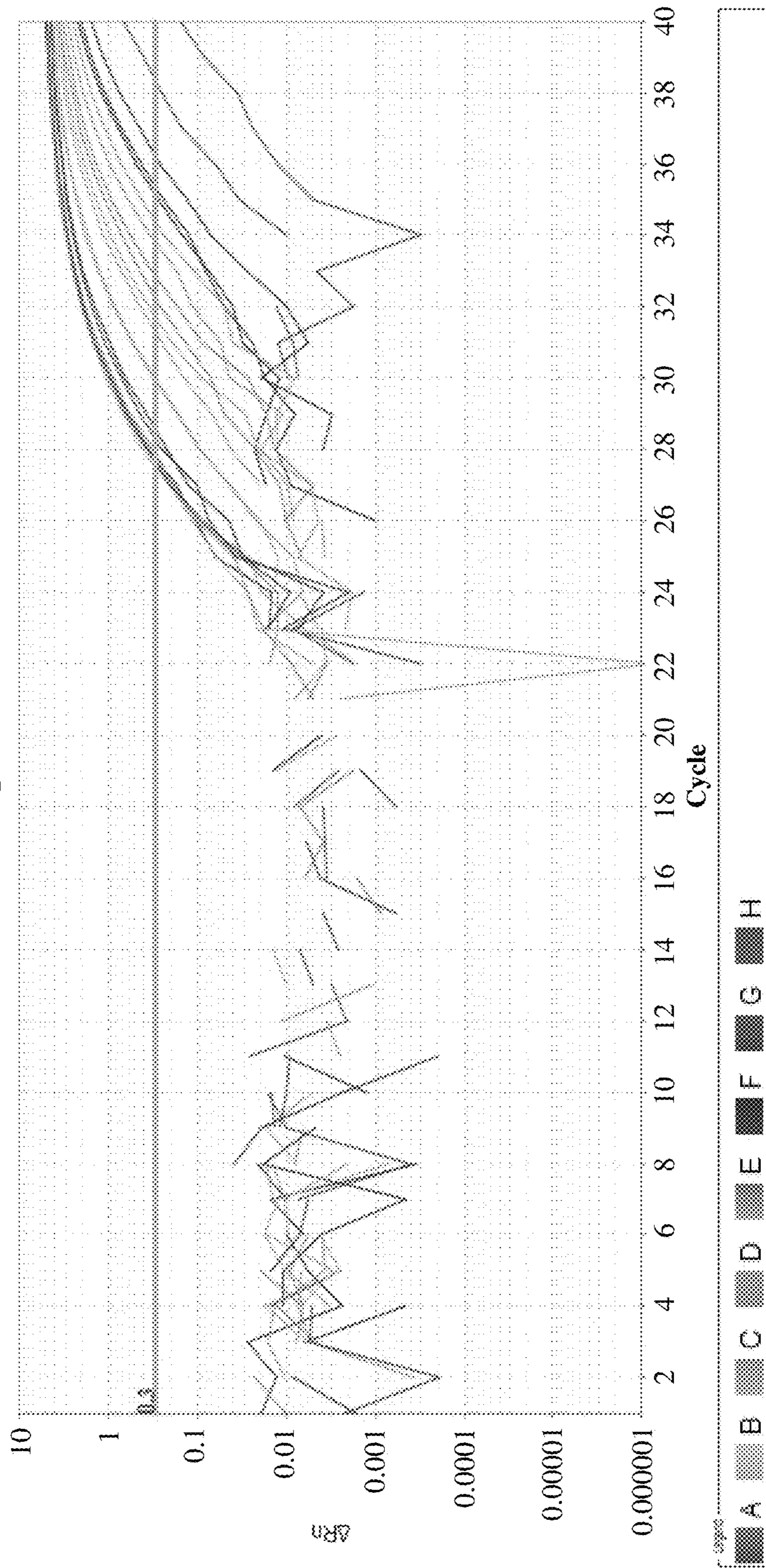
Amplification Plot
