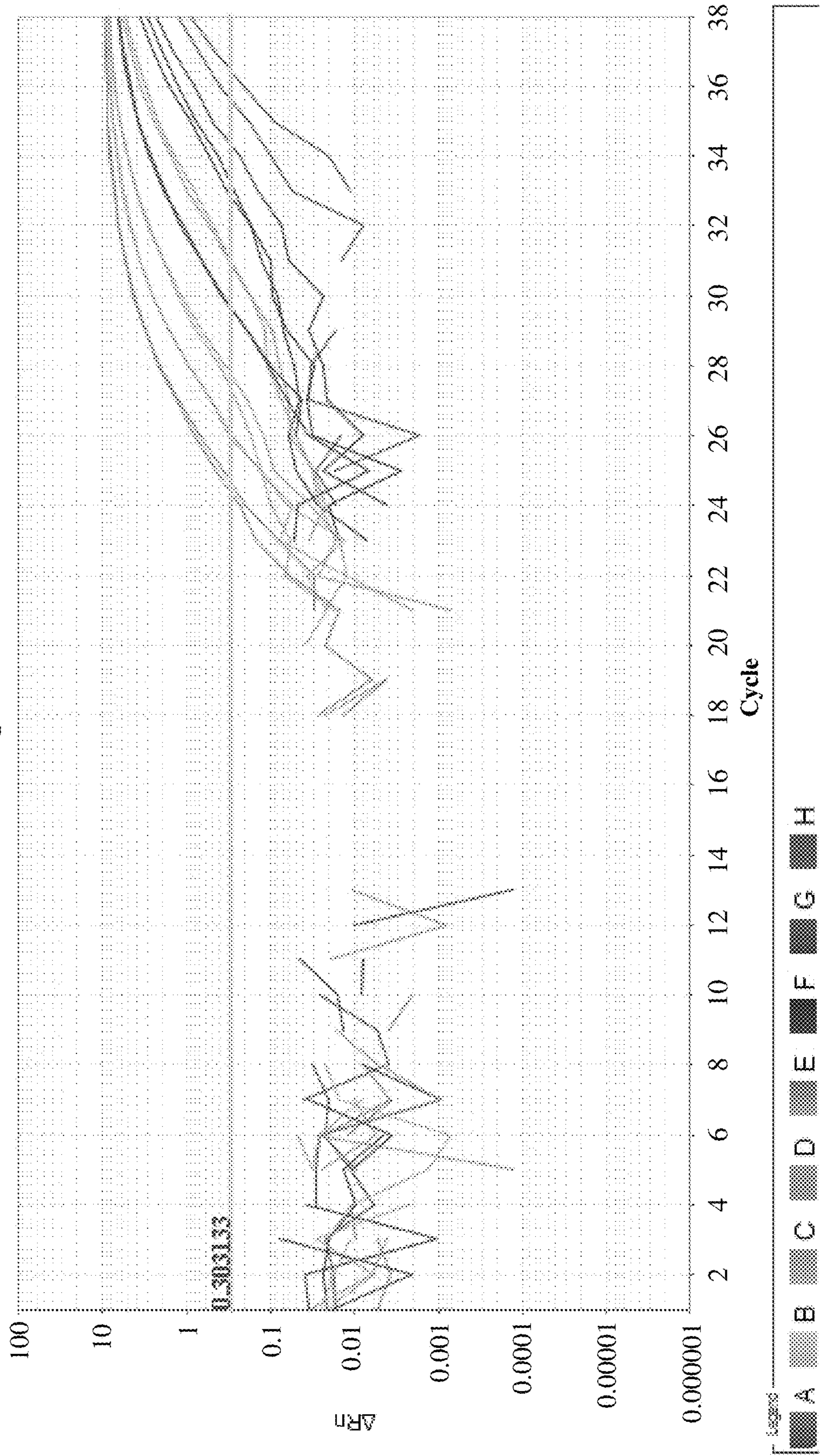
Amplification Plot
