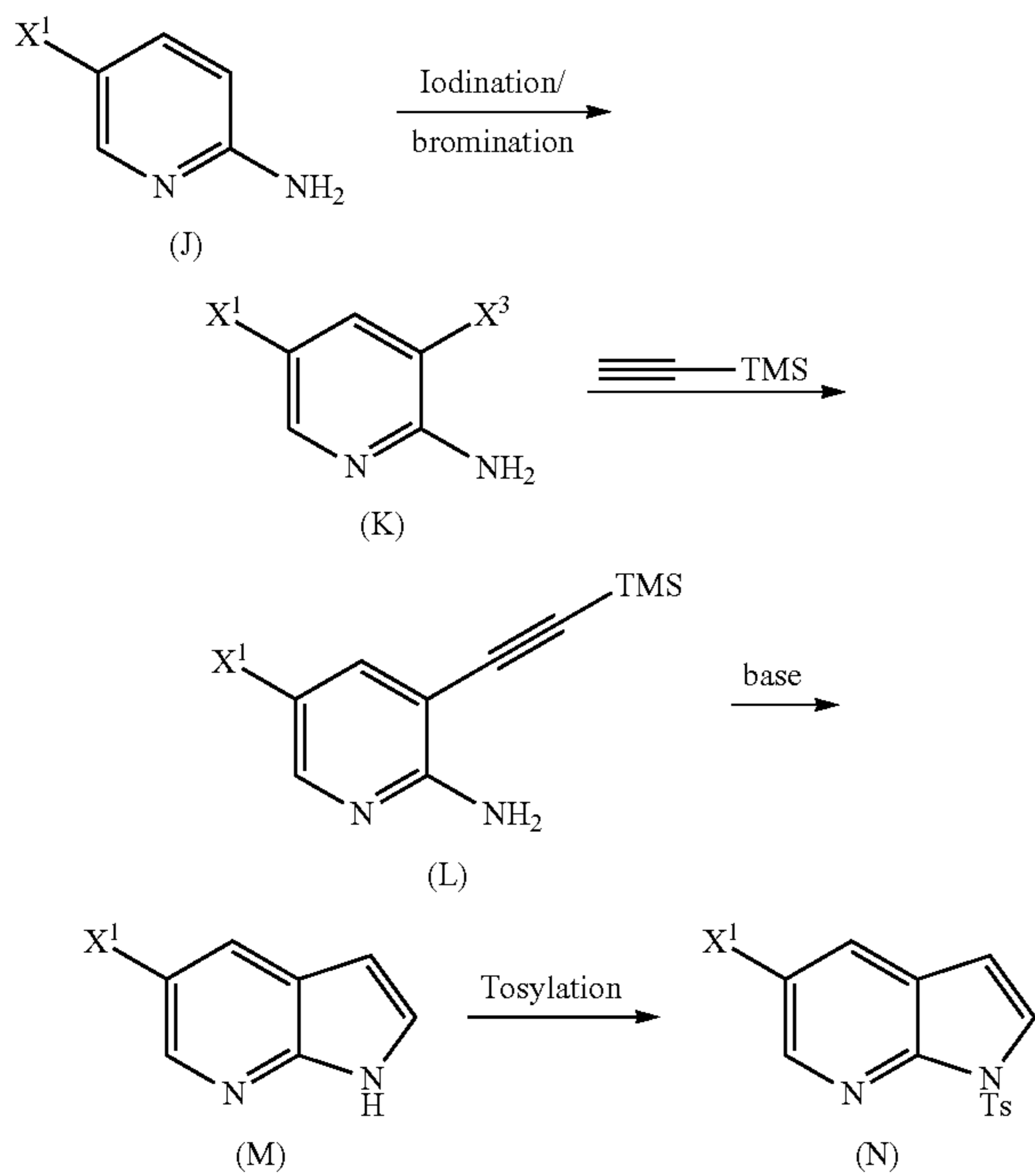
Scheme 8
