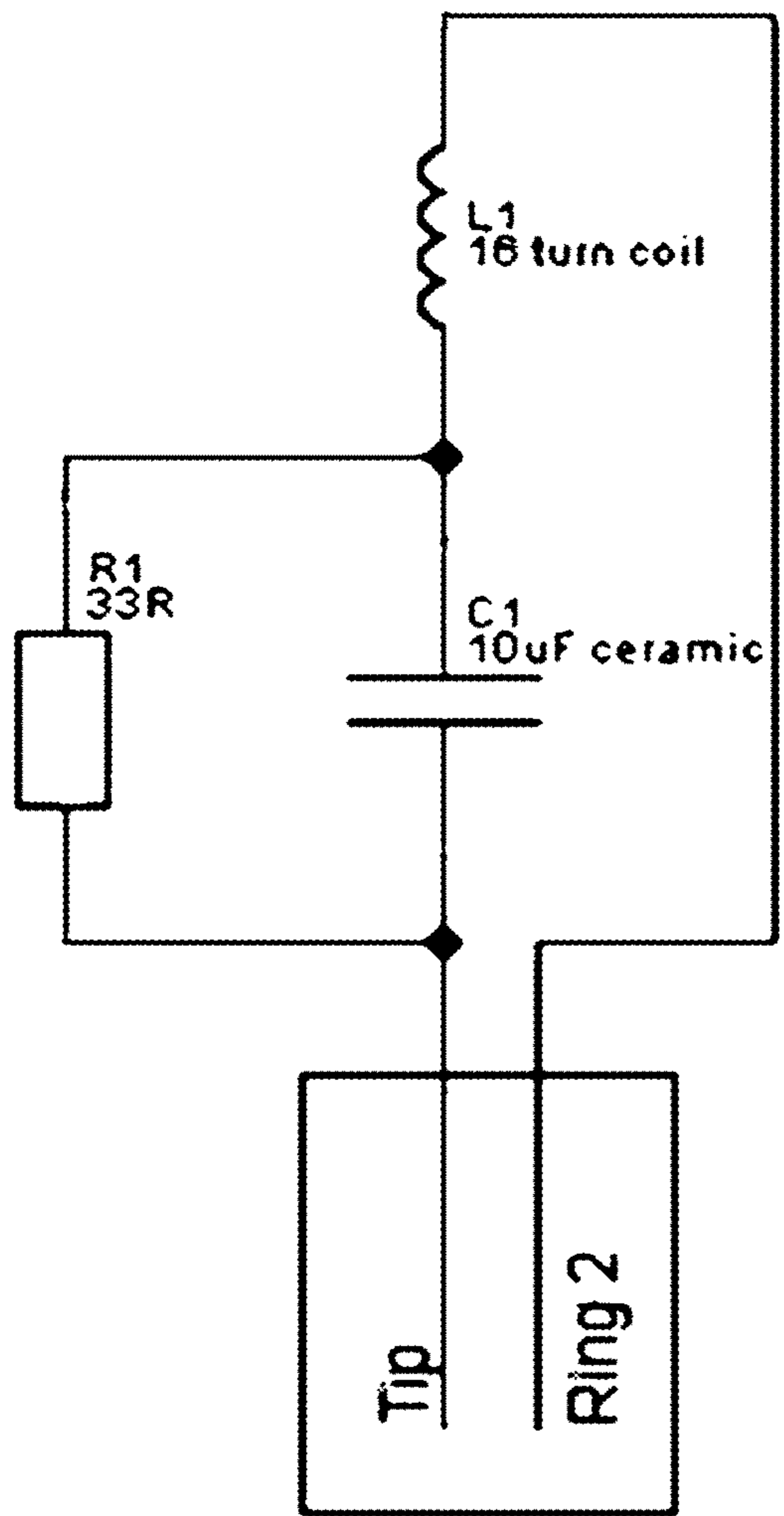
TRRS 4-way jack socket Fig. 1
