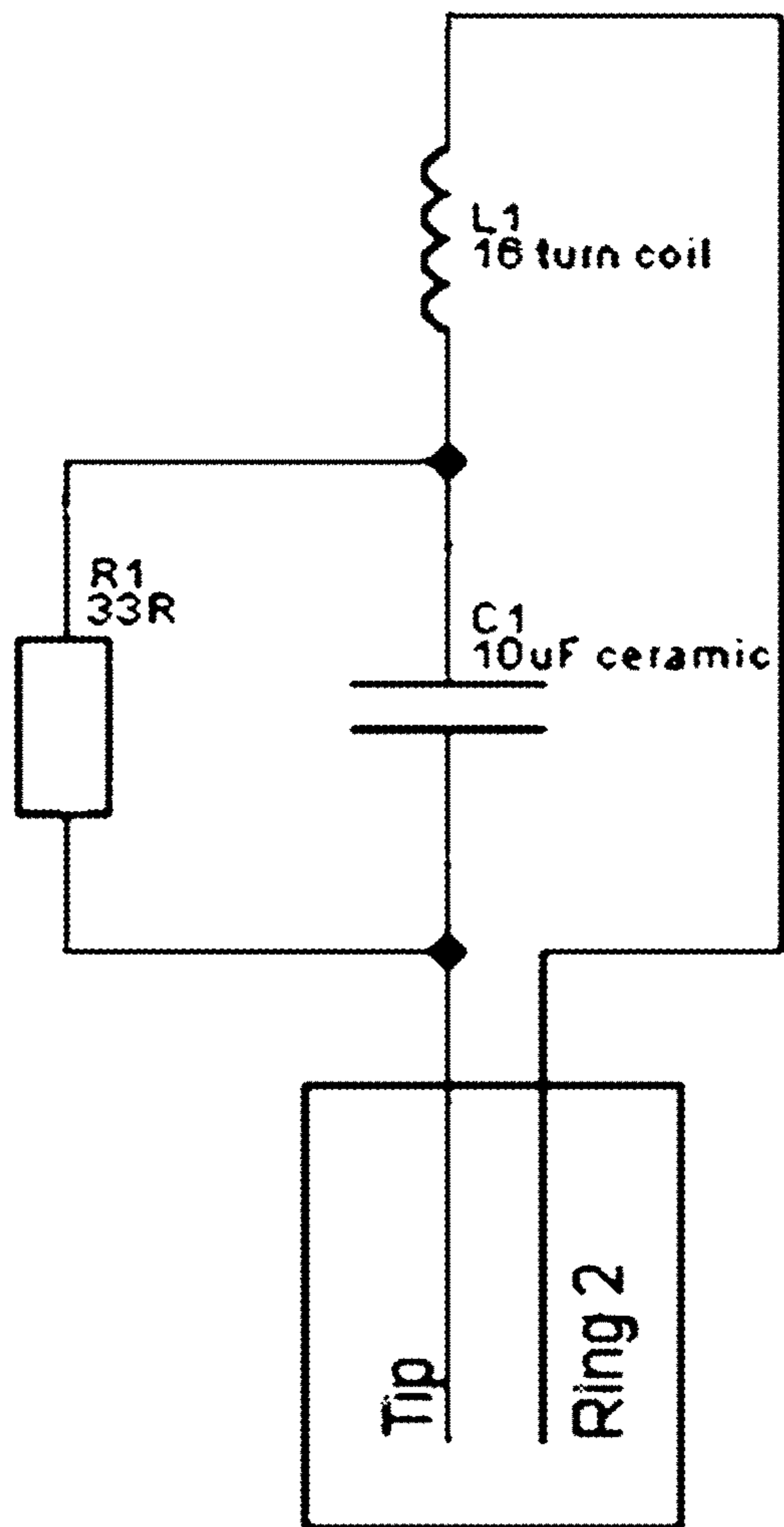
TRRS 4-way jack socket Fig. 1
