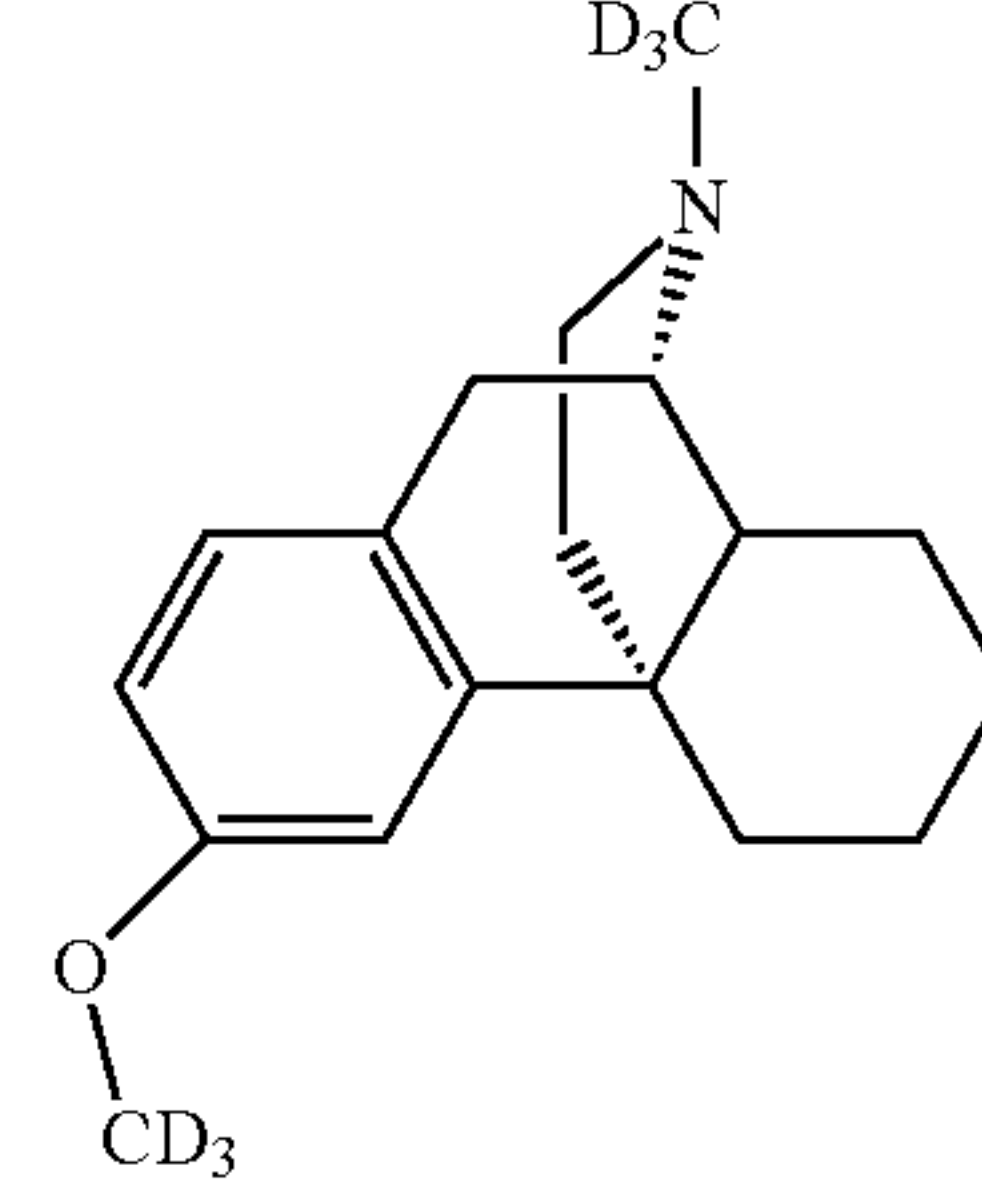
d6-dextromethorphan
