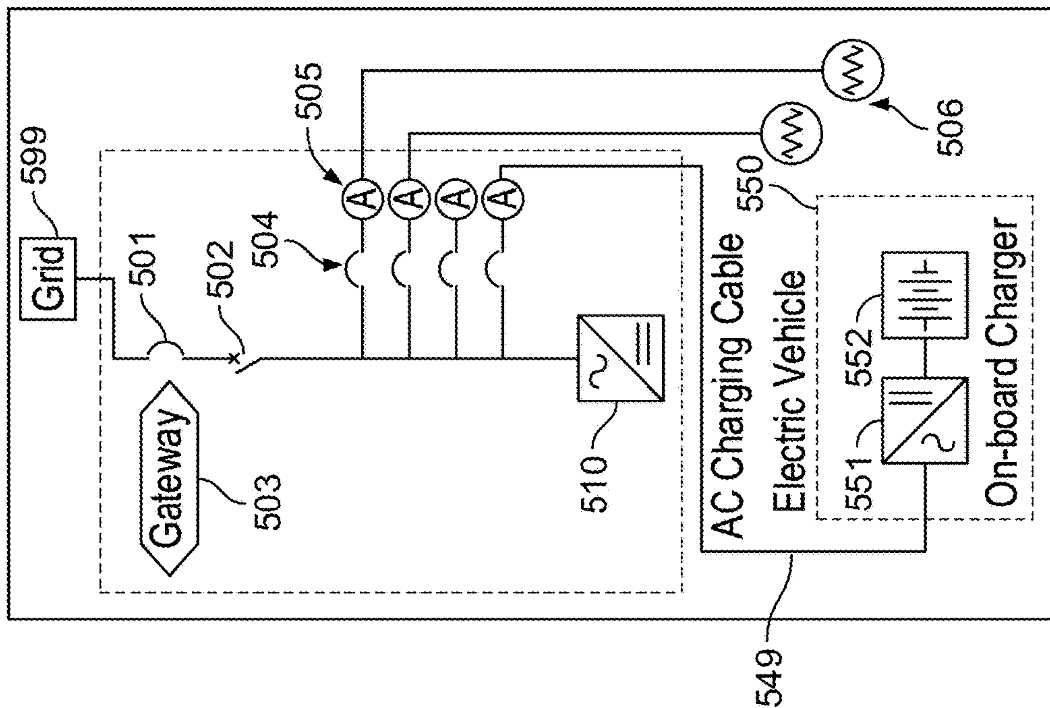
AC-coupled Vehicle Charging
