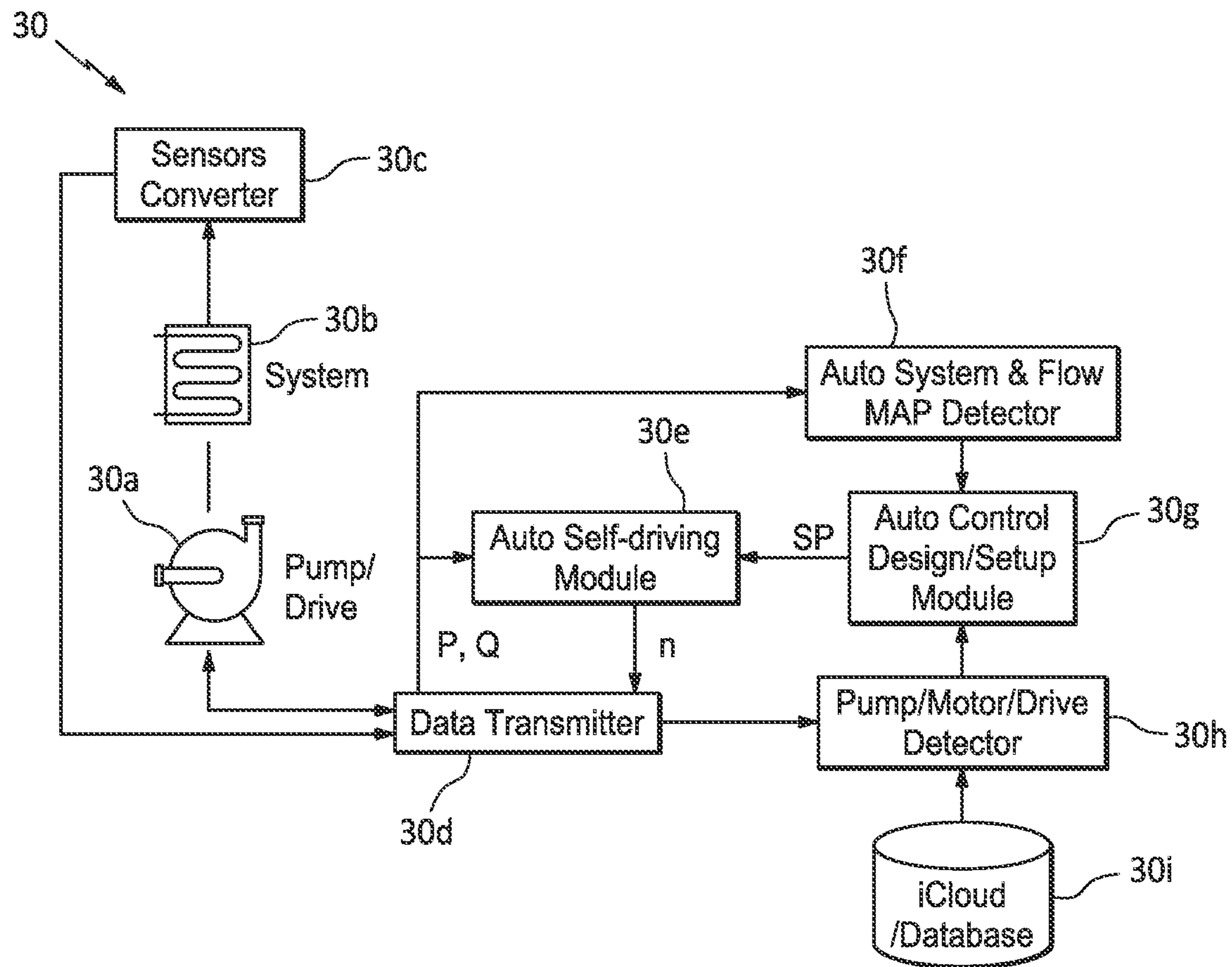
FIG. 3 : ASD-pumps functional model.
