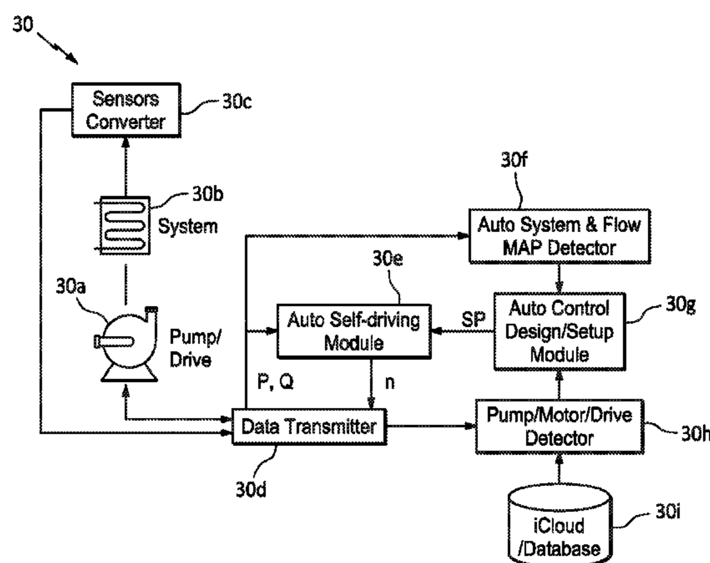
ASD-pumps functional model.
