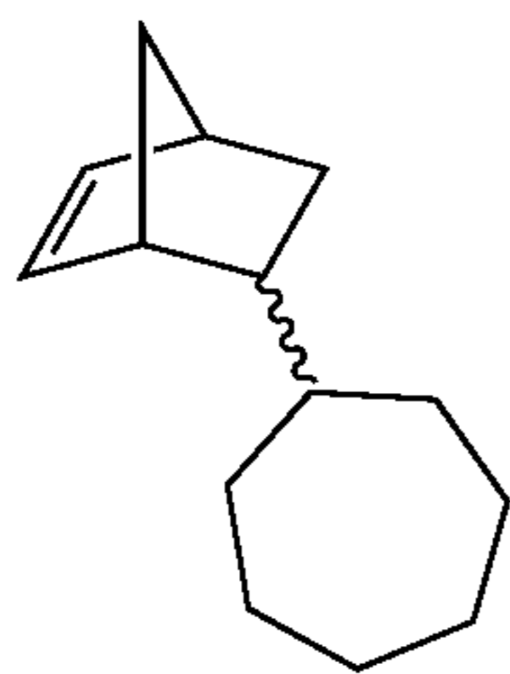
5-cycloheptylbicyclo[2.2.1]hept-2-ene (NBCyHep).
