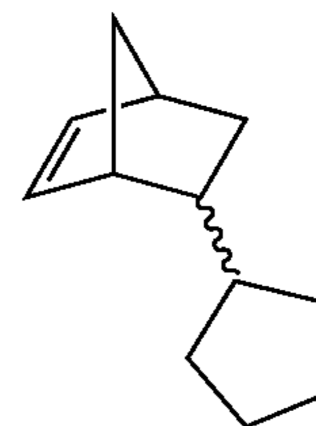
5-cyclopentylbicyclo[2.2.1]hept-2-ene (NBCyPen)
