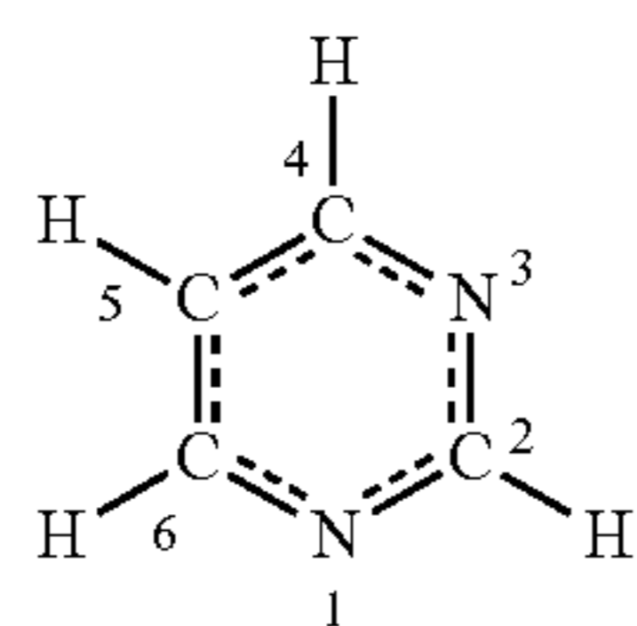
Pyrimidine
