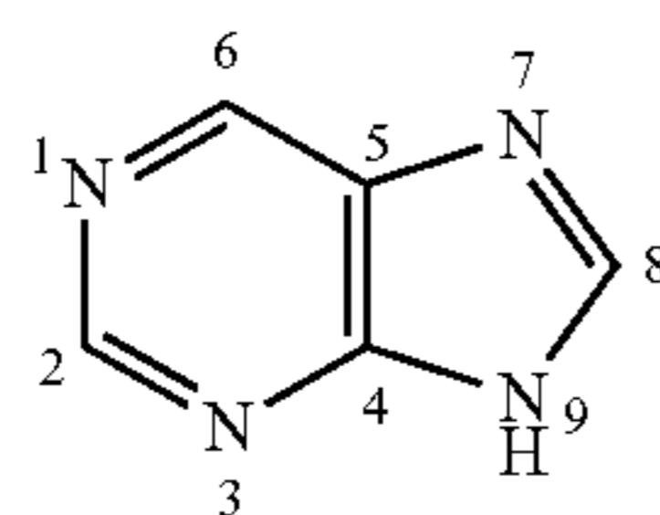
Purine
