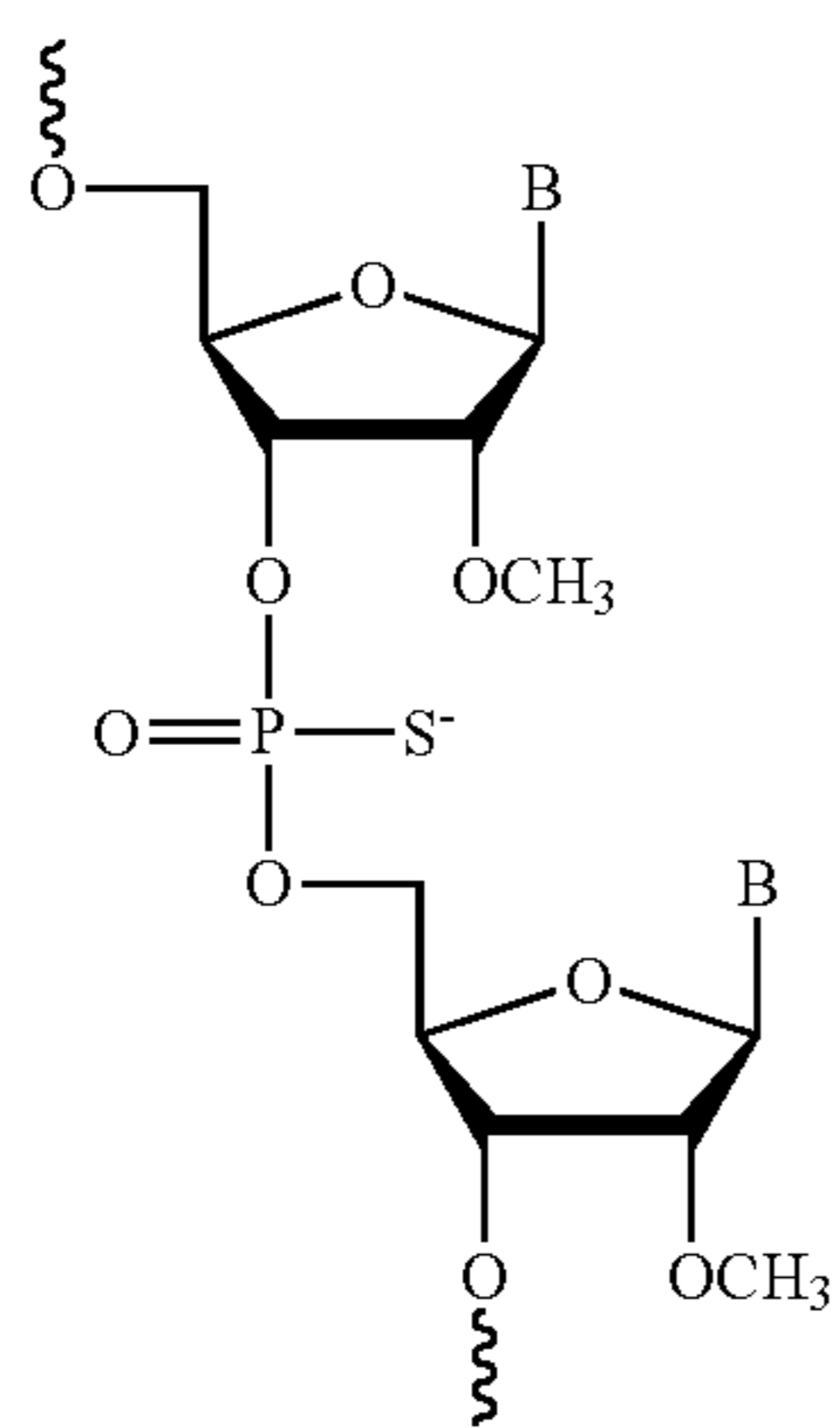
2'-O-Methyl PS
