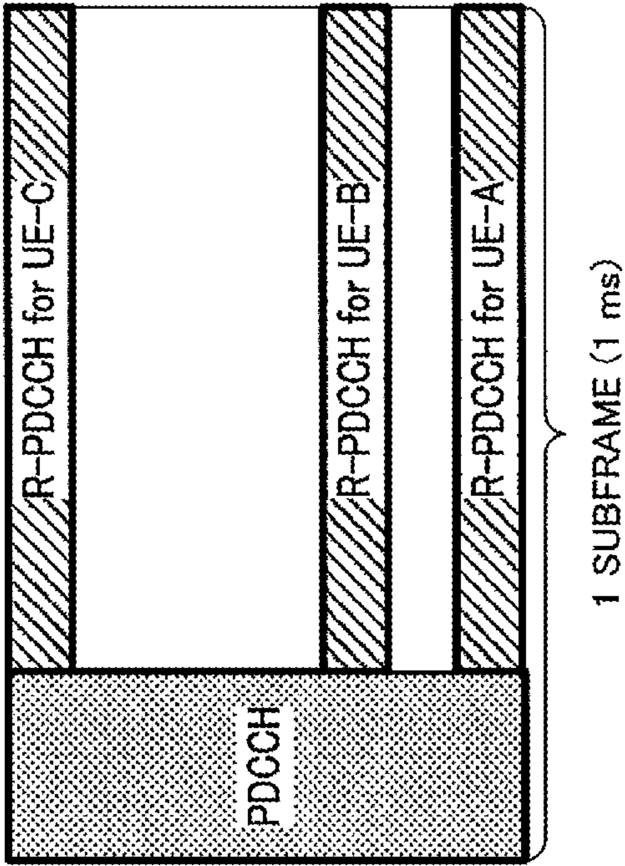
FIG.1A(FDM)
