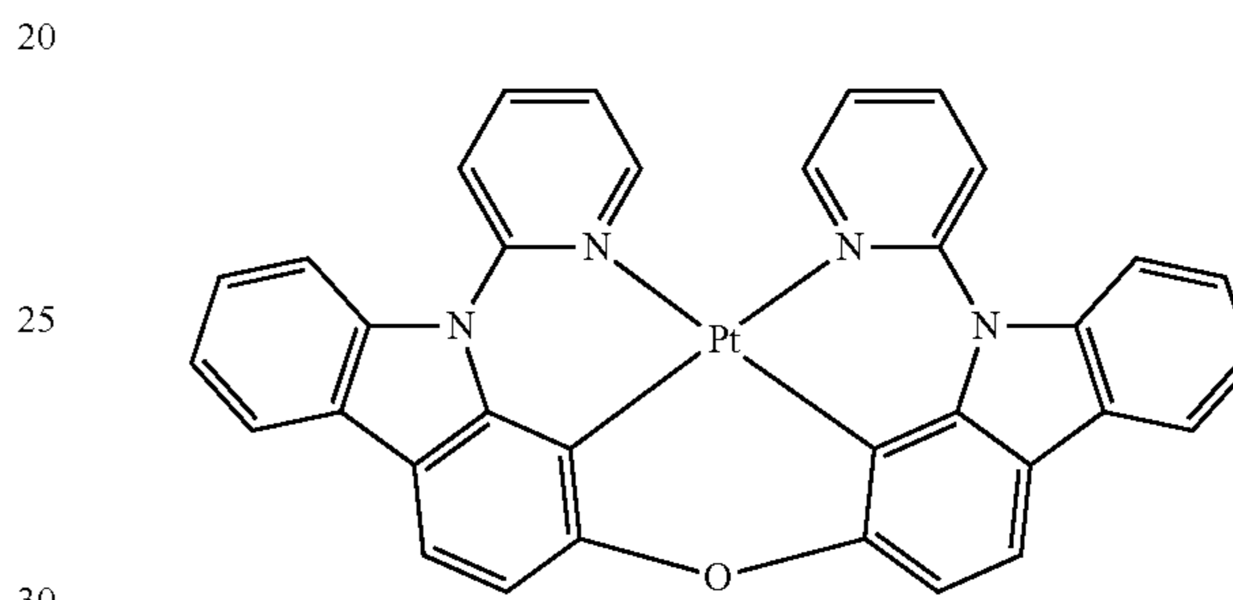
PtNON (EML Emitting Material)
