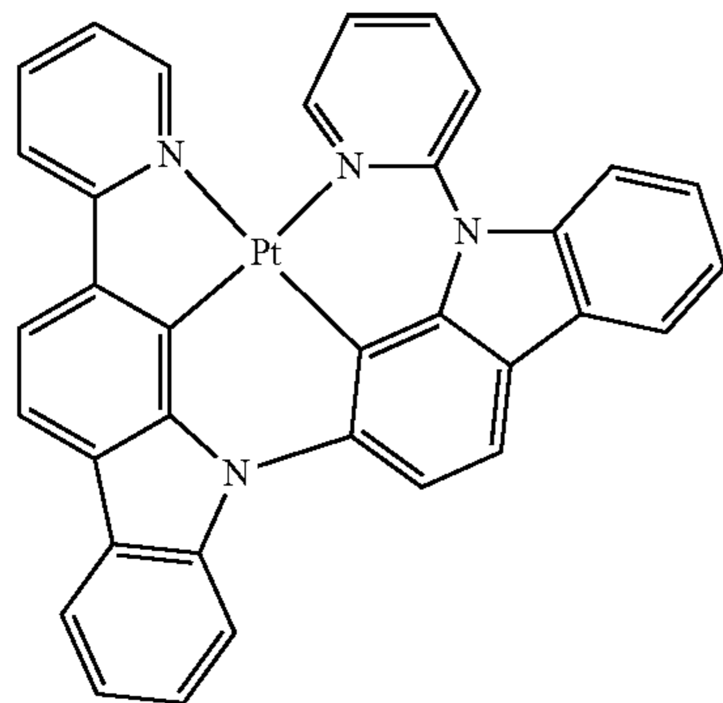
PtN3N (EML Emitting Material)
