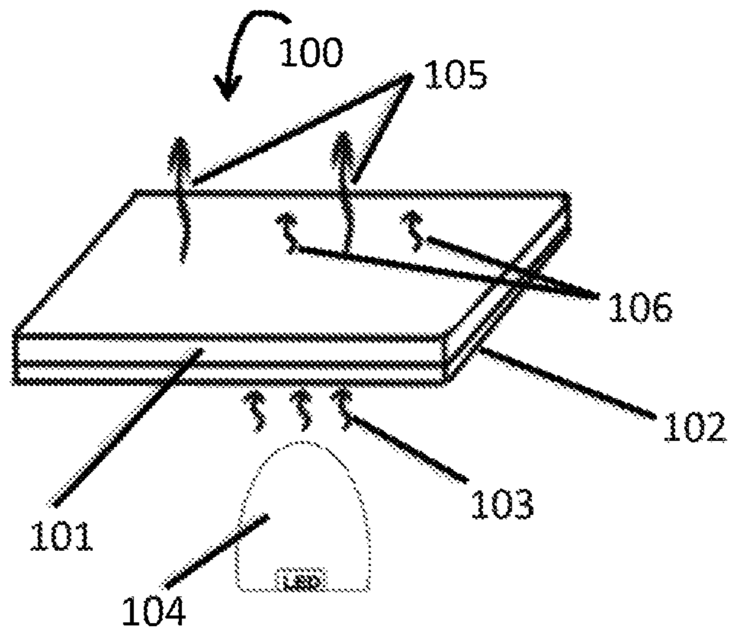
Figure 1 (prior art)
