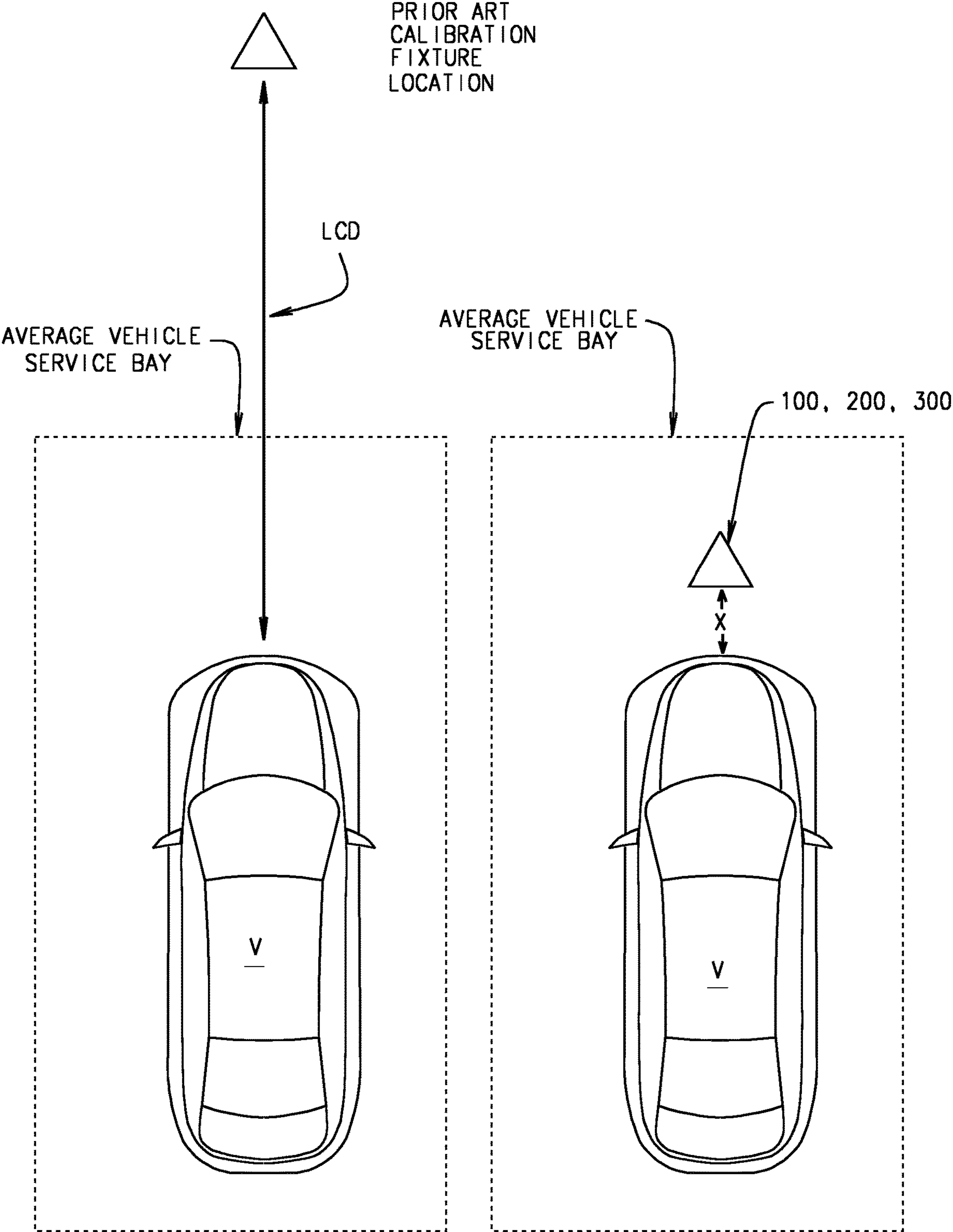
FIG. 10 PRIOR ART
