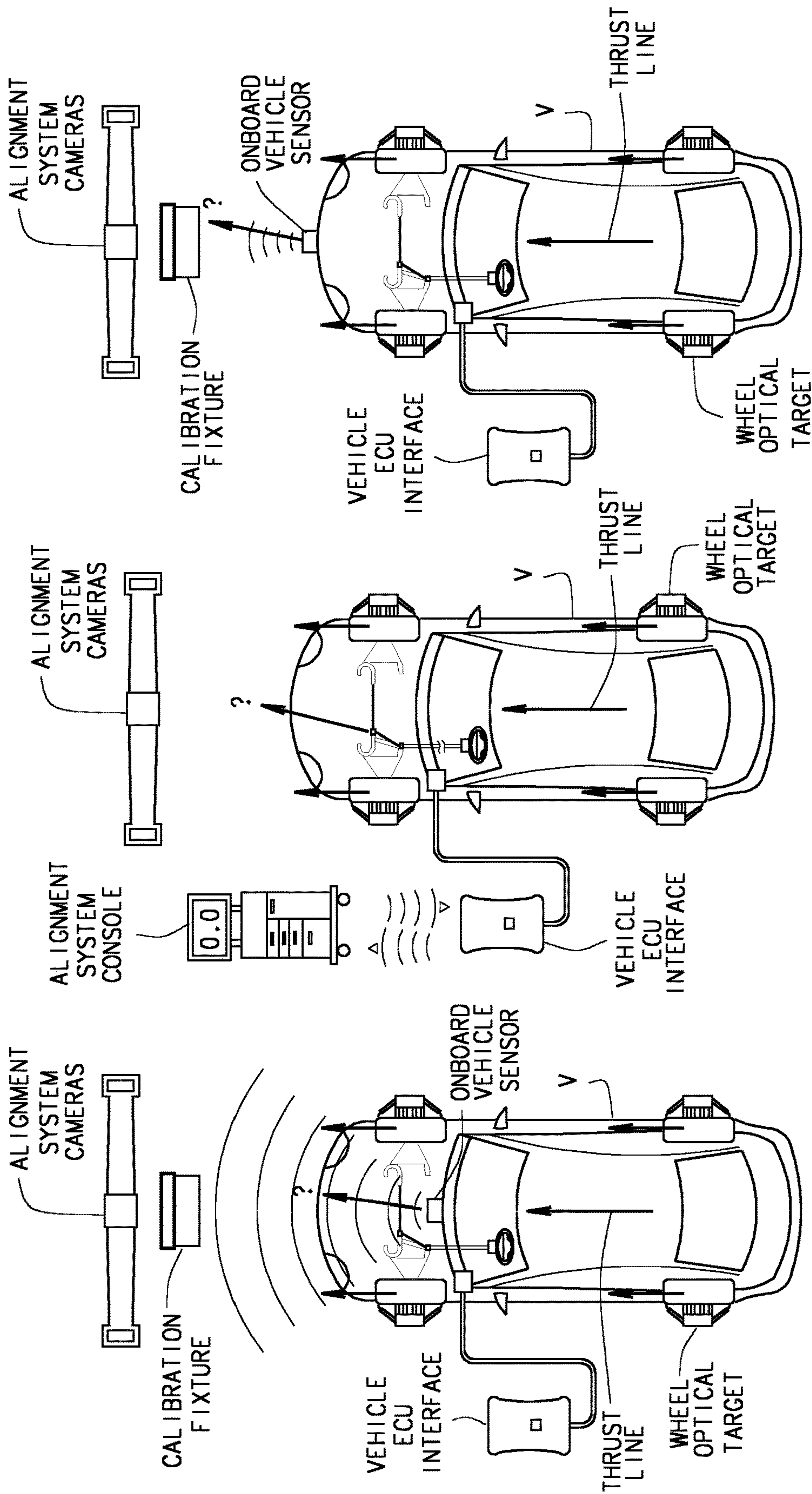
FIG. 1 PRIOR ART
