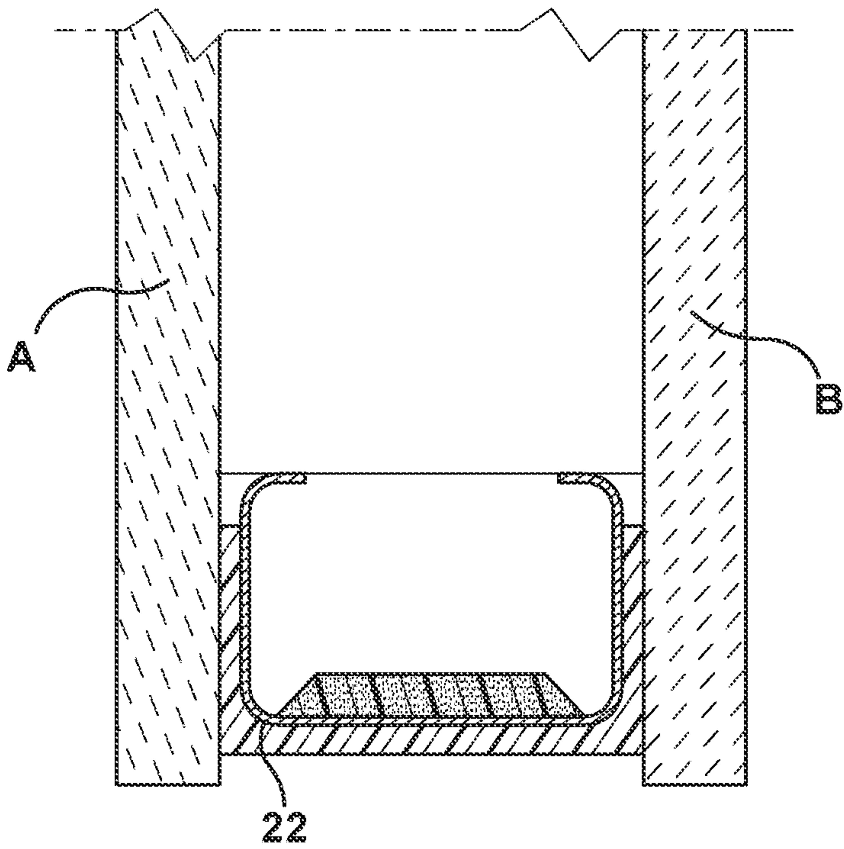
Fig. 3 (PRIOR ART)
