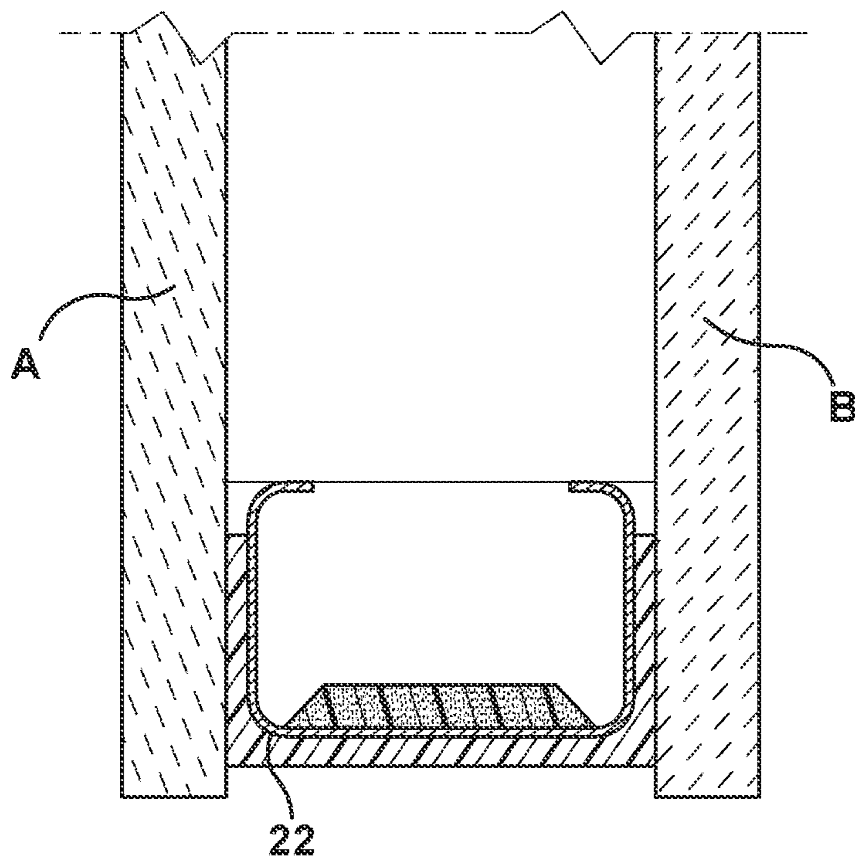
Fig. 3 (PRIOR ART)
