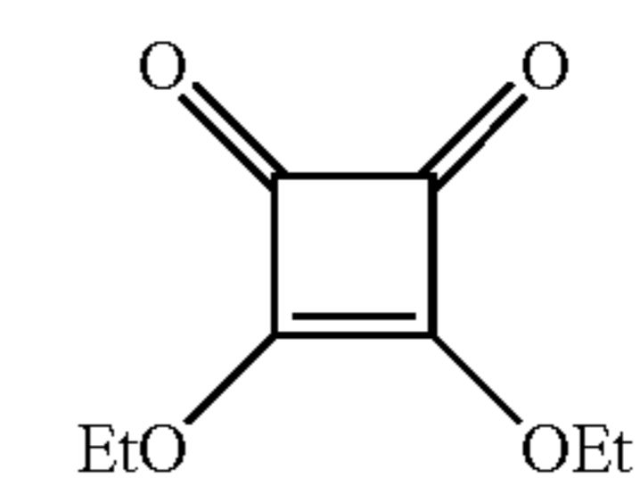
Squaric acid
