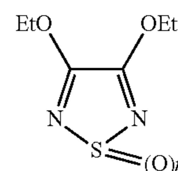
Dithiadiazoleoxide
