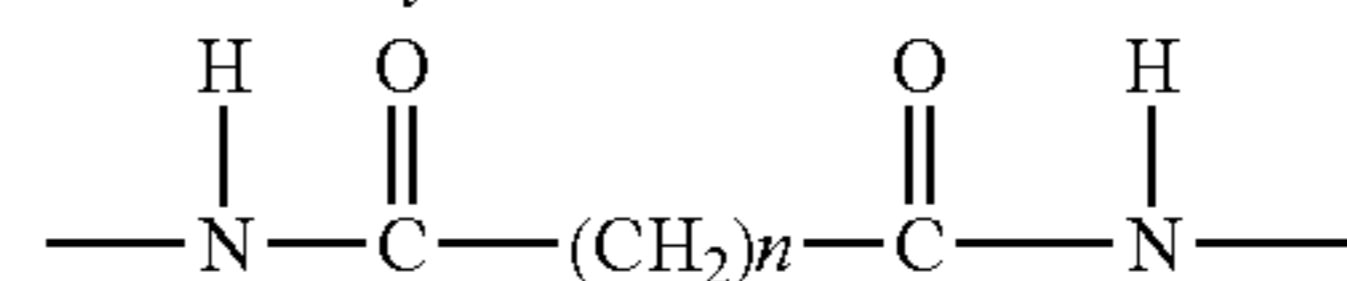
Coupling via bifunctional NHS reagent
