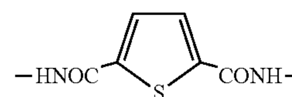
Acylation via Thiofuran
