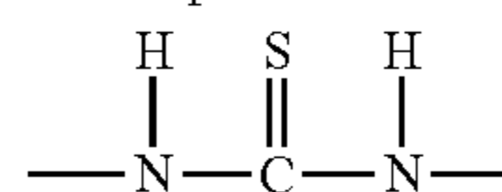
Thiourea
