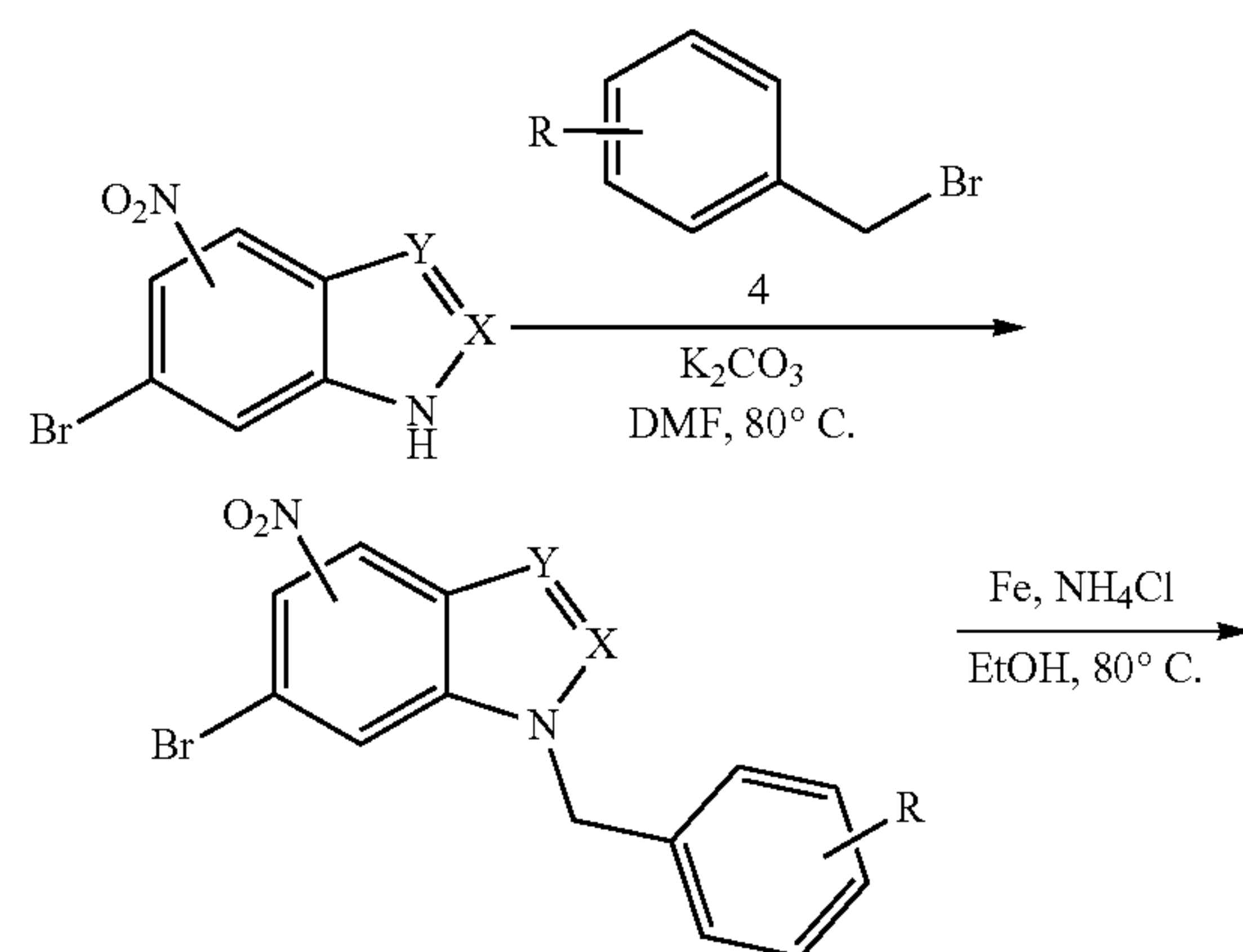
Scheme 2
