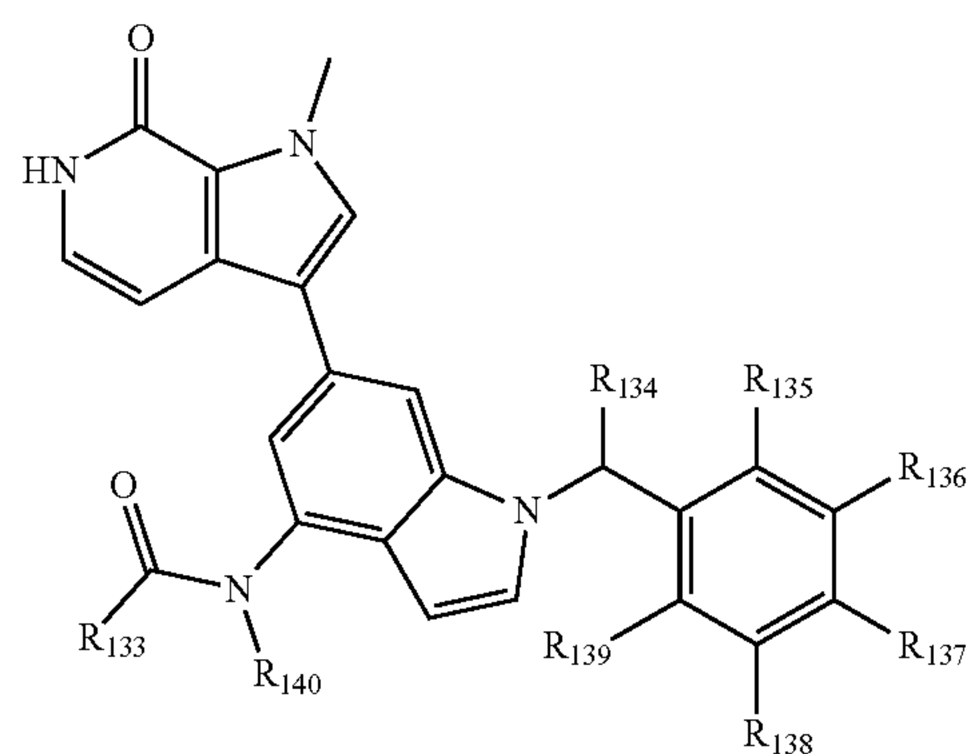
Formula XVI
