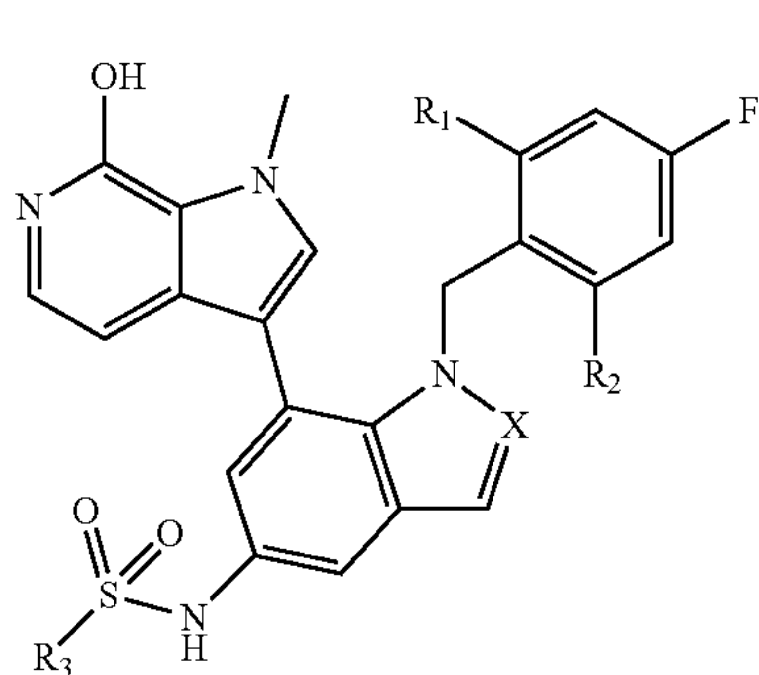
Formula XXIV
