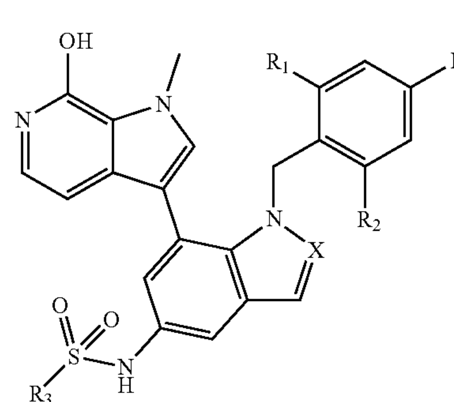
Formula XXIV
