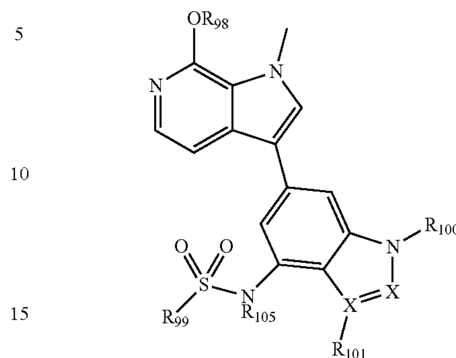
Formula VII
