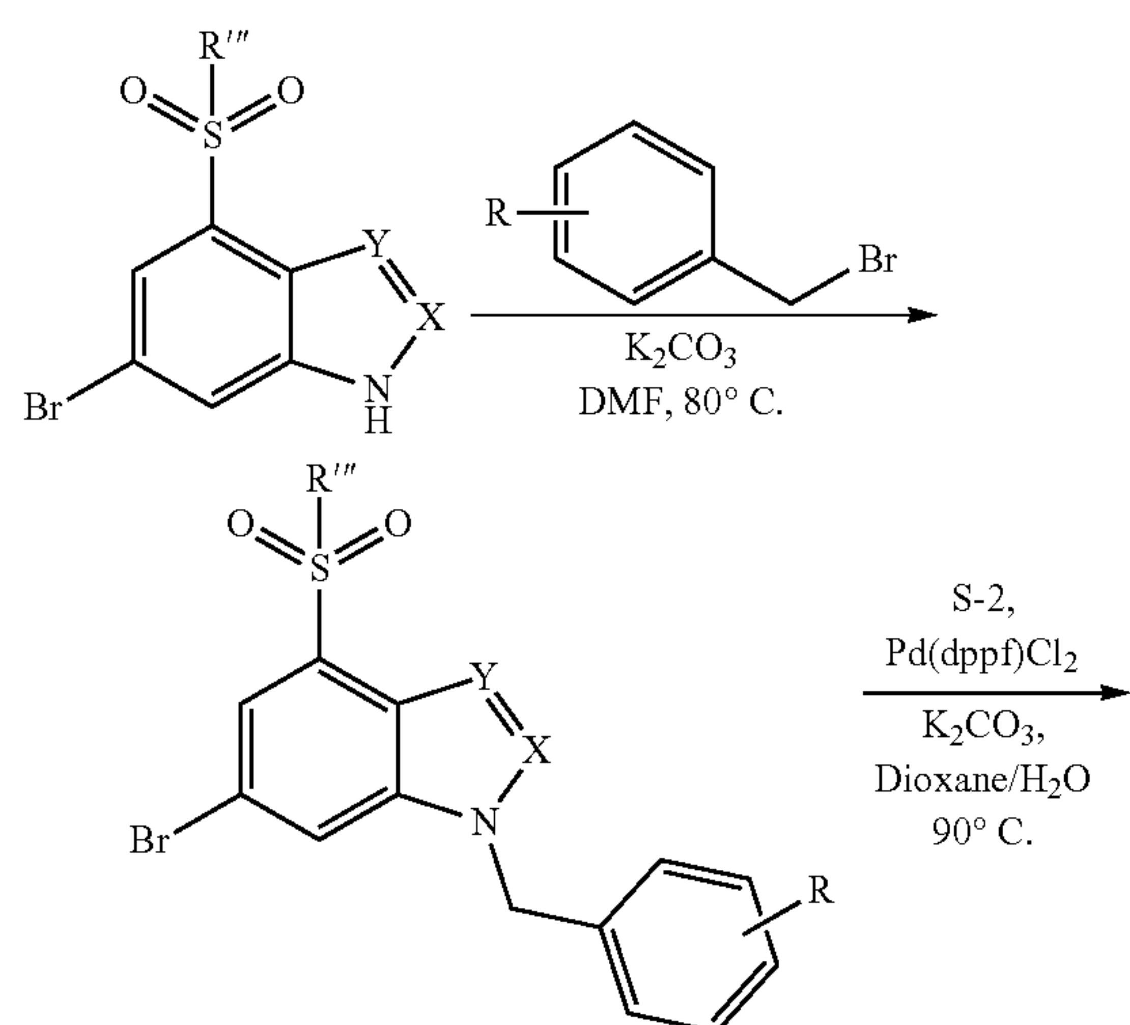
Scheme 4
