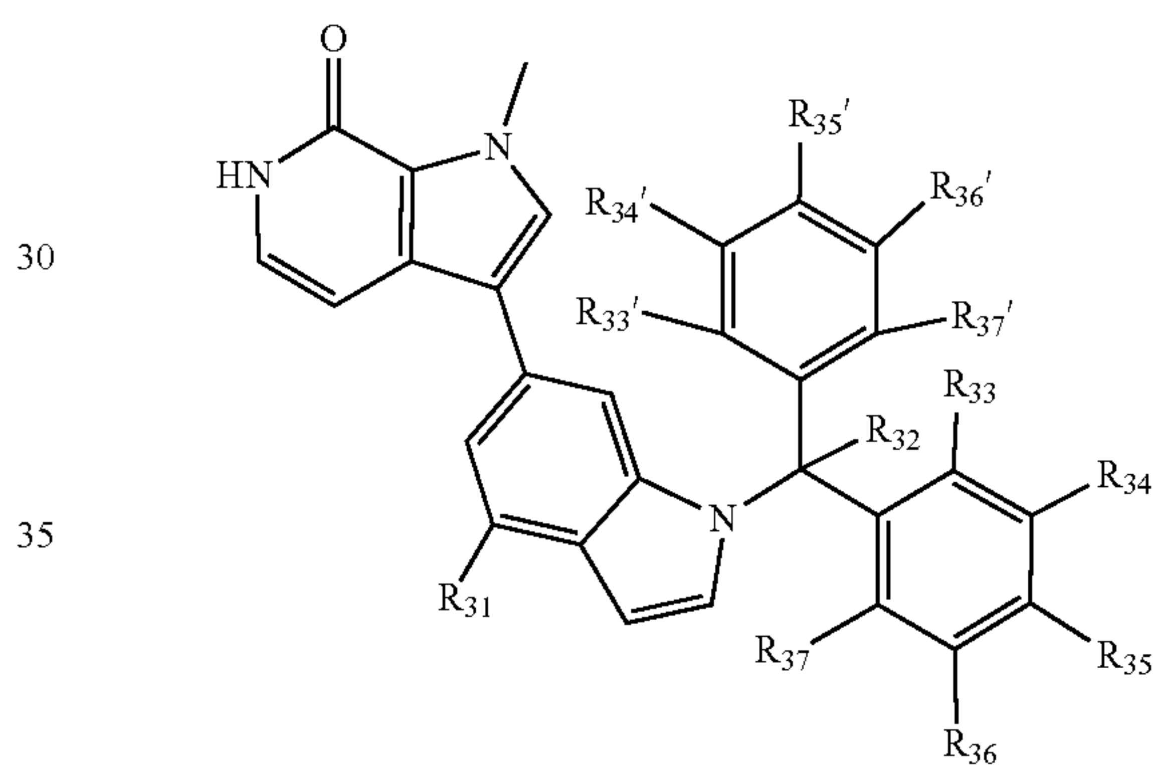
Formula XXI
