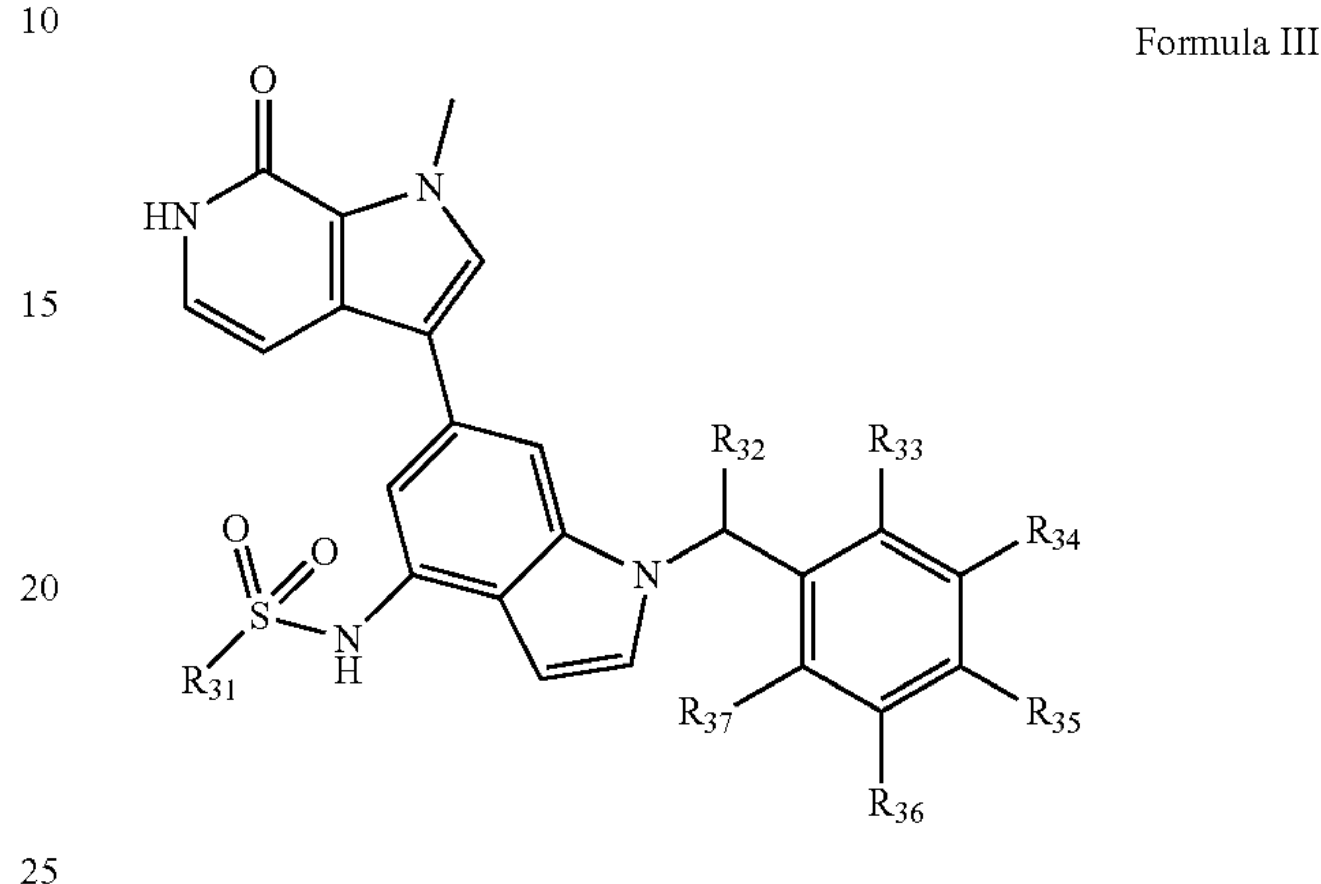
Formula II
