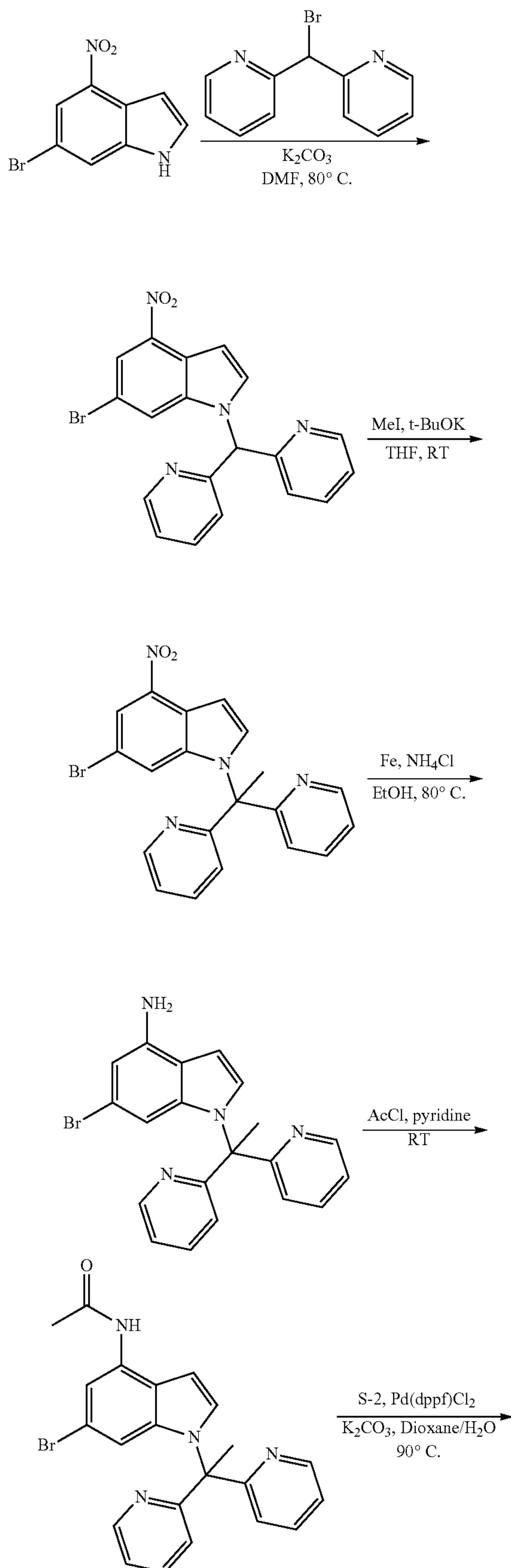
Scheme 10
