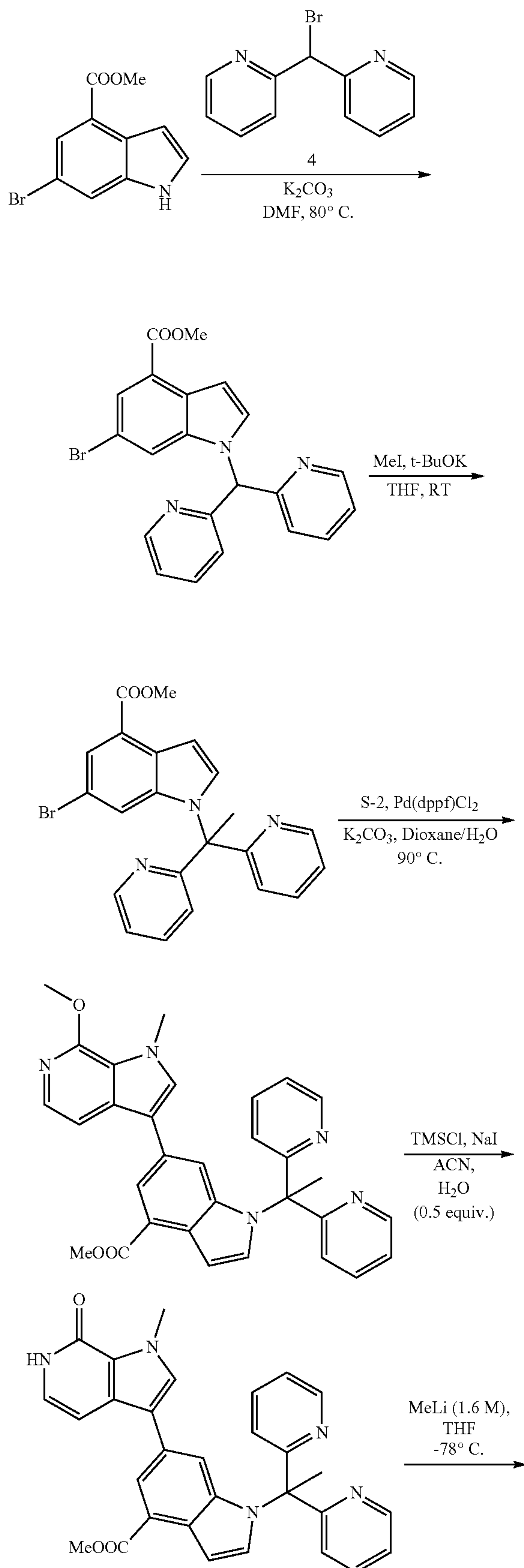
Scheme 12
