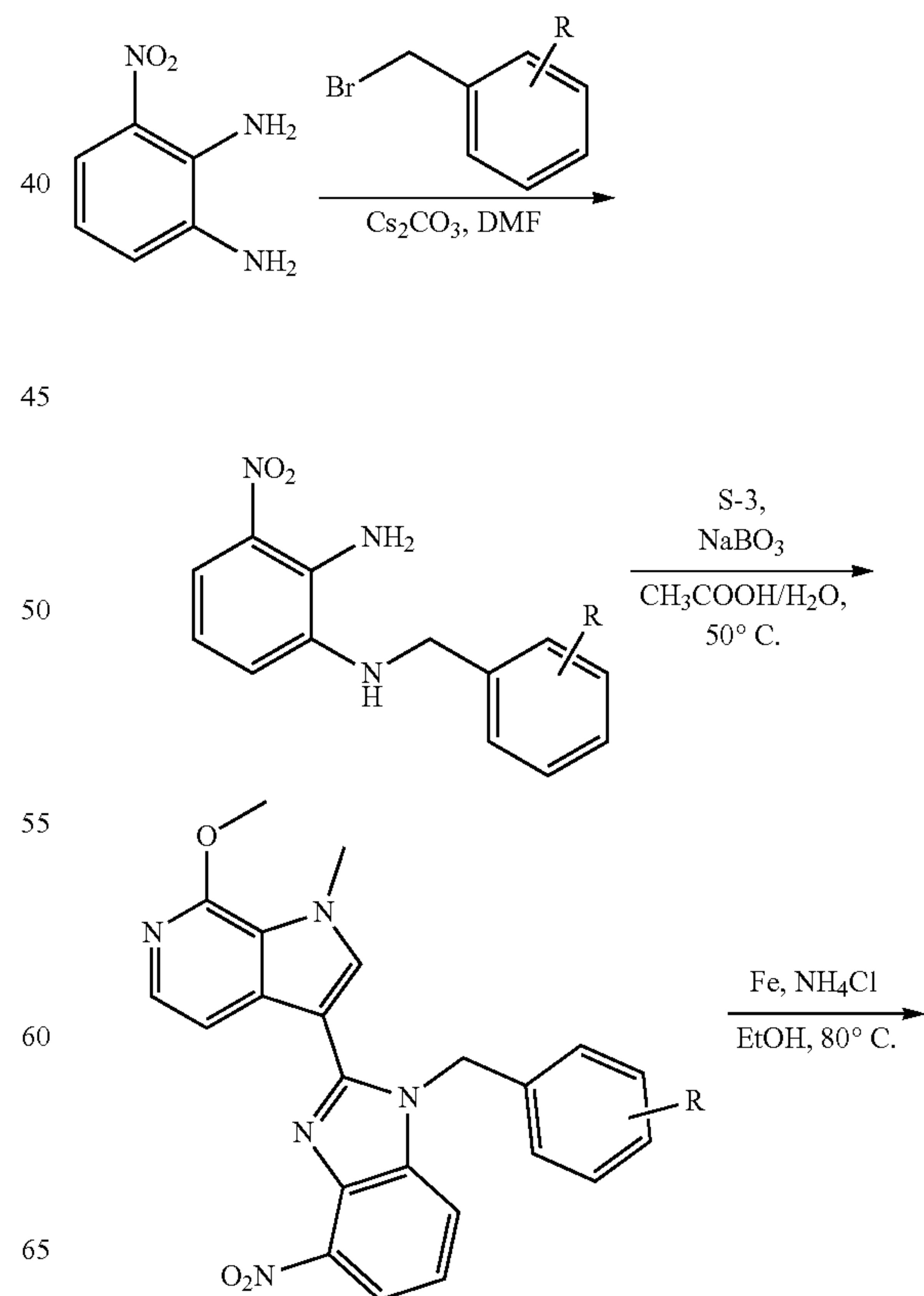
Scheme 5
