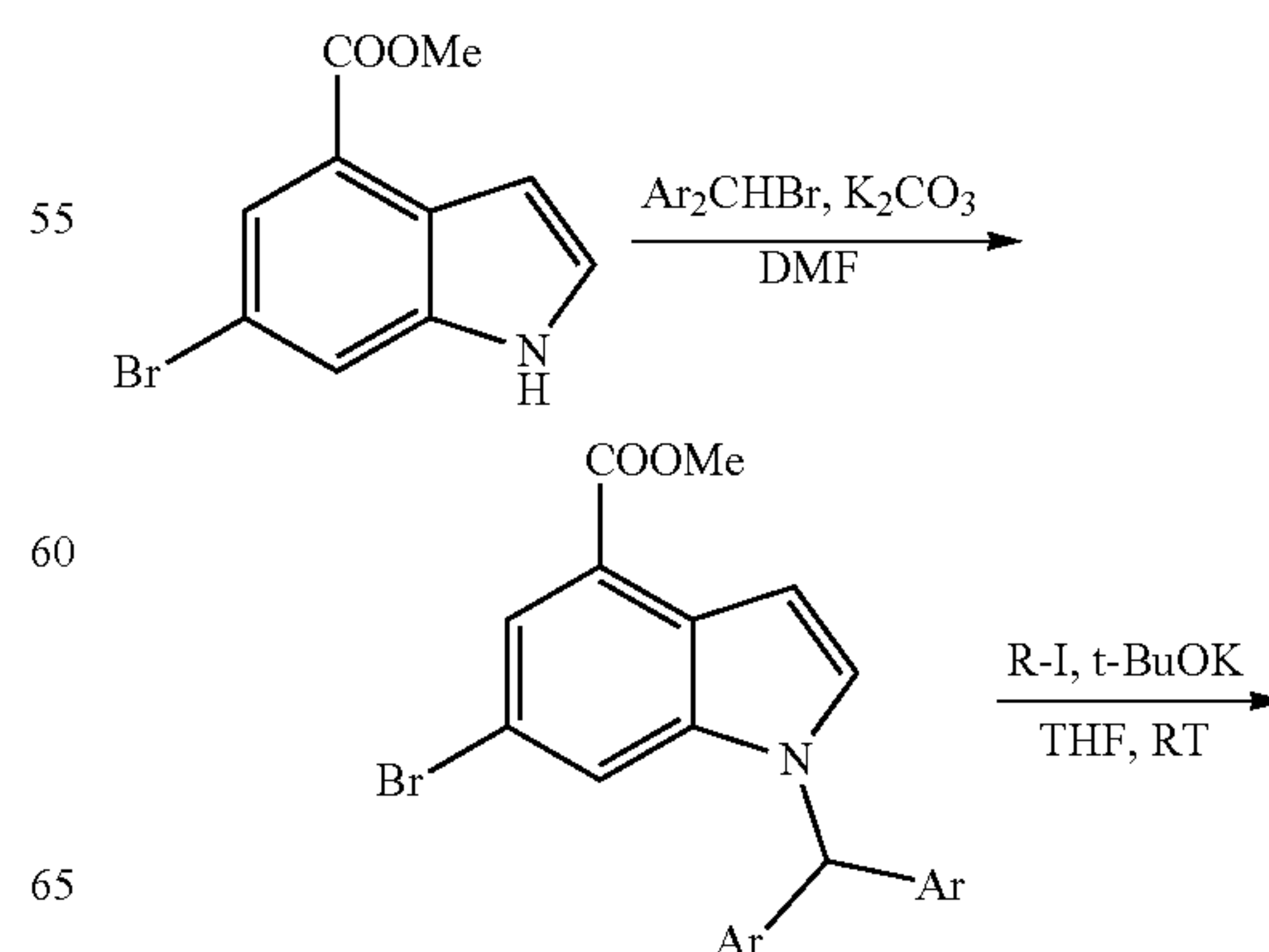
Scheme 3
