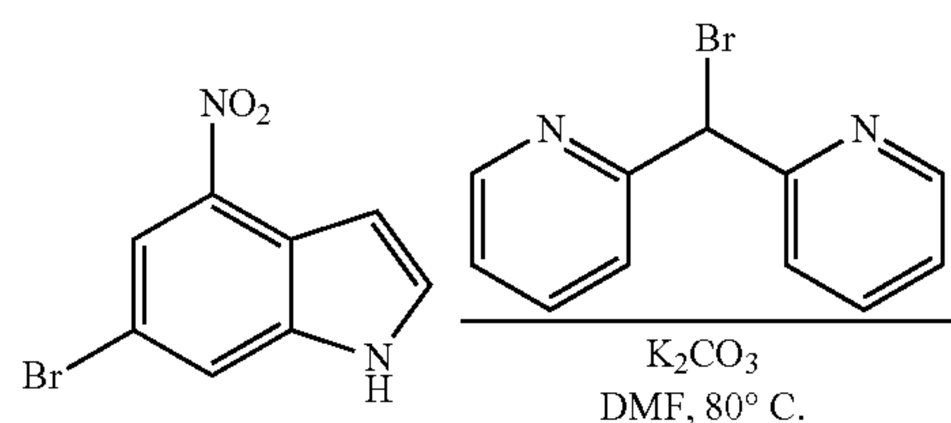
Scheme 11
