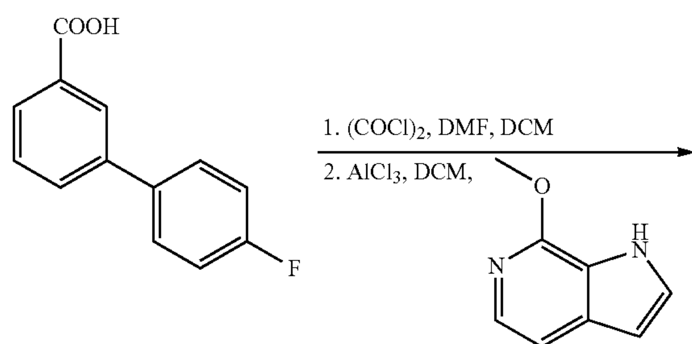
Scheme 6
