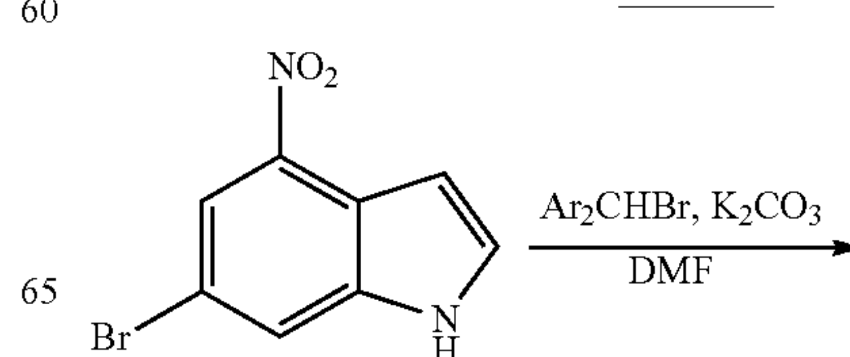
Scheme 7
