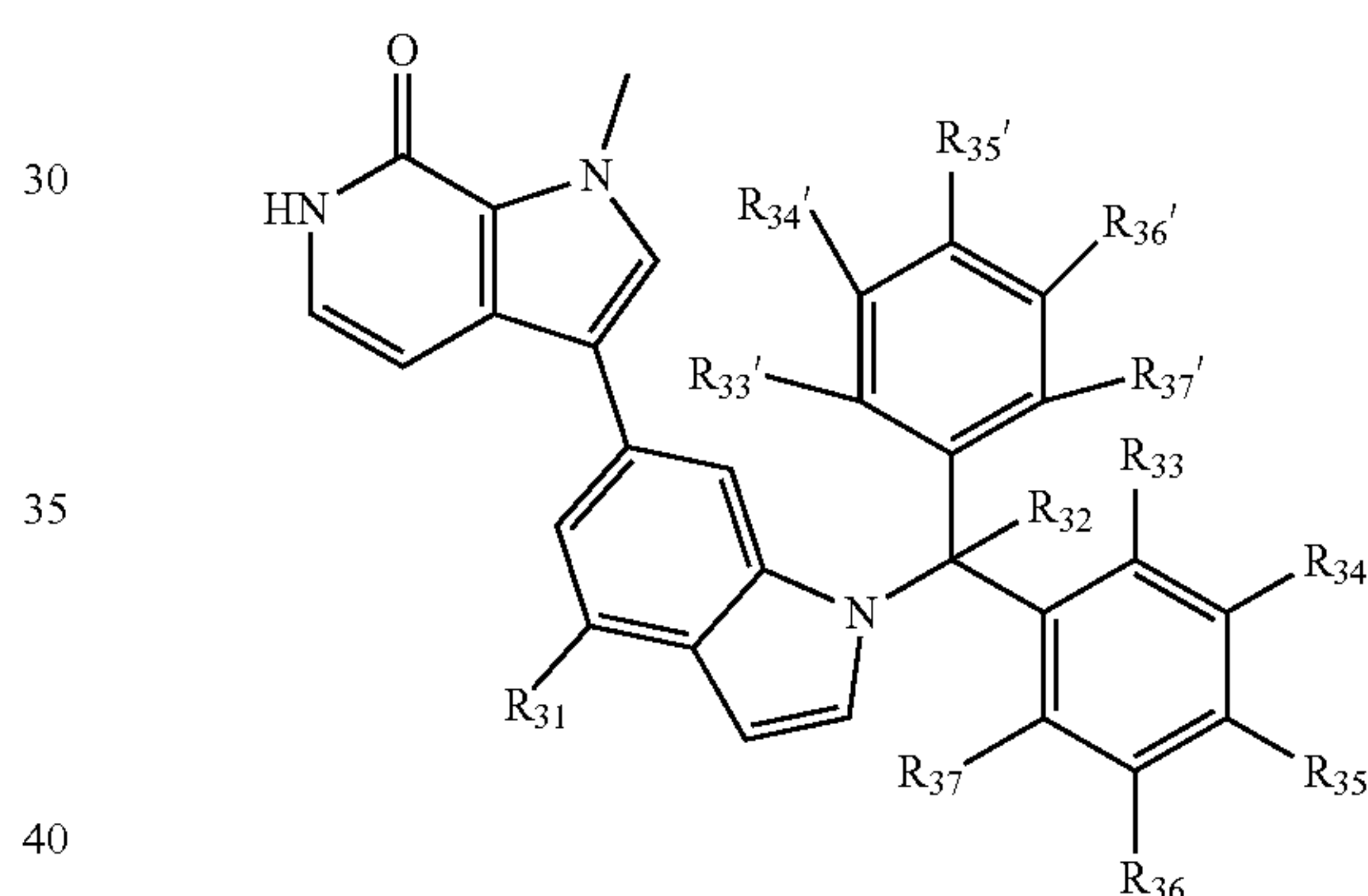
Formula XXI
