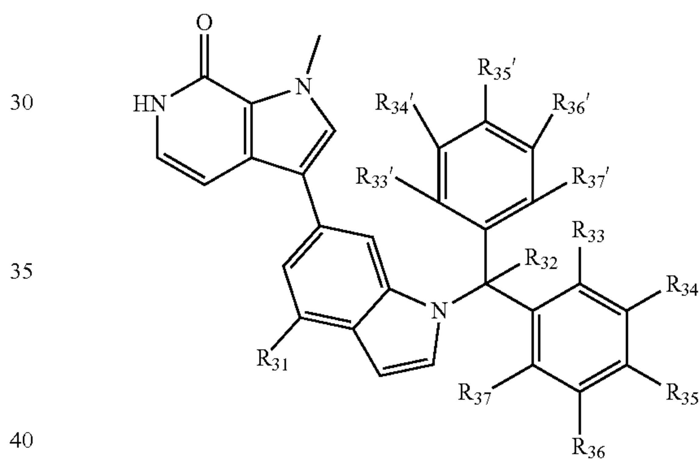
Formula XXI
