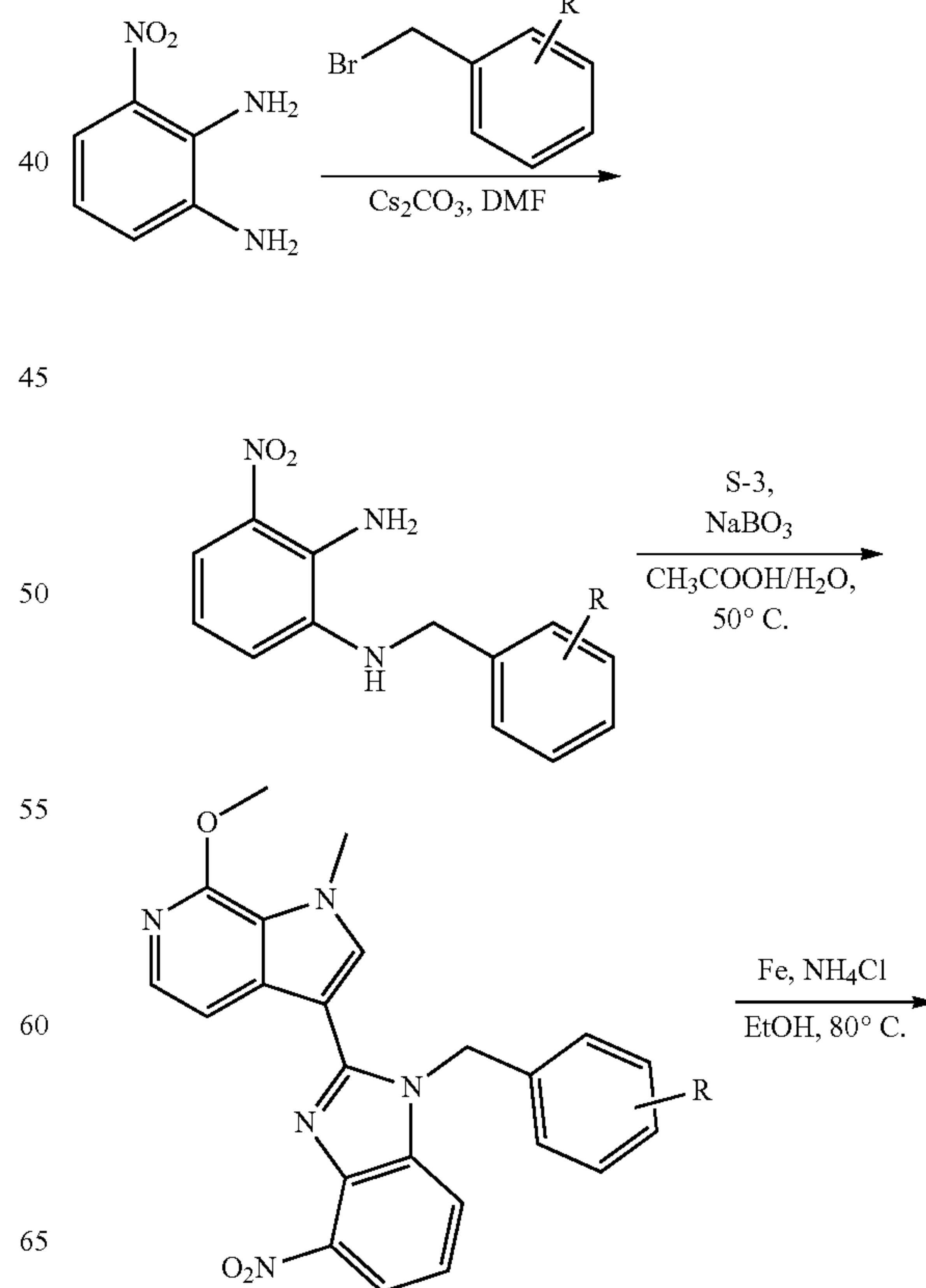
Scheme 5
