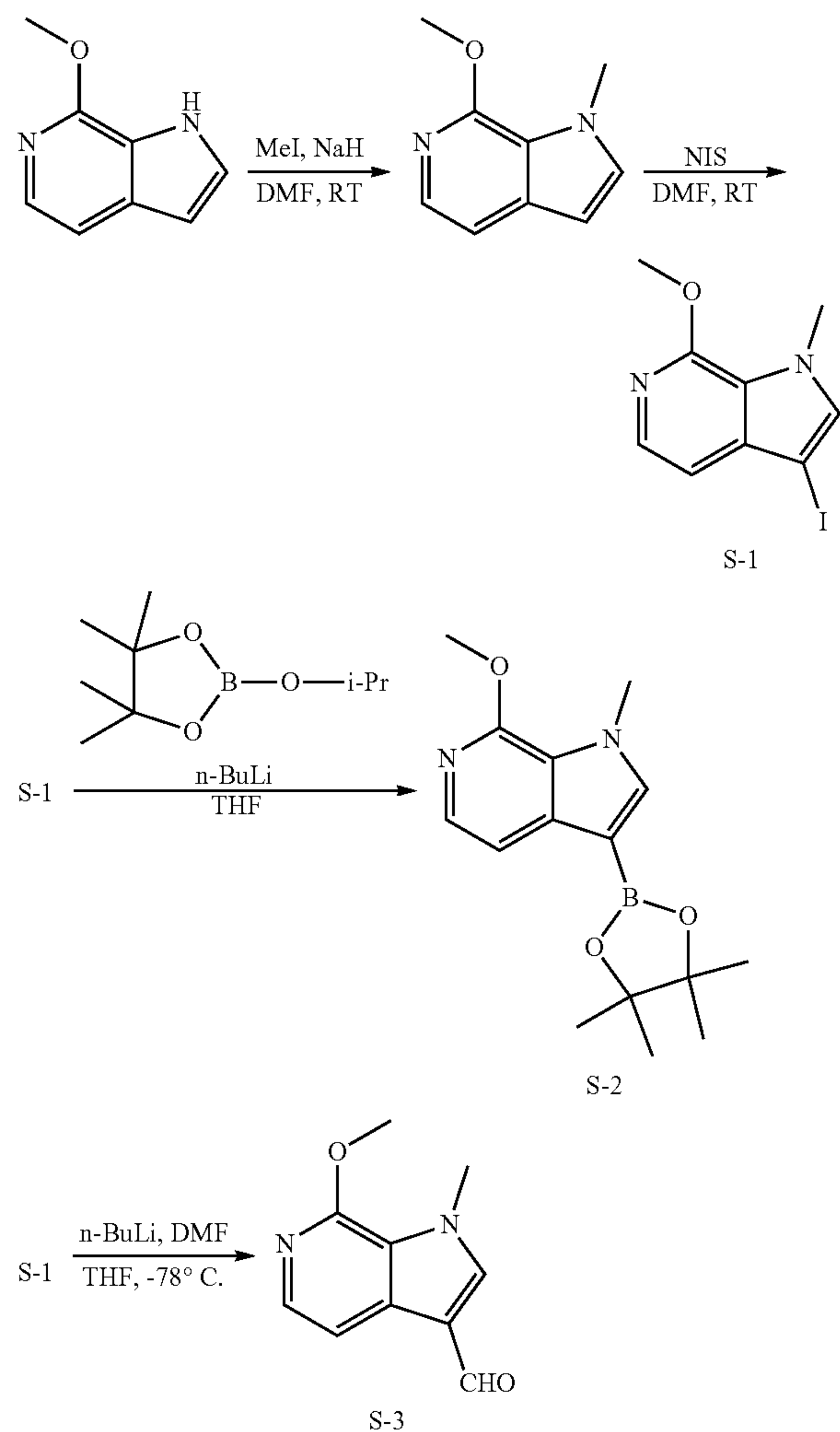
Scheme 1
