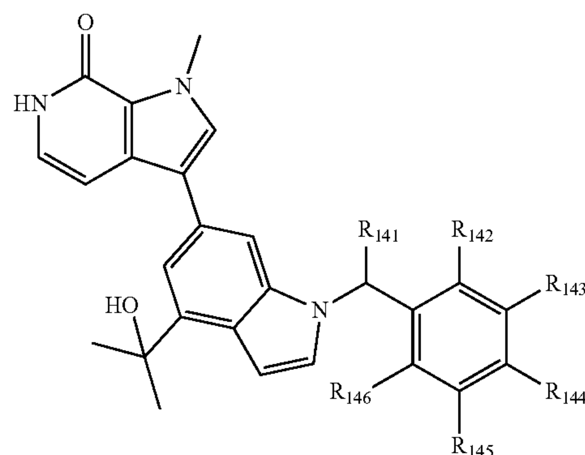
Formula XVII
