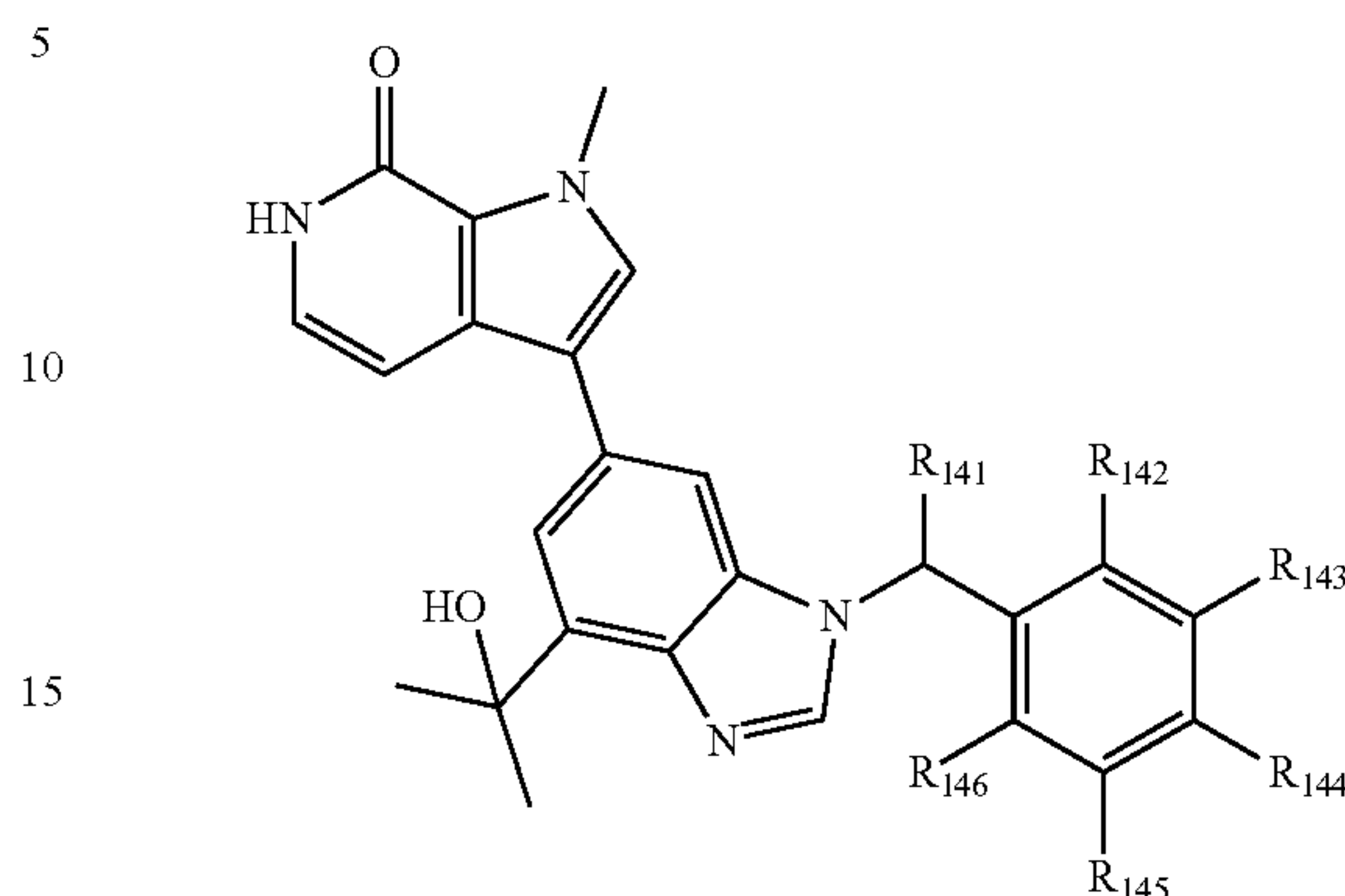
Formula XVII
