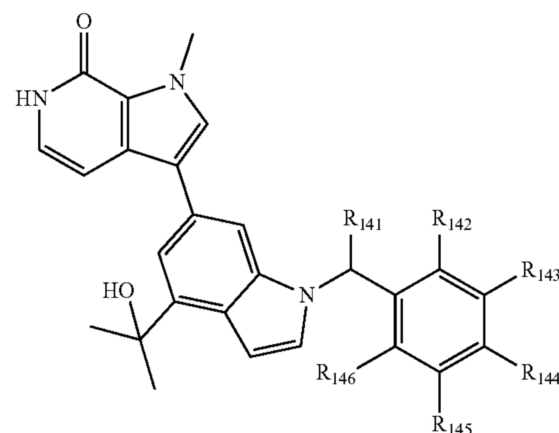
Formula XVII
