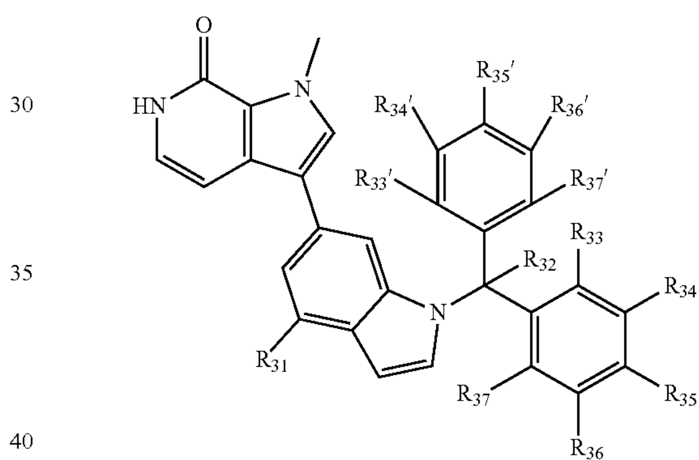
Formula XXI
