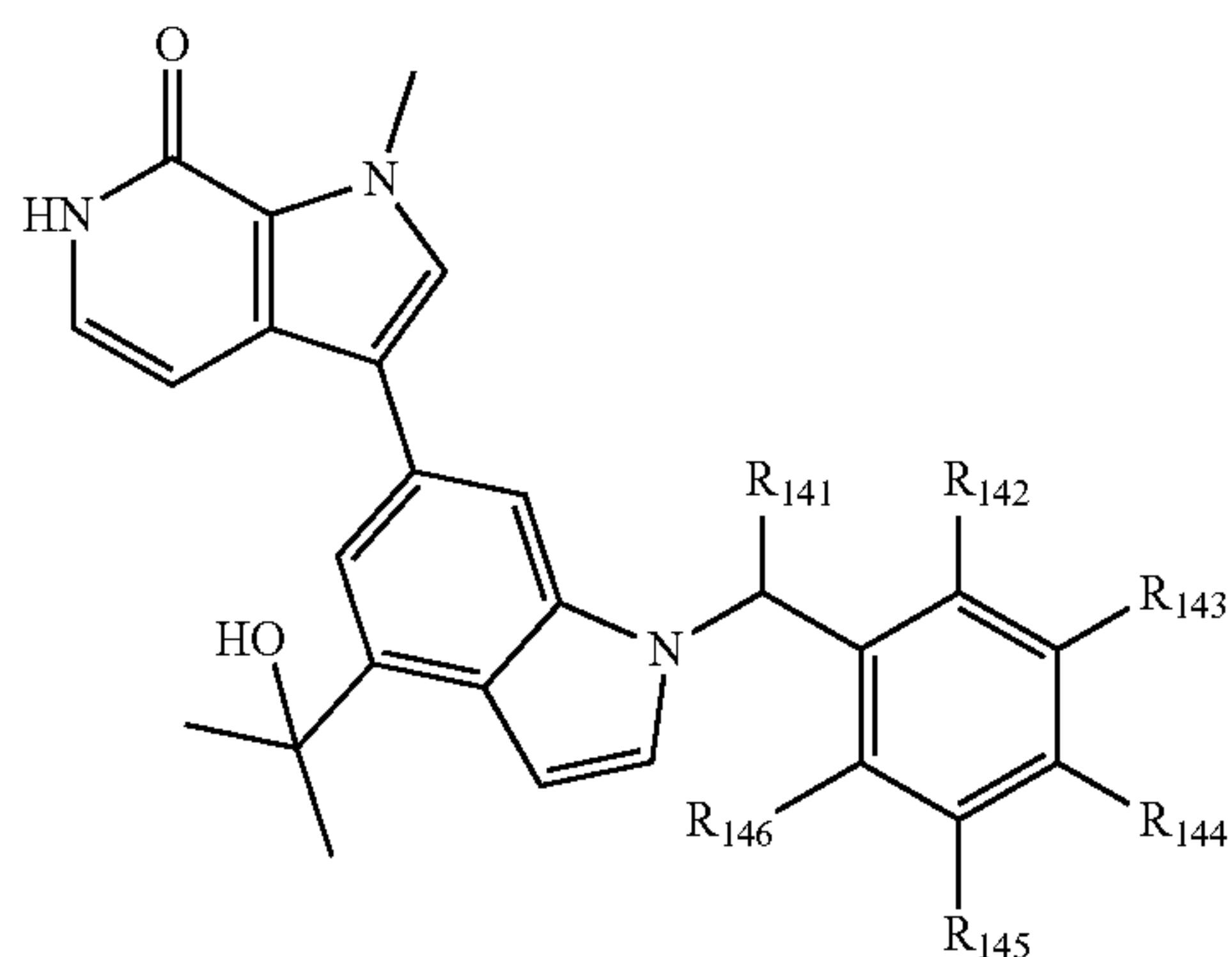
Formula XVII
