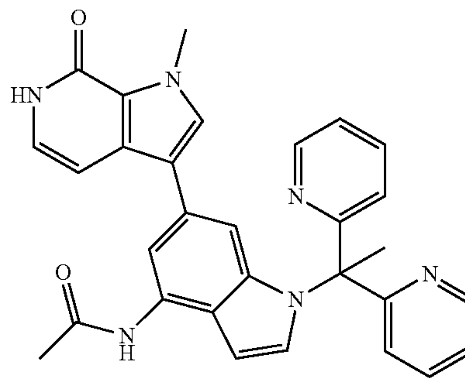
N-(1-(1,1-di(pyridin-2-yl)ethyl)-6-(1-methyl-7-oxo-6,7-dihydro-1H-pyrrolo[2,3-c]pyridin-3-yl)-1H-indol-4-yl)acetamide
