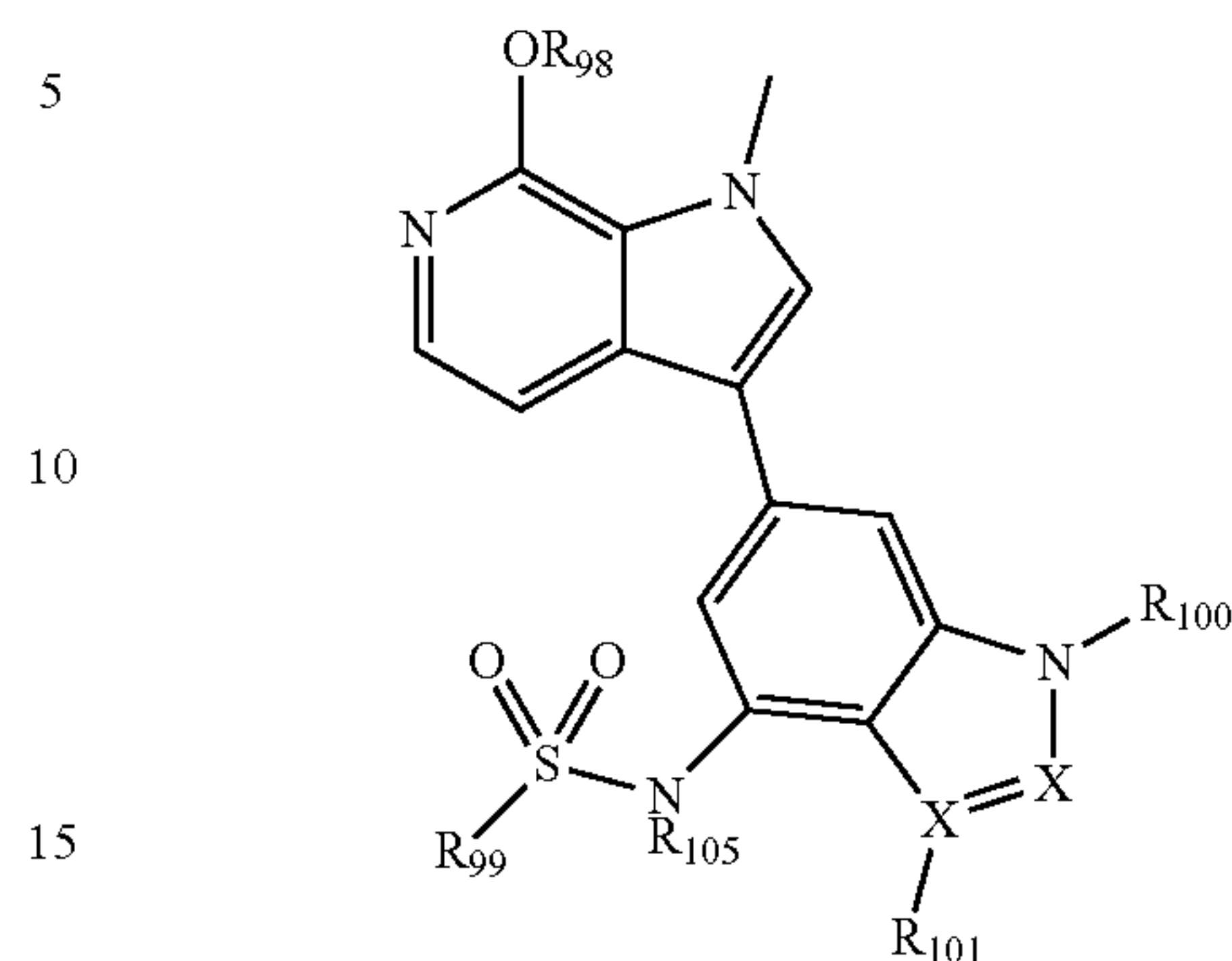
Formula VII
