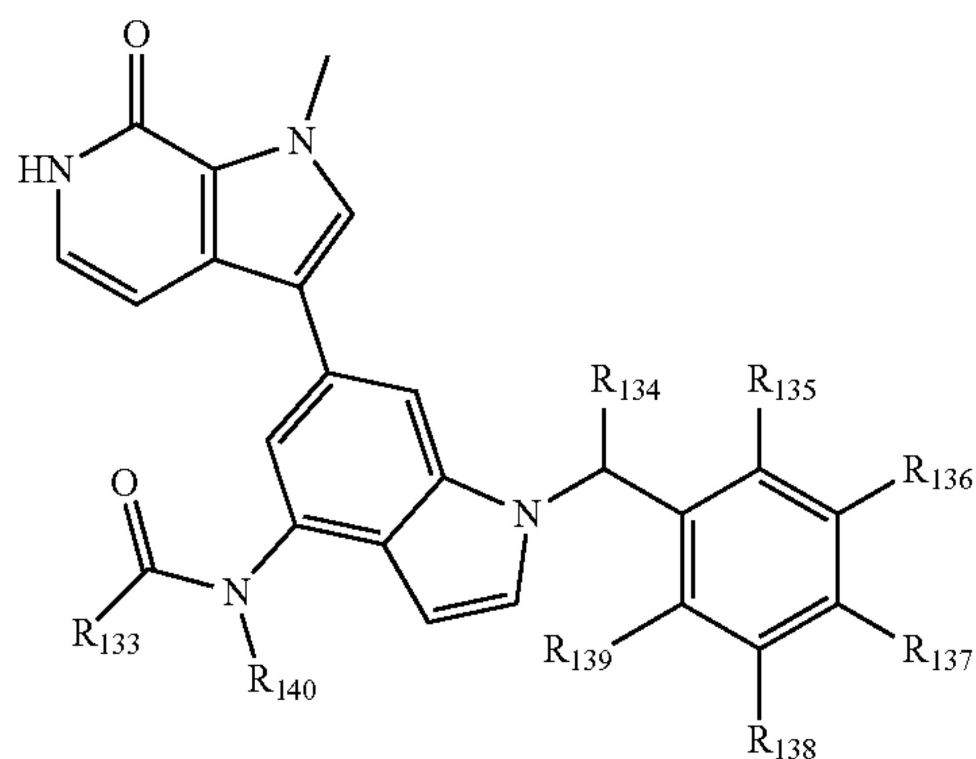
Formula XVI
