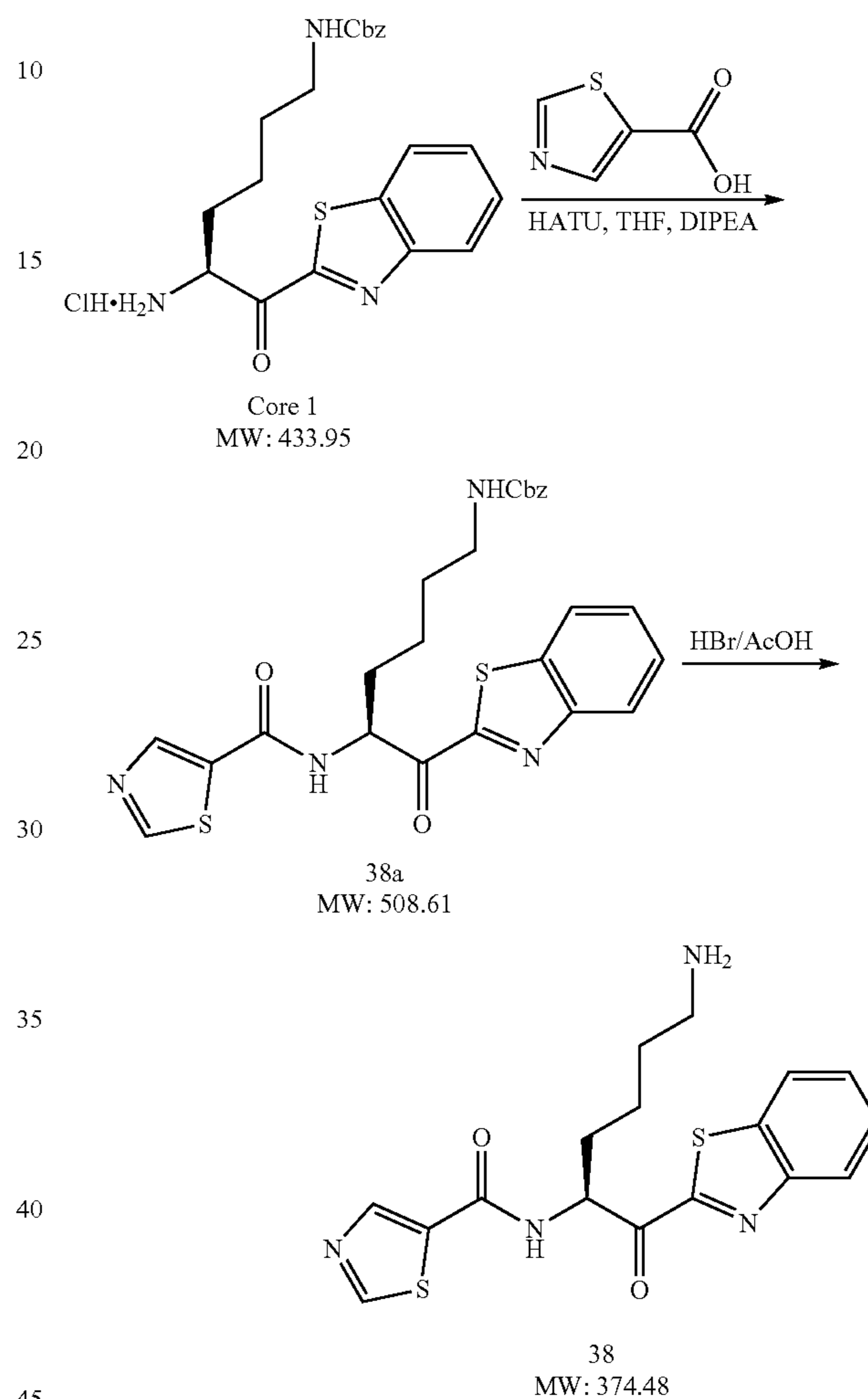
Scheme 29
