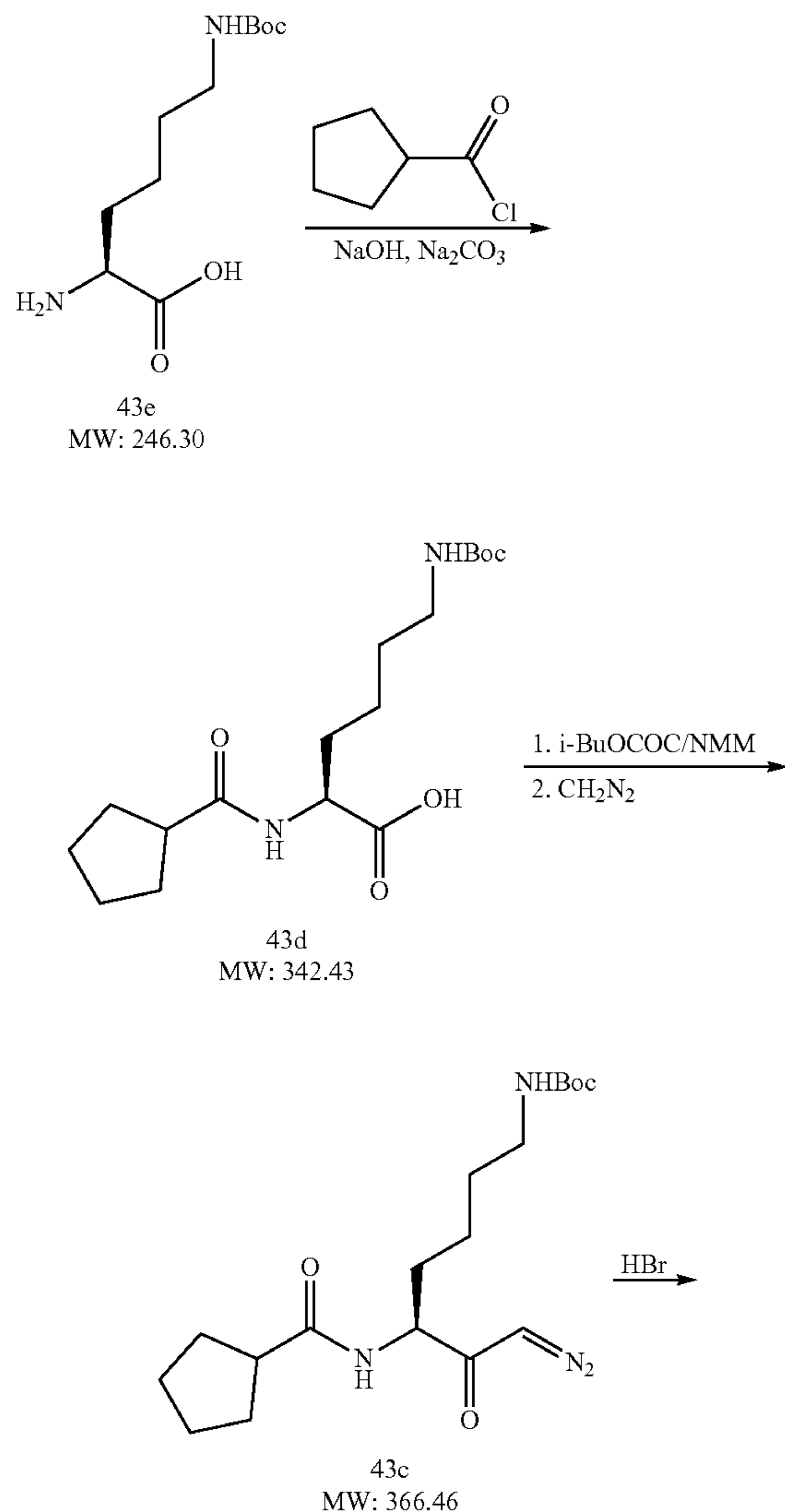
Scheme 34
