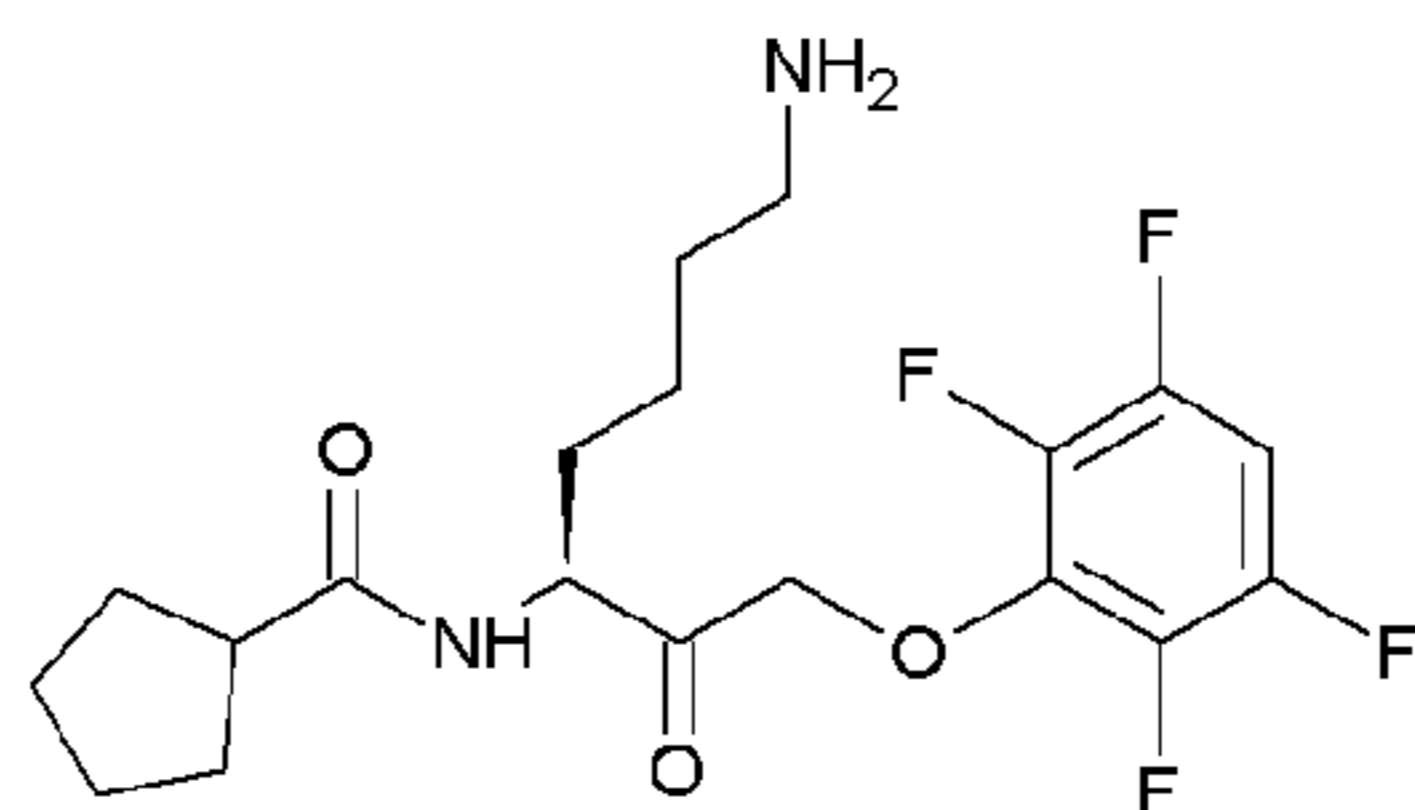
Compound 43
