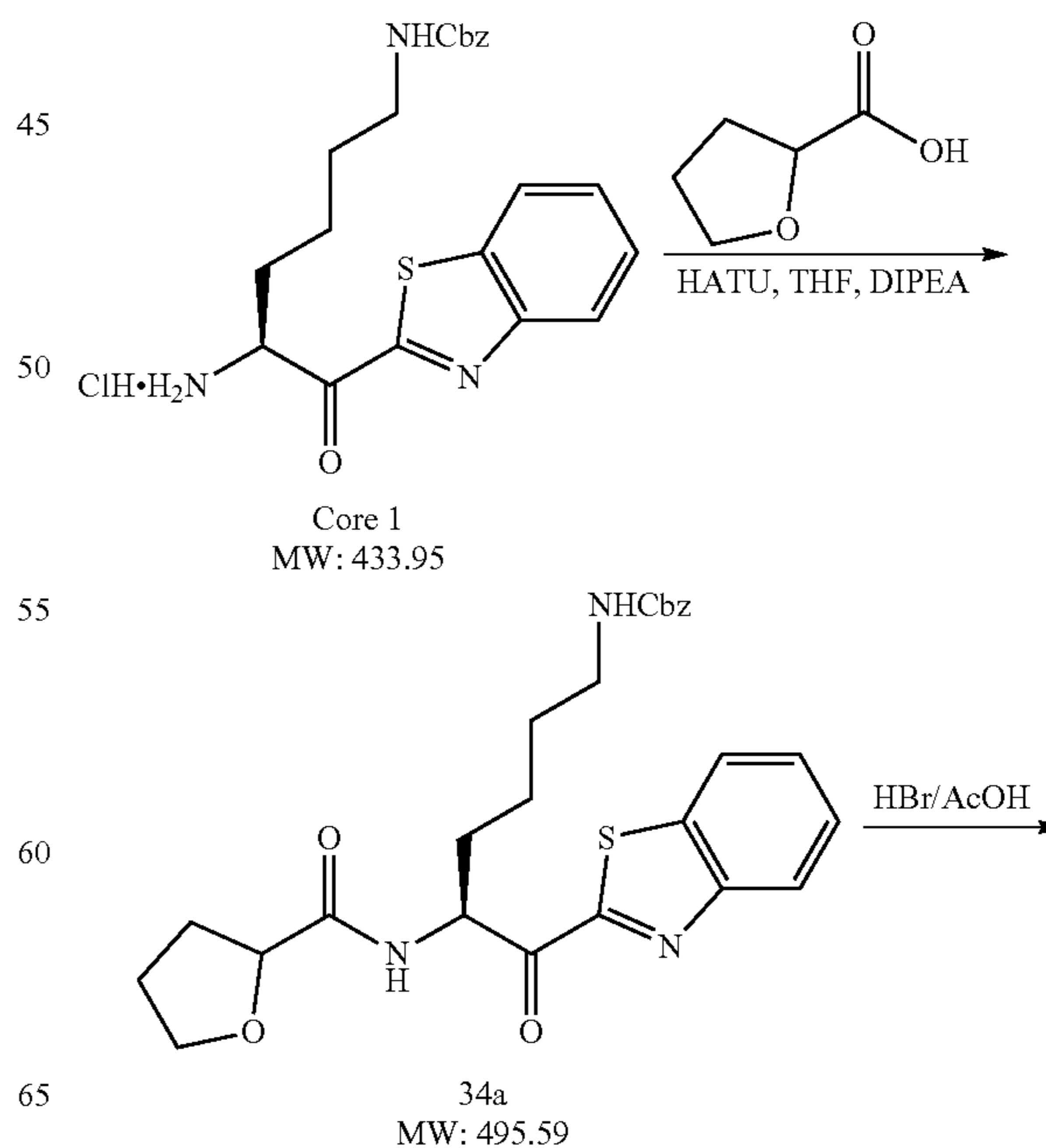
Scheme 28
