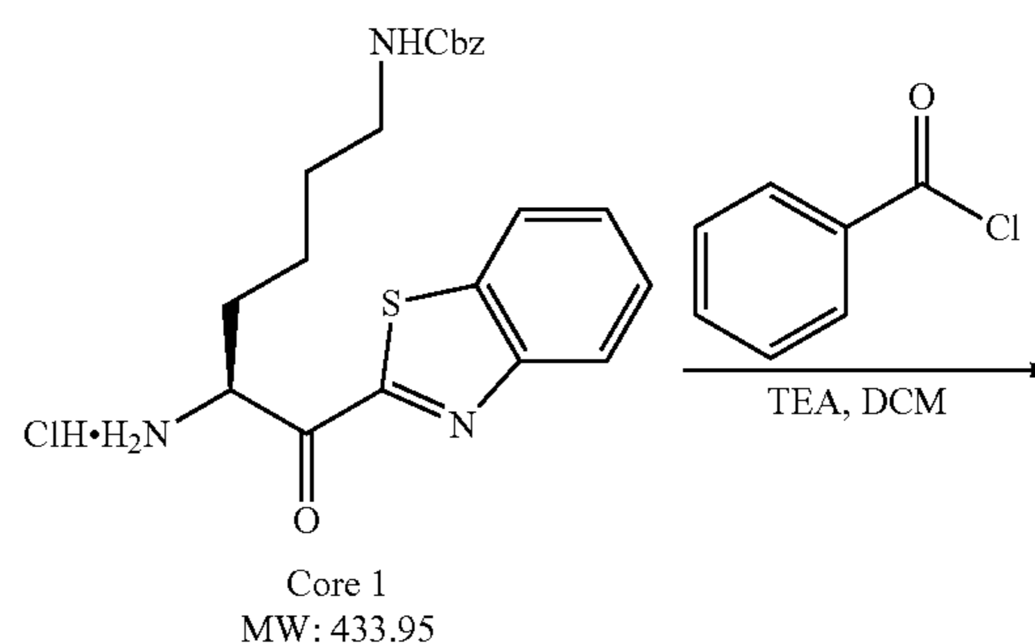
Scheme 8
