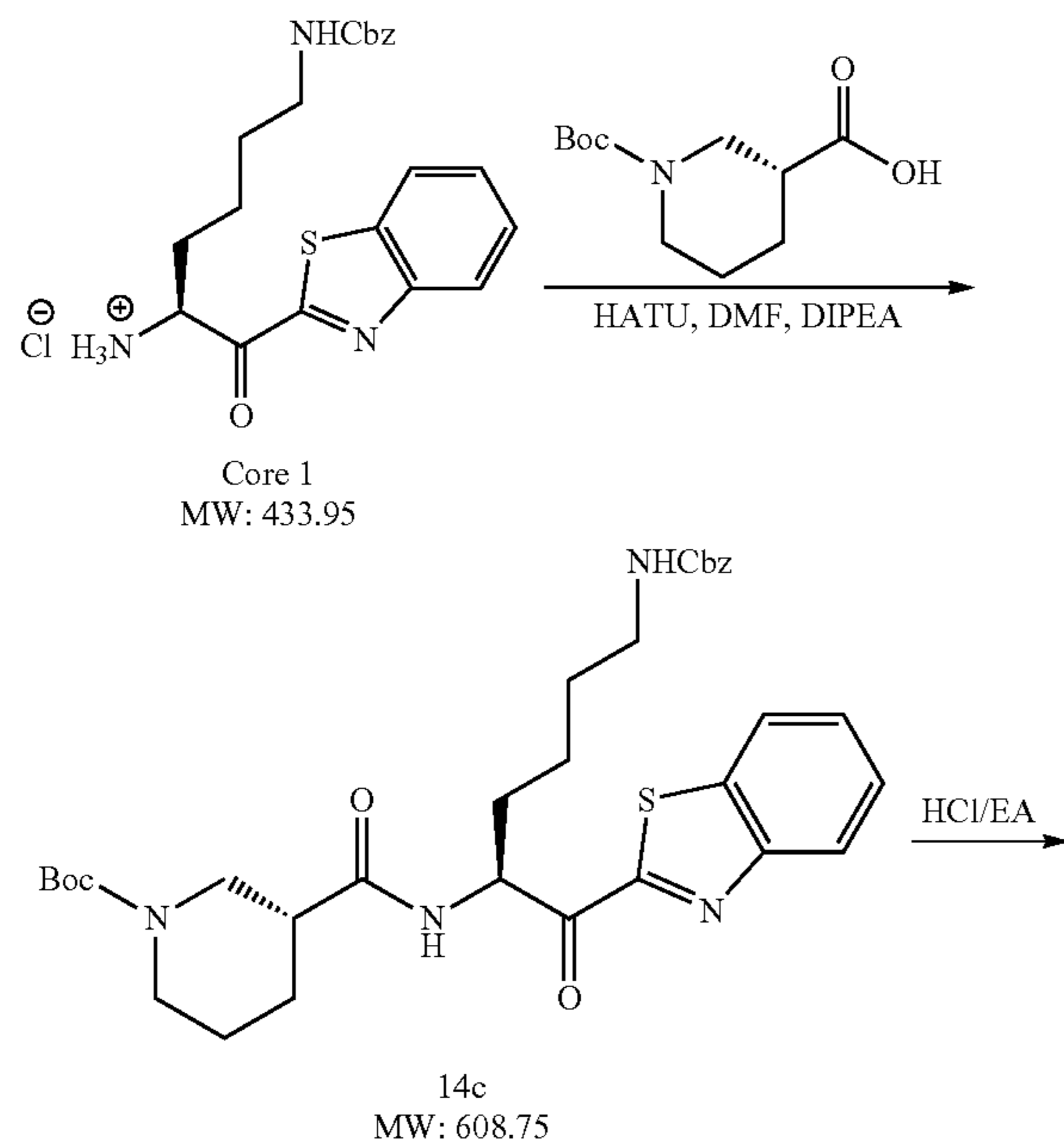
Scheme 17
