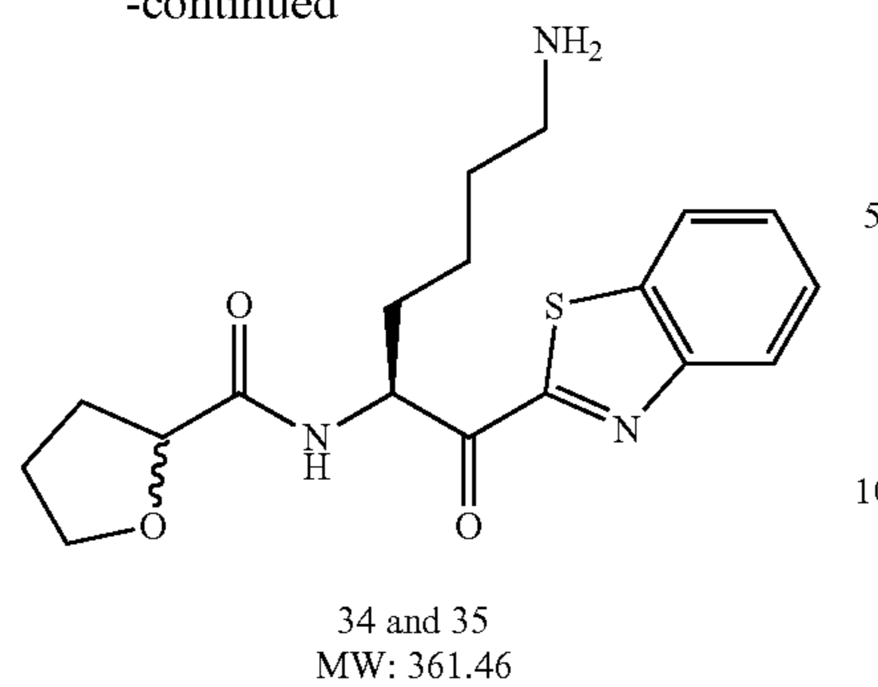
Benzyl-N-[(5S)-6-(1,3-benzothiazol-2-yl)-6-oxo-5-(tetrahydrofuran-2-carboxylamino)hexyl]carbamate (2)
