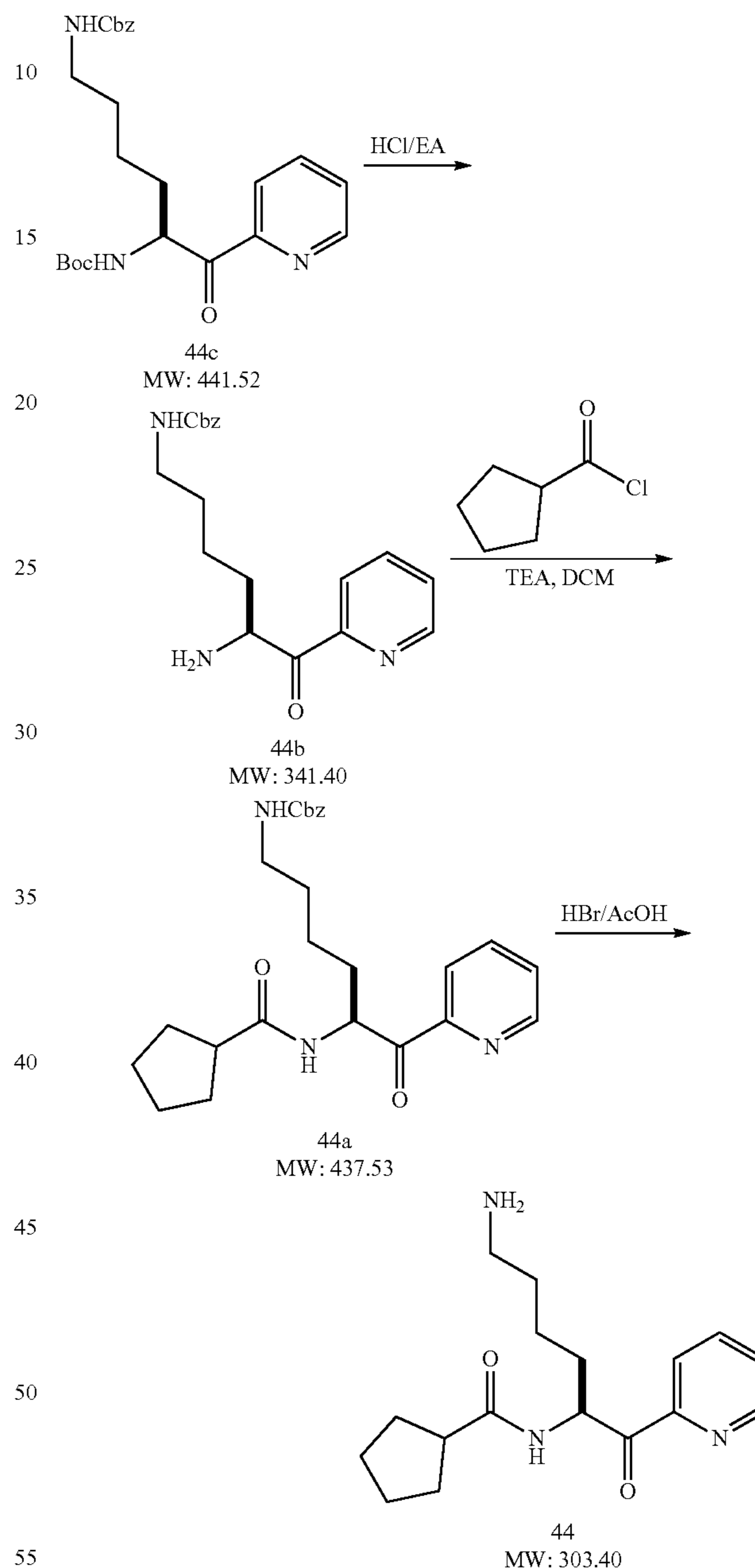
Scheme 35
