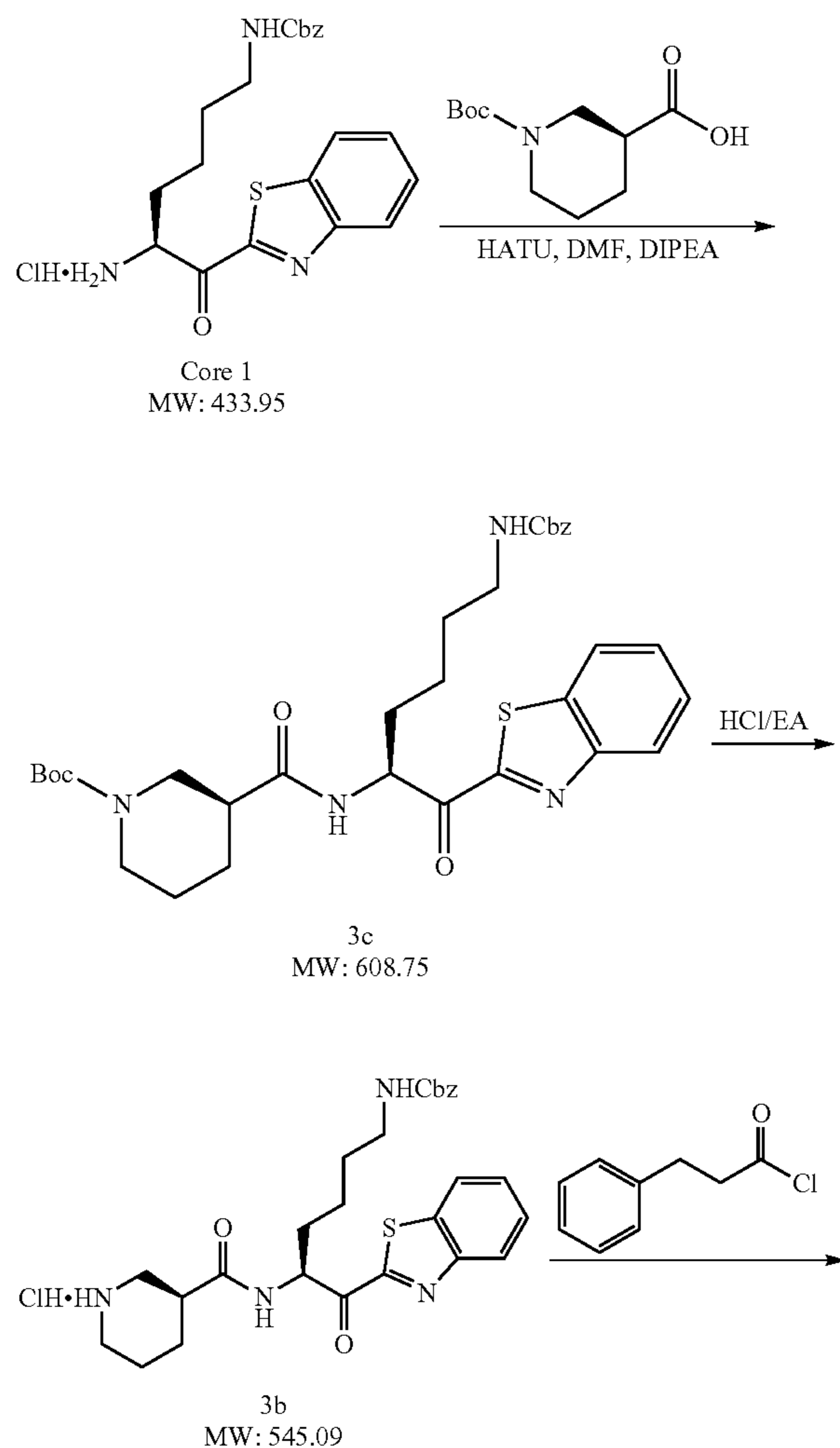
Scheme 10
