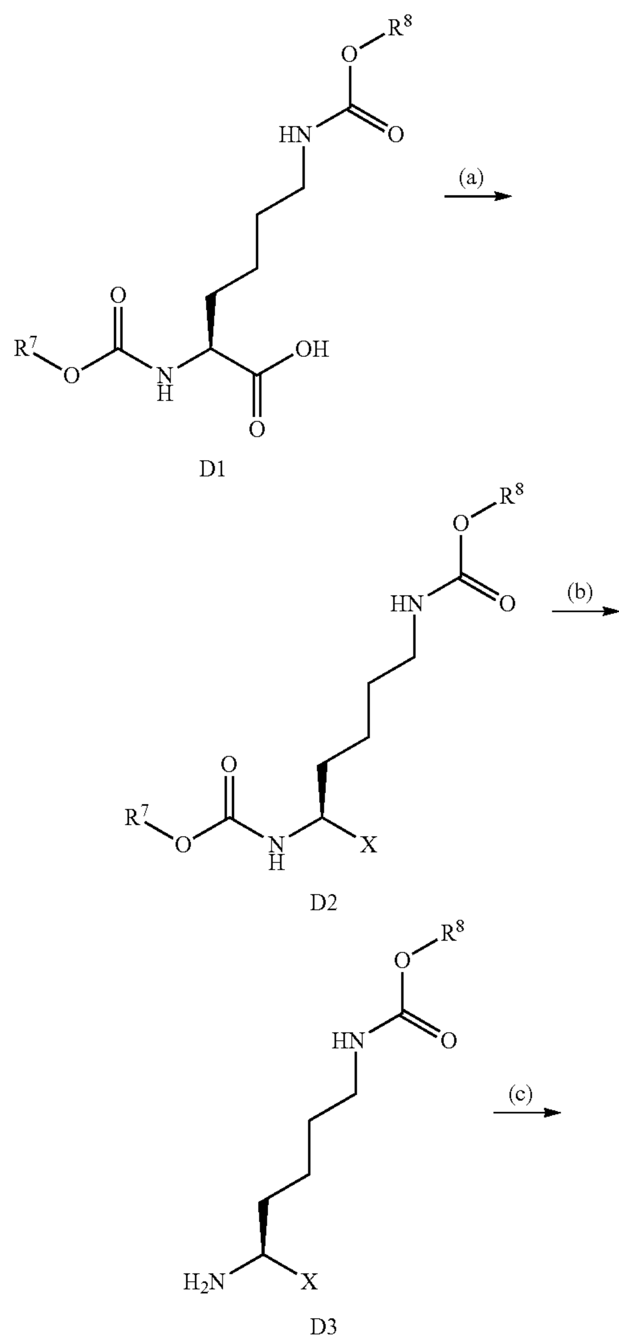
Scheme 1
