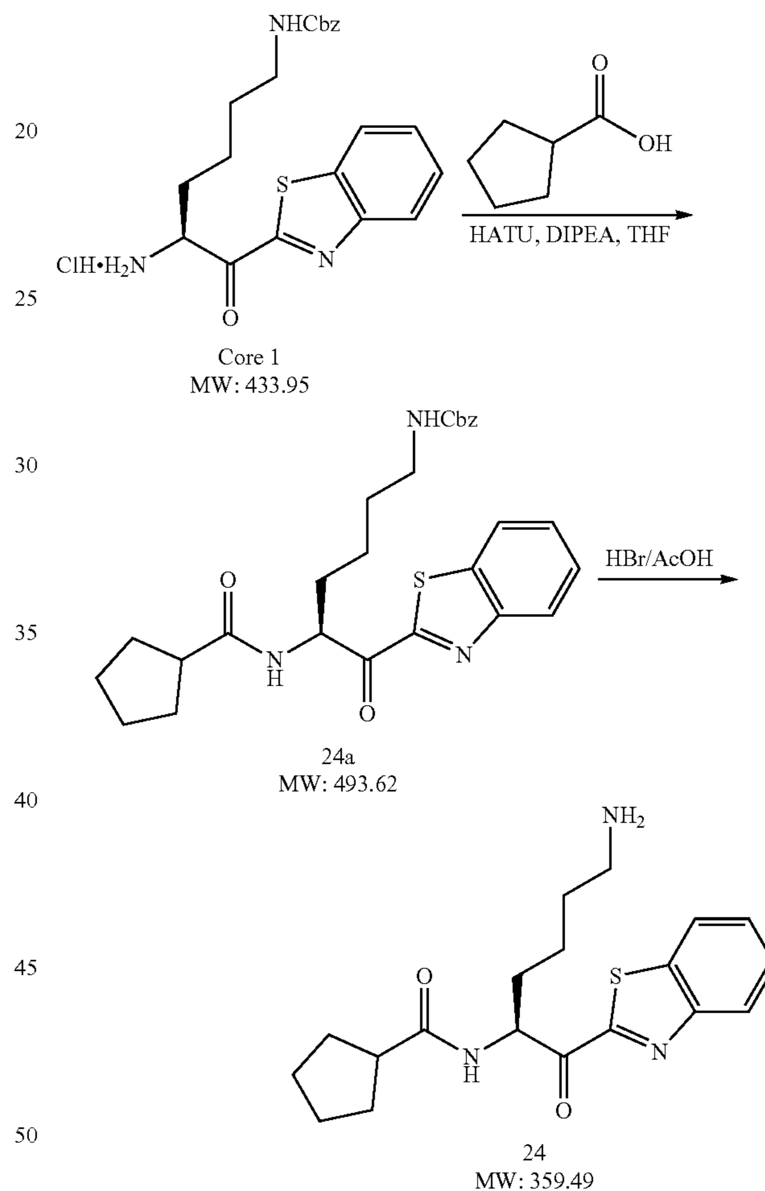
Scheme 21
