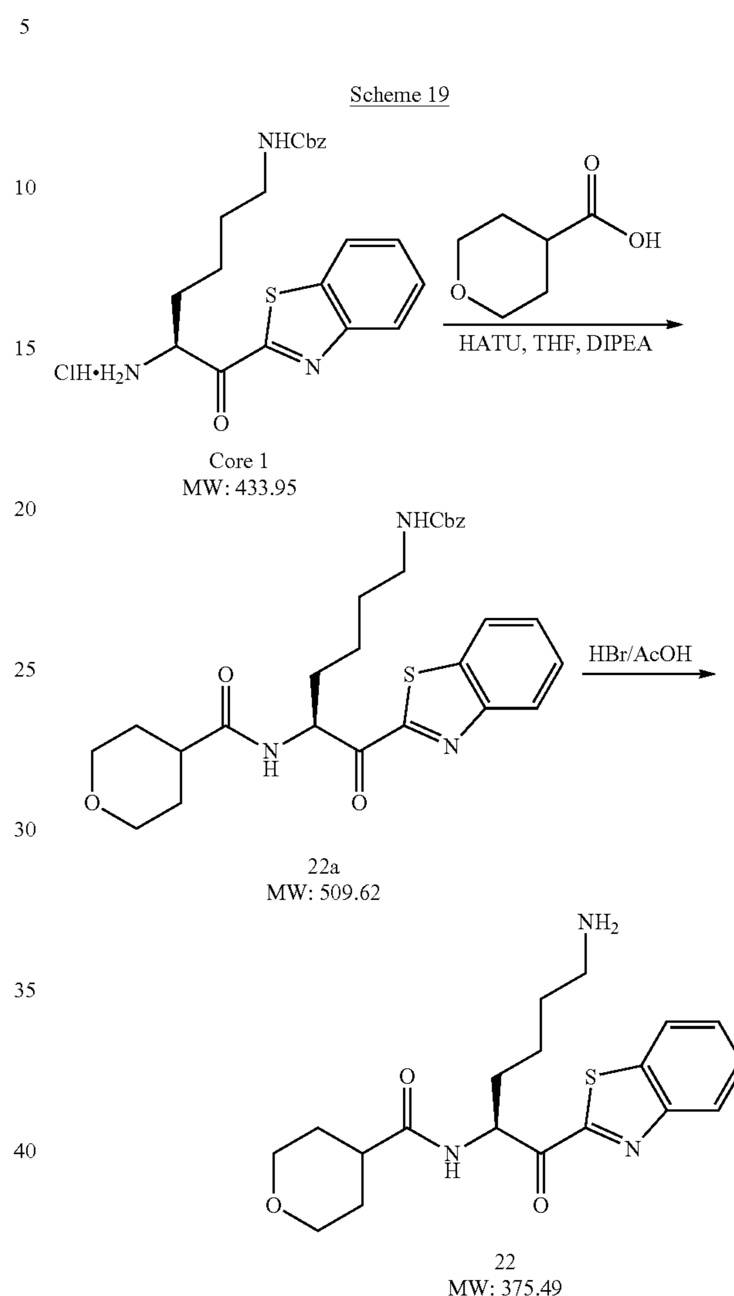
Benzyl-N-[(5S)-6-(1,3-benzothiazol-2-yl)-6-oxo-5-(tetrahydropyran-4-carboxylamino)hexyl]carbamate (22a)
