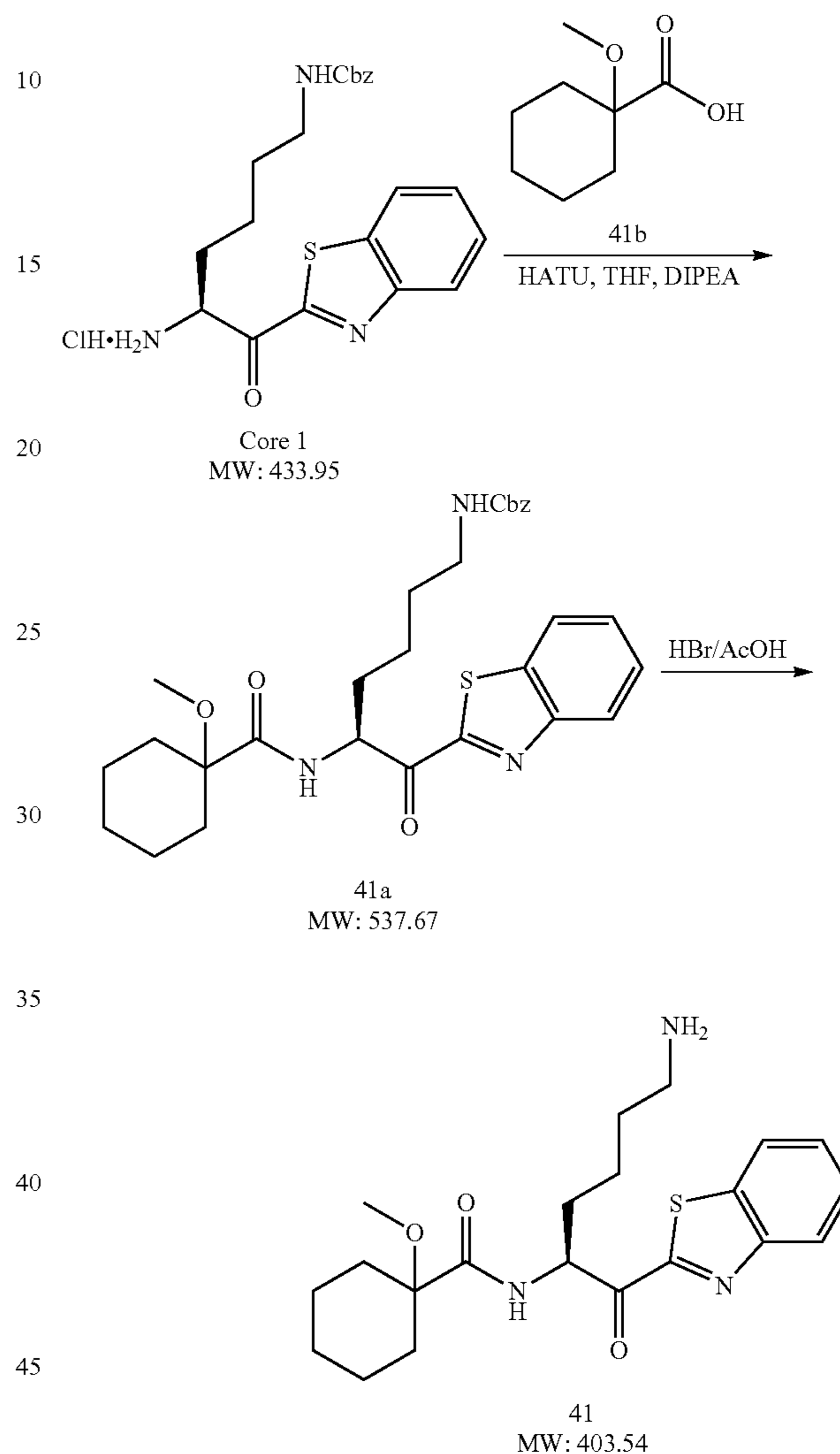
Scheme 32
