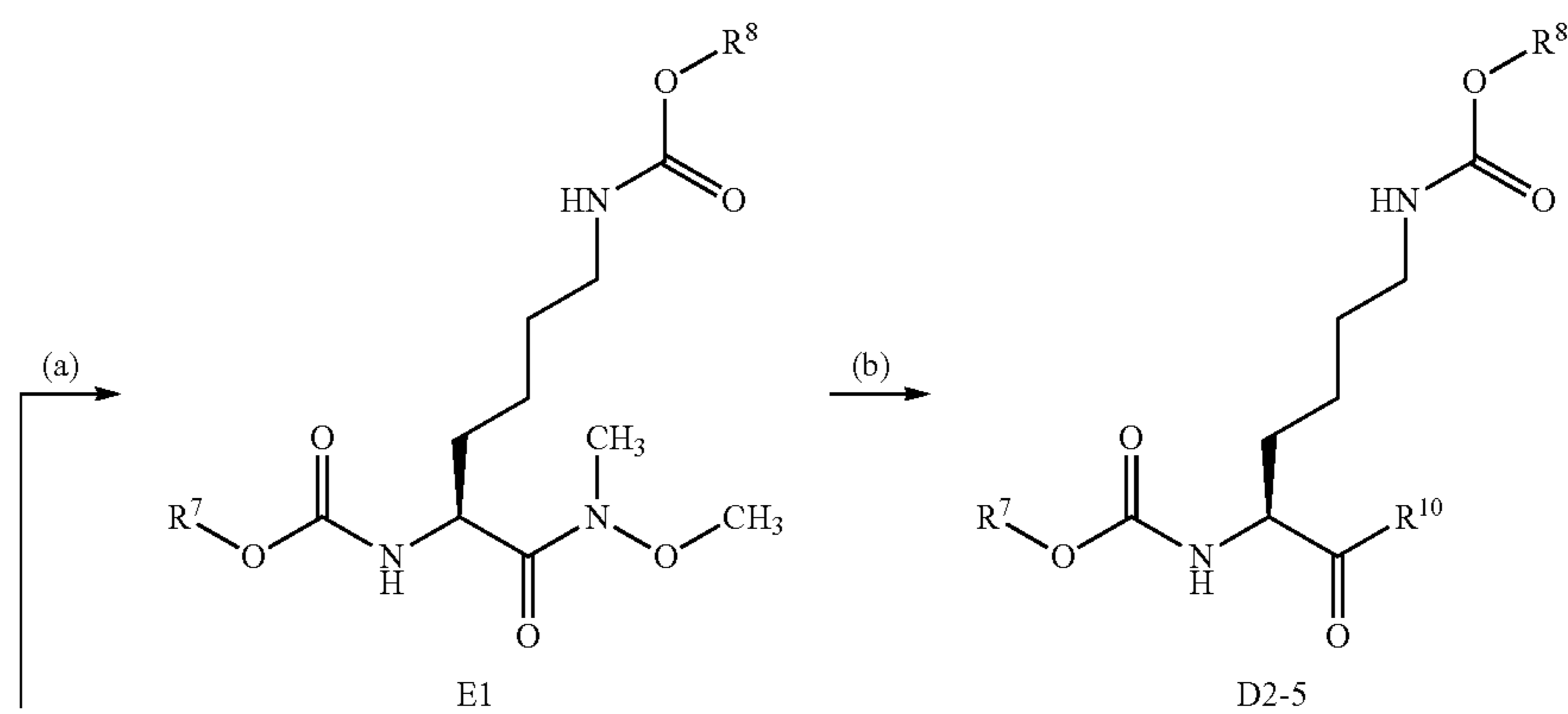
Scheme 2
