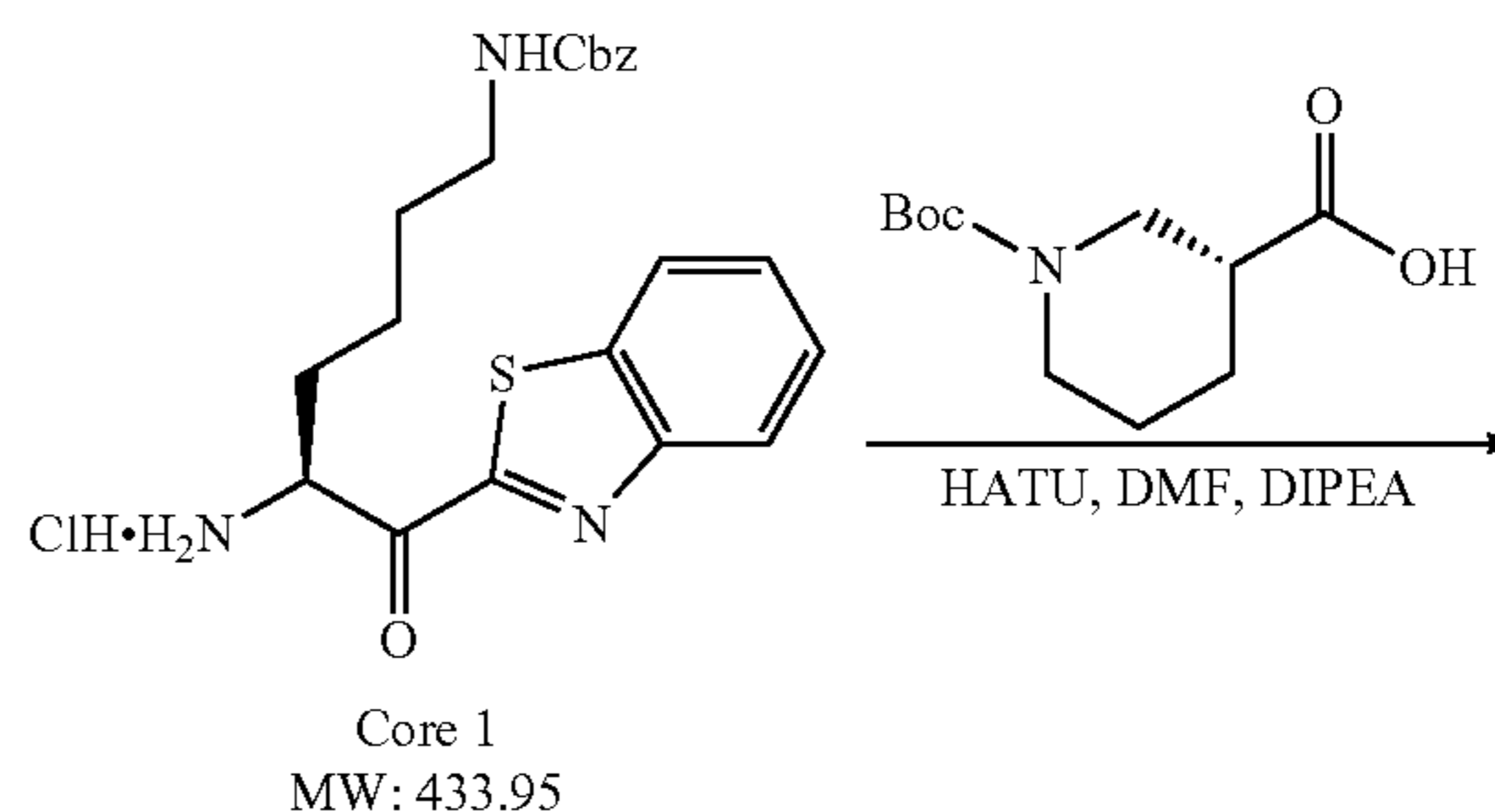
Scheme 14
