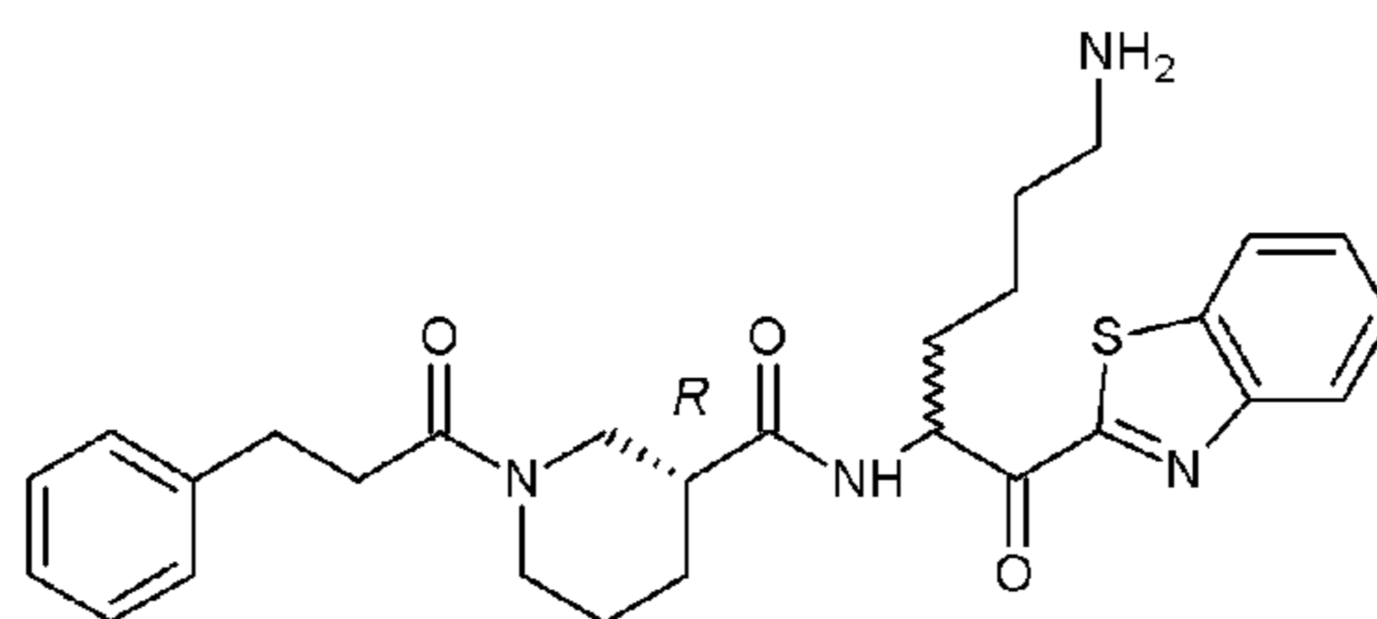
Compound 4
