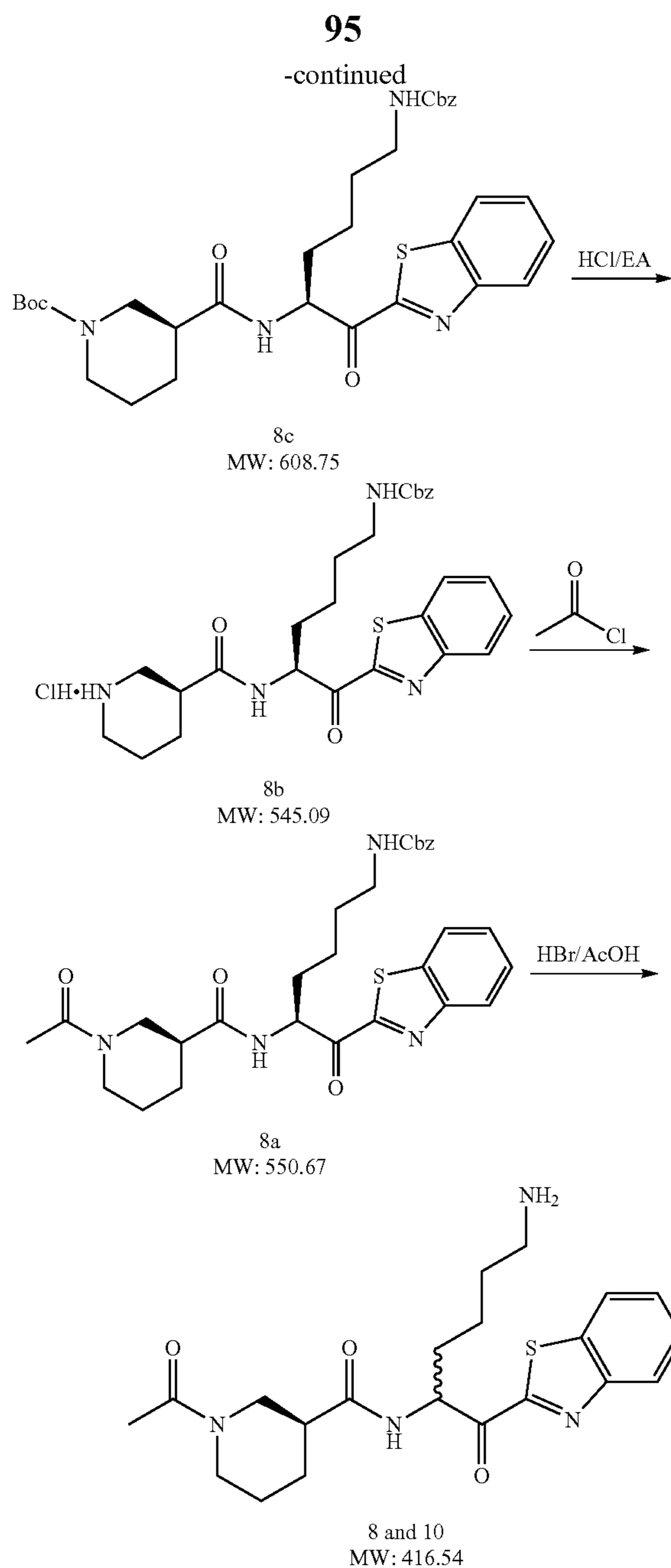
Tert-butyl-(3S)-3-[[[(1S)-1-(1,3-benzothiazole-2-carbonyl)-5-(benzyloxycarbonylamino)pentyl]carbamoyl]piperidine-1-carboxylate (8c)
