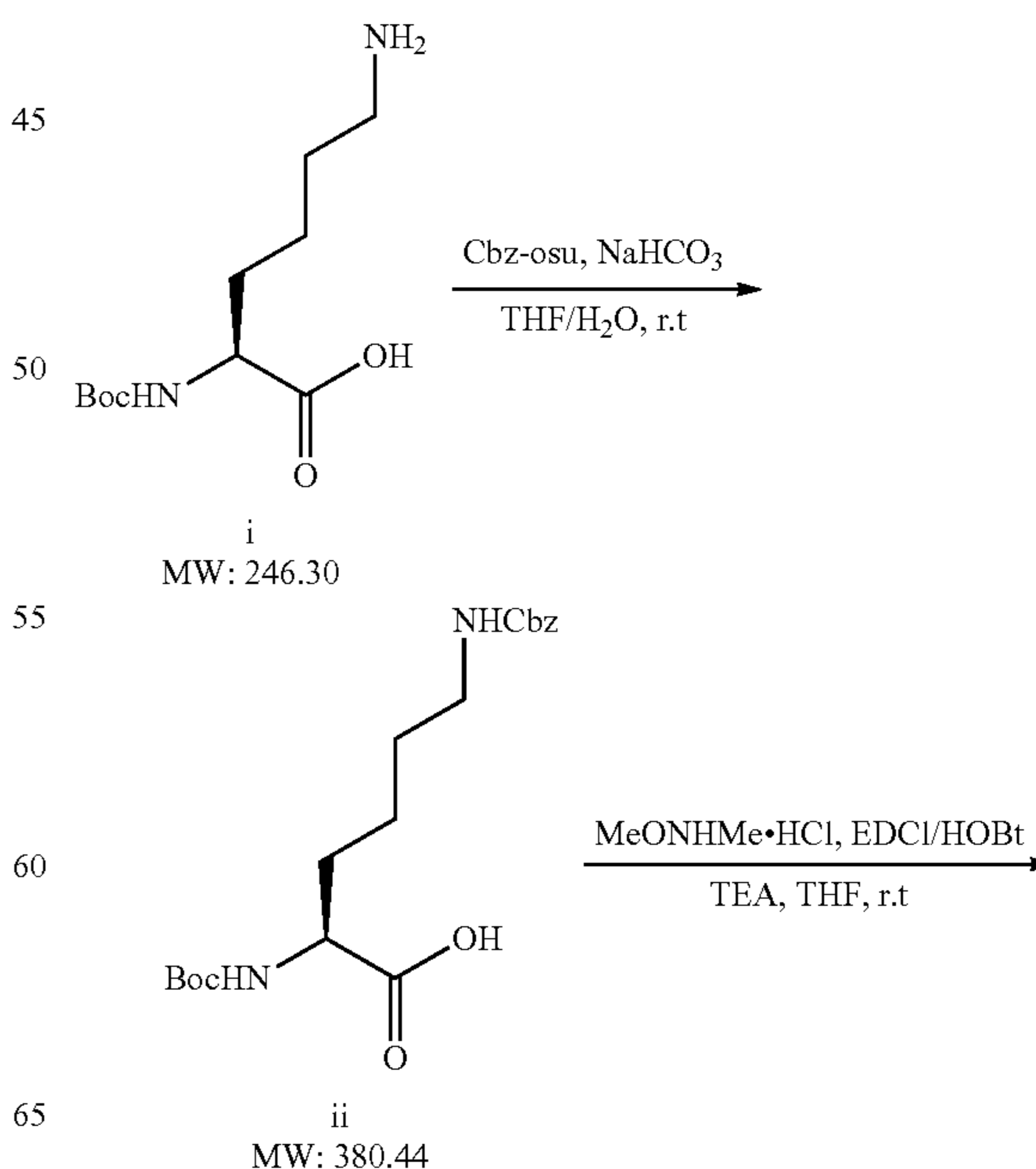
Scheme 7
