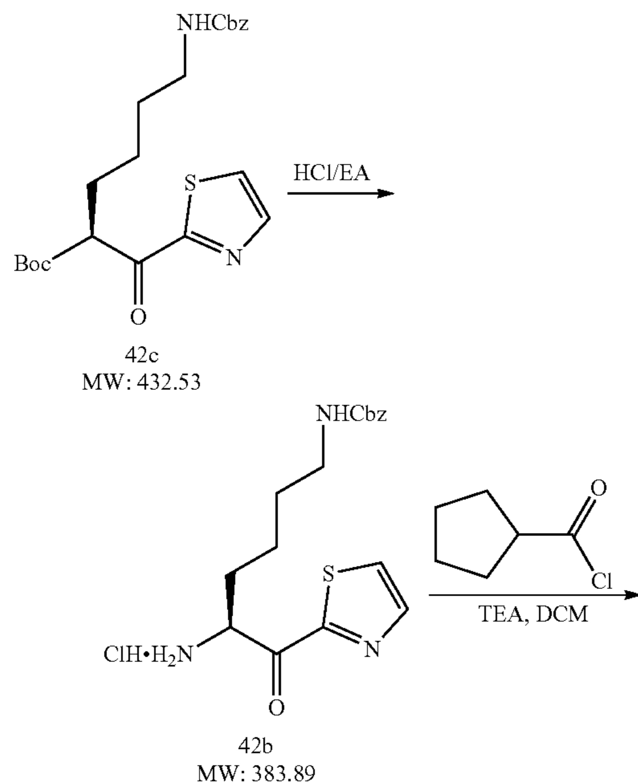
Scheme 33
