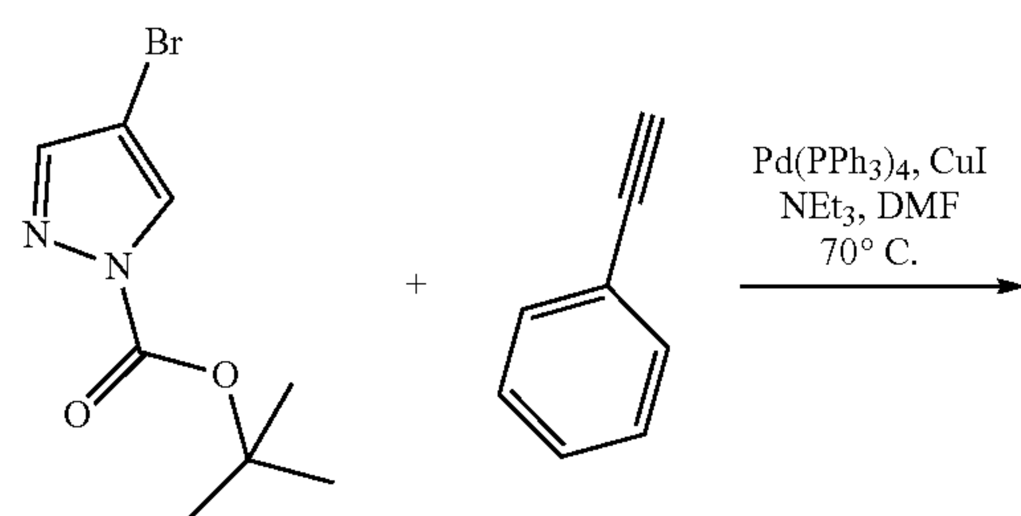
Scheme 1g Preparation of intermediate 4-(phenylethynyl)-1H-pyrazole for preparing e.g., Example 1b-102
