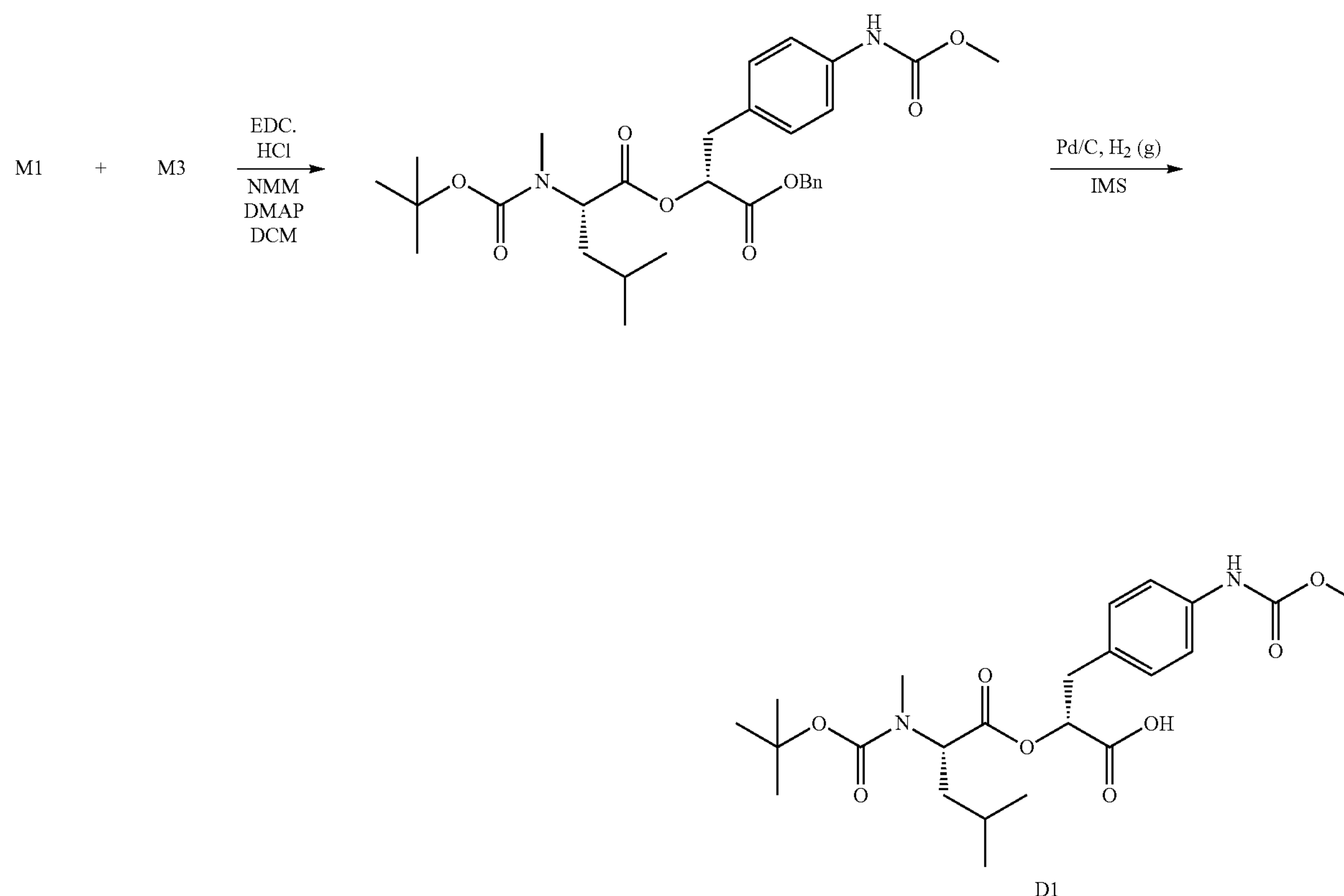
Scheme 1b. Route for Stepwise Synthesis of Bis-Iodo PF1022a
