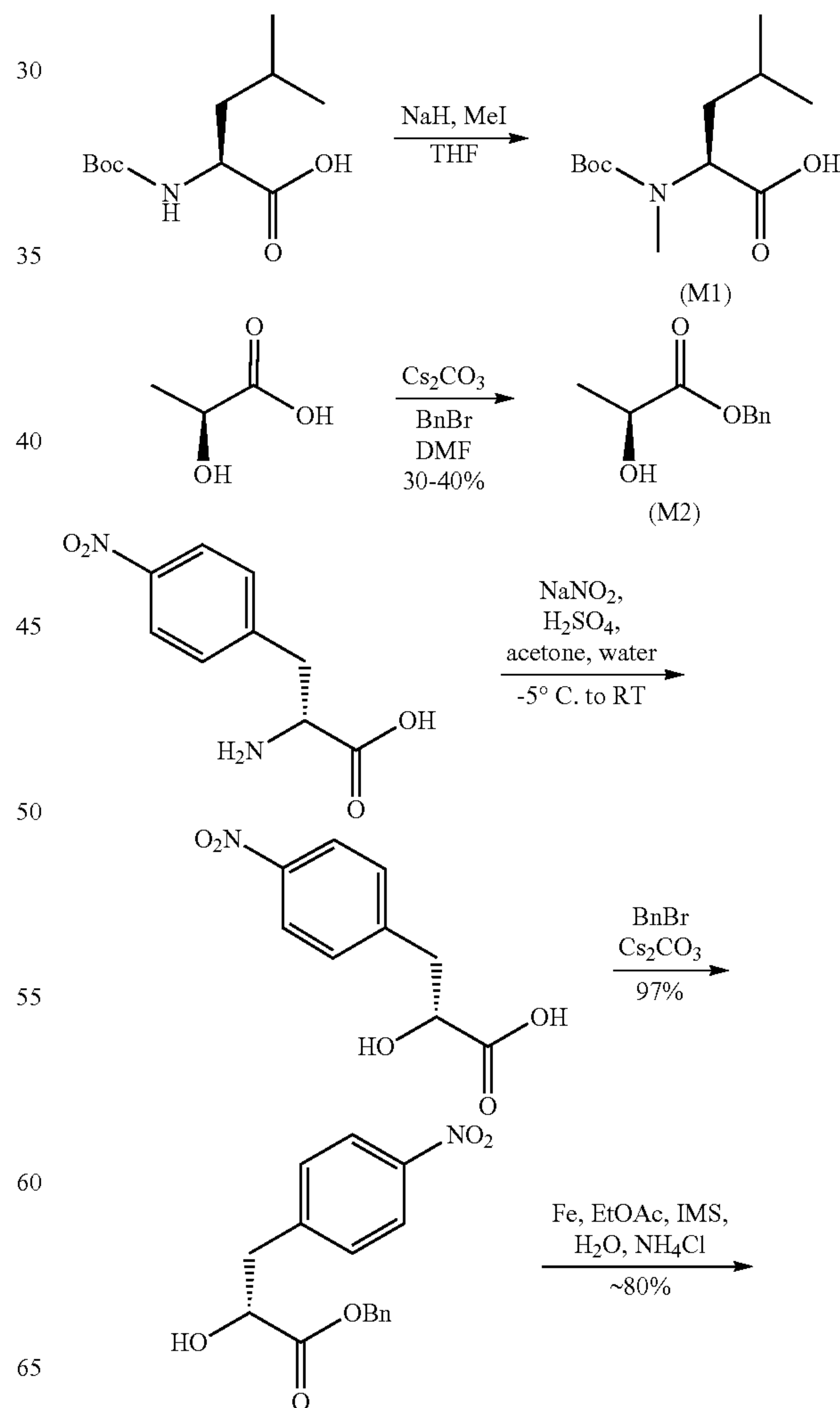
Scheme 1a Synthetic Scheme for Preparation of Monomers M1, M2, M3 and M4.
