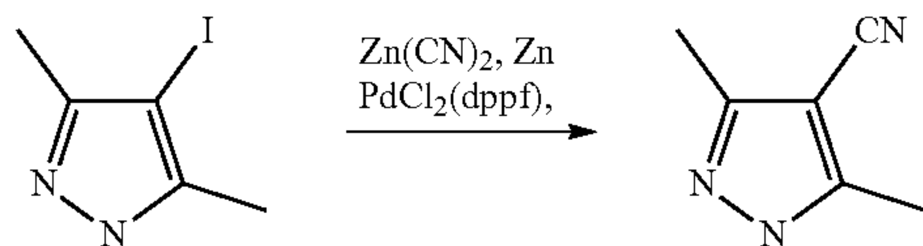
Scheme 1f Preparation of intermediate 3,5-dimethyl-1H-pyrazole-4-carbonitrile for preparing e.g., Example 1b-117
