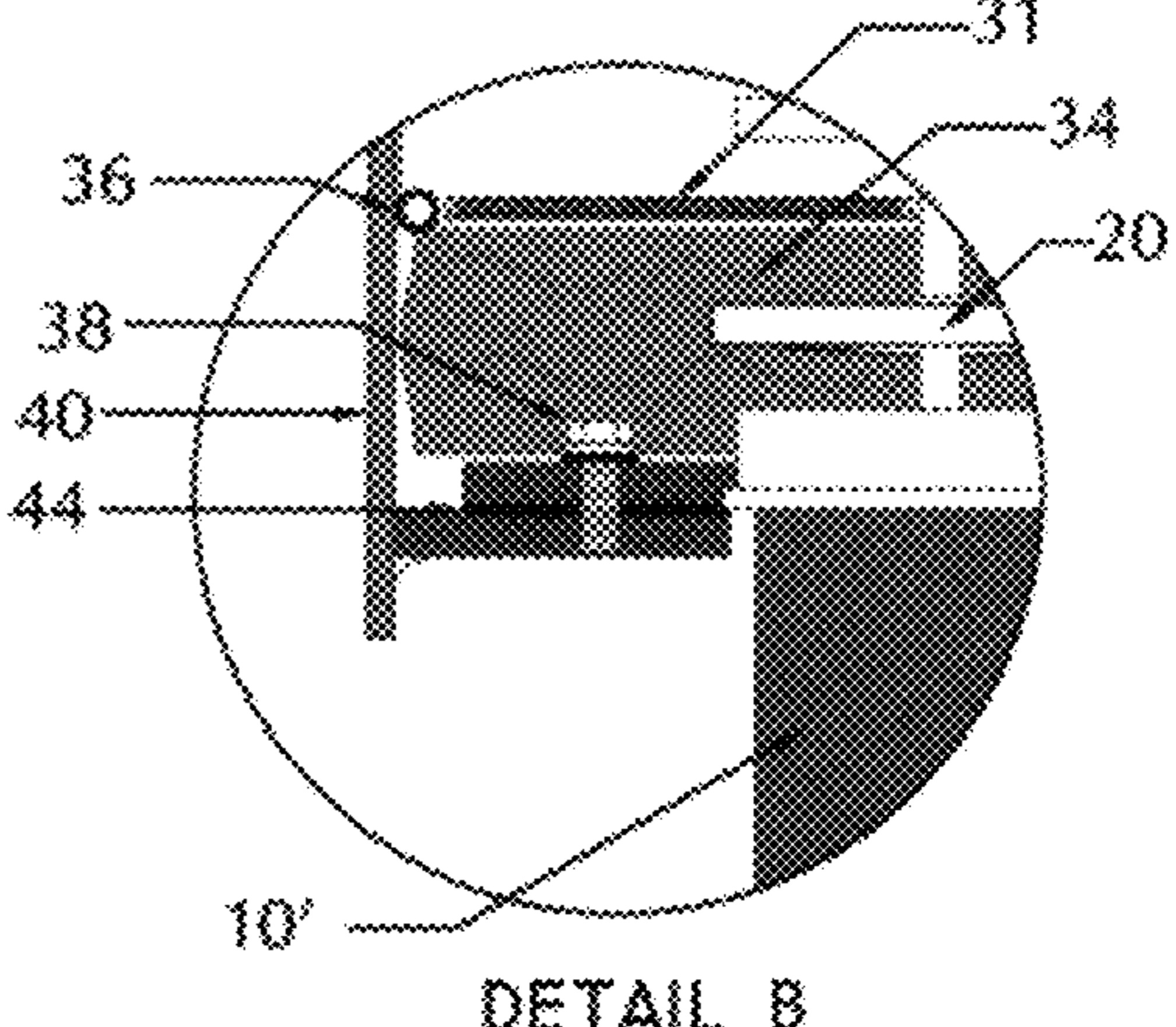
DETAIL B
