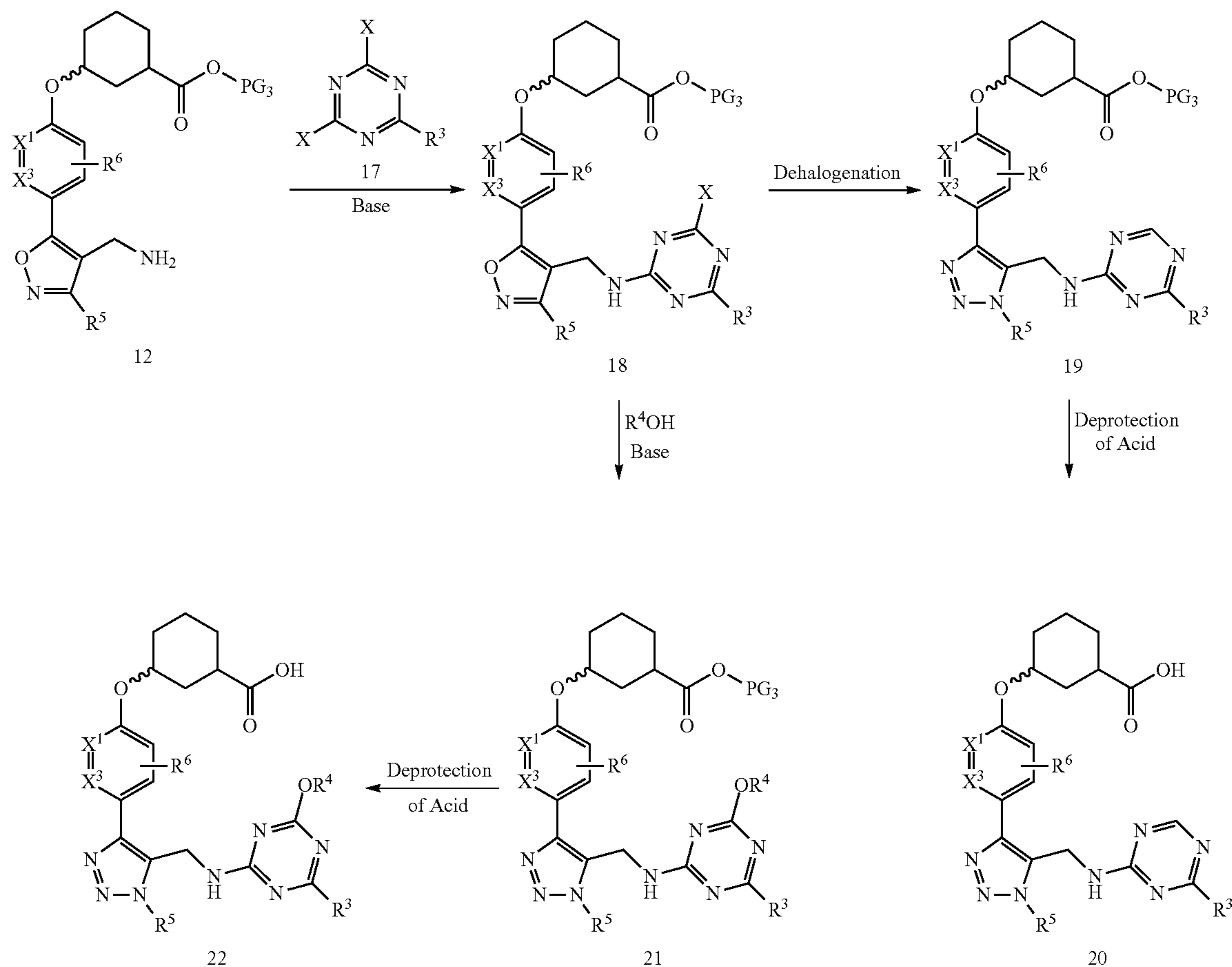
Scheme 3
