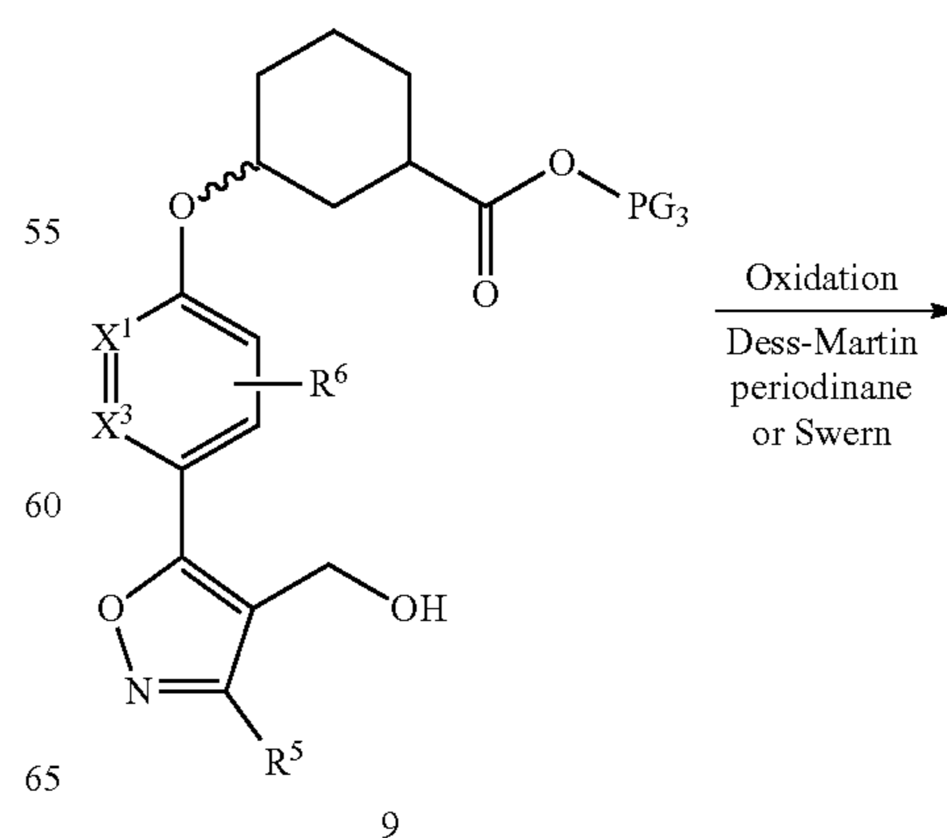
Scheme 7
