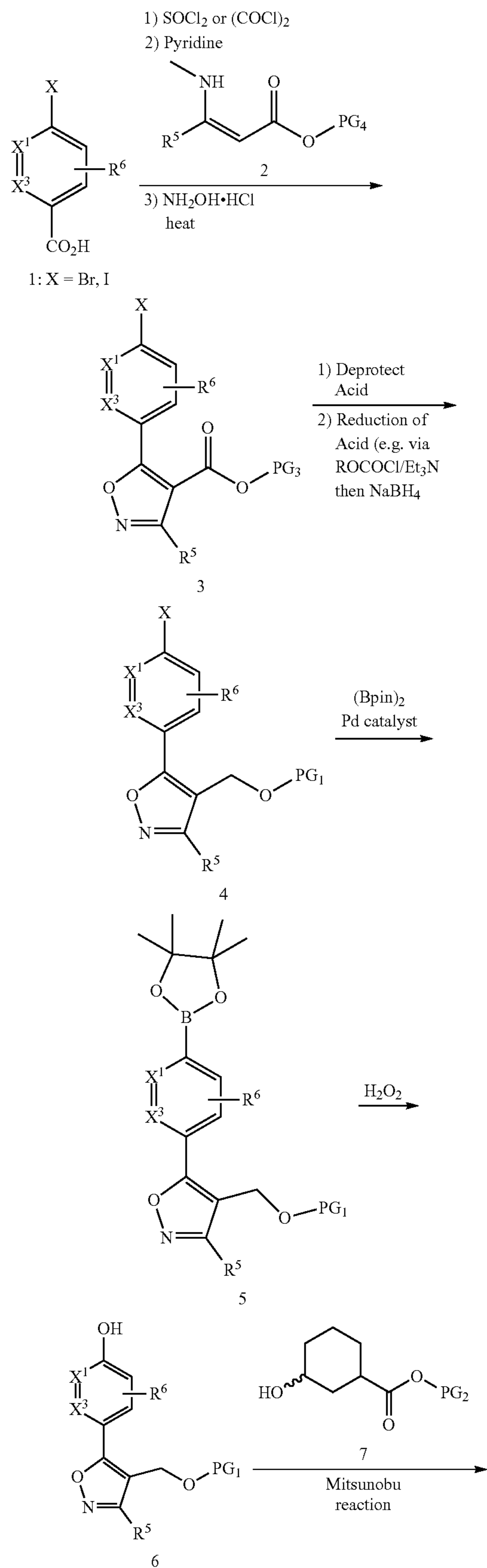
Scheme 1
