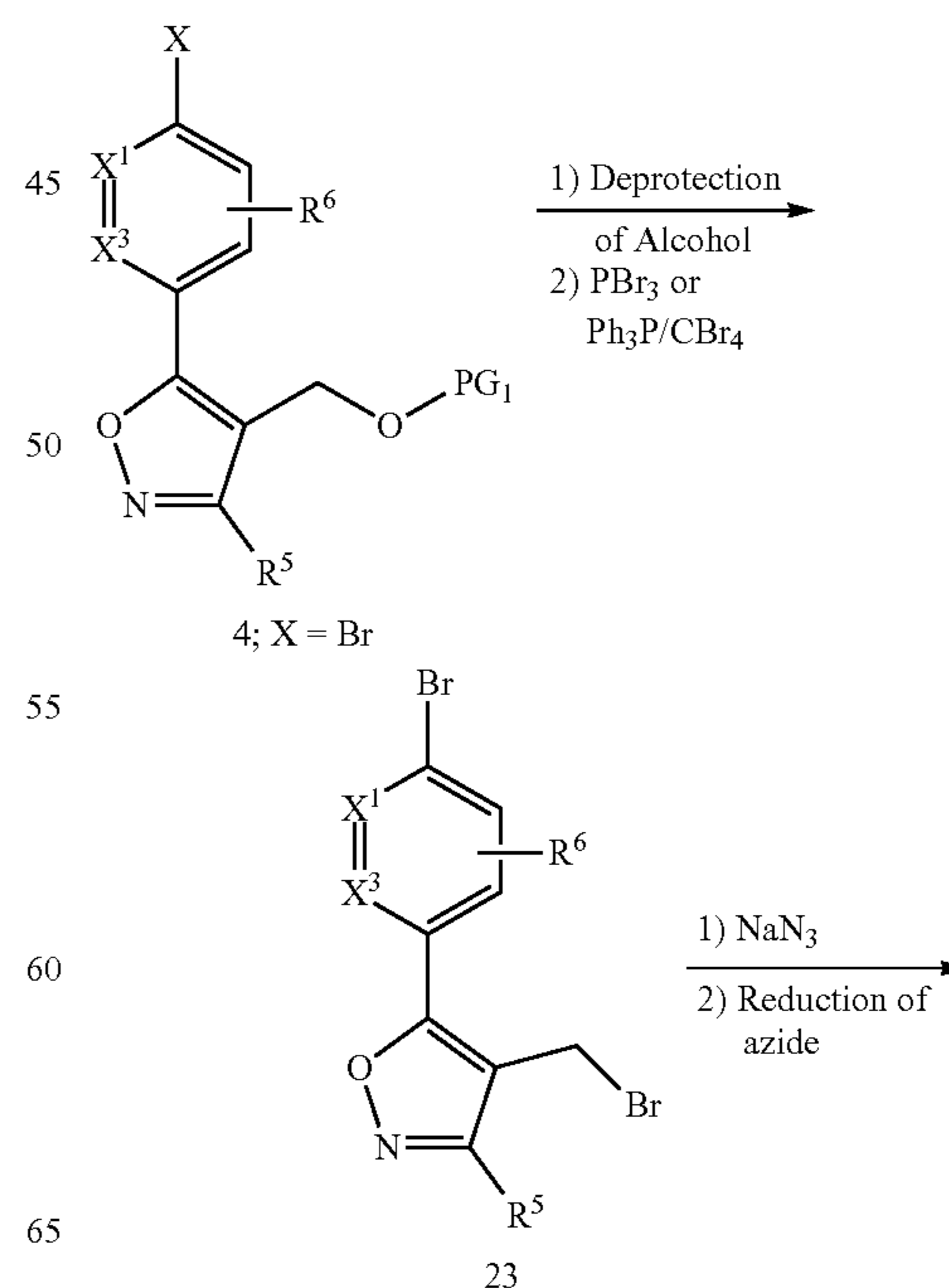
Scheme 4
