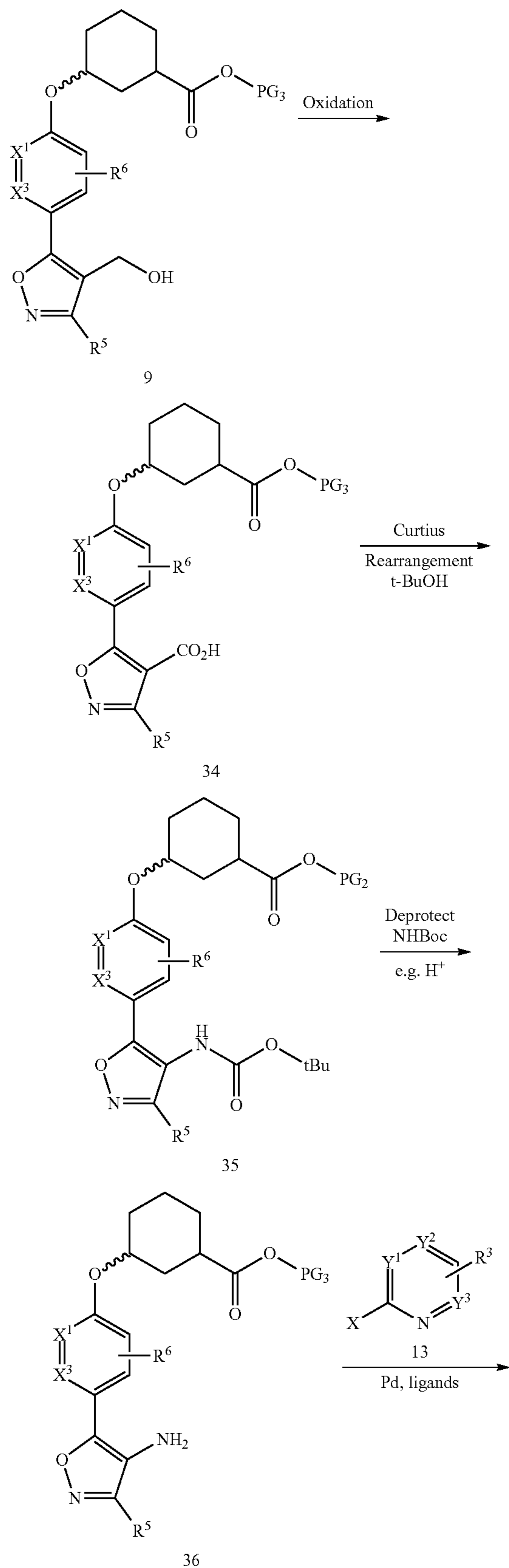
Scheme 6
