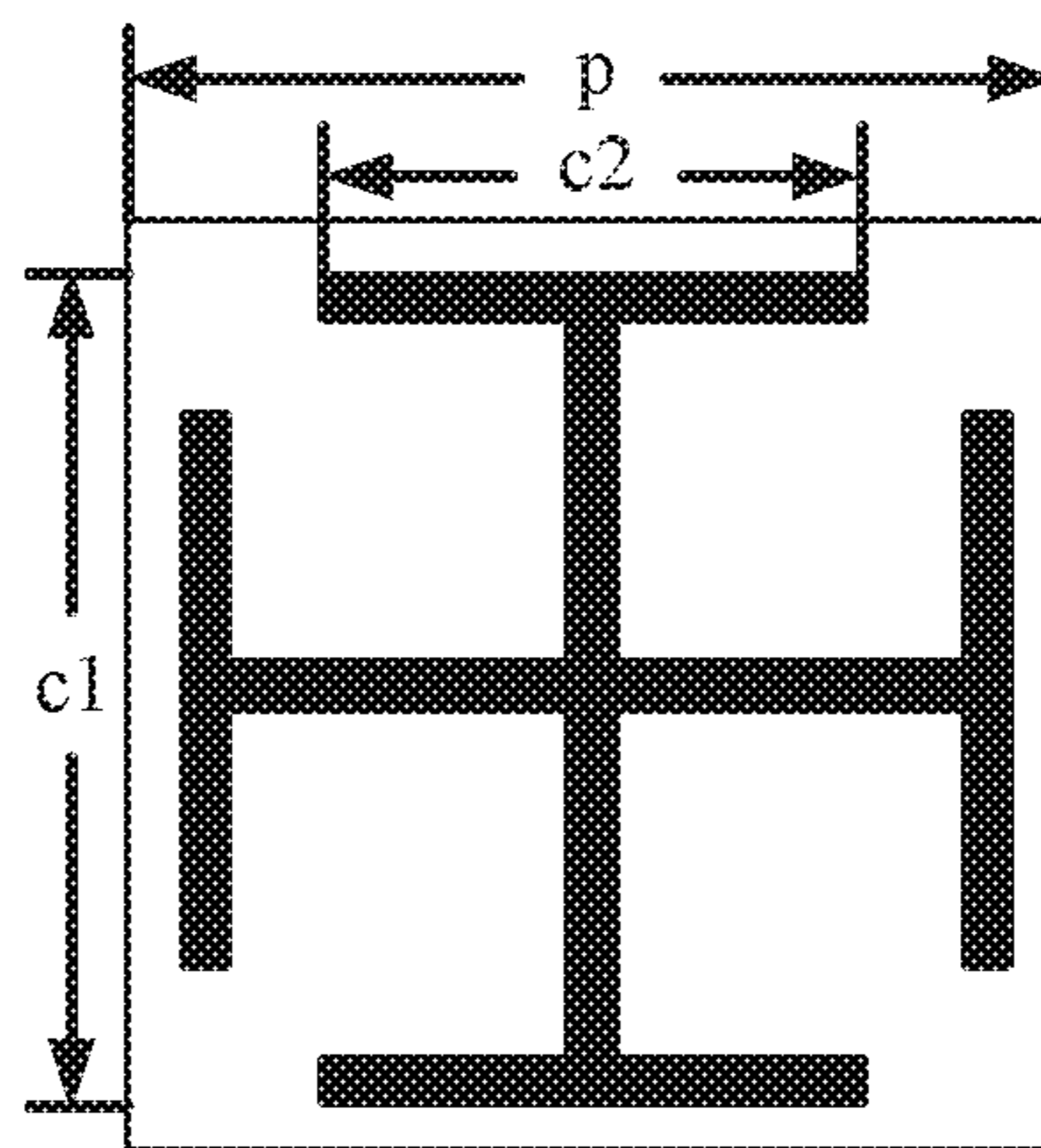
Top view
