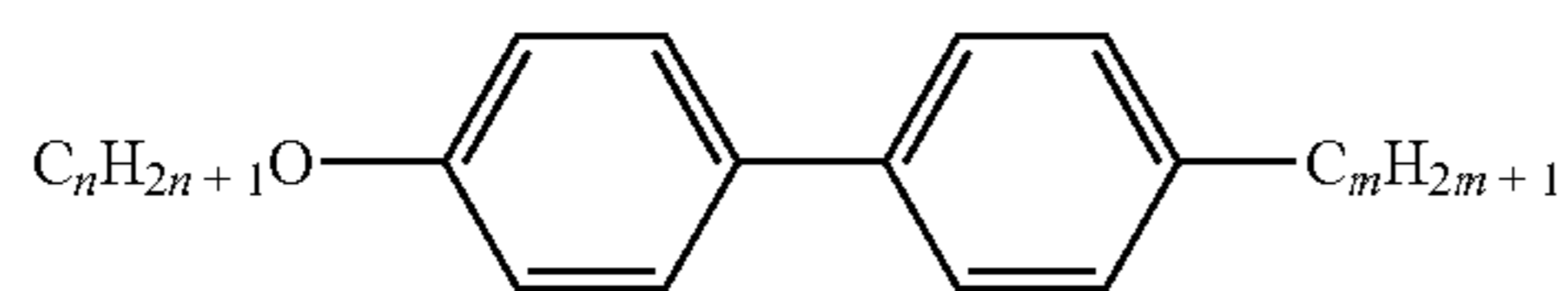
PP-nO-m
