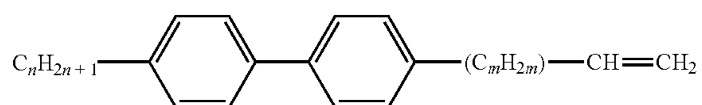
PP-n-mV
