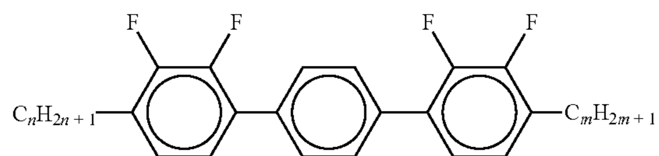
YPY-n-m
