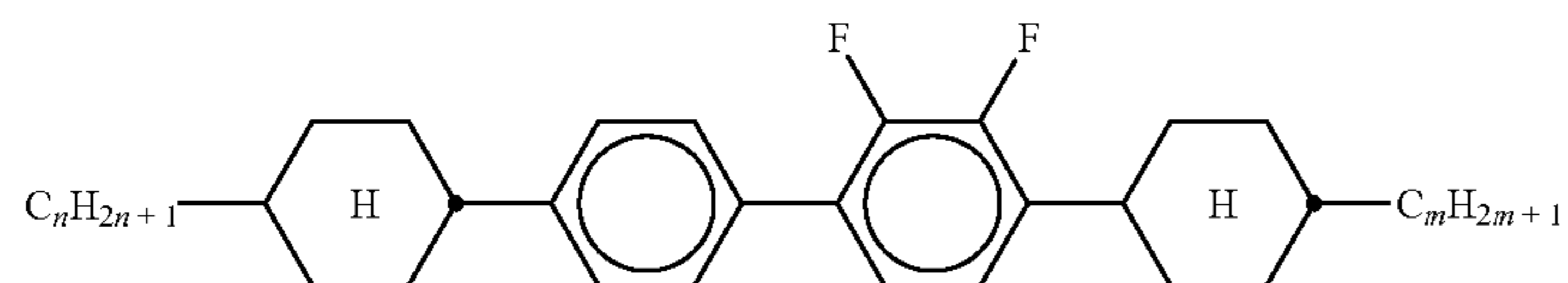
CPYC-n-m
