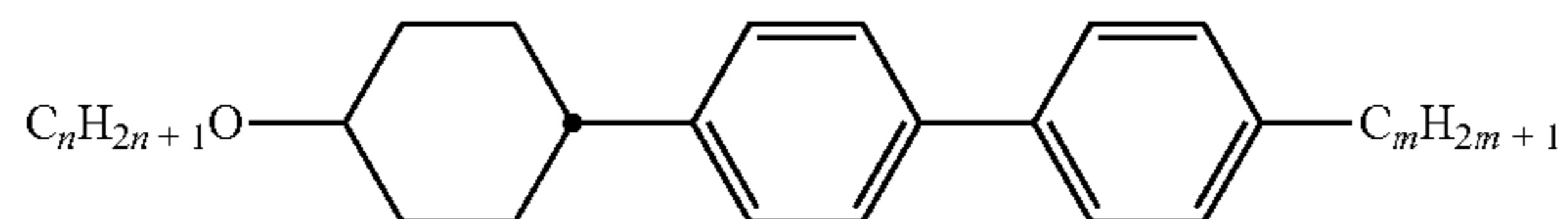
CPP-nO-m
