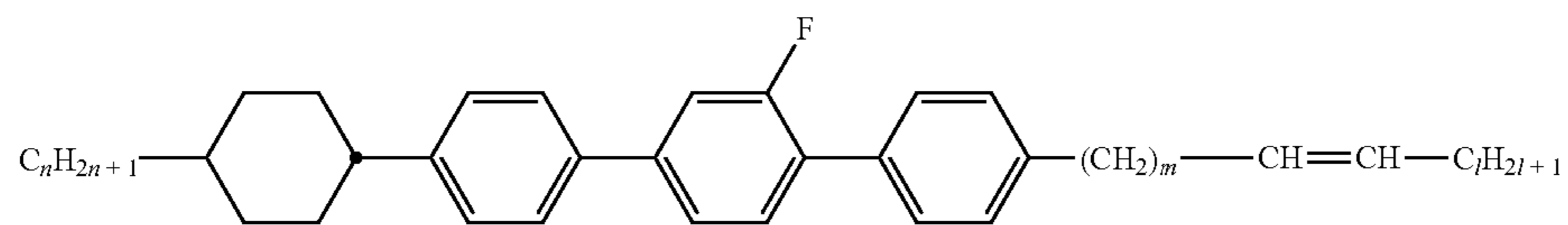
CPGP-n-mVI
