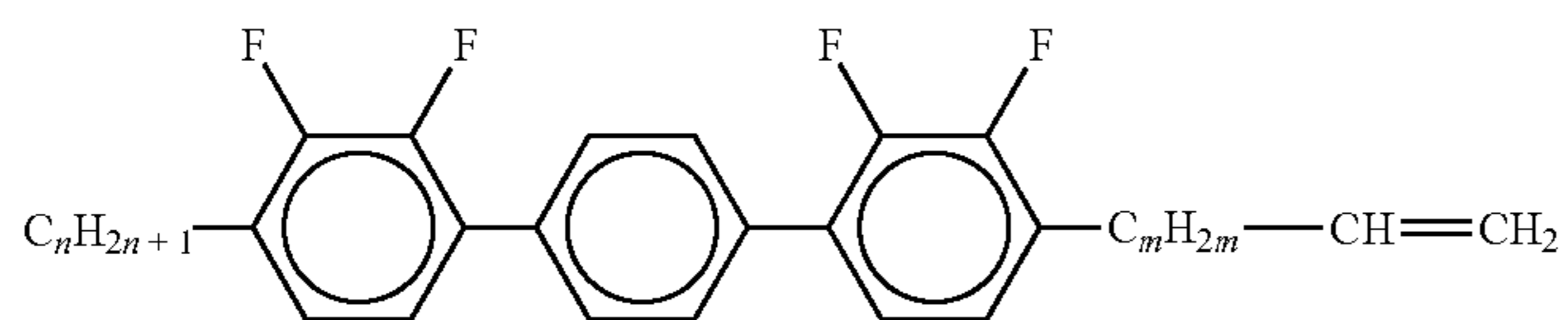
YPY-n-mV
