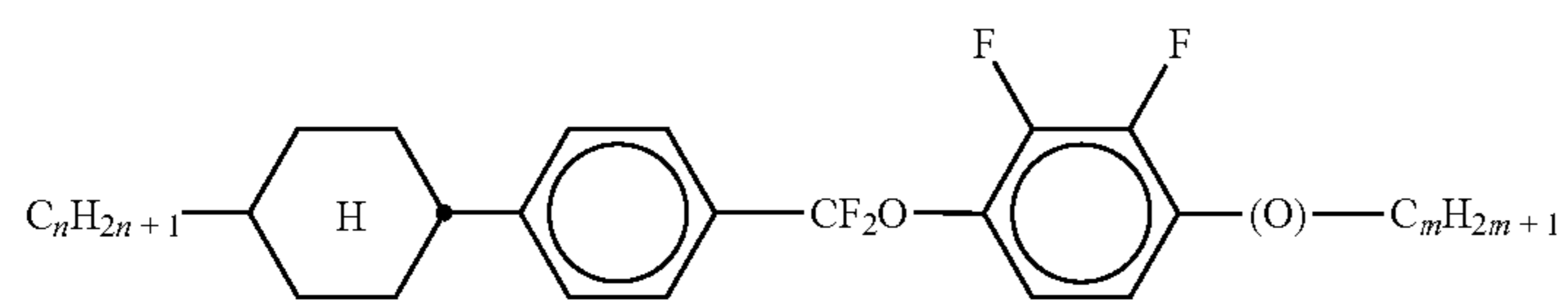
CPQY-n-(O)m
