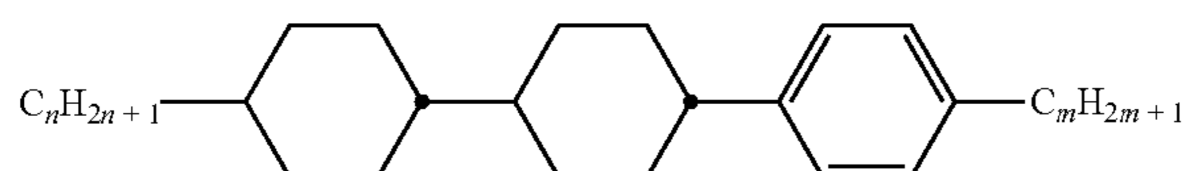
CCP-n-m
