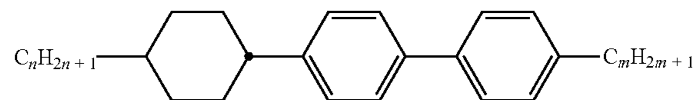
CPP-n-m
