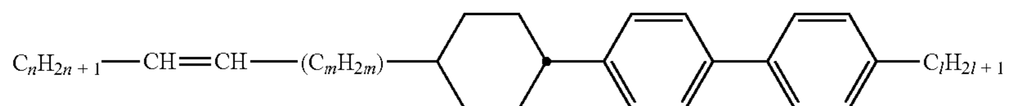
CPP-nVm-I
