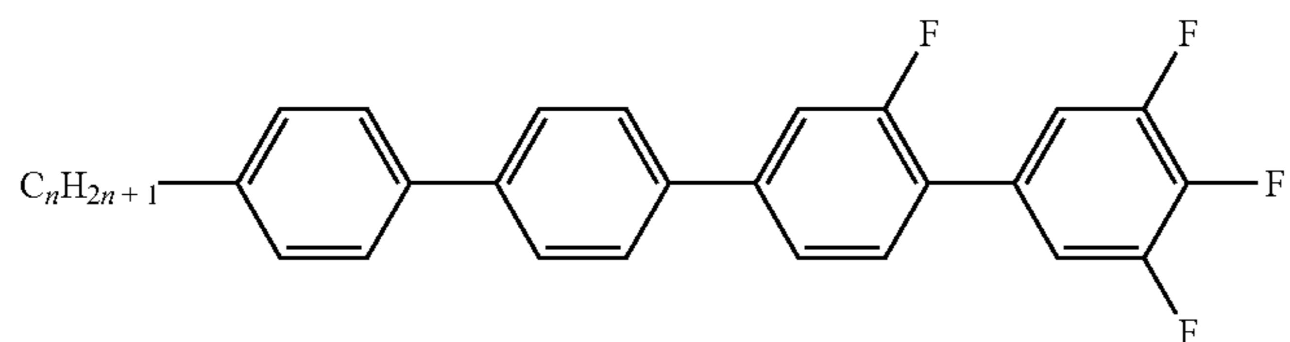
PPGU-n-F
