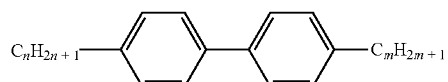
PP-n-m
