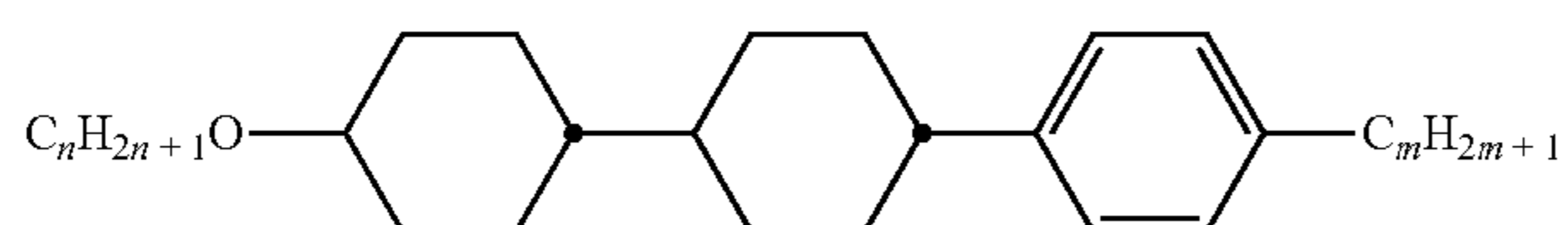
CCP-nO-m
