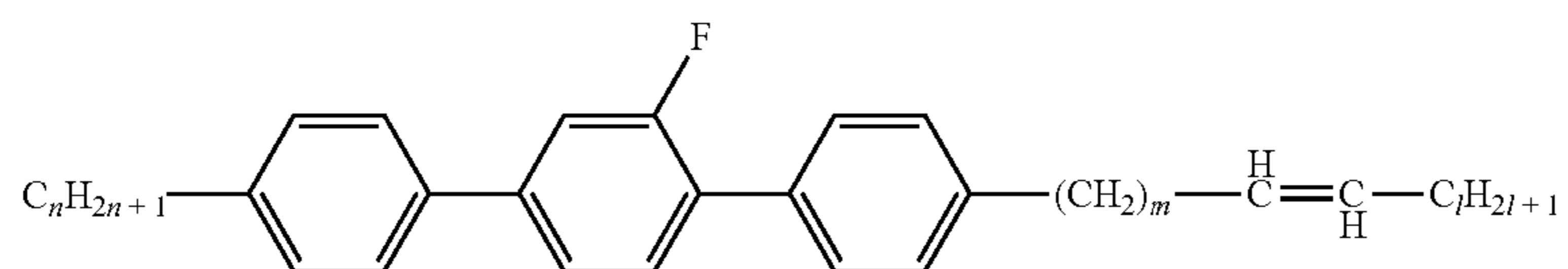
PGP-n-mVI
