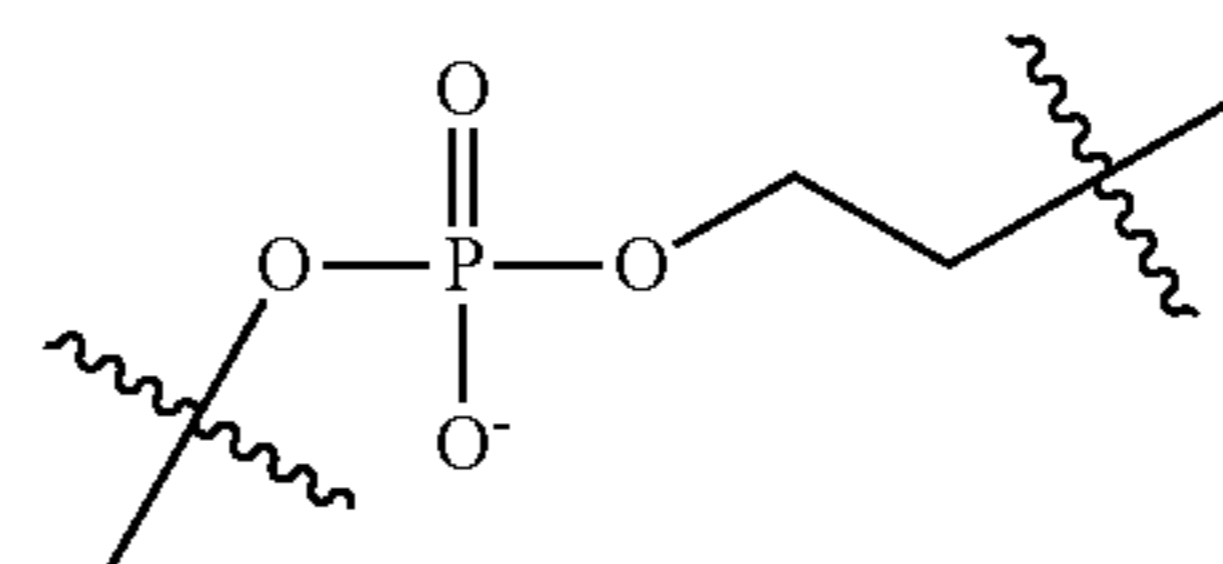
“C linker”
