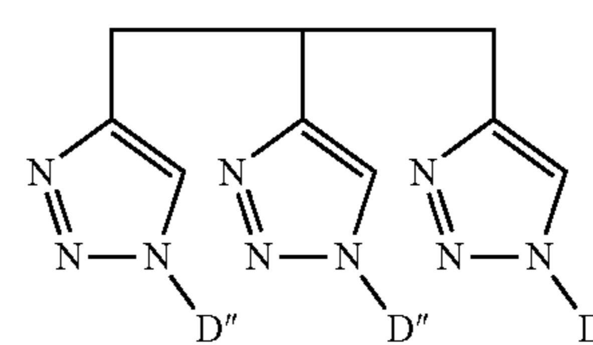
Compound 18
