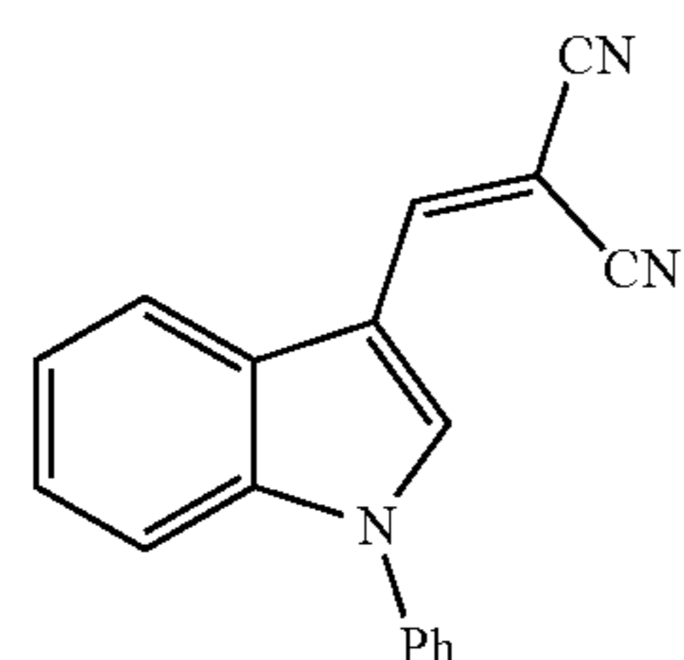
2-((1-Phenyl-1H-indol-3-yl)methylene)malononitrile (JXL021)
