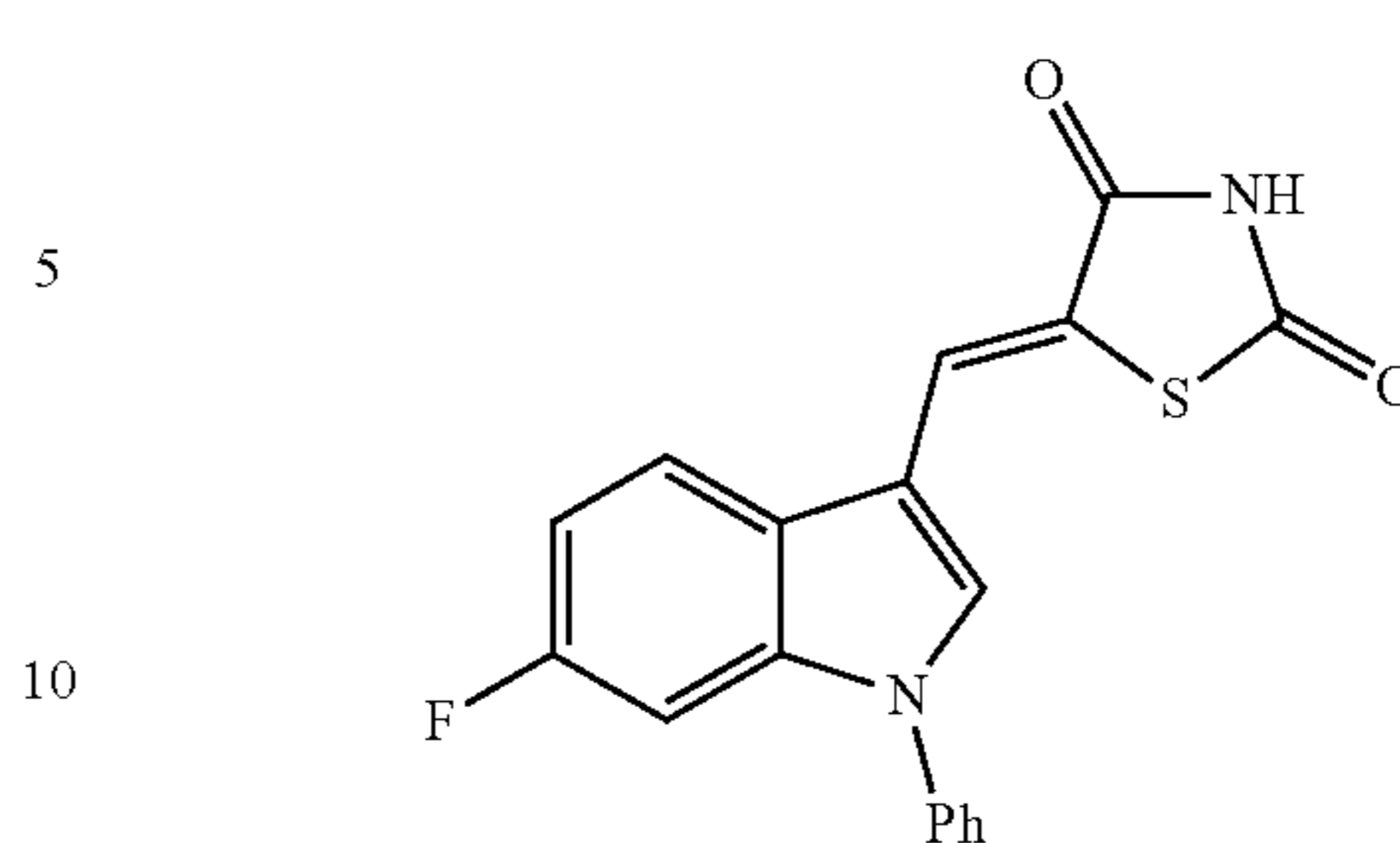
(Z)-5-((6-Fluoro-1-phenyl-1H-indol-3-yl)methylene)thiazolidine-2,4-dione (JXL071)
