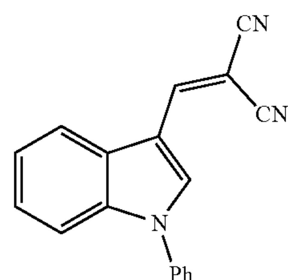
2-((1-Phenyl-1H-indol-3-yl)methylene)malononitrile (JXL021)
