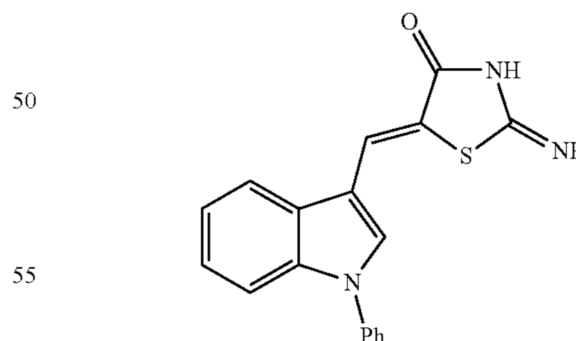
(Z)-2-Imino-5-((1-phenyl-1H-indol-3-yl)methylene)thiazolidin-4-one (JXL023)
