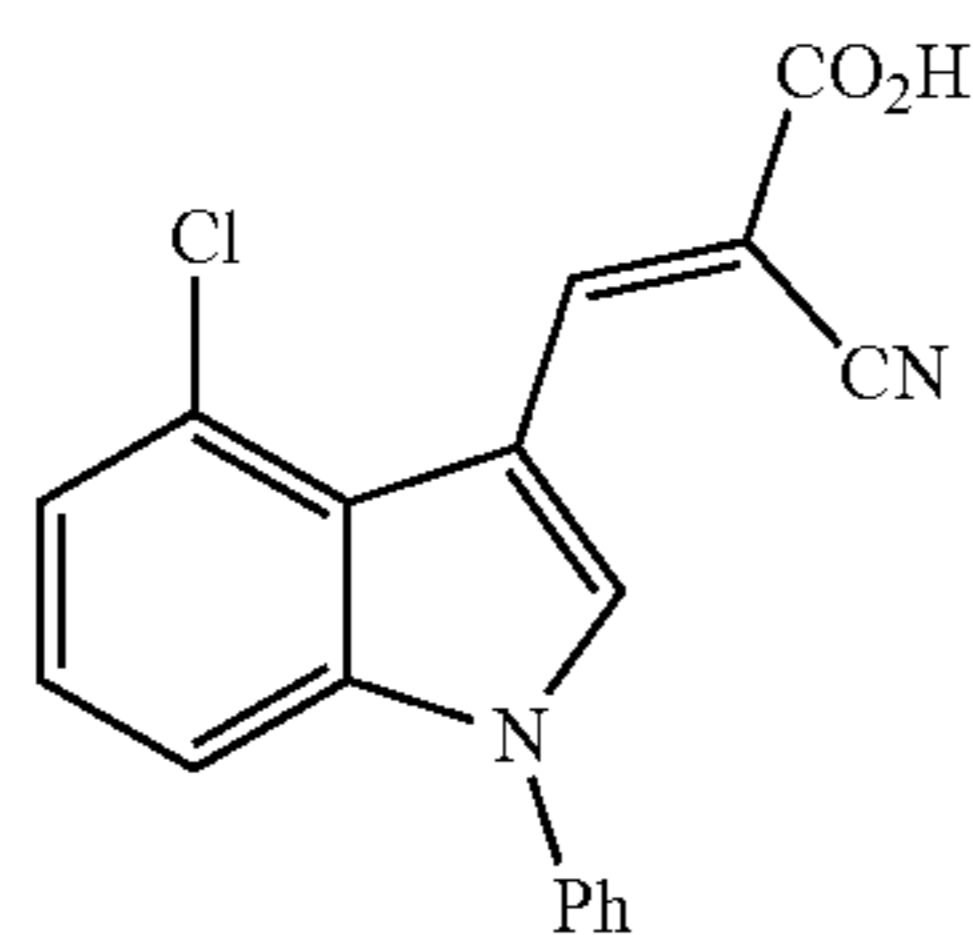
(E)-3-(4-Chloro-1-phenyl-1H-indol-3-yl)-2-cyanoacrylic acid (JXL035)
