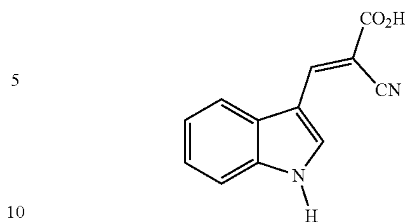
(E)-2-Cyano-3-(1H-indol-3-yl)acrylic Acid (JXL002)
