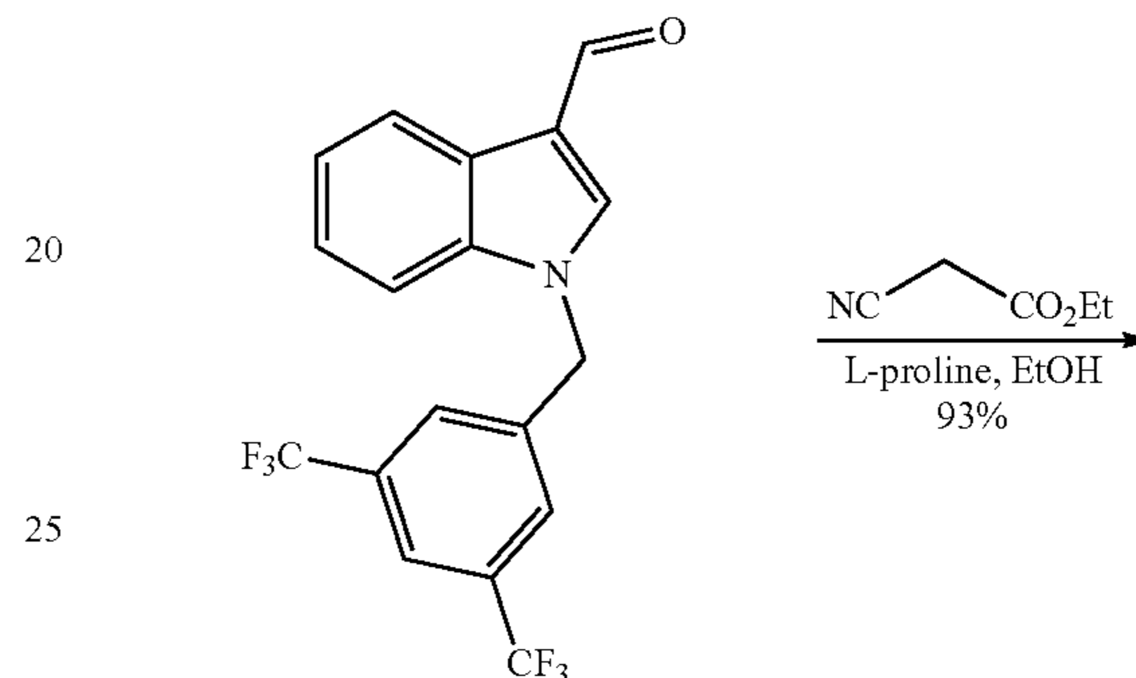
(E)-2-Cyano-3-(5-fluoro-1-phenyl-1H-indol-3-yl)acrylic Acid (JXL029)
