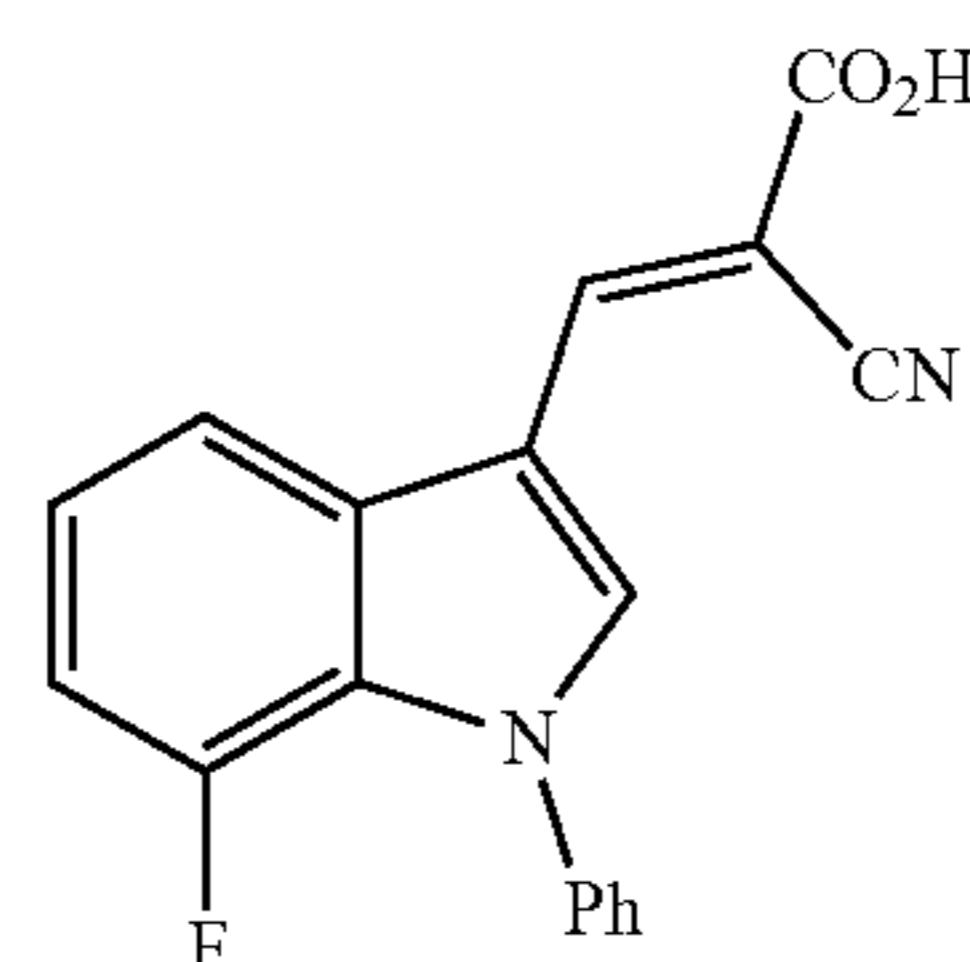
(E)-2-Cyano-3-(7-fluoro-1-phenyl-1H-indol-3-yl) acrylic Acid (JXL028)
