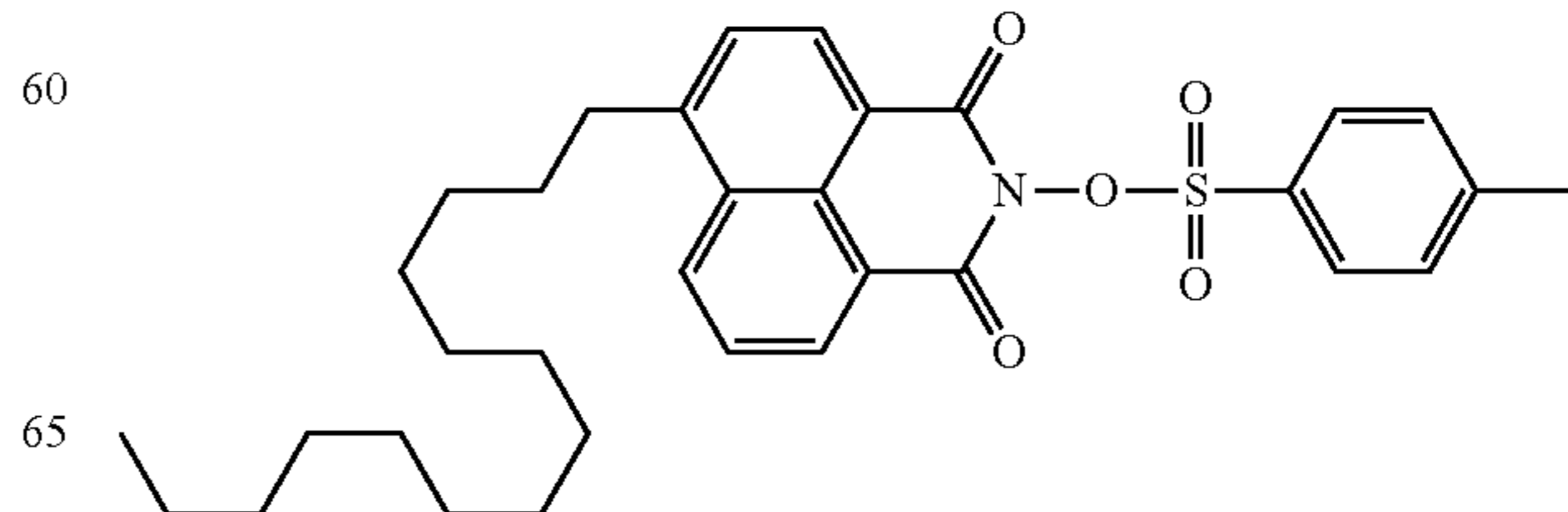
Compound No.32
