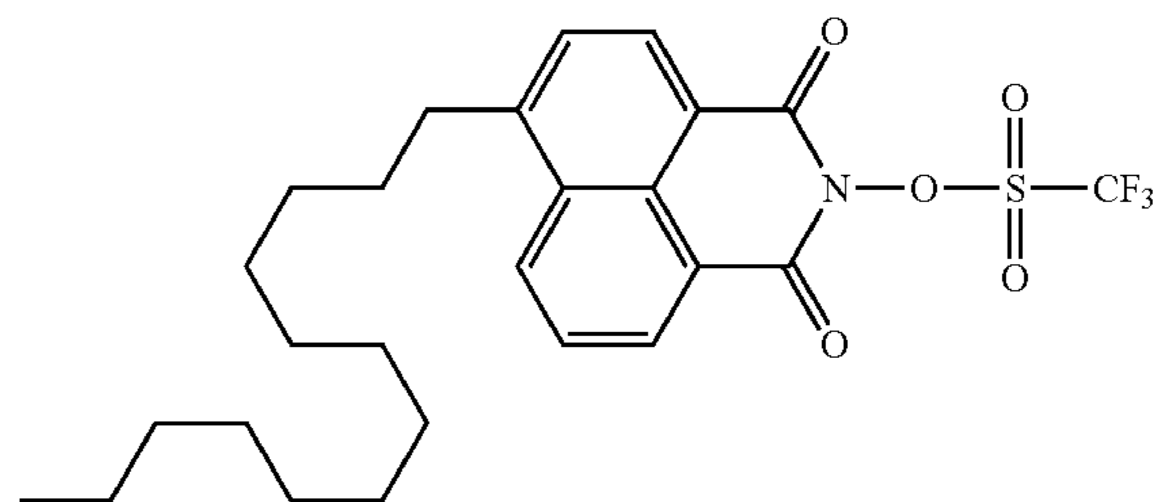
Compound No.24
