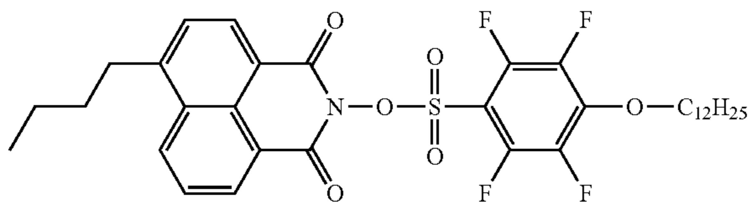
Compound No.18
