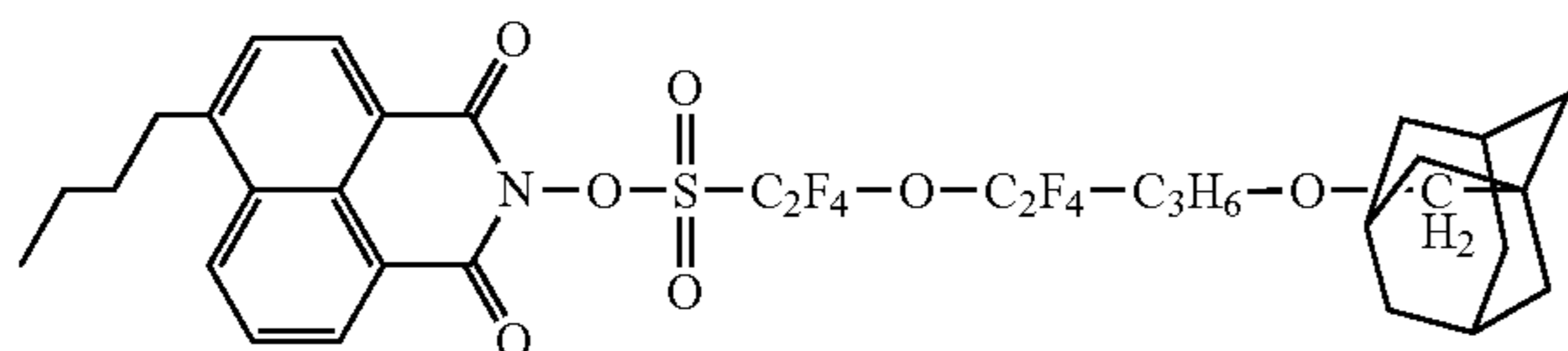
Compound No.17
