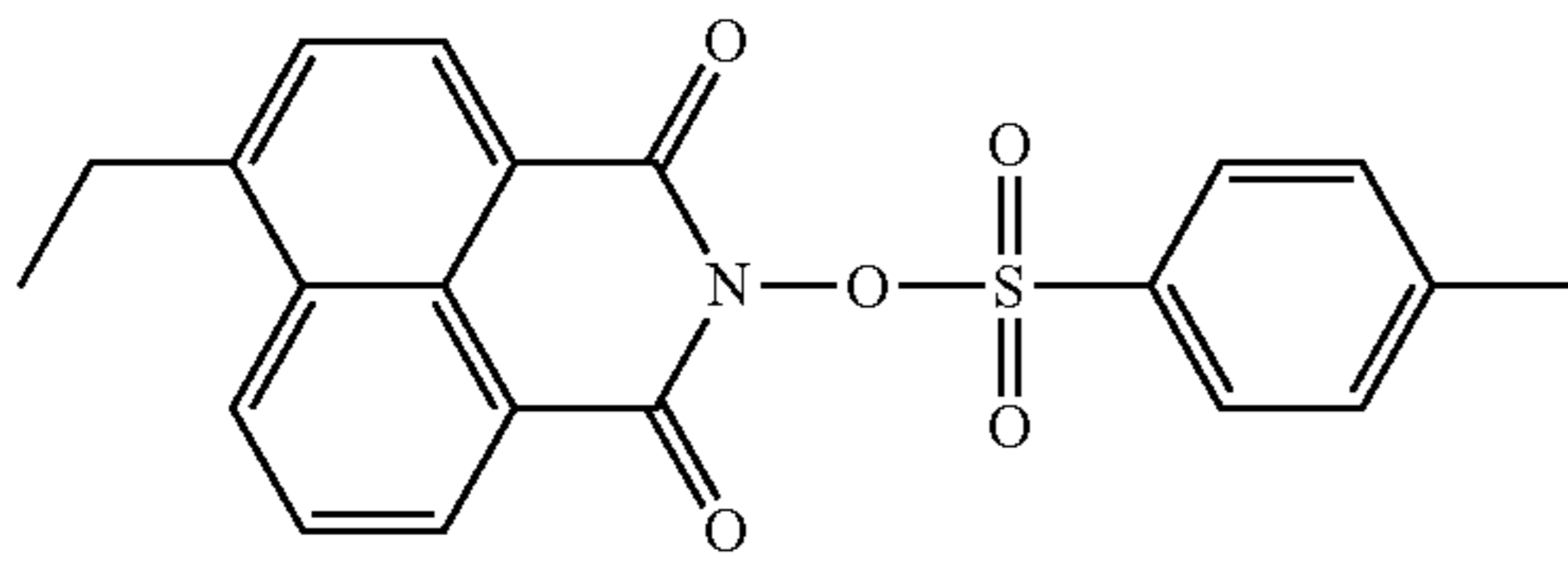
Compound No.42
