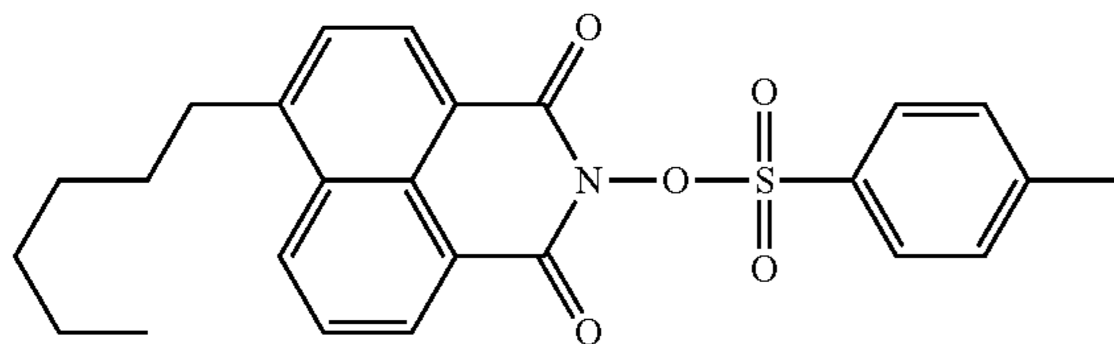
Compound No.44
