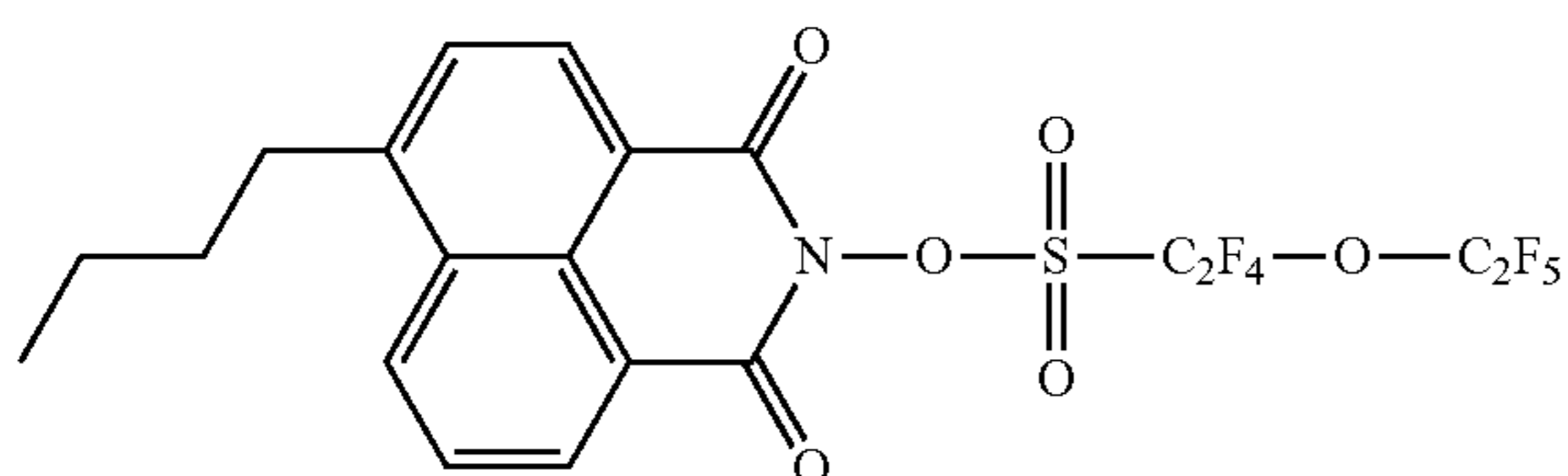
Compound No.14
