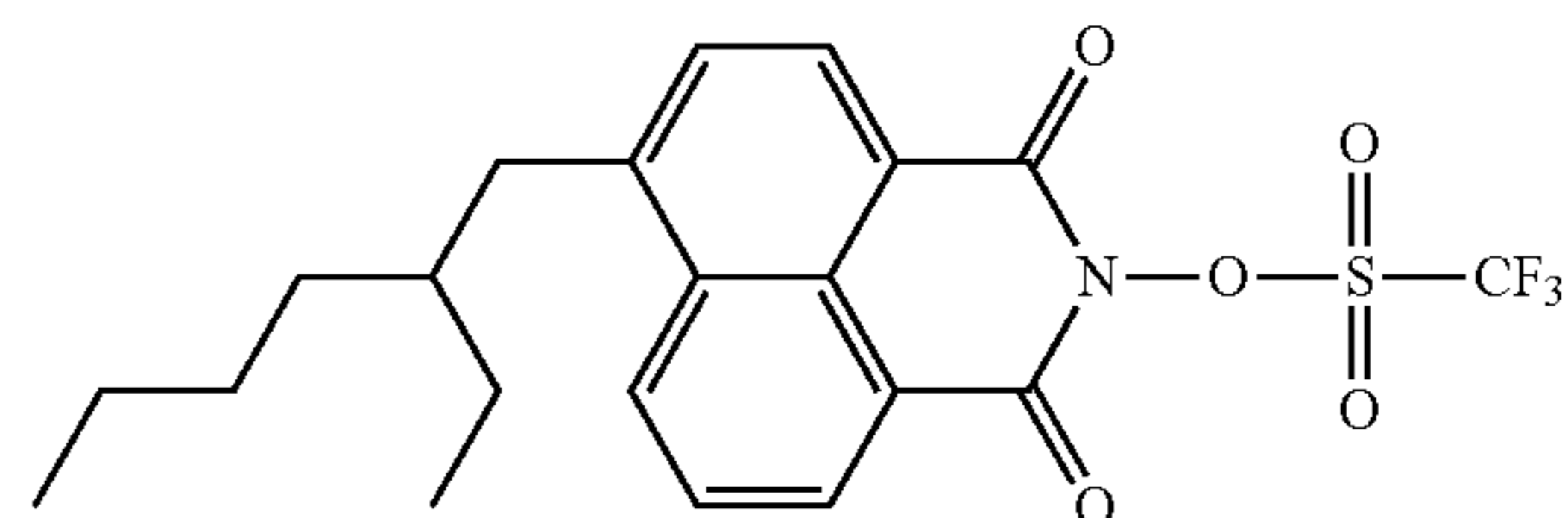
Compound No.23
