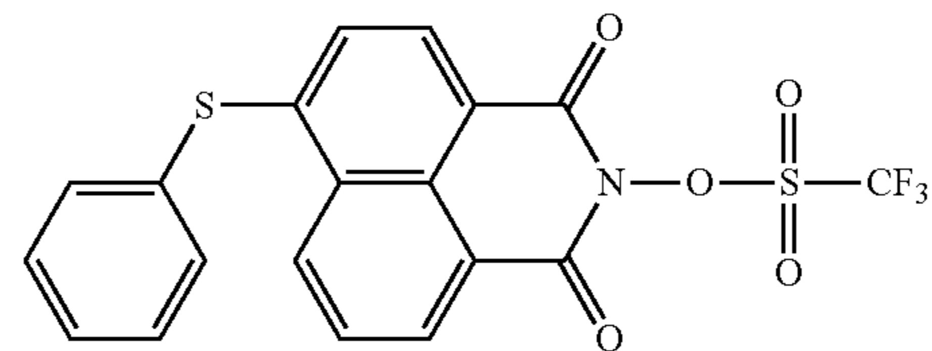
Compound No.53
