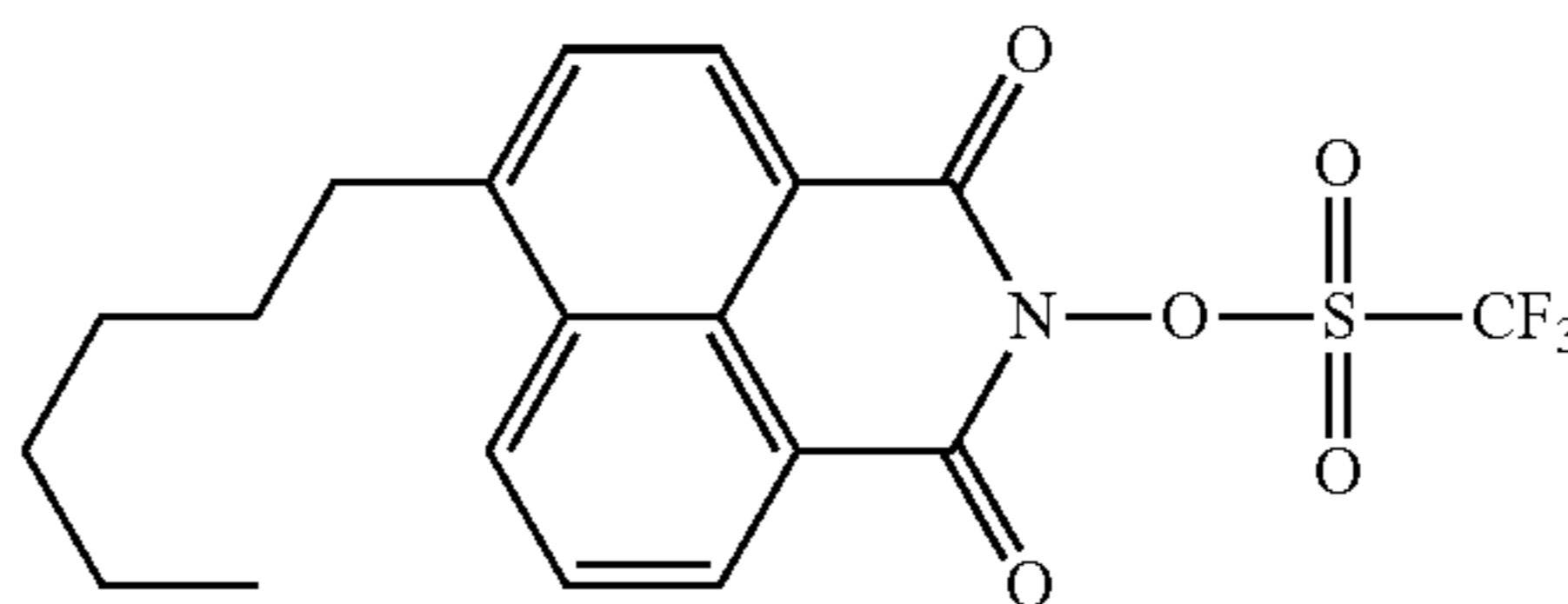
Compound No.21
