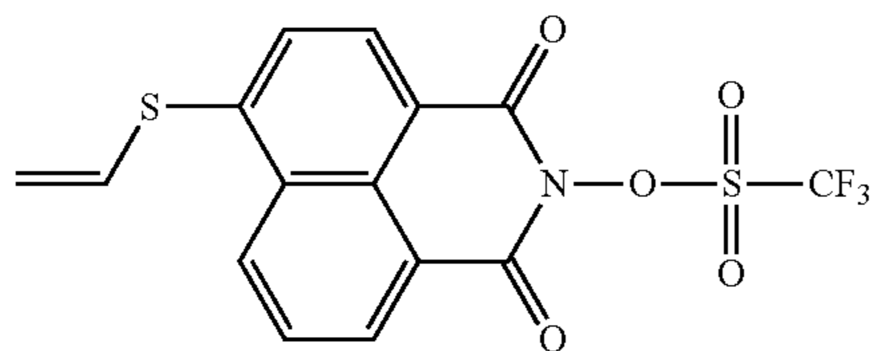
Compound No.58
