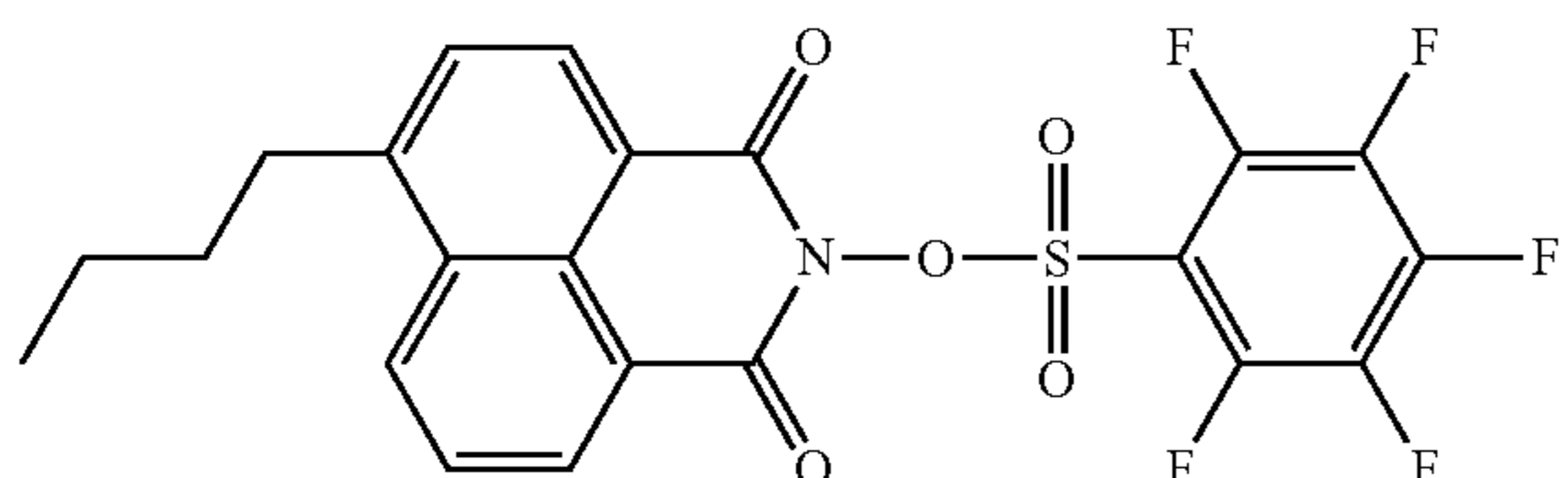
Compound No.14
