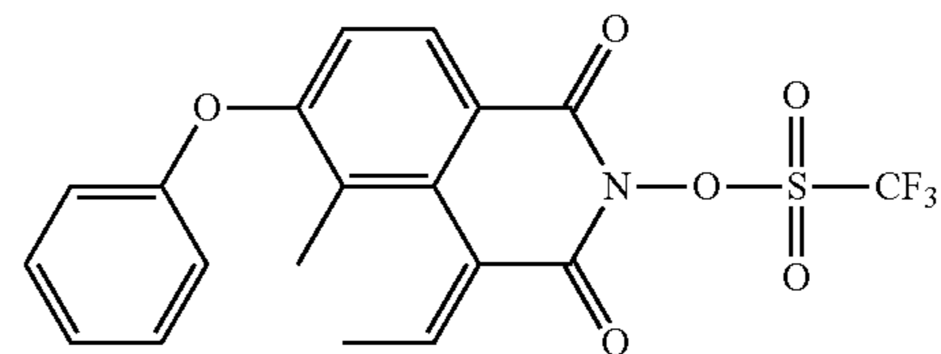
Compound No.52
