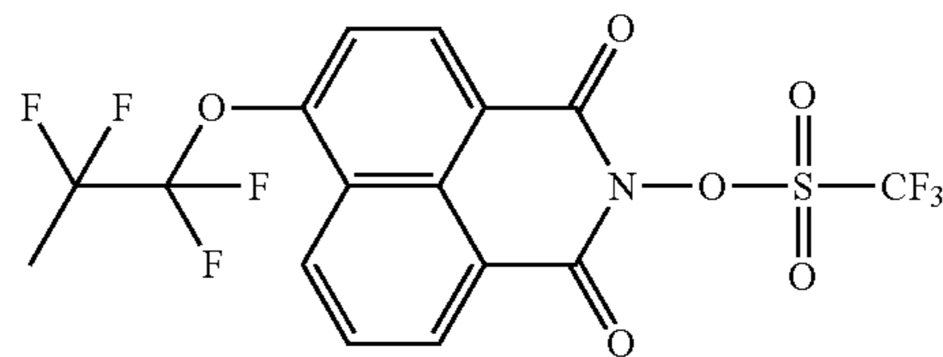
Compound No.51
