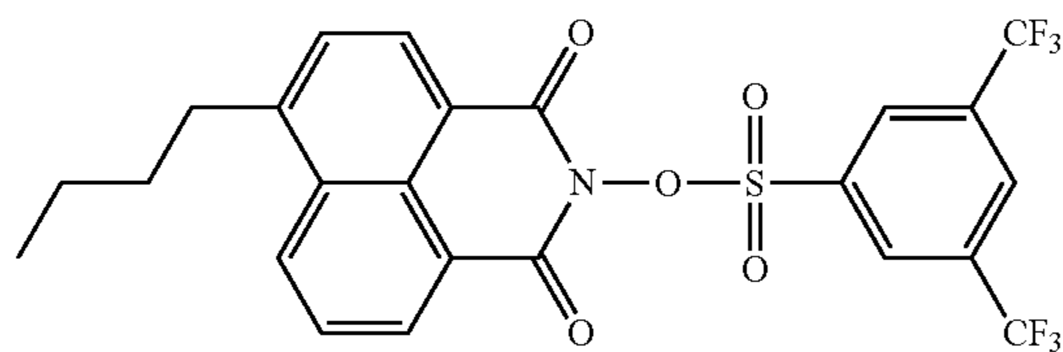
Compound No.12
