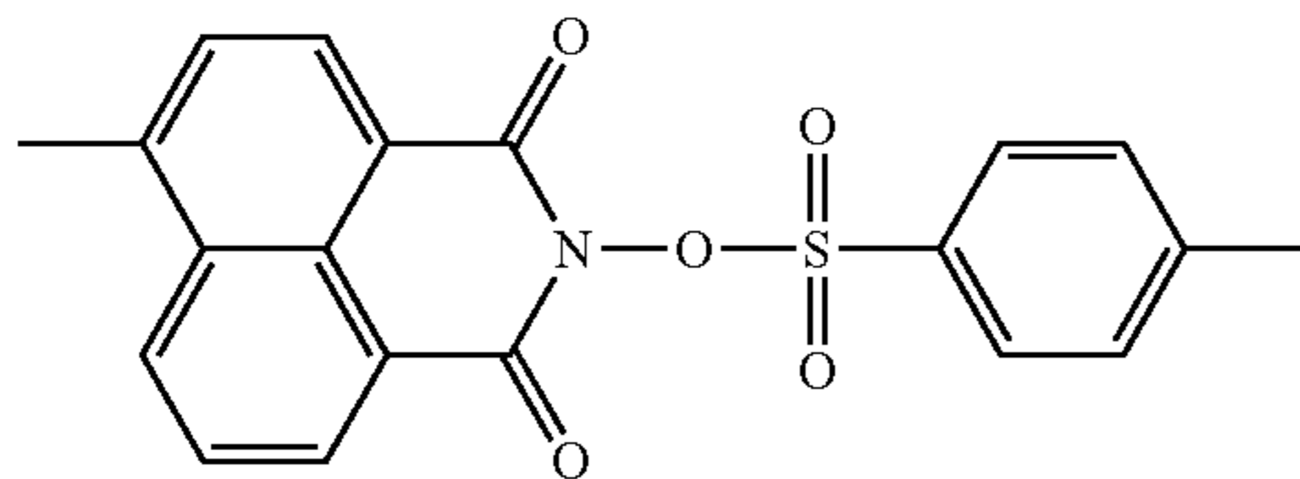
Compound No.43
