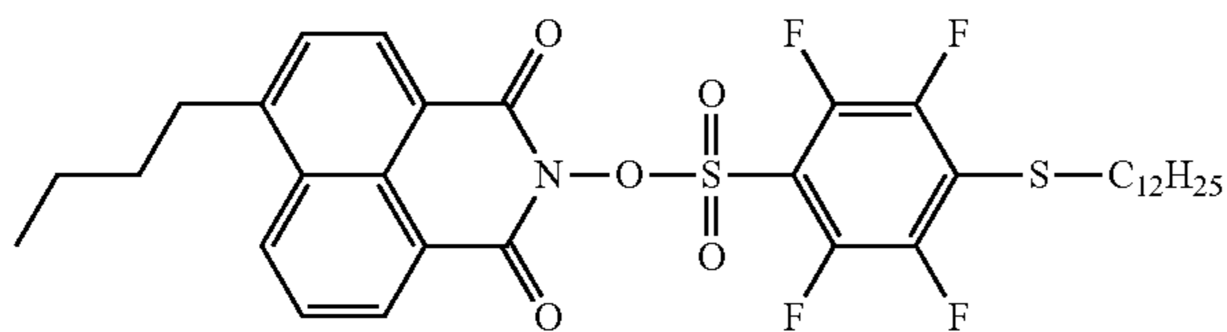
Compound No.18
