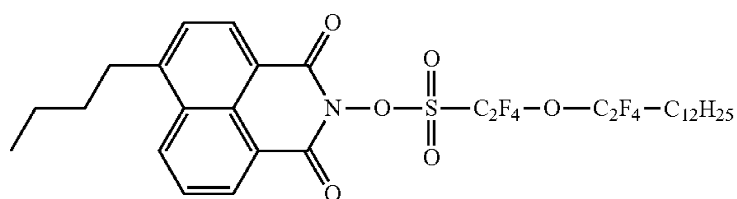
Compound No.16
