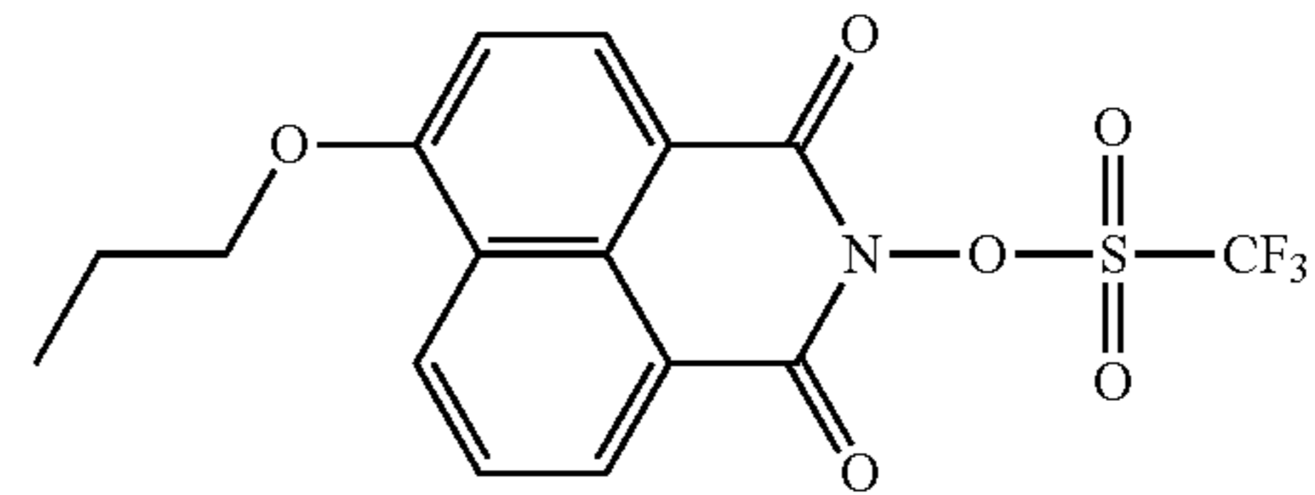
Compound No.49
