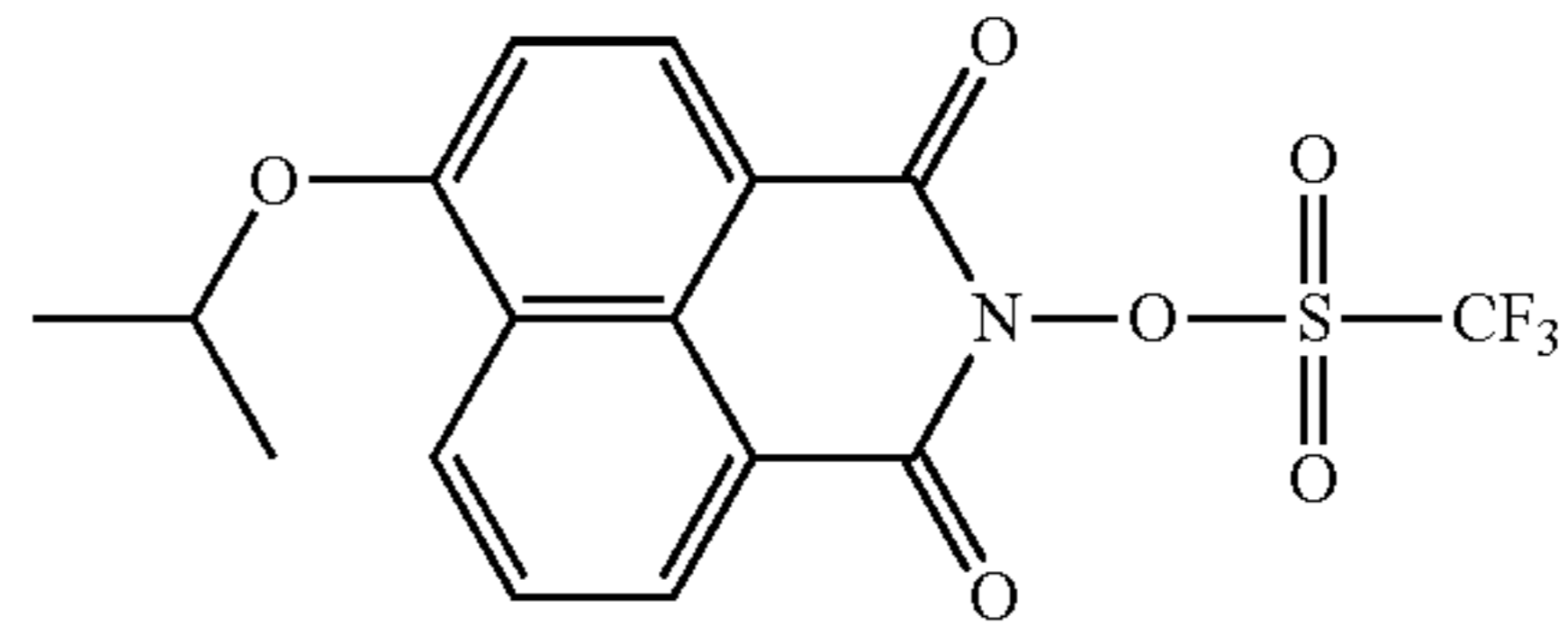
Compound No.49
