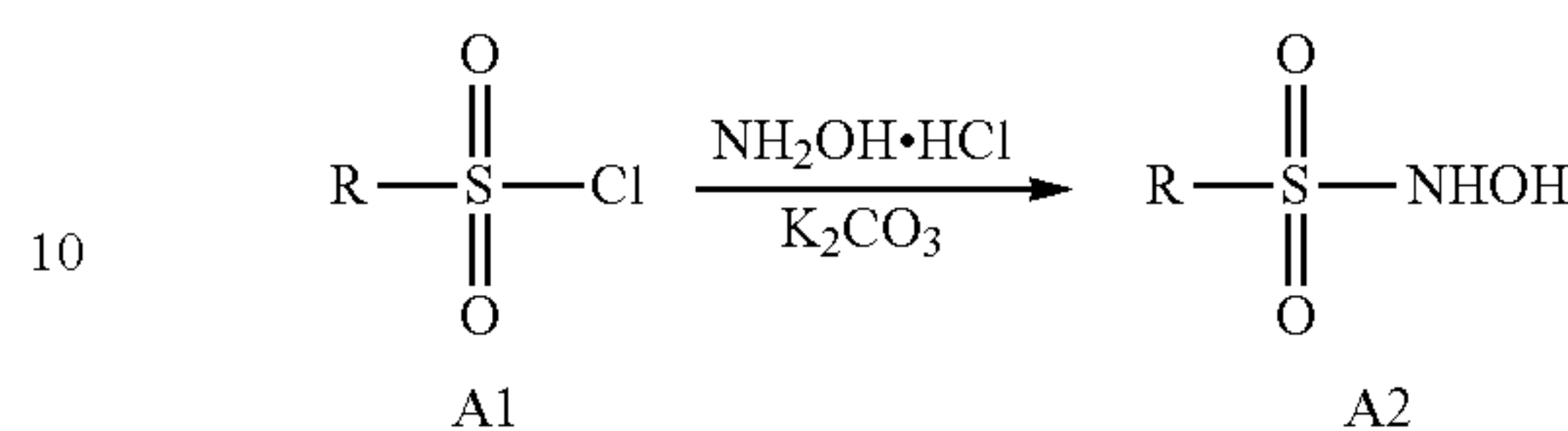
Scheme A. General Synthesis of N-Hydroxysulfonamides.
