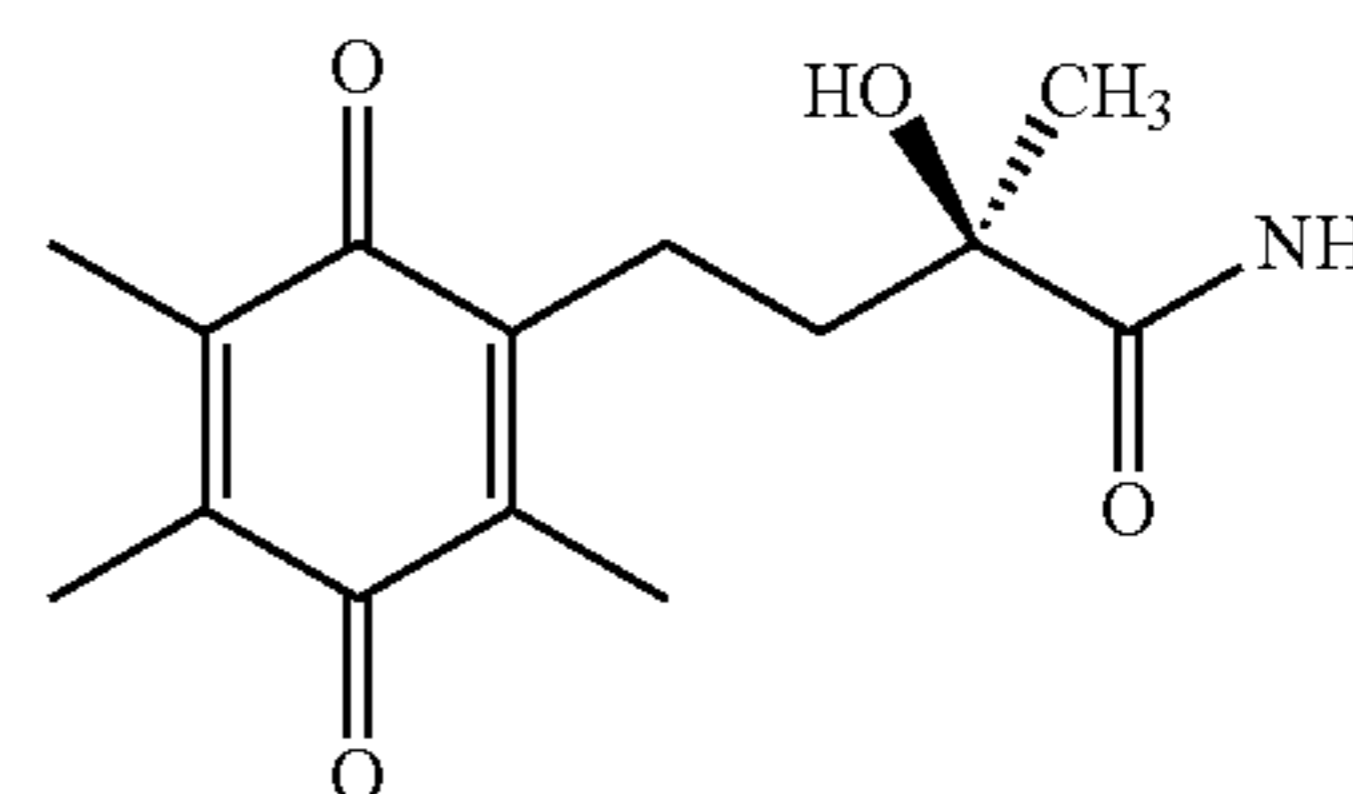
(R)-2-hydroxy-2-methyl-4-(2,4,5-trimethyl-3,6-dioxocyclohexa-1,4-dienyl)butanamide
