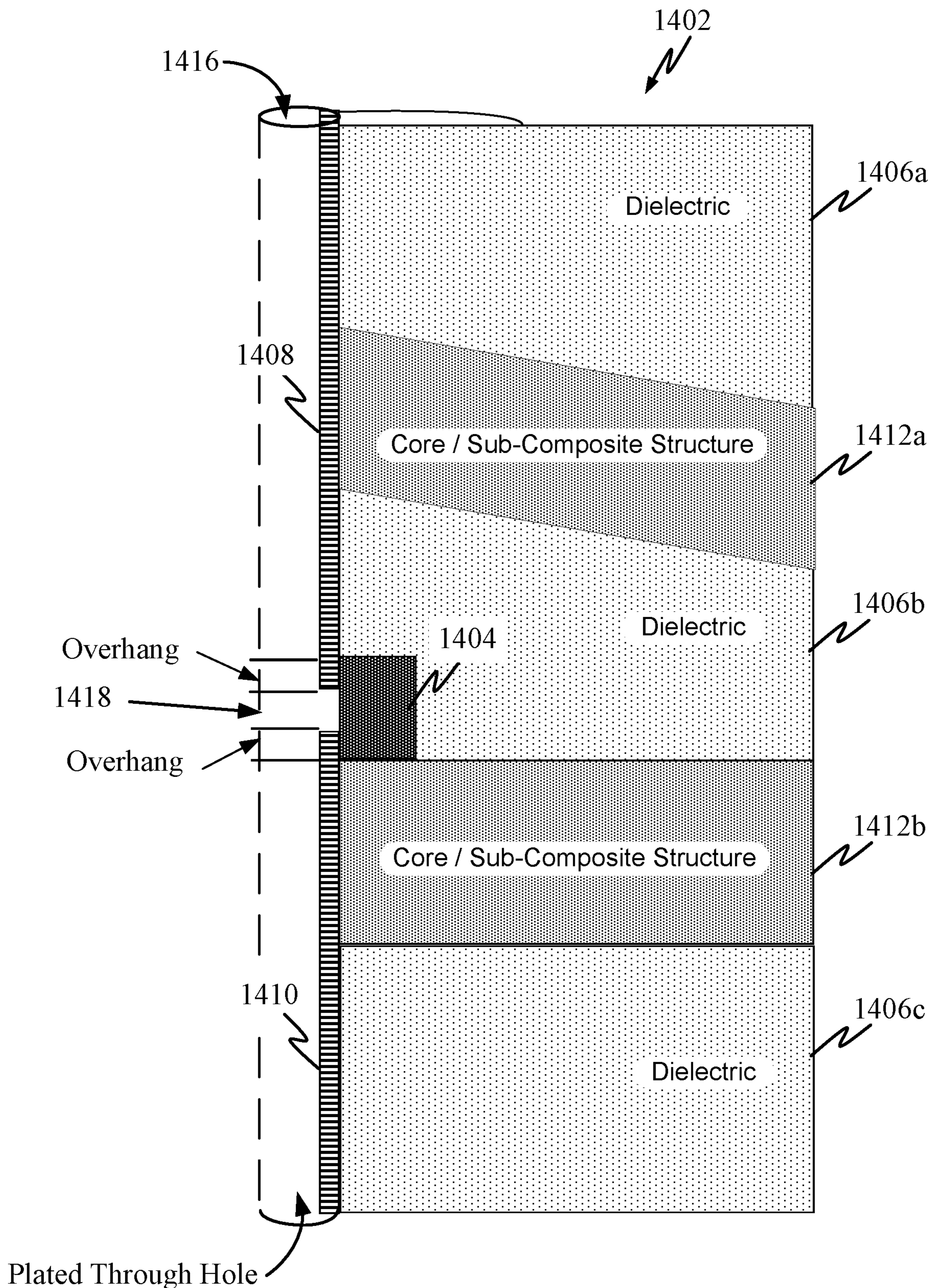
FIG. 14 (Practical Structure)
