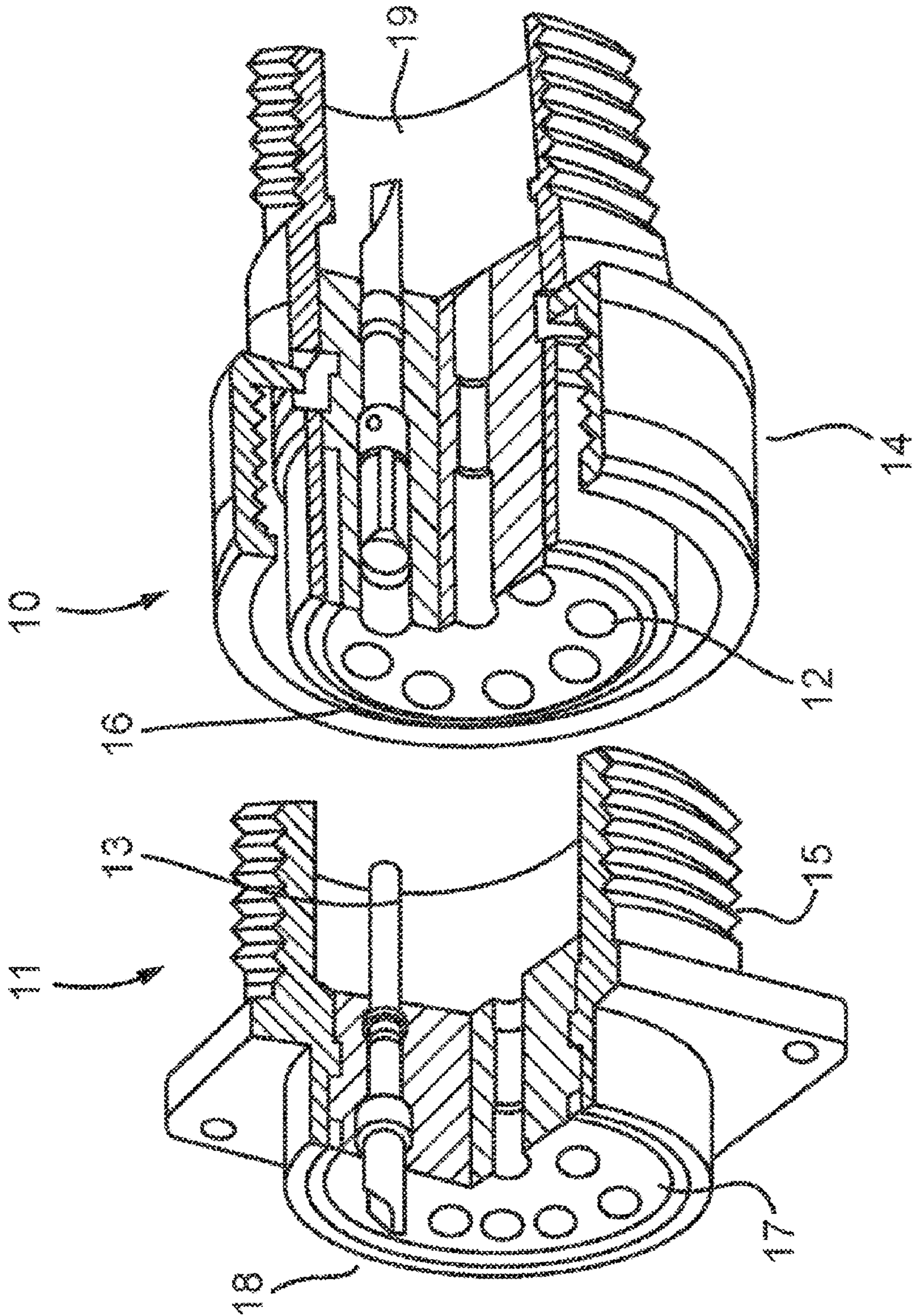
Figure 1 (PRIOR ART)
