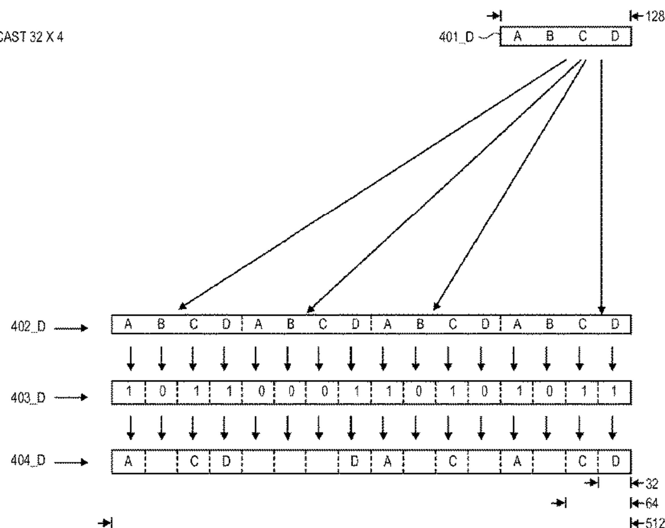
VBROADCAST 64 X 2
