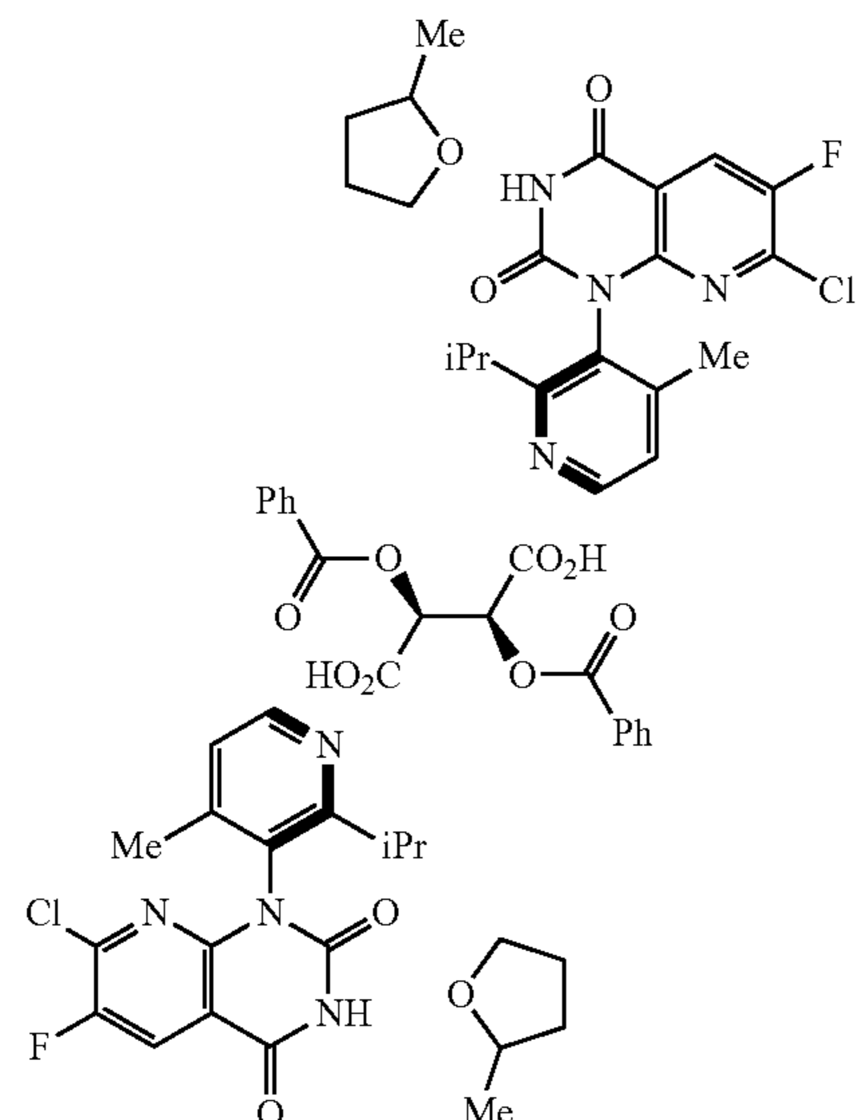
M-Dione/DBTA/2-MeTHF cocrystal 4a
