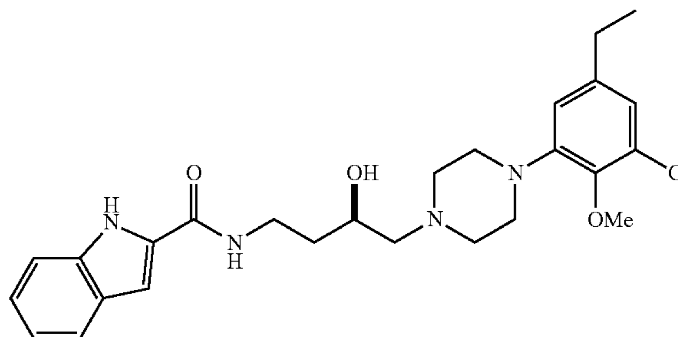
(R)-N-(4-(4-(3-chloro-5-ethyl-2-methoxyphenyl)piperazin-1-yl)-3-hydroxybutyl)-1H-indole-2-carboxamide ((R)-29
