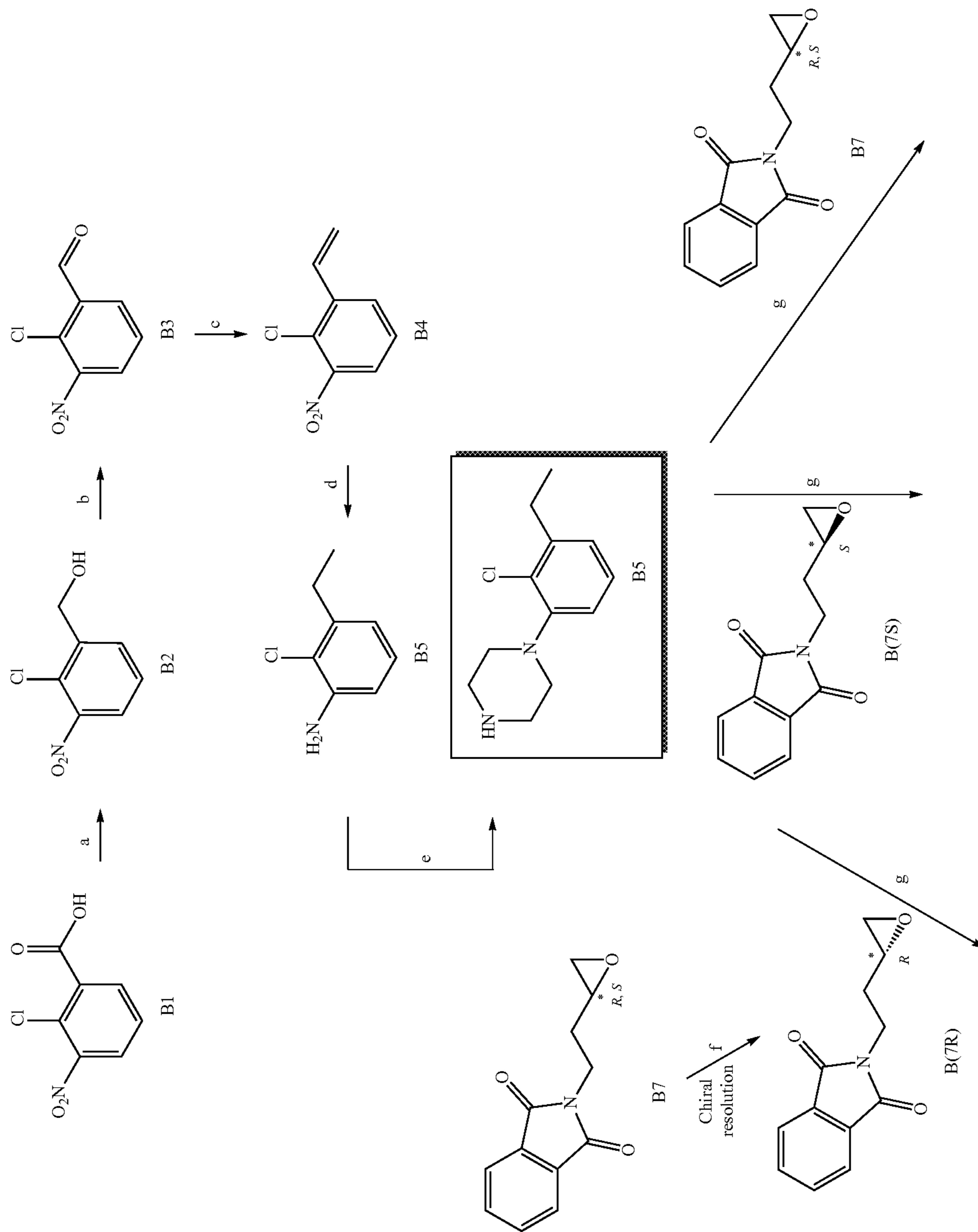
Scheme 2. Synthesis of (±), (R), and (S)-19
