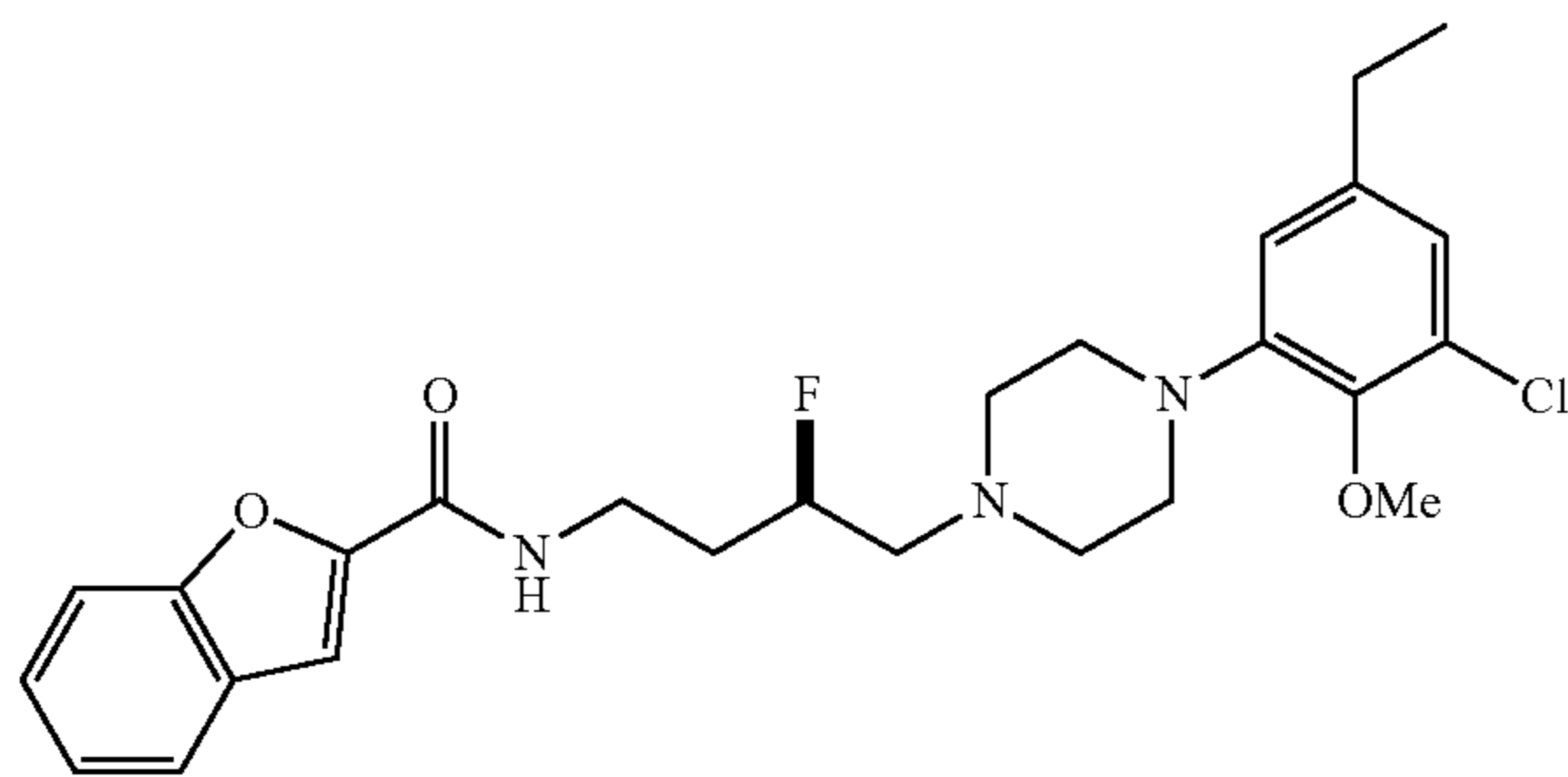
(R)-N-(4-(4-(3-chloro-5-ethyl-2-methoxyphenyl)piperazin-1-yl)-3-fluorobutyl)benzofuran-2-carboxamide
